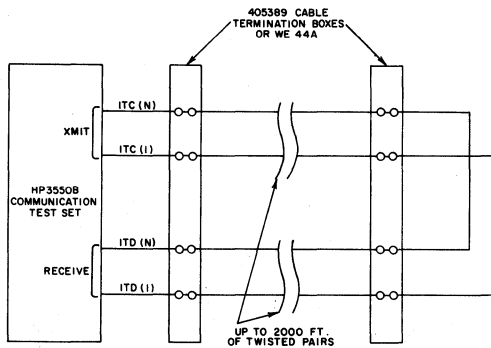
Fig. 21—Loop-loss Measurements
