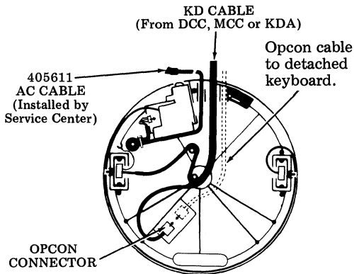
Fig. 2—Removal of Opcon Cable
