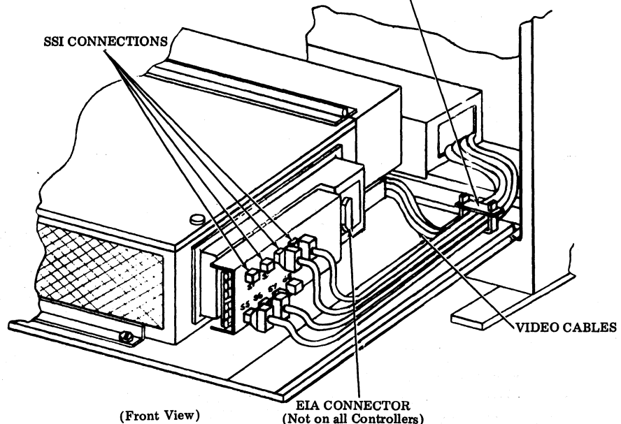
Fig. 7—Typical Controller Interconnection
