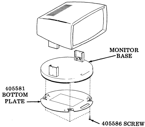
Fig 1.—Monitor Base Removal
