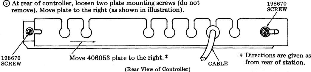
(Rear View of Controller)
