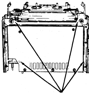
402539 IMMOBILIZATION SCREWS (4 Places)
