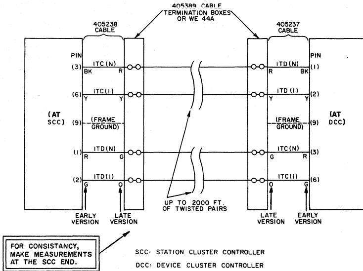
Fig. 18—DC Tests On Cable Pairs Between SCC & DCC
