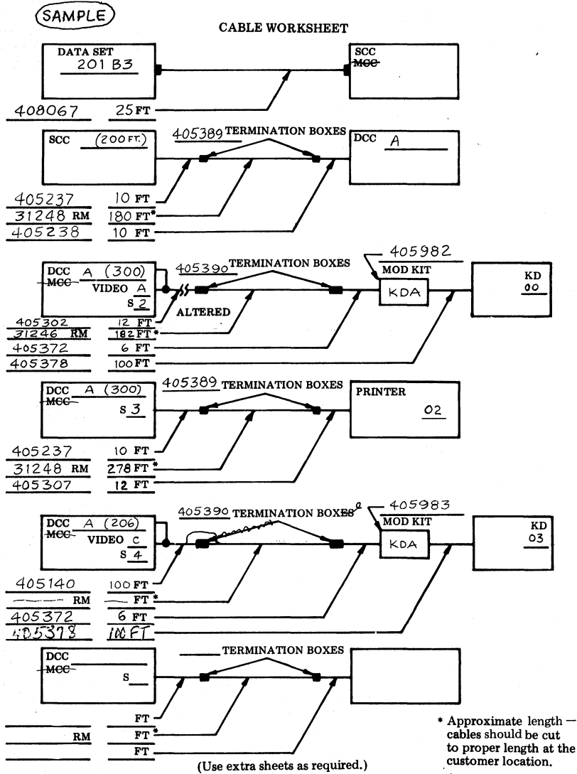
Fig. 5—Sample Cable Worksheet
