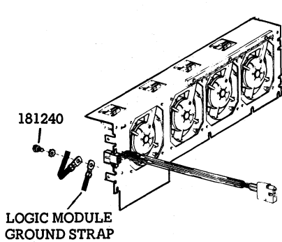
Fig. 4—Ventilation Assembly Detail
