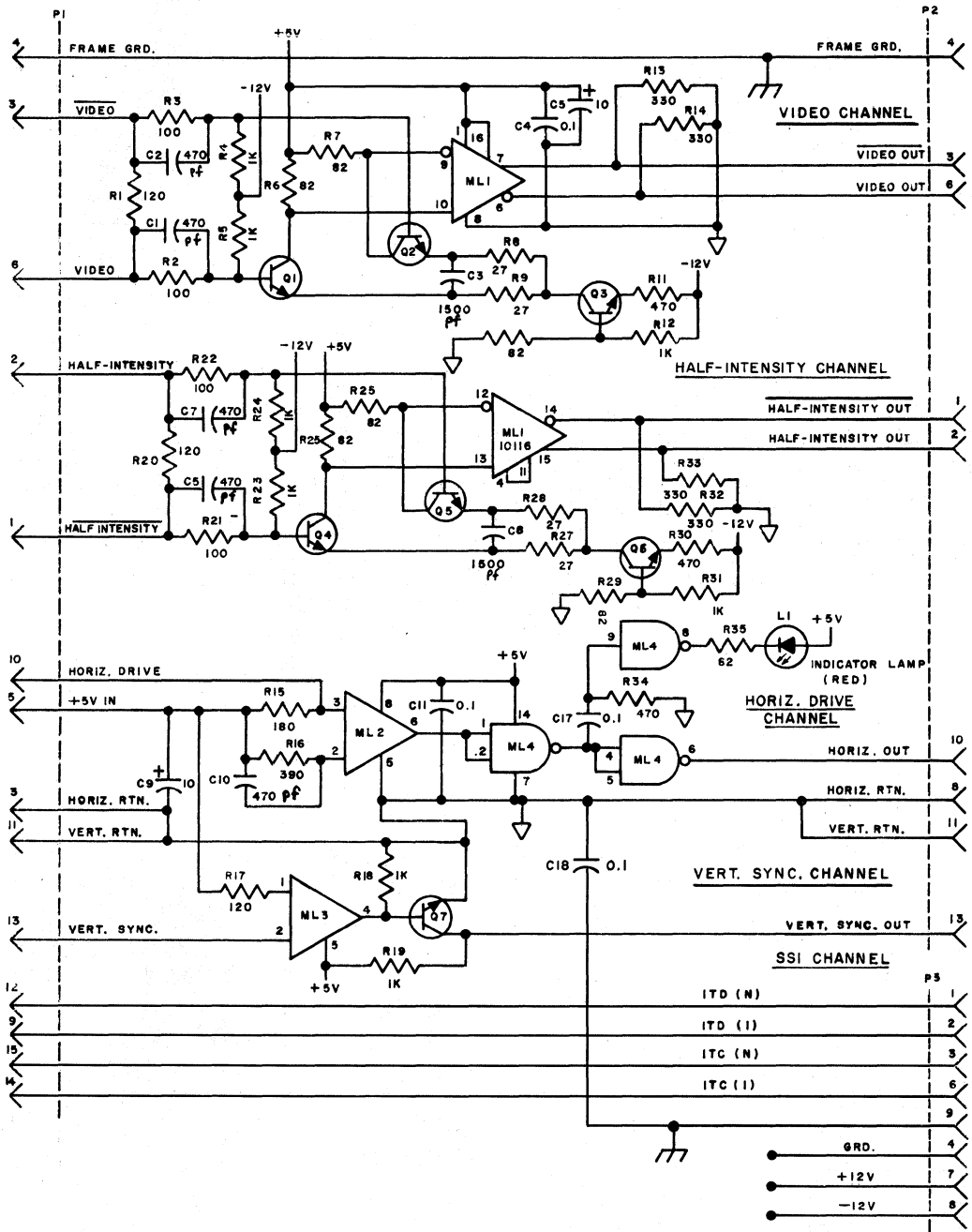
Fig. 10—KDA Receiver Circuits
