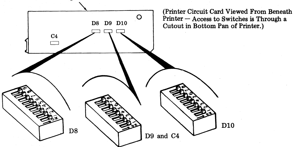
410072 Printer Logic Circuit Card
