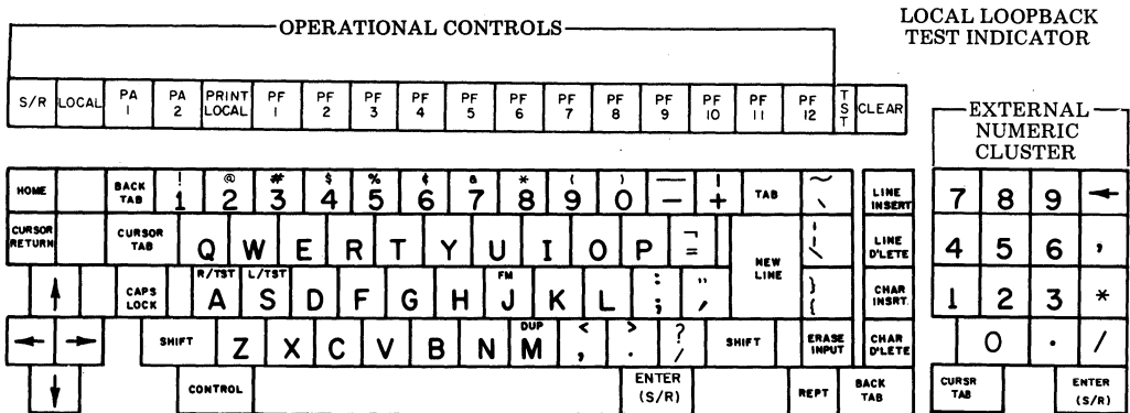
Fig. 5—Opcon Keytop Layouts (Cont)
