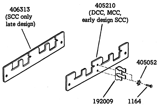
Fig. 5 – Clamp Plate Components (At Rear of Controller)
