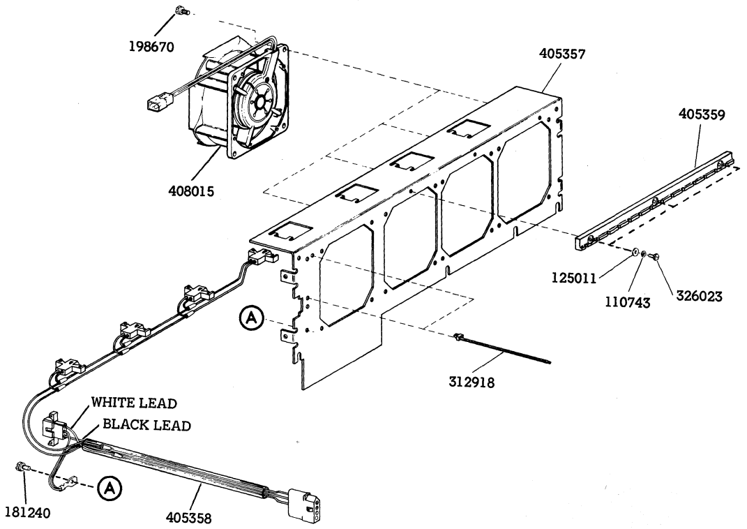
Fig. 2 - 405360 Ventilation Assembly Components
