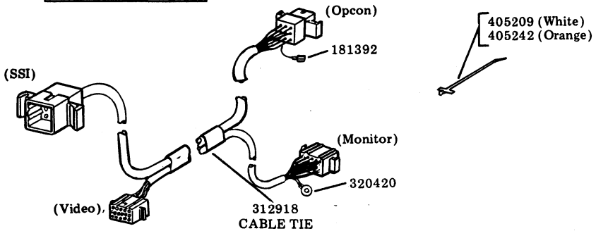
Fig. 16—40KDA to KD Cable Assemblies
