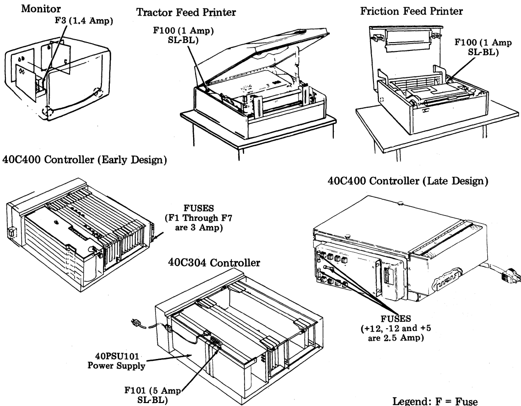
Fig. 4—Fuse Locations
