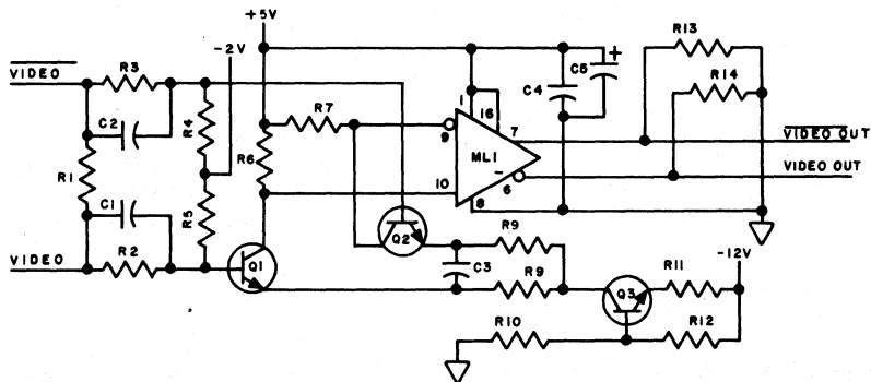
Fig. 3—Video Amplification
