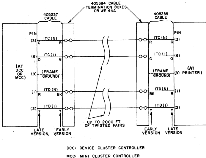
Fig. 19—DC Tests On Cable Pairs Between DCC (Or MCC) & Printer
