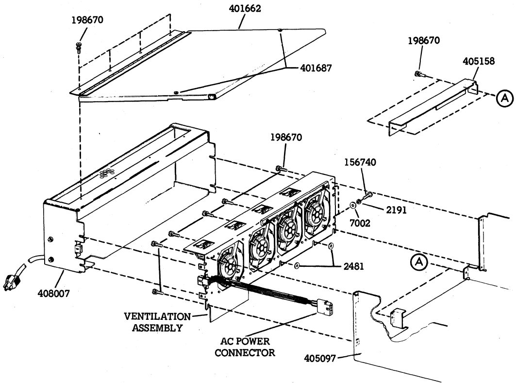
Fig. 3—Mounting Hardware for Fan Guard, Ventilation Assembly, and Cover
