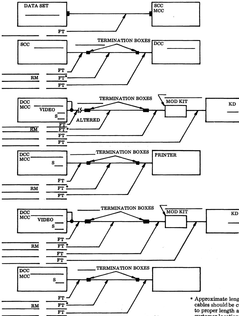
Fig. 6—Blank Cable Worksheet
