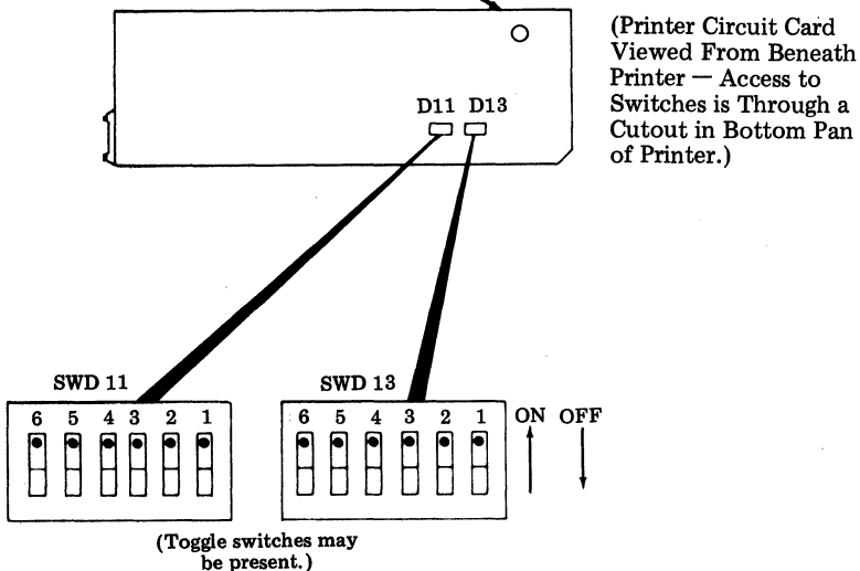
410729 — Printer Logic Circuit Card
