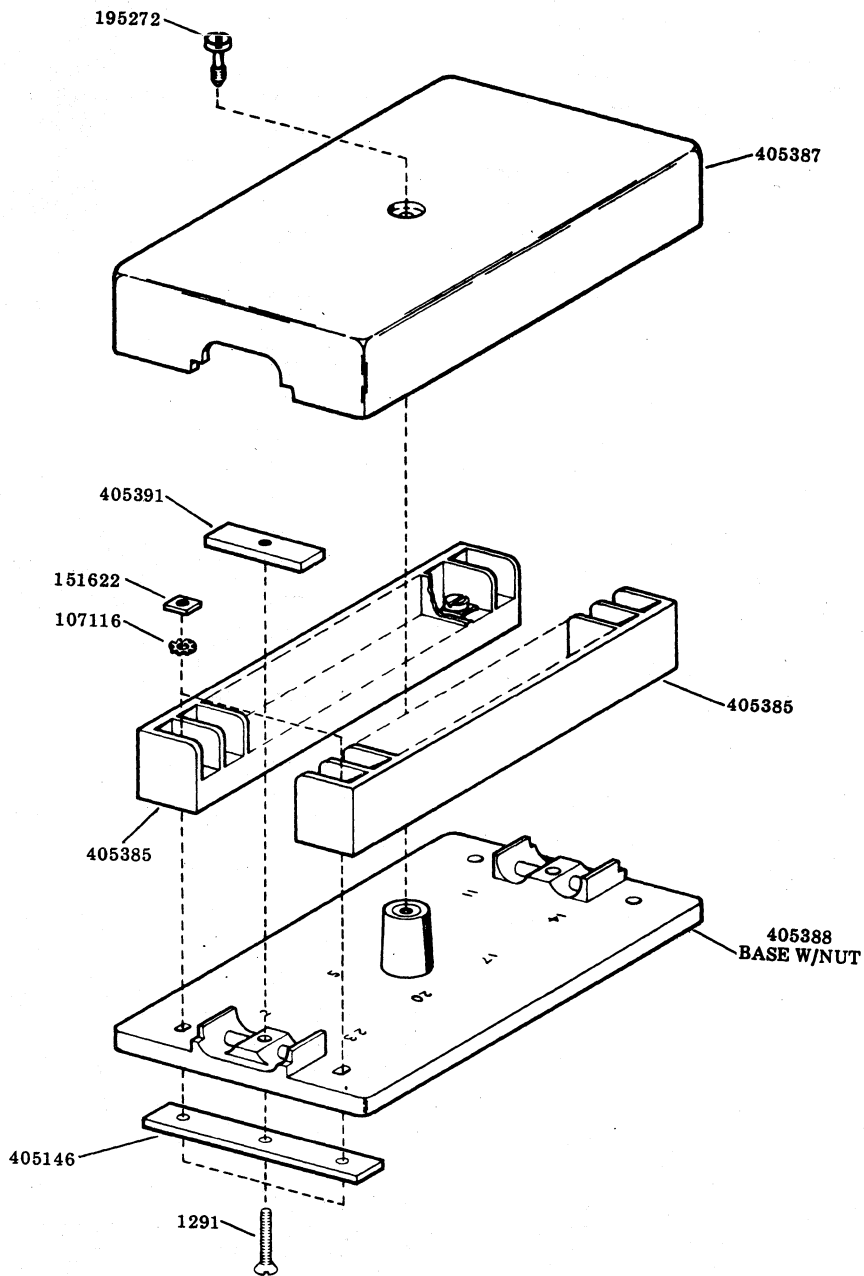
Fig. 17—405390 Cable Termination Box (24 Position)
