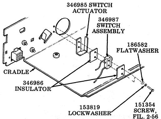
Fig. 10—Installation of Switch Actuator
