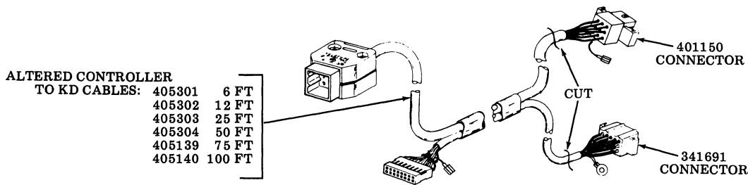
Fig. 8— Controller to KD Cable Alteration
