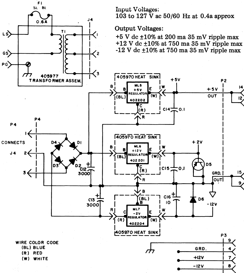
Fig. 7—Power Supply
