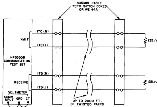
Fig. 20—Cross-talk Measurements
