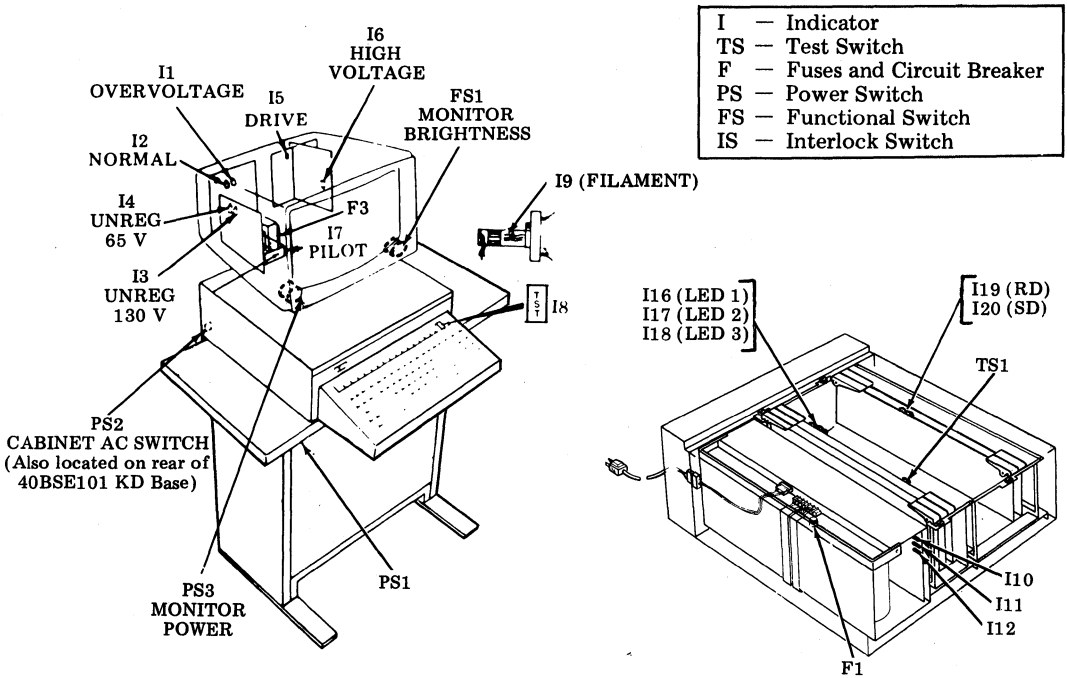
Fig. 1—Test Switches and Indicators (Controller and KD)
