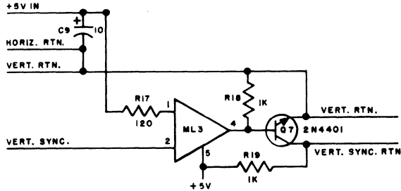
Fig. 5—Vertical Channel Signals
