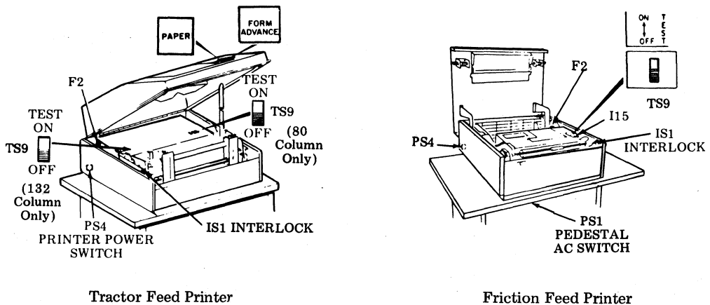
Fig. 2—Test Switches and Indicators (Printer)
