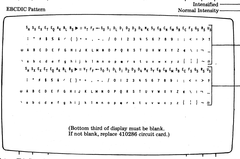
Fig. 3—Self-Test Mode Displays
