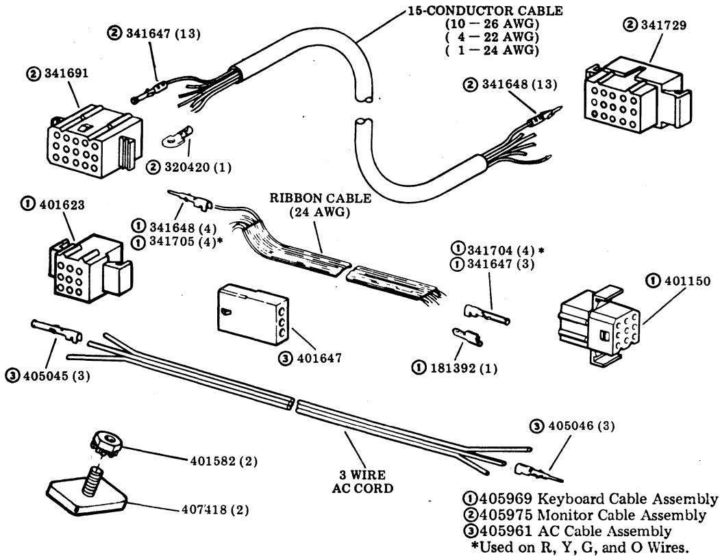
Fig. 14—405983 Modification Kit (Cabinet Mounting)
