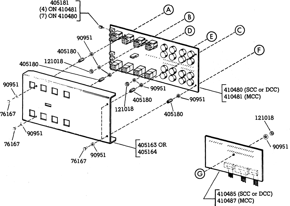
Fig. 6—405150, 405151, and 405152 Interconnection Modules
