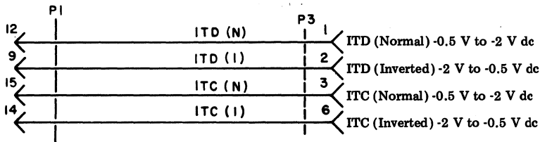
Fig. 6—SSI Transmission
