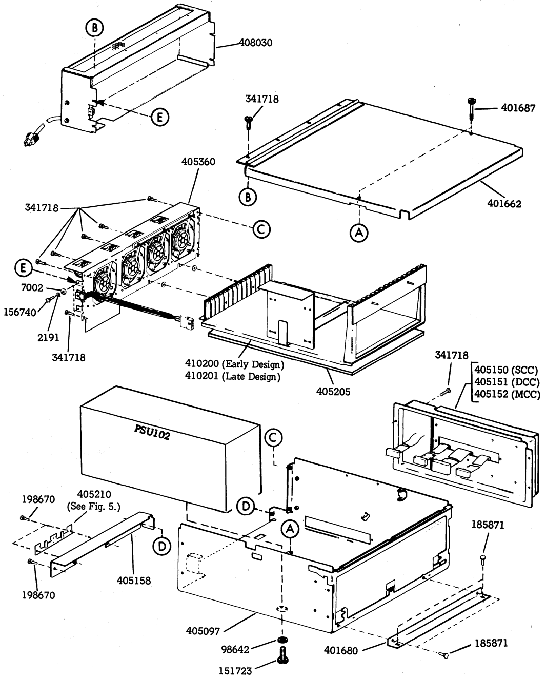
Fig. 1—Overview of Controller Components
