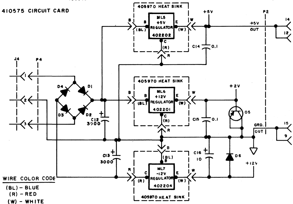
Fig. 9—Power Diagram
