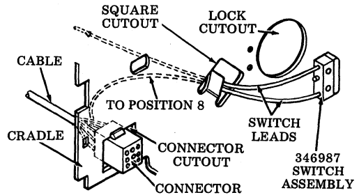
Fig. 9—Installation of Switch
