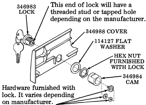
Fig. 7—Lock Cover Assembly
