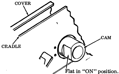
Fig.11—Direction of Cam When Inserted in Cradle
