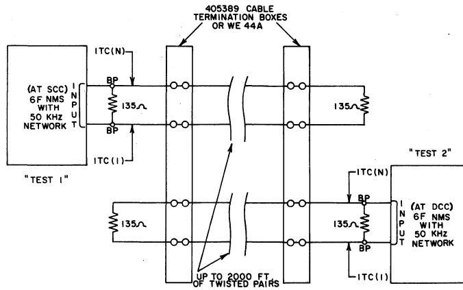
Fig. 22—Noise Measurements
