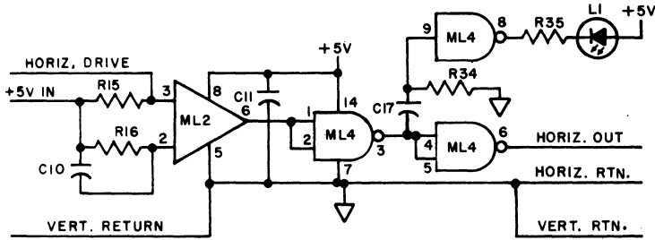
Fig. 4—Horizontal Drive Input
