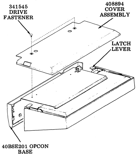
Fig. 4—408894 Cover and Opcon Base Removal
