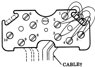
WE44A CONNECTOR BLOCK
