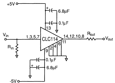
Figure 1: Recommended Circuit
