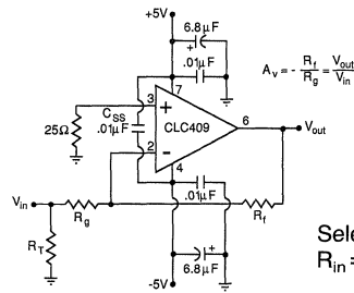
Figure 2: recommended inverting gain circuit
