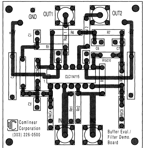
Figure 2 Board Layout and Component Placement
