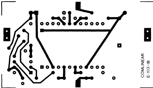
Figure 2: Component side (top), inverting
