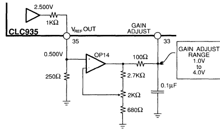
Analog Input Range Adjust Circuit
