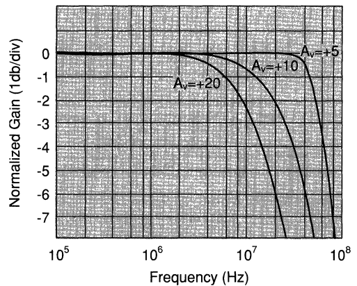
Figure 5: Small signal frequency response vs. gain ( I_{cc} = 1mA )
