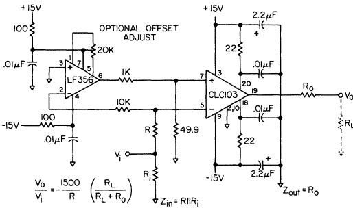
Figure 1: Inverting circuit with offset adjust circuitry
