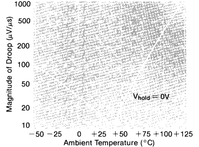
Droop Rate Magnitude vs. Temperature
