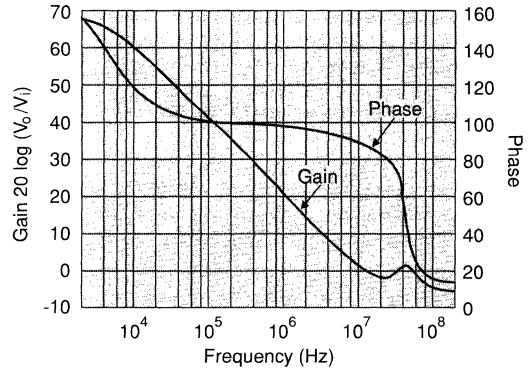
Figure 12: Integrator frequency response
