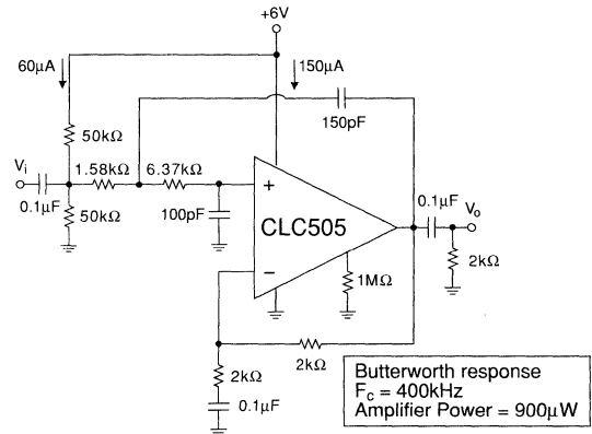
Figure 13: Single supply μpower active filter
