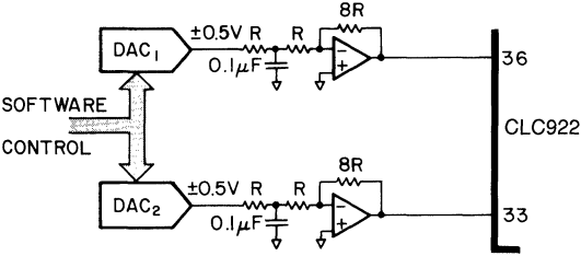
Simple DAC's provide Auto-cal Capability
