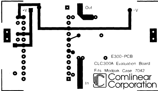
Figure 5: Component (top) side
