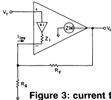
Figure 3: current feedback topology
