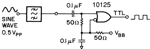
SINE to TTL Conversion Circuit
