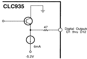
CLC935 Internal ECL Termination Circuit
