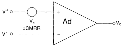
Figure 4: Input-referred common mode error model
