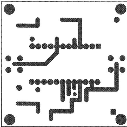
Figure 4: Bottom side metal (viewed from top side)
