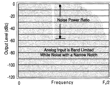
Figure 6: Typical Noise Power Ratio Spectrum
