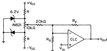
Non-Inverting
