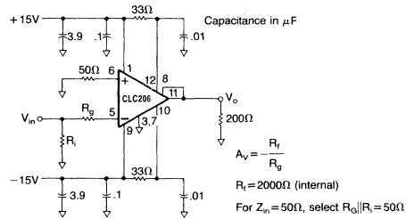
Figure 2: recommended inverting gain circuit
