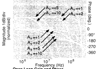
Open Loop Gain and Phase
