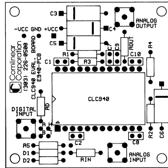
Figure 6: component placement guide
