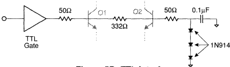
Figure 5D: TTL Interface
