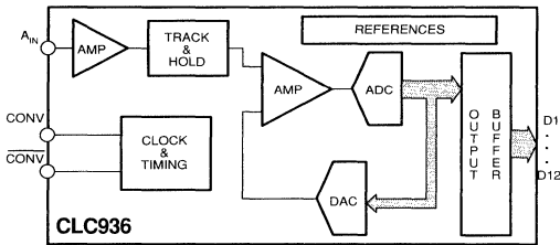
CLC936 Functional Block Diagram
