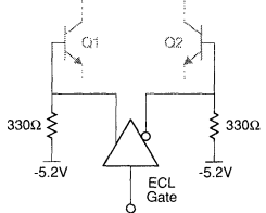
Figure 5B: Differential ECL Interface
