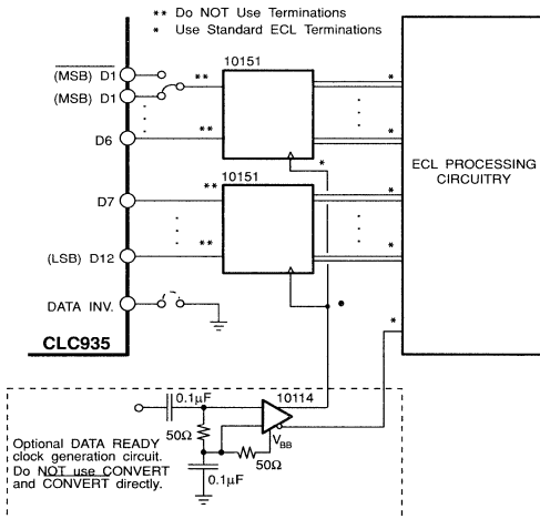
Recommended Output Buffering Circuits
