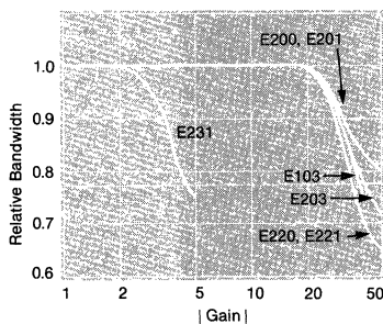
Relative Bandwidth vs. Gain
