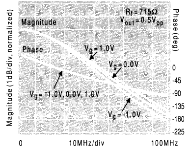
Frequency Response, A_{Vmax} = +100
