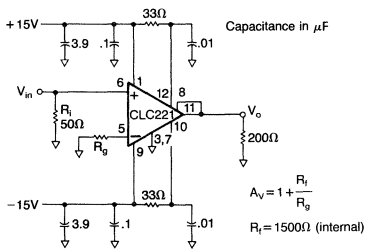
Figure 1: suggested non-inverting gain circuit
