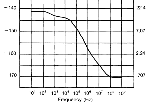
Noise Spectral Density
