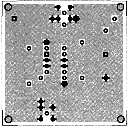
Figure 4: Component side (top) showing extensive ground plane
