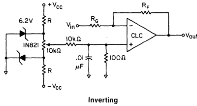
Inverting
