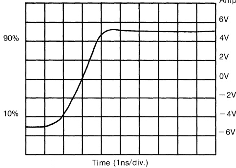
Pulse Response
