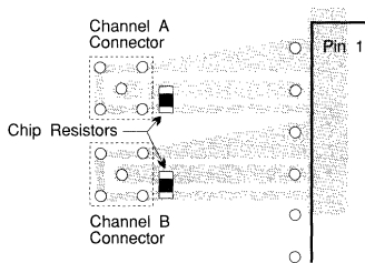
Figure 6: Alternate Layout Using Guard Ring
