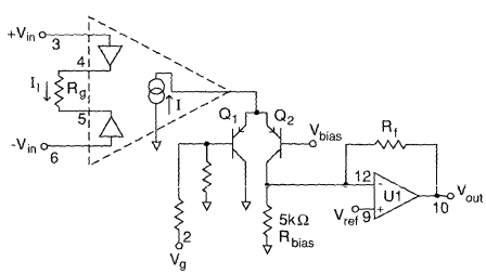
Figure 1: CLC520 Simplified Schematic
