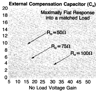
Figure 6: External Compensation Capacitance ( C_x )
