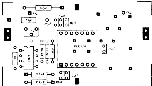
Figure 3: Component placement guide
