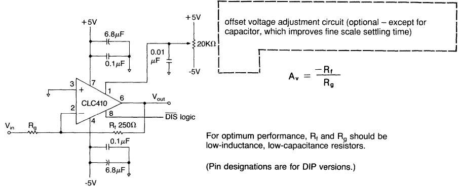
Figure 2: recommended inverting gain circuit
