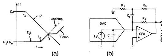
Fig. 10: DAC output capacitance compensation.
