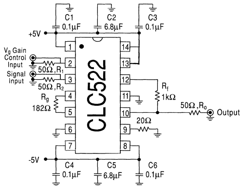
Figure 1: CLC522 typical application circuit
