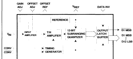
Block Diagram
