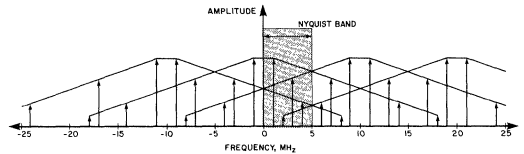
Figure 8: A complex signal having frequency components at 1MHz, 7MHz, 14MHz, and 18MHz is shown being sampled at 10MHz. The original spectrum is replicated at multiples of the sampling frequency. Note that the Nyquist band ( f_s/2 ) contains all of the original components—each component is aliased in once and only once.
