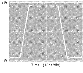
Large Signal Pulse vs. Ccomp
