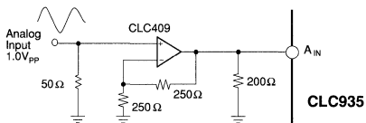
Figure 3: Analog Input Buffering
