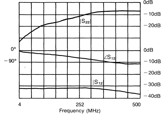
Reverse Isolation [ S_{12} ] and Output Return Loss [ S_{22} ]
