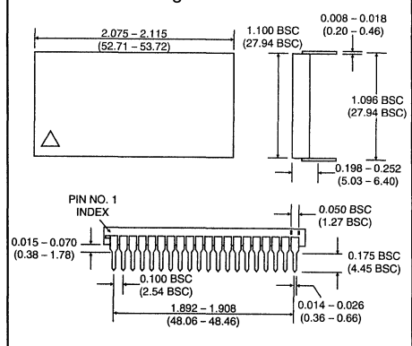
Package Dimensions
