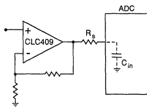
Figure 3: input amplifier to ADC
