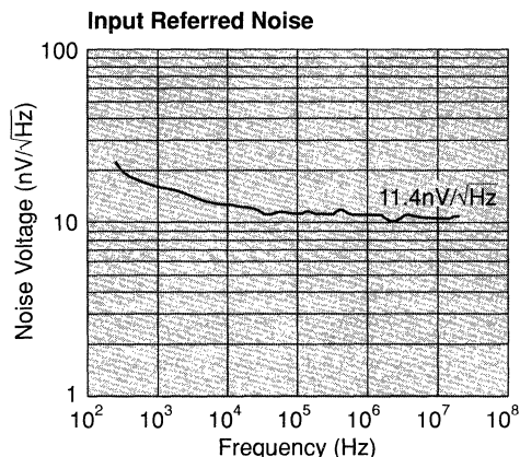
Figure 11: Input noise voltage
