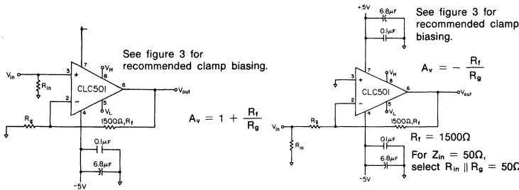
Figure 1: recommended non-inverting gain circuit
