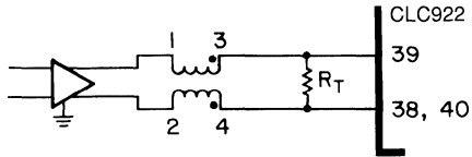
Typical Balun Circuits
