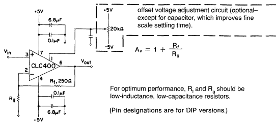
Figure 1: recommended non-inverting gain circuit
