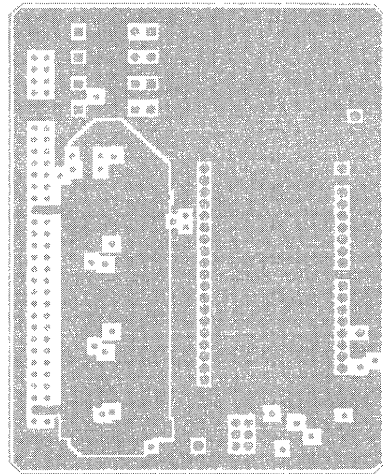
Layer 2 - Ground Plane
