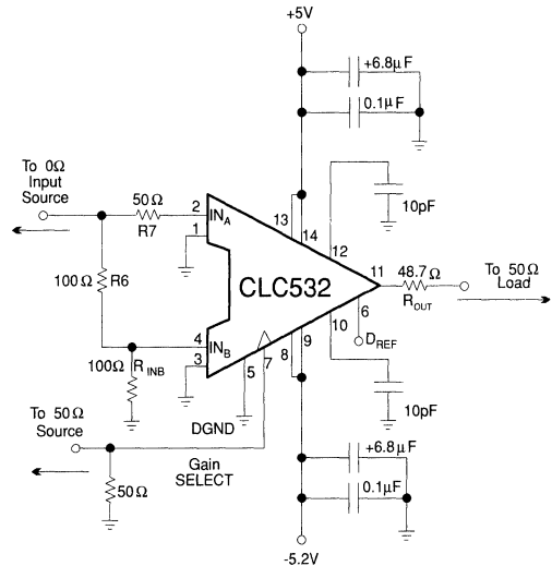
Figure 8: Basic Gain Select Configuration
