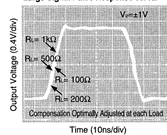
Large Signal Pulse Response vs. Rl
