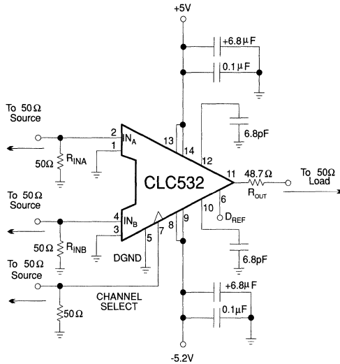
Figure 3: Basic Evaluation Schematic
