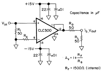
Figure 1: recommended non-inverting gain circuit
