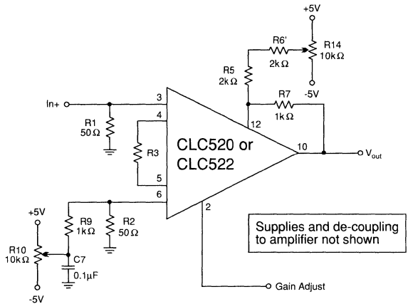
Figure 7: Input and output stage DC nulling
