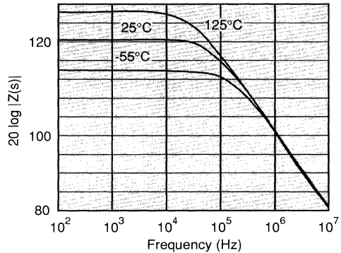
Figure 3: 20 \log |Z(s)| at 1mA = I_{cc} over temperature
