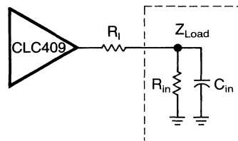
Figure 4: Experimental results indicate that this circuit offers the best bandwidth, flatness, and settling time for driving capacitive loads of up to 300pF in flash A to D converter applications.
