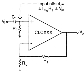
Figure 7: Effect of R_f on DC input offset voltage
