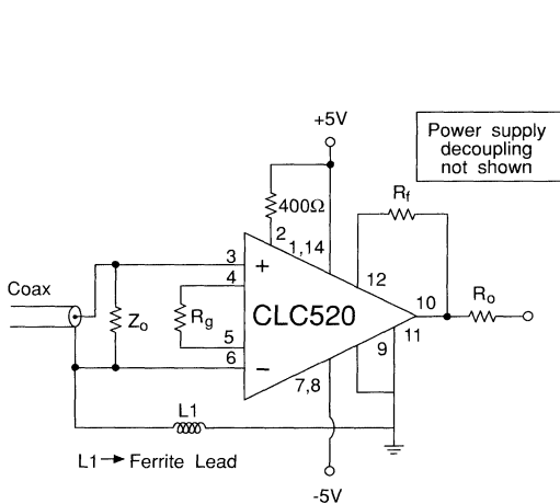
Figure 12: Differential coax line receiver
