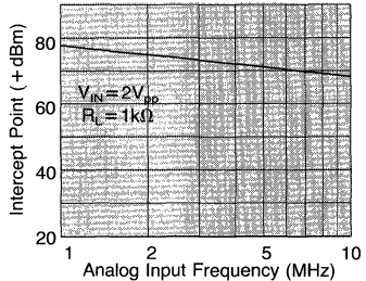
3rd Harmonic Distortion Intercept vs. Frequency
