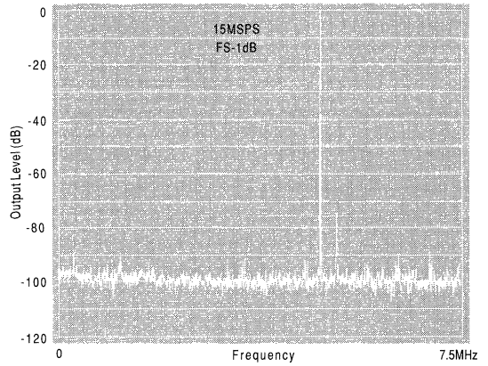
4.99MHz Output Spectrum
