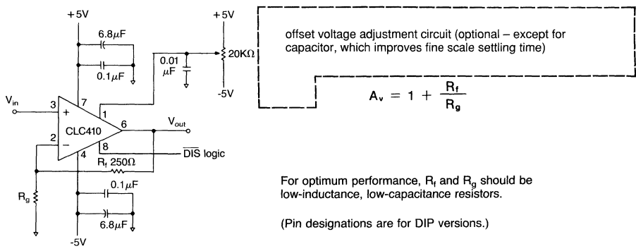
Figure 1: recommended non-inverting gain circuit
