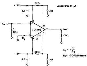
Figure 1: recommended non-inverting gain circuit
