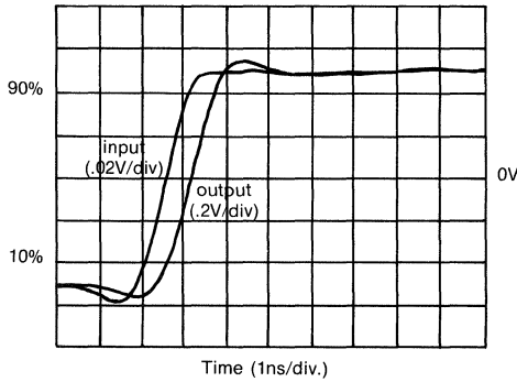
Pulse Response
