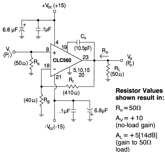
Figure 1: Test Circuit
