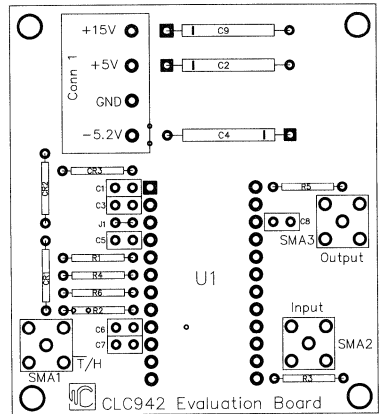
Component Placement Guide
