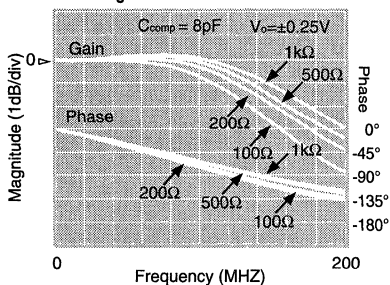
Large Signal Frequency Response vs. Load
