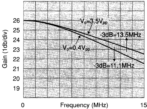
Figure 6: Frequency response vs. signal level
