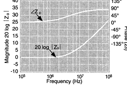
Input Impedance
