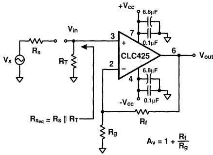
Figure 1: Non-inverting Amplifier Configuration
