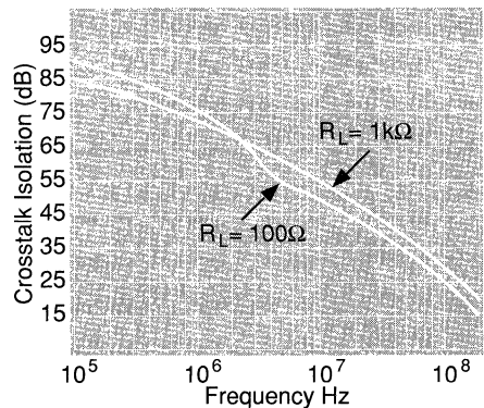
Figure 2: All-Hostile Crosstalk Isolation
