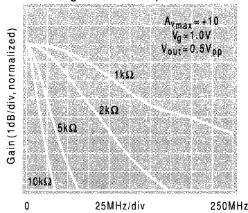
Small Signal Gain vs. R_I
