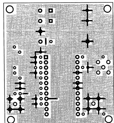
Component Side (viewed from top)
