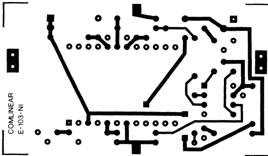
Figure 6: Component side (top), non-inverting
