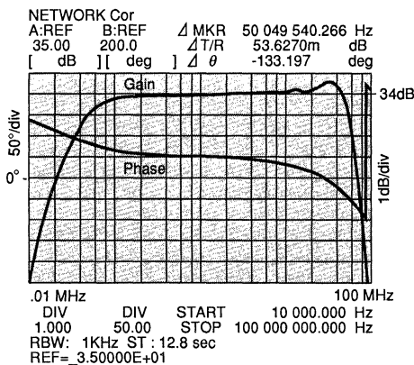
Transfer Function Figure 7b
