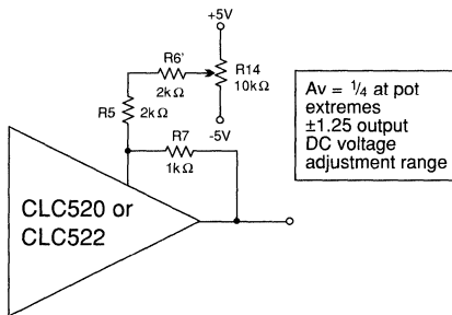
Figure 6: Summing in an output DC offset
