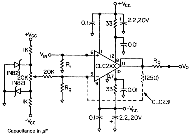
Schematic
