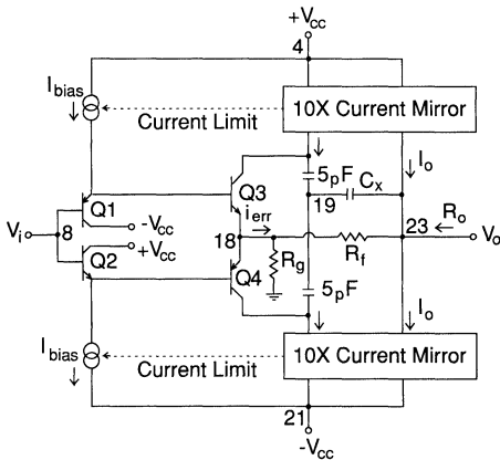
Figure 2: Simplified Circuit Diagram
