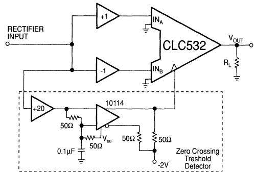
Figure 9: Low Distortion Full Wave Rectifier
