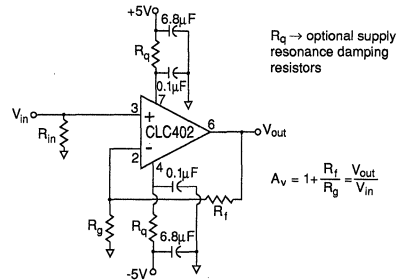
Figure 2: recommended non-inverting gain circuit
