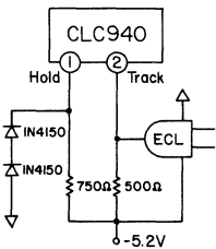
Figure 2: Single-ended ECL control
