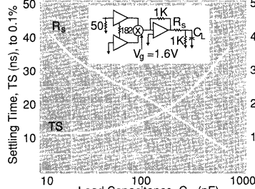
Settling Time vs. Capacitive Load, A_{VMAX} = \pm 10
