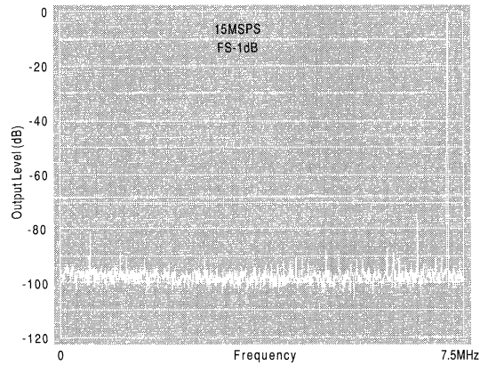
7.22MHz Output Spectrum
