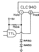
Figure 4: TTL control
