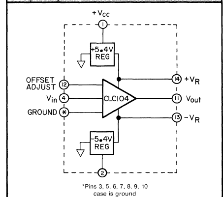
EQUIVALENT CIRCUIT
