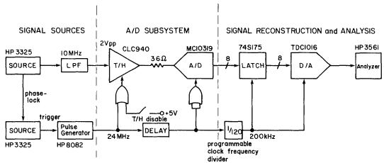
Figure 3: The T/H test system schematic shows the three blocks: signal sources, A/D subsystem, and signal reconstruction and analysis.
