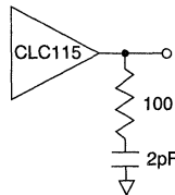
Figure 2: AC load
