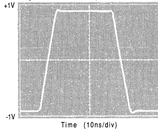
Large Signal Pulse vs. Ccomp
