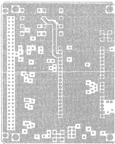
Layer 3 - Power Plane
