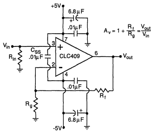
Figure 1: recommended non-inverting gain circuit
