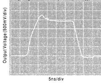
Long Term Settling Time
