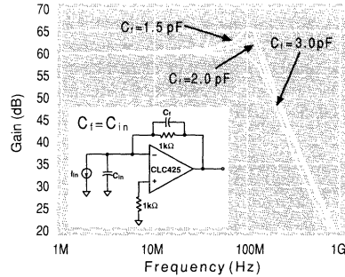
Figure 12: Transimpedance Amplifier Frequency Response
