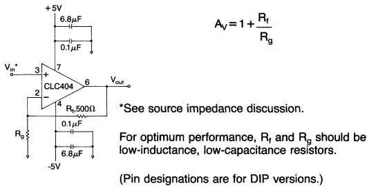
Figure 1: recommended non-inverting gain circuit
