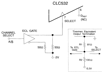
Figure 2: ECL Level Channel SELECT Configuration
