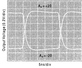
Short Term Settling Time
