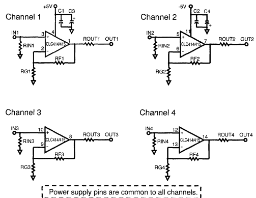
Figure 2: Board Schematic
