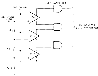
Figure 1: Simplified schematic of the flash A/D.
