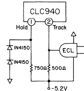
Figure 3: single-ended ECL control
