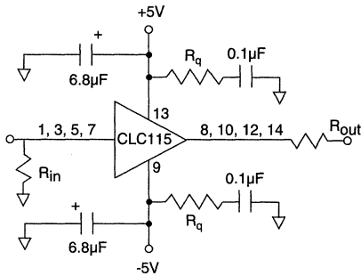
Figure 1: recommended circuit
