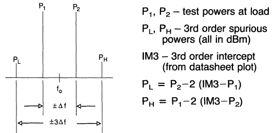
Figure 3: 3rd order spurious calculations
