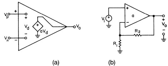
Fig. 1: Circuit model of the conventional op amp, and connection as a noninverting amplifier.
