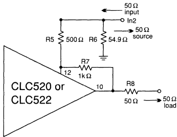
Figure 5: Summing a high-speed signal into the output
