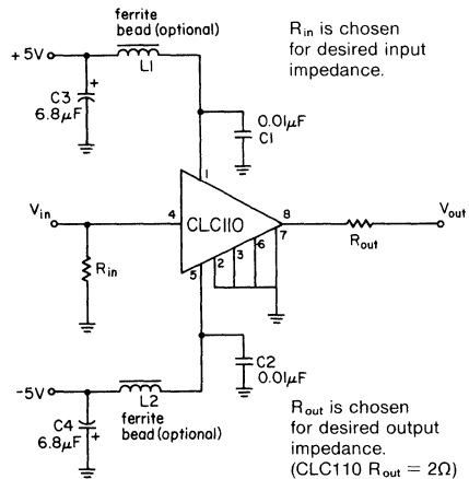
Figure 1: Recommended circuit and evaluation board schematic
