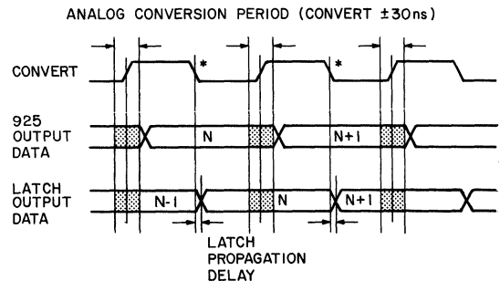
Recommended Latch/DATA READY Timing
