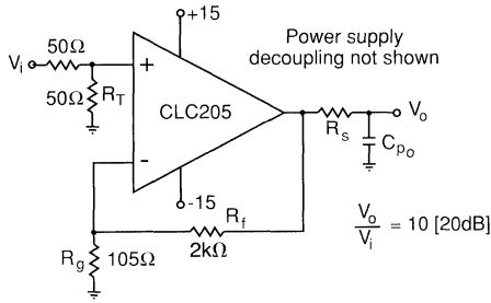
Figure 2a: Simulation circuit for capacitive loading test
