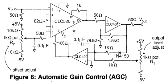
Figure 8: Automatic Gain Control (AGC) Loop
