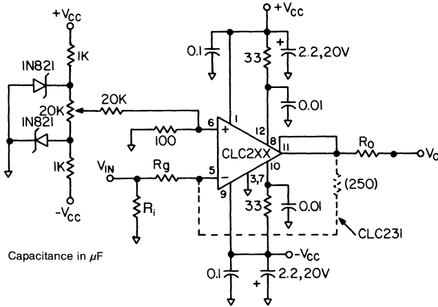
Schematic
