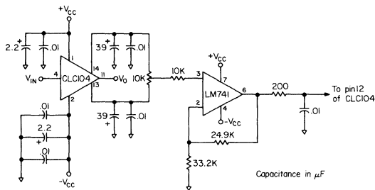
Figure 1: Circuit diagram showing offset voltage adjustment circuitry
