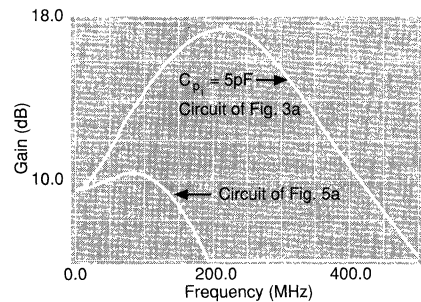
Figure 5b: Frequency response demonstrating zero cancellation
