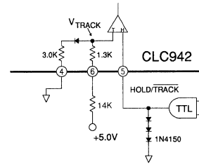
Figure 2: TTL compatible driver circuit
