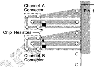
Figure 3: Analog Input Using Guard Ring
