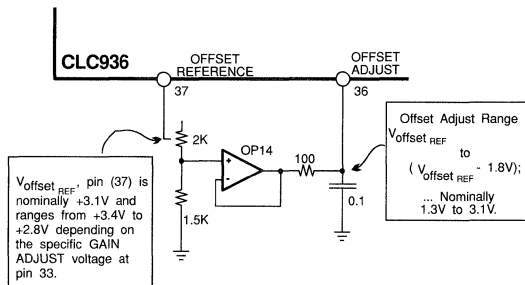
Offset Adjust Circuit
