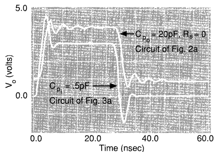
Figure 4: Contrasting pulse responses for C_{po} and C_{pi}
