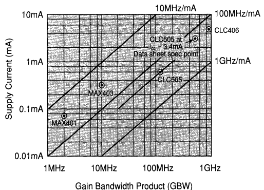
Figure 8: GBW vs. supply current
