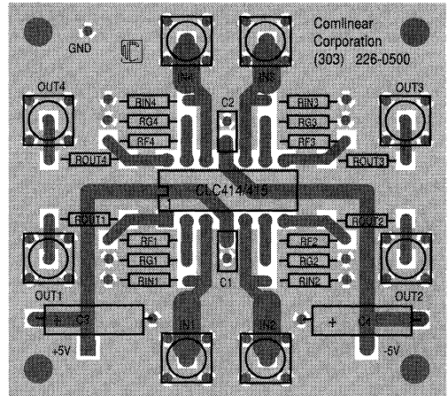
Figure 1: Board Layout and Component Placement
