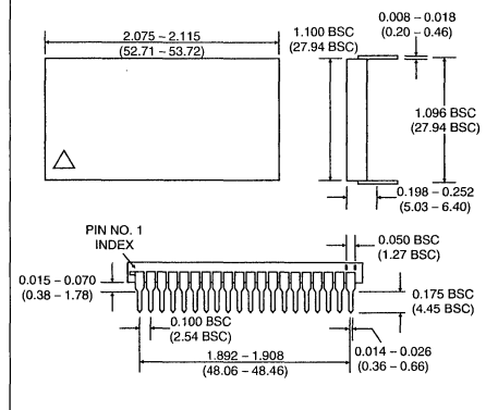
Package Dimensions
