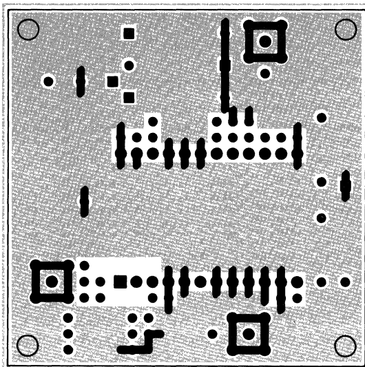
Figure 7: Component side (top) showing extensive ground plane
