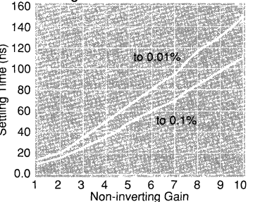
Settling Time vs. Gain
