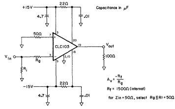
Figure 2: recommended inverting gain circuit
