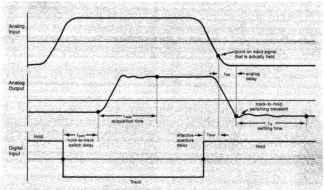
Figure 3: T/H amplifier waveforms for timing analysis.
