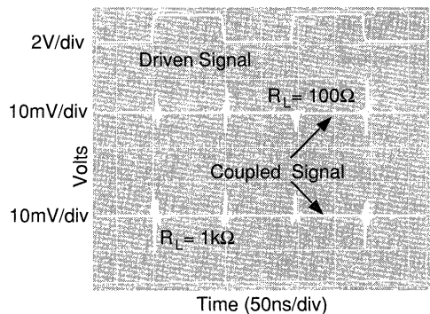
Figure 3: Most Susceptible Channel-to-Channel Pulse Coupling
