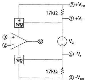
Figure 3: CLC411 Equivalent Circuit
