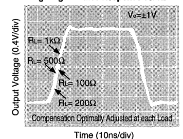
Large Signal Pulse Response vs. R_L
