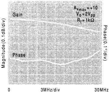
Gain Flatness & Linear Phase Deviation
