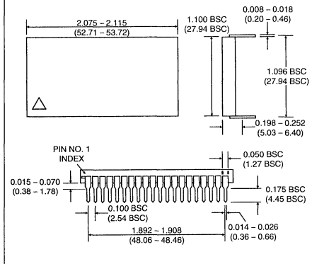
Package Dimensions
