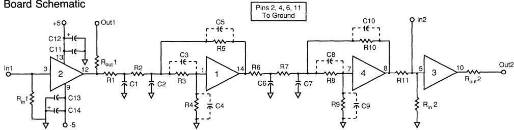
Figure 3 Board Schematic
