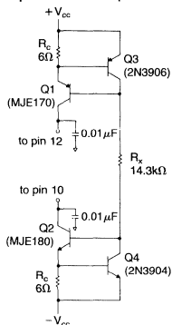
Figure 4: Active current limit circuit (100mA)
