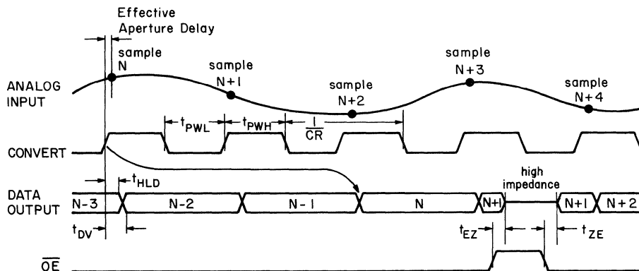
Timing Diagram
