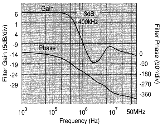
Figure 15: Very low power, single supply, active filter frequency response
