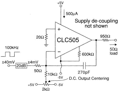
Figure 10: Low power integrator test circuit
