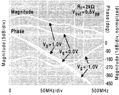
Frequency Response, A_{Vmax} = +2
