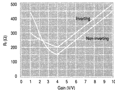
Figure 4: Recommended R_f vs. Gain
