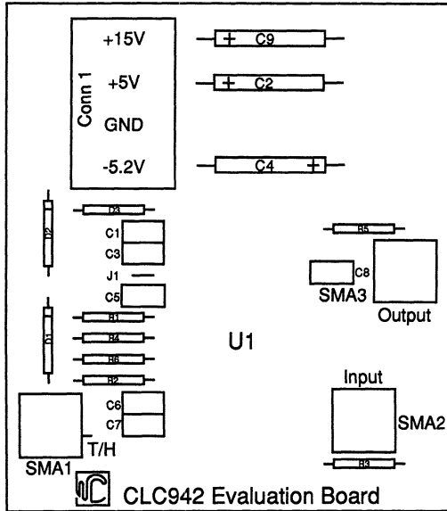
Component Placement Guide
