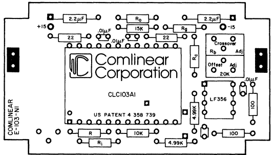
Figure 8: Component placement guide, non-inverting
