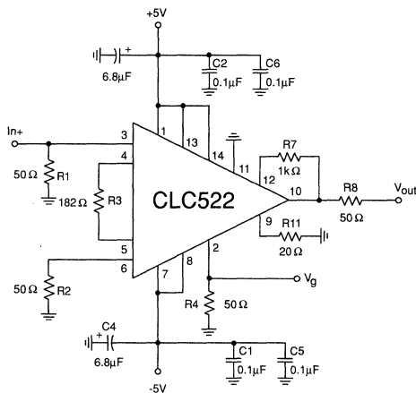
Figure 3: Basic CLC522 connection
