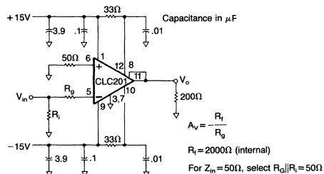
Figure 2: suggested inverting gain circuit
