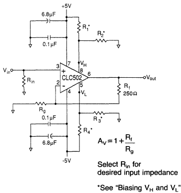
Figure 1: recommended non-inverting gain circuit
