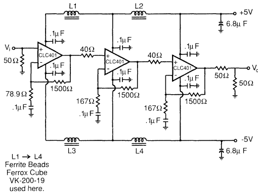
Figure 8: Wideband, high gain, cascaded amplifiers
