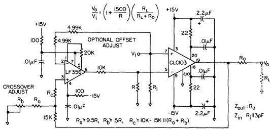
Figure 5: Non-inverting circuit with offset adjust circuitry
