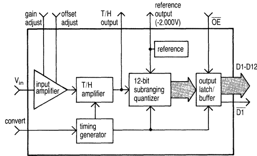
CLC925 Block Diagram
