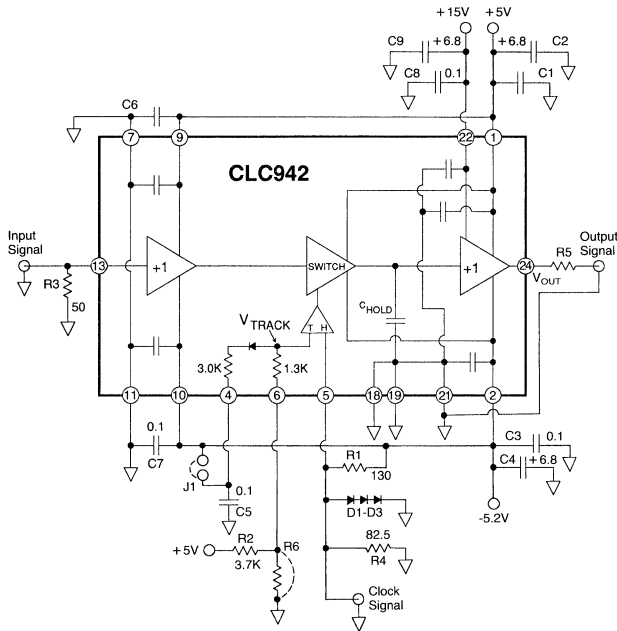
CLC942 Evaluation Board Schematic
