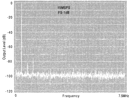
406kHz Output Spectrum
