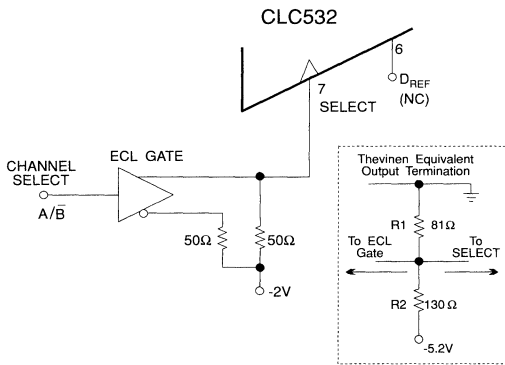
Figure 7: Standard ECL Terminations
