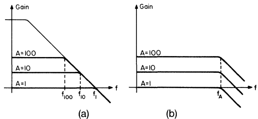
Fig. 7: Comparing the gain-bandwidth relationship of conventional op amps and current-feedback amplifiers.
