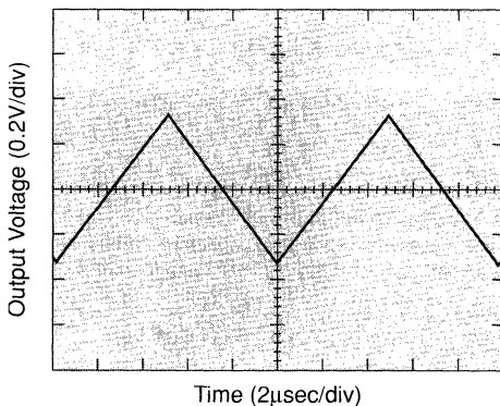
Figure 11: Integrator output to square wave input
