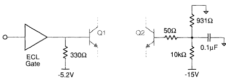
Figure 5C: ECL Interface
