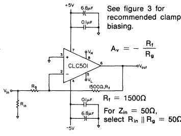
Figure 2: recommended inverting gain circuit
