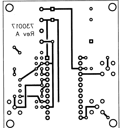
Solder Side (viewed from top)
