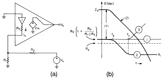
Fig. 8: Test circuit to investigate the effect of R_o , and noise-gain curves for the case of: (1) purely resistive feedback, (2) a capacitance in parallel with R_2 , and (3) the same capacitance in parallel with R_1 .
