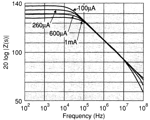
Figure 2: 20 \log |Z(s)| at different supply currents
