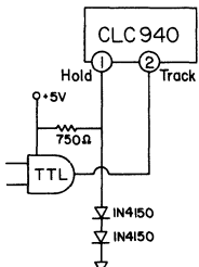
Figure 3: TTL control
