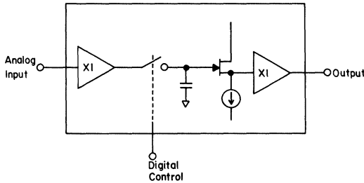
Figure 1: Block diagram of a high-speed T/H amplifier.
