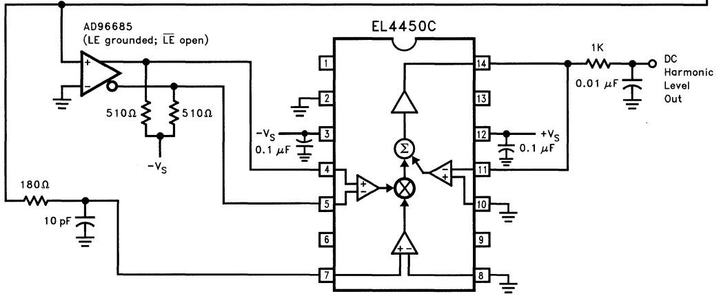
Figure 4. Harmonic Select and Measure Section
