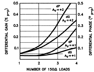
Differential Gain and Phase (30 MHz)
