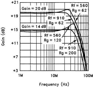
Gain of 5, 10 vs Various Rf, Rg at ± 5V
