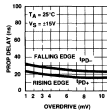
Propagation Delay vs Overdrive
