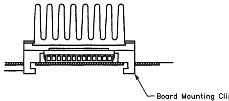
Figure 7. PSOP 2 with Heatsink and a Mounting Clip
