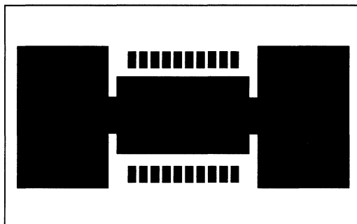
Figure 3. Typical Footprint for a Heat Dissipating Copper Clad
