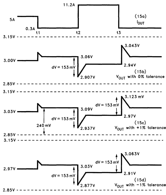
Figure 15. EL7560 Transient Output Voltage Response
