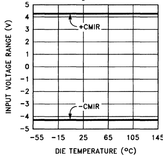
Input Voltage Range vs Die Temperature
