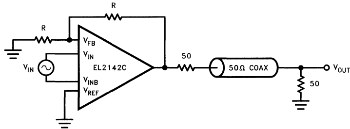
Figure 2. Coaxial Cable Driver
