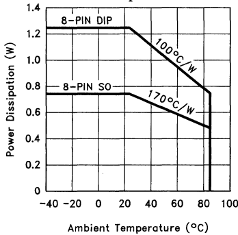
8-Pin Package Power Dissipation vs Ambient Temperature
