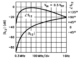
Reverse Gain and phase
