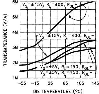
Transimpedance ( R_{OL} ) vs Die Temperature
