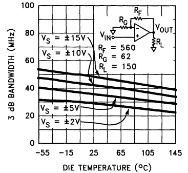
3 dB Bandwidth vs Temperature for A_v = +10
