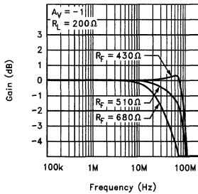
Receive Amplifier Frequency Response at V_S = ±15V
