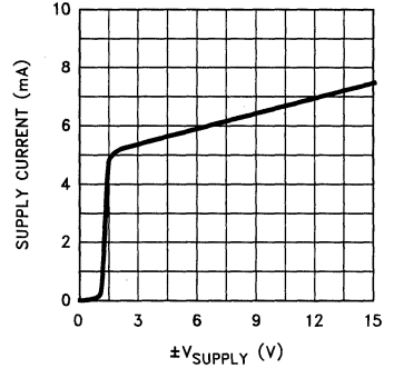
Supply Current vs Supply Voltage (Per Amplifier)
