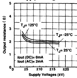
Output Resistance vs Supply Voltage
