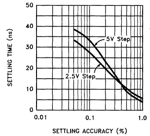
Settling Time vs Settling Accuracy
