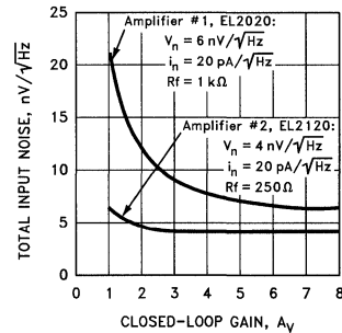
Figure 14. Noise vs Gain for Two CMF Amplifiers
