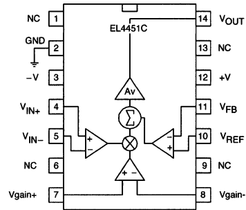
Figure 4. EL4451C
