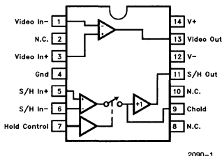
14-Pin DIP Package
