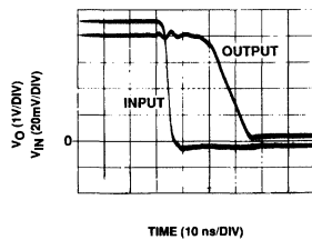
Propagation Delay (-) 5 mV Overdrive
