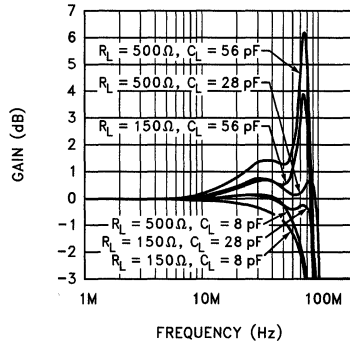
Frequency Response for Various R_L, C_L
