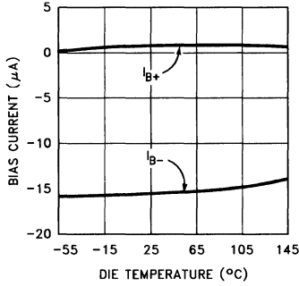
Input Bias Current vs Die Temperature
