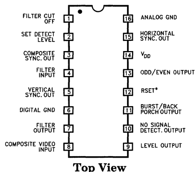
EL4583C SO, PDIP Packages
