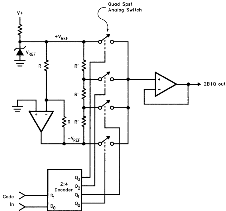
Figure 1. Classic 2B1Q Modulator
