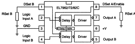
Figure 1. EL7962/72/82C Block Diagram
