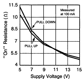
"On" Resistance vs Supply Voltage
