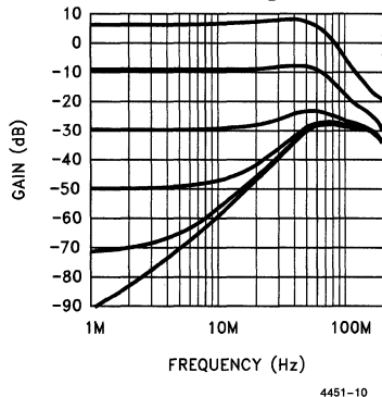
Frequency Response for Various Gain Settings
