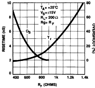
Risetime and Overshoot vs R_F for A_V = +2
