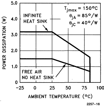
14-Lead Plastic DIP Maximum Power Dissipation vs Ambient Temperature
