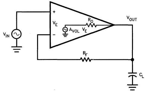
Figure 5. Capacitive Loads
