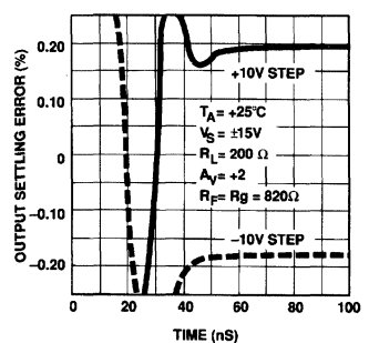
Output Settling Error vs Time
