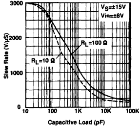
Slew Rate vs Capacitance Load
