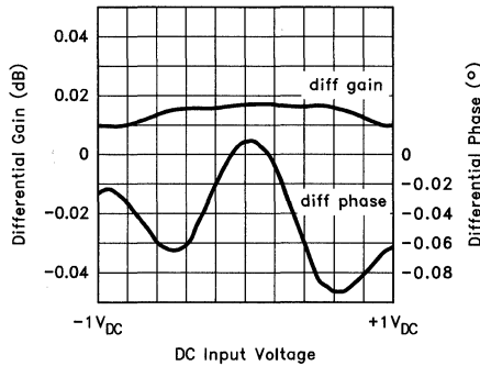
Differential Gain & Phase at 3.58 MHz
