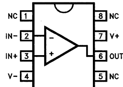
DIP and SO Package
