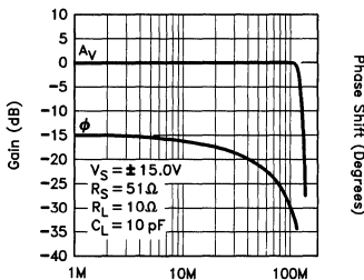
Voltage Gain and Phase vs Frequency
