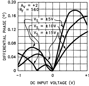
Differential Phase vs DC Input Voltage, R_L = 150
