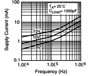
Average Supply Current into V HI vs. Voltage and Frequency
