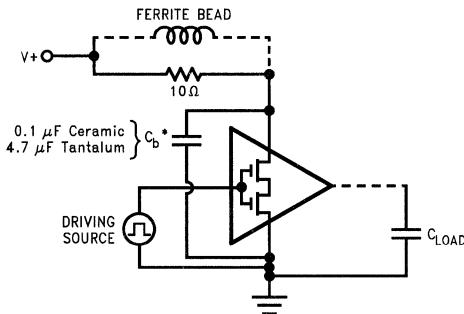
Figure 3. Suggested Decoupling/Bypassing
