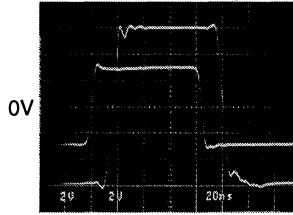
Large Signal Pulse Response
