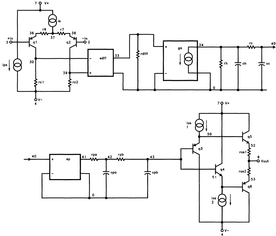
EL2244C/EL2444C Model
