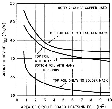
0952-4 Thermal Resistance of Dual-4-Fused-Lead SOL-20 Package
