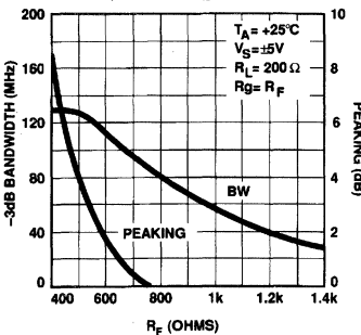
Bandwidth and Peaking vs R_F for A_V = +2, V_S = +5\text{V}
