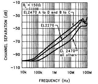
Channel Separation vs Frequency
