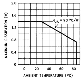
Maximum Power Dissipation vs Ambient Temperature—16-Pin SOL
