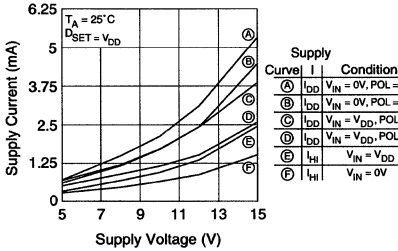
Quiescent Supply Current vs. Supply Voltage
