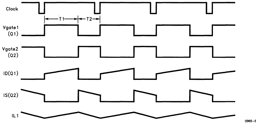
Figure 5. Gate Drive and Current Waveforms under Continuous Mode
