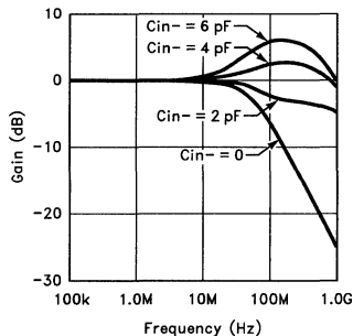
Figure 8. Ideal CMF Response with Various Values of C_{\text{IN}^-}
