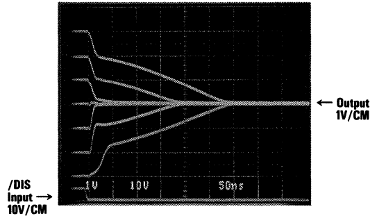
Disable Response for a Family of Inputs
