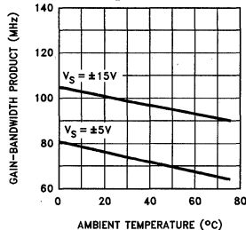
Gain-Bandwidth Product vs Temperature
