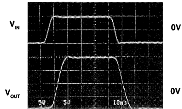
Large Signal Response
