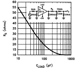
Recommended R_S vs Load Capacitance
