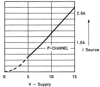
Peak Drive vs Supply Voltage
