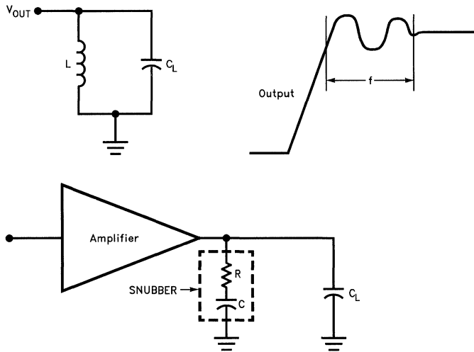
Figure 6. Snubbers
