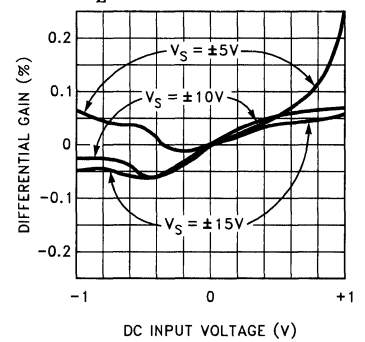
Differential Gain vs DC Input Voltage RL = 150
