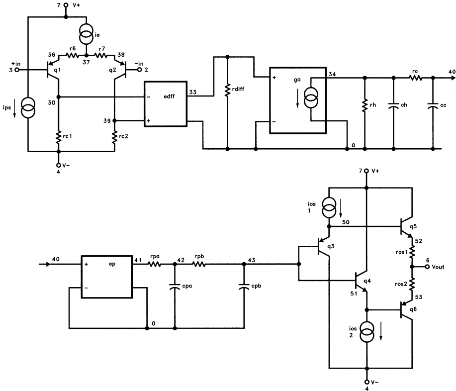
EL2045C Model
