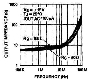
Output Impedance vs Frequency
