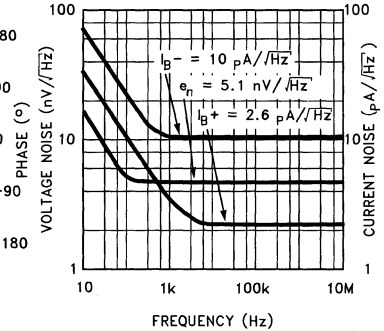
Voltage and Current Noise vs Frequency
