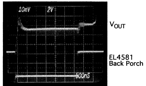
Figure 14. Back-Porch Sync Edge Feed-Through
