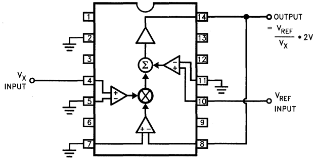
Divider Connection
