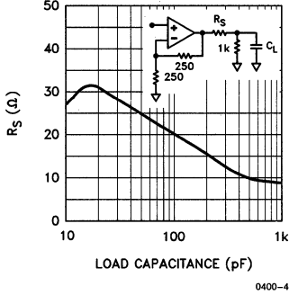
Recommended R_S vs Load Capacitance
