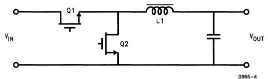
Figure 4. Buck Converter with Synchronized Switches
