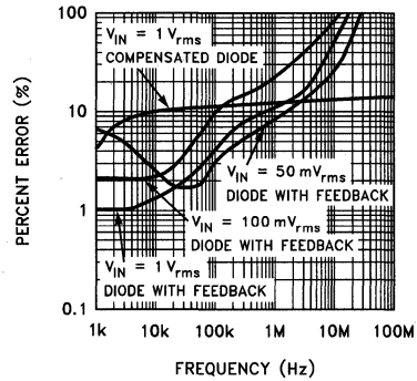
Figure 4. Error vs Frequency
