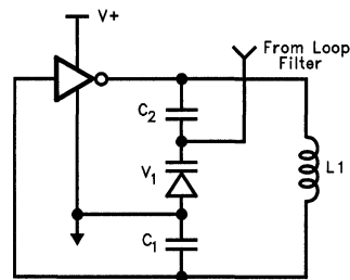
Colpitts Oscillator
