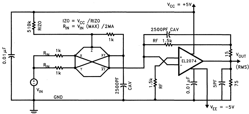
Figure 8. Single Multiplier Implicit RMS Computing Loop (RMS #2)
