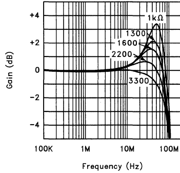
Gain Flatness vs Rf at ± 15V
