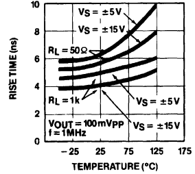
Rise Time vs Temperature
