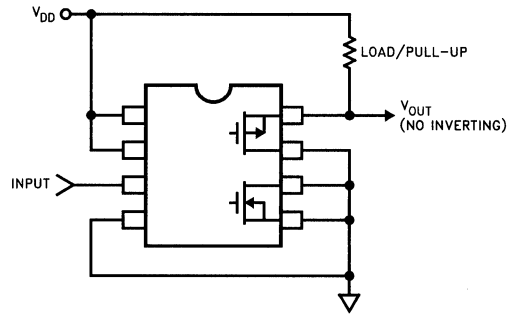
PMOS Follower
