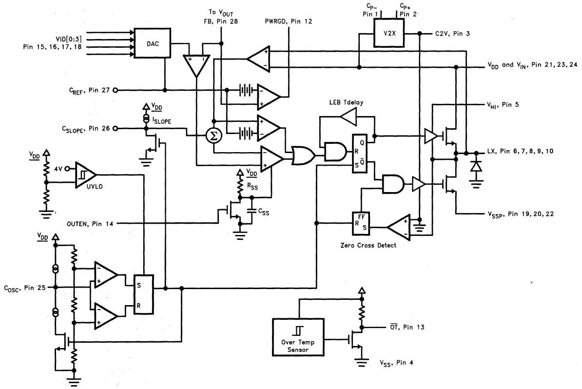
Figure 1. EL7560 Functional Block Diagram
