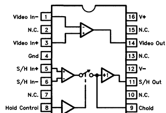
16-Pin SOL Package
