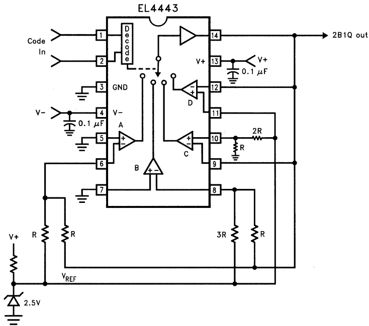
Figure 2. EL4443 in Simple 2B1Q Modulator
