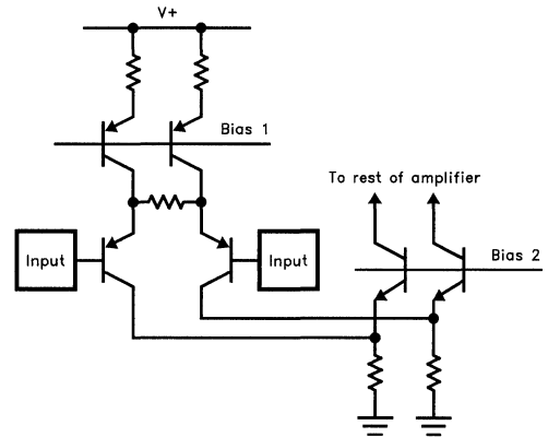
Figure 1. Typical Single-Supply Amplifier Input Stage
