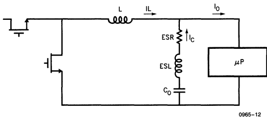
Figure 13. Output Current Path during Transient
