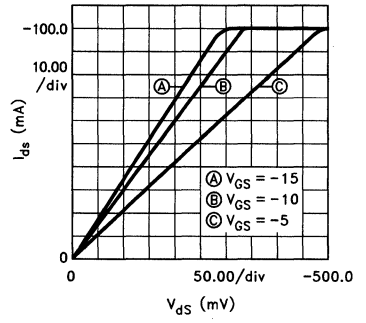
Output Conduction vs V_{GS}
