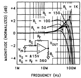
Frequency Response for Various R_L
