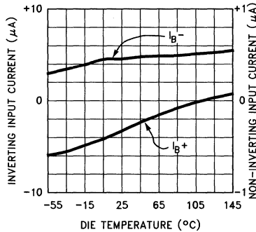
Input Current vs Die Temperature
