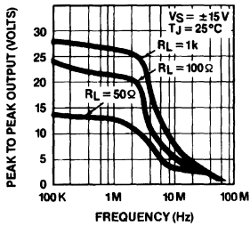
Maximum Undistorted Output Voltage vs Frequency
