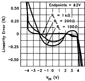
Integral Linearity Error
