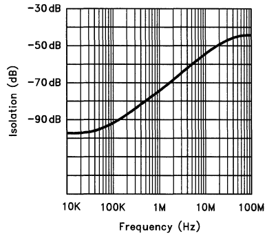
EL4393 MUX Channel Channel Isolation
