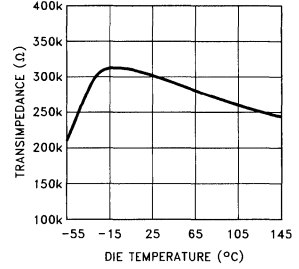
Transimpedance ( R_{OL} ) vs Die Temperature
