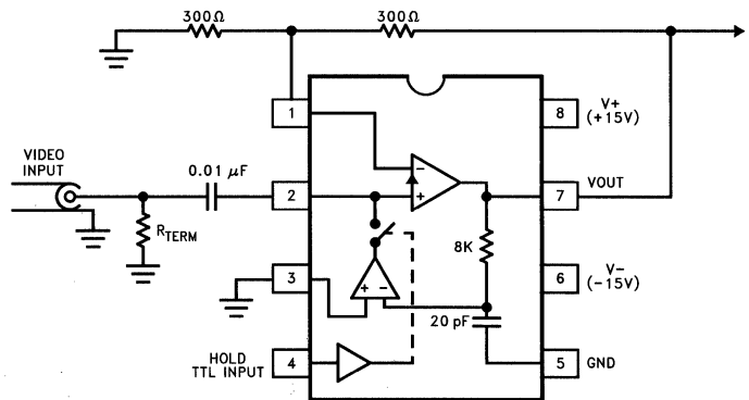
DC restoring amplifier with a gain of 2, restoring to ground.
