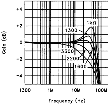
Gain Flatness vs Rf at ± 5V
