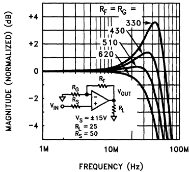
Frequency Response for Various R_F & R_G
