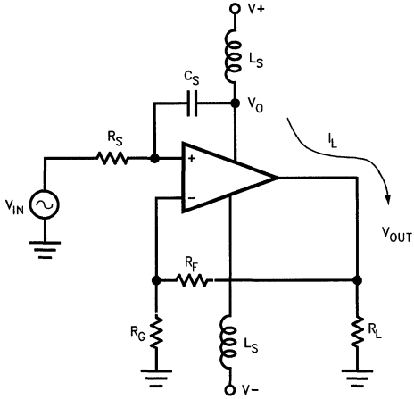
Figure 3. Power Supply Induced Oscillations
