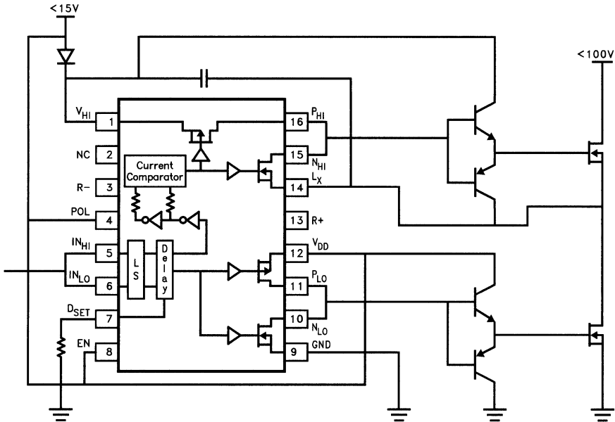
Figure 1. EL7661 Half Bridge Driver with Output Current Boost
