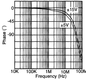
Phase Shift for A_V = 2 R_F = R_G = 1300\Omega
