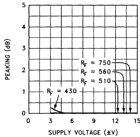
Peaking vs Supply Voltage for A_V = +10
