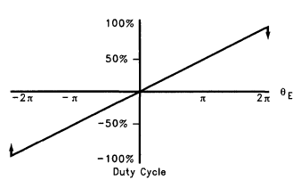
Charge Pump Duty Cycle Vs θ E
