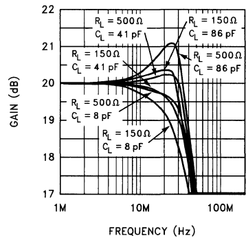
Frequency Response for Various R_L , C_L , V_S = \pm 15\text{ V}
