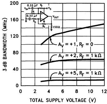
3 dB Bandwidth vs Supply Voltage for Non-Inverting Gains
