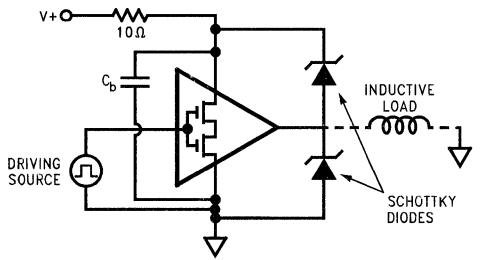
Figure 2. Suggested Configuration for Driving Inductive Loads
