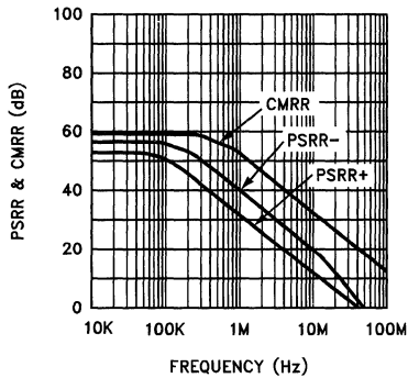
PSRR & CMRR vs Frequency
