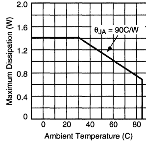
Maximum Power Dissipation vs Ambient Temperature— 16-Pin SOL
