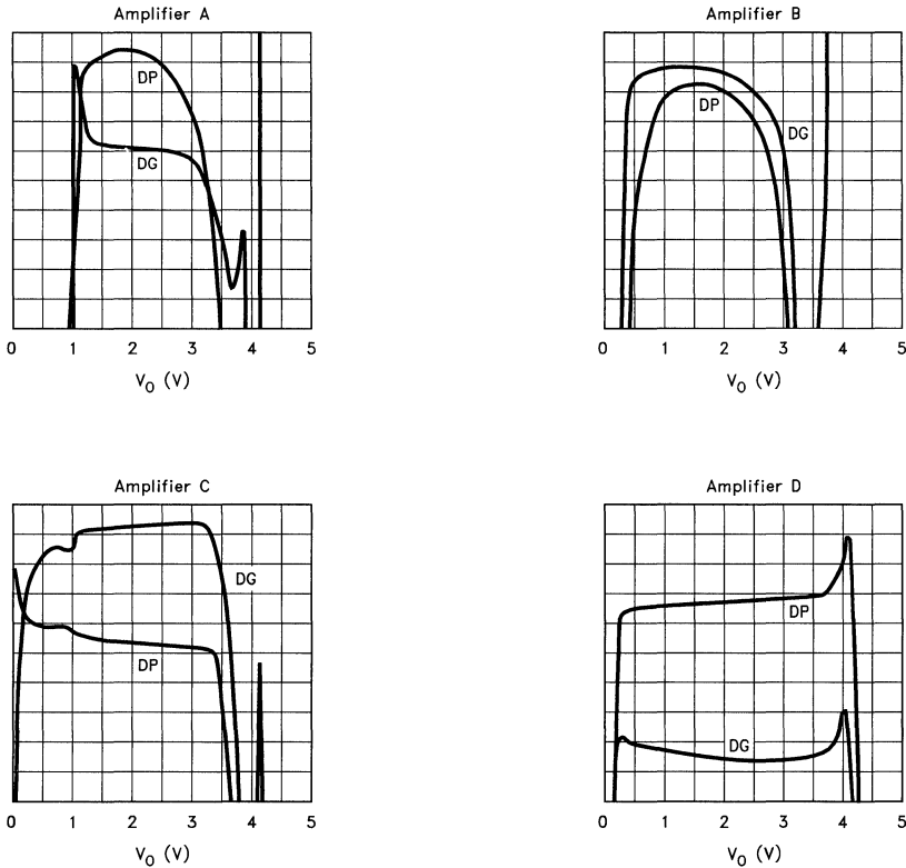
Figure 3. Differential Gain and Phase Error, A_V = 1 , R_L = 500 , V_{IN} = 0V-5V , DG = 0.2\%/div , DP = 0.2^\circ/div
