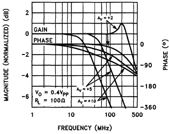
Non-Inverting Frequency Response
