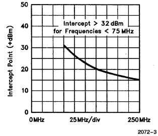
2-Tone, 3rd Order Intermodulation Intercept
