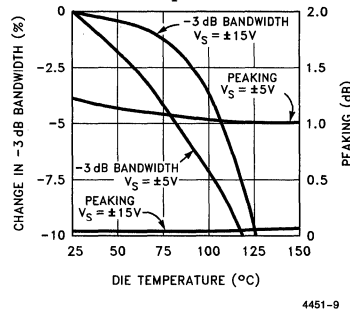
-3 dB Bandwidth and Peaking vs Die Temperature
