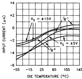
Input Current vs Die Temperature
