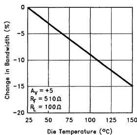
Driver Bandwidth vs Temperature
