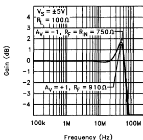
Driver Frequency Responses Equalized for Gains of +1 and -1
