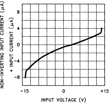
+ Input Bias Current vs Input Voltage
