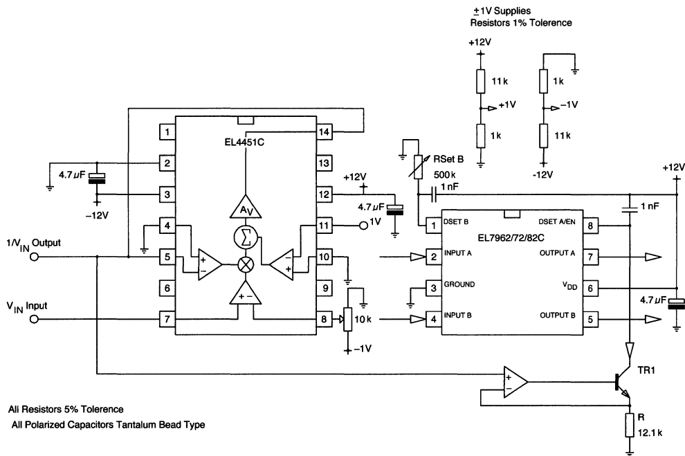
Figure 7. Voltage To Current Conversion Using An OpAmp
