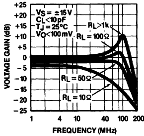
Voltage Gain vs Frequency Various Resistive Loads
