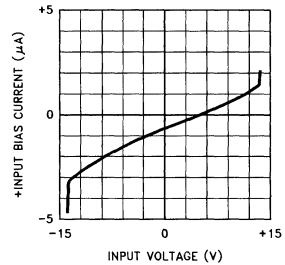
+ Input Bias Current vs Input Voltage
