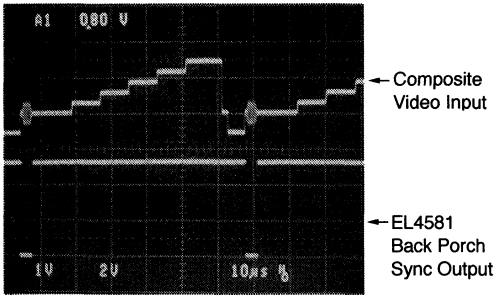
Photo 1. DC Restore
