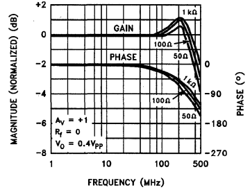
Frequency Response for Various R_L 's
