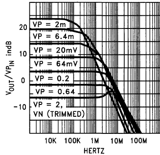
Figure 5. Gain/Frequency Response in 10 dB D.C. Steps at the Input
