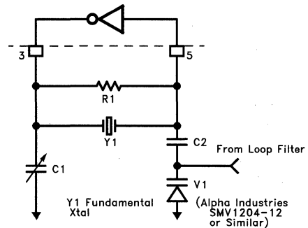
Typical Xtal VCO
