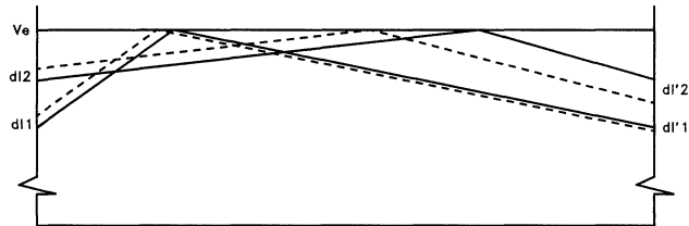
Figure 10. Inductor Current Error
