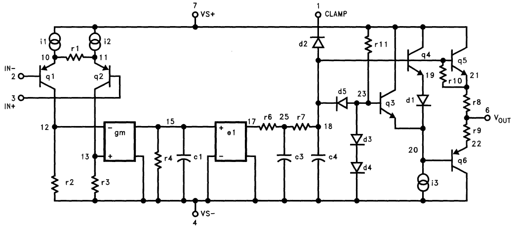
EL2257C/EL2357C Macromodel - (one channel) — Contd.
