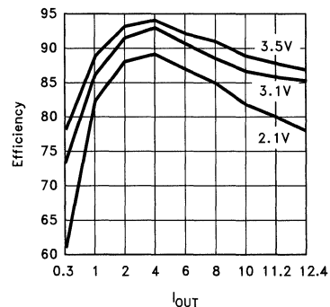
Figure 17. VRM Efficiency
