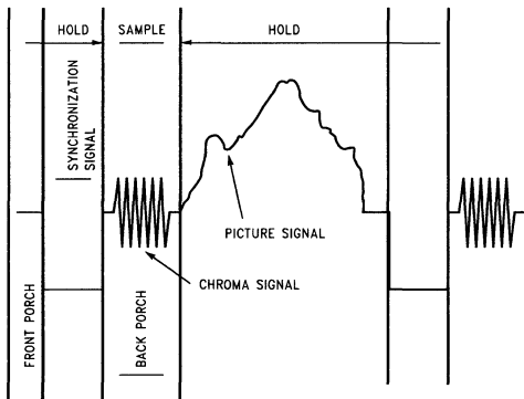
Figure 1. Video Signal
