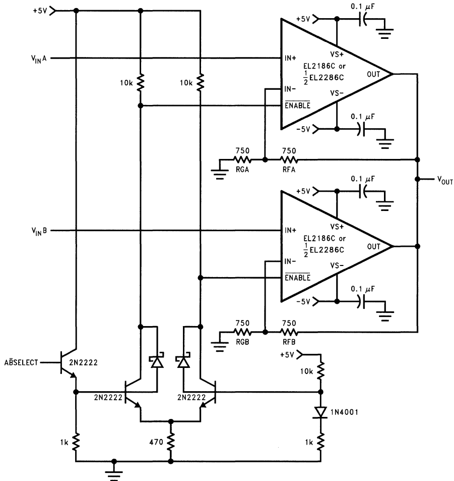
Low Power Multiplexer with Single-Ended TTL Input
