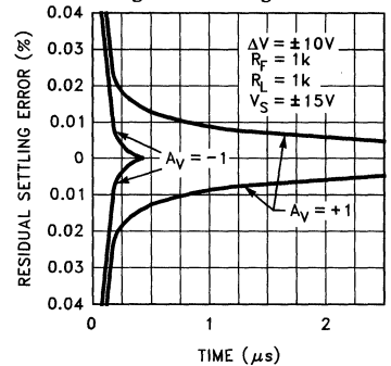
Long Term Settling Error
