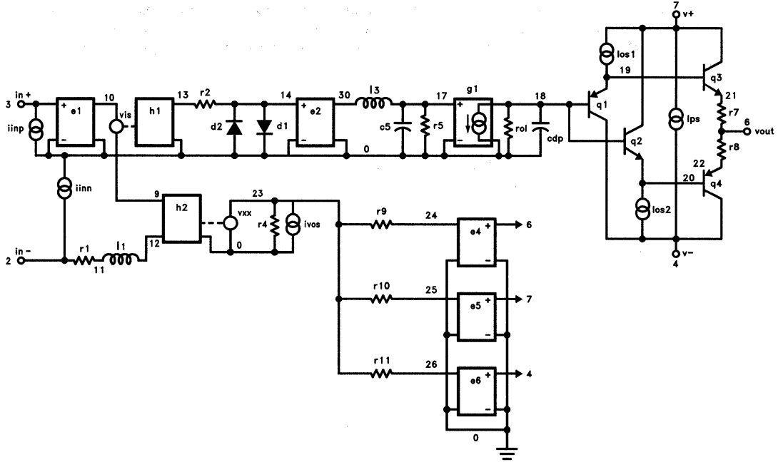
EL2120 Macromodel
