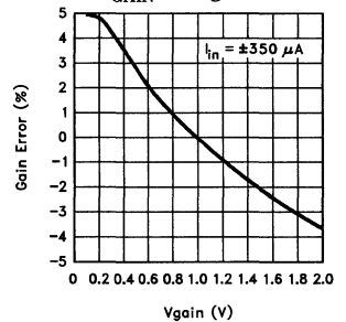
Normalized Gain Error vs V_{GAIN} Voltage
