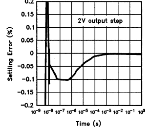
Long-Term Settling Time
