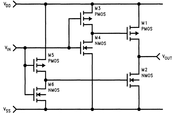
Figure 3A. Super Inverter
