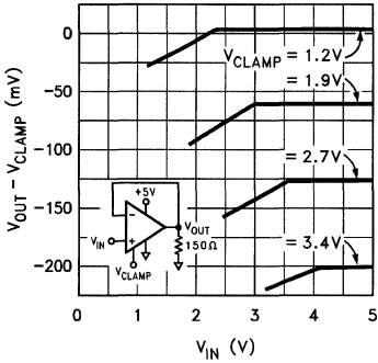
Clamp Accuracy R_L = 150\Omega
