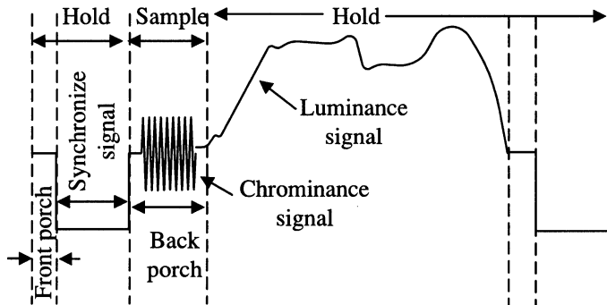
Figure 2. Typical Composite Video Signal
