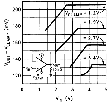
Clamp Accuracy R_L = 10\text{ k}\Omega
