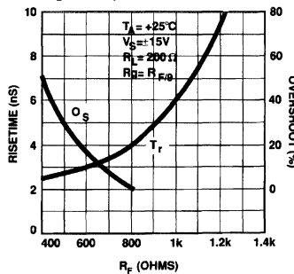
Risetime and Overshoot vs R_F for A_V = +10
