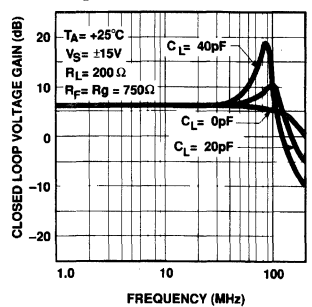
Voltage Gain vs Frequency for A_V = +2 , various Capacitive Loads
