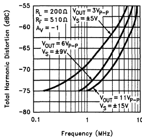
Receive Amplifier Harmonic Distortion vs Frequency (Single Amplifier)
