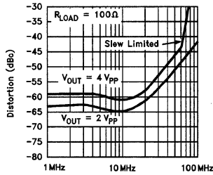
2nd Harmonic Distortion
