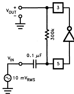
Test Circuit 1
