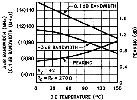
-3 dB Bandwidth, 0.1 dB Bandwidth, and Peaking vs Temperature at V_S \pm 15V
