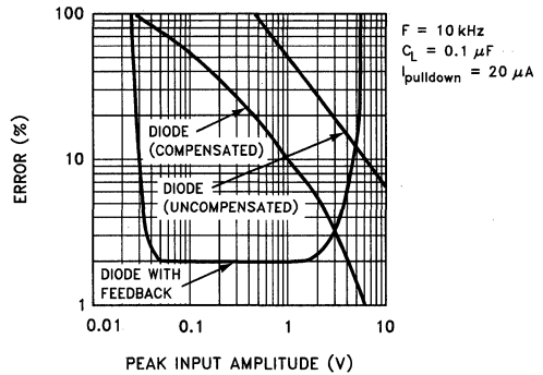
Figure 2. Error vs Amplitude
