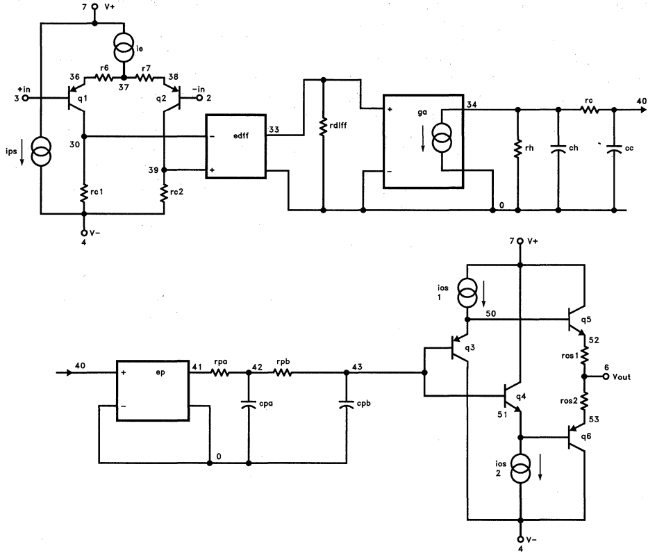
EL2245C/EL2445C Model
