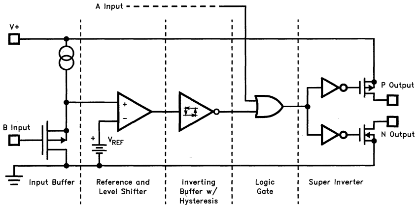
Simplified Schematic
