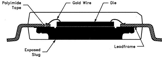
Figure 1. 28 PSOP 2 Structure
