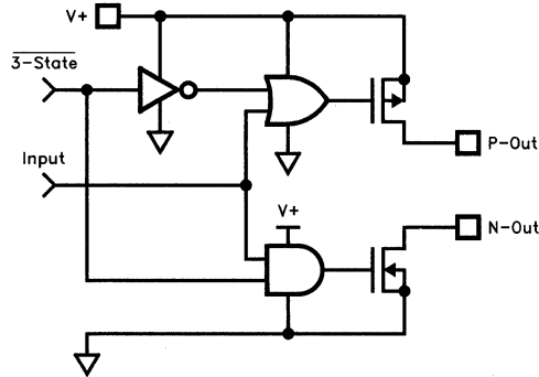
Simplified Schematic
