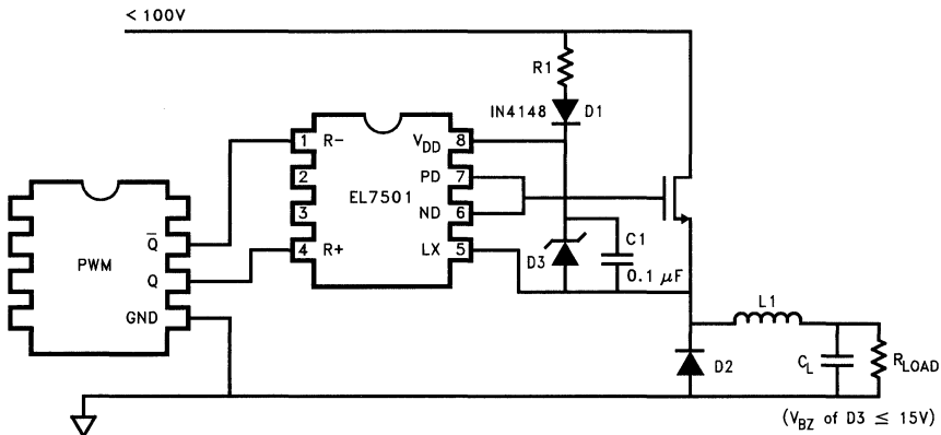
EL7501 Buck Regulator with High Side Drive (Alternate Biasing Scheme) Second Method
