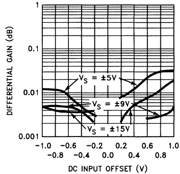
Differential Gain vs DC Input Offset; A_V = 2 , F_O = 3.58 \text{ MHz} , R_L = 150\Omega
