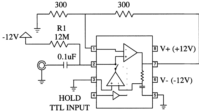
Figure 9. I_{B+} Bias Current Correction
