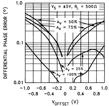
Differential Phase Error vs V_{offset} for Gain = 100%, 75%, 50% and 25%. F = 3.58 MHz
