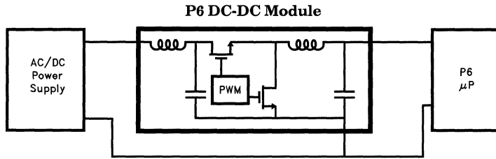
Figure 18. A Simplified Power System Block Diagram
