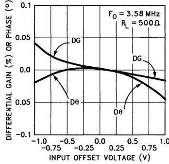
EL4431 Differential Gain and Phase vs Input Offset Voltage for V_S = \pm 12V
