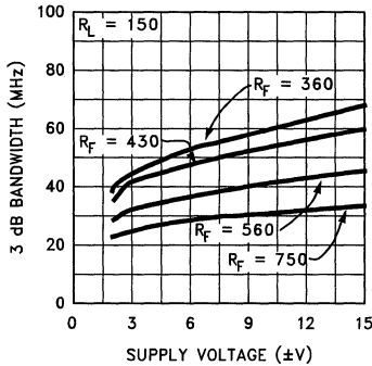
3 dB Bandwidth vs Supply Voltage for A_v = +10
