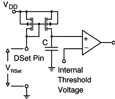
Figure 2. DSet Input Circuitry
