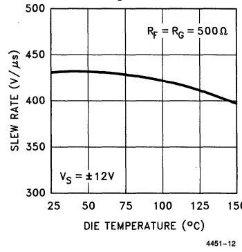
Slew Rate vs Die Temperature
