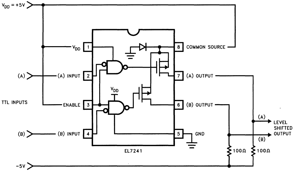
Level Shifter
