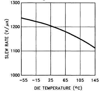
Slew Rate vs Die Temperature
