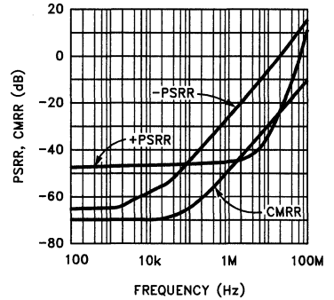
PSSR and CMRR vs Frequency
