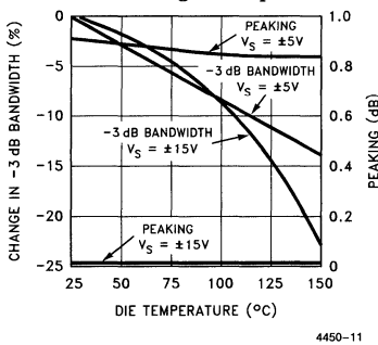
Change in Bandwidth and Peaking vs Temperature
