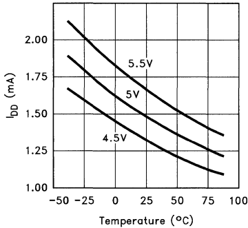
Supply Current, Quiescent R SET = 681k
