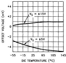
Offset Voltage vs Die Temperature
