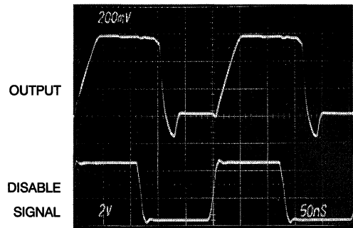
Enable/Disable with -VE Voltage Output
