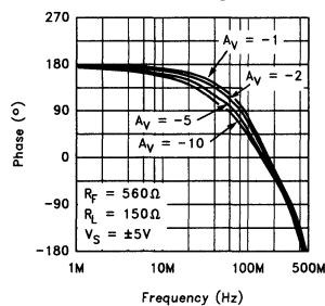
Inverting Frequency Response (Phase) (SOT23-5 Package)
