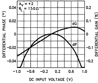
Differential Gain and Phase vs DC Input Voltage at 3.58 MHz
