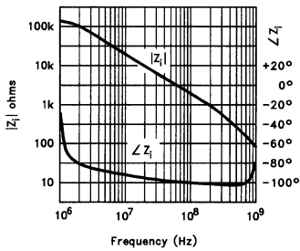
Input Impedance
