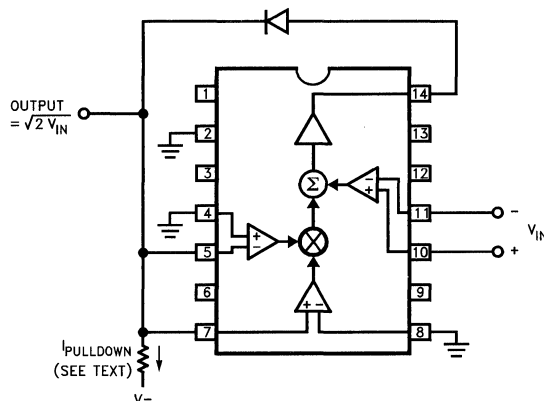
Square-Rooter
