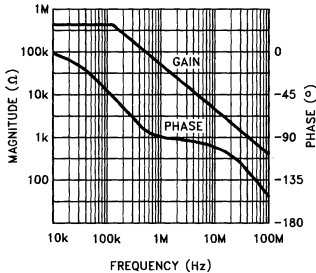
Transimpedance ( R_{OL} )
