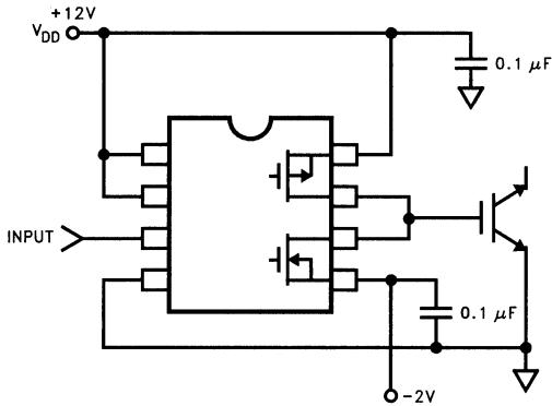
IGBT Driver (with Negative Swing)
