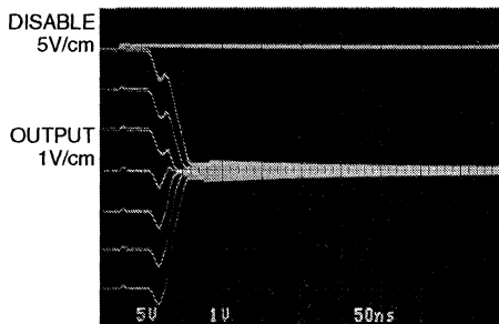
A_V = +2, R_L = 150, V_S = \pm 15V 2166-9
