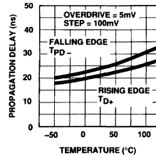
Propagation Delay vs Temperature
