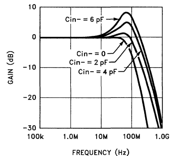
Figure 9. Realistic CMF Response with Various Values of C_{\text{IN}^-}
