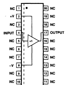
EL2001 SOL Pinout
