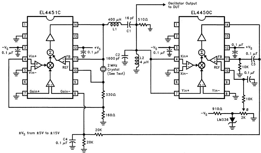
Figure 2. Low-Distortion Oscillator
