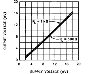
Output Voltage Range vs Supply Voltage
