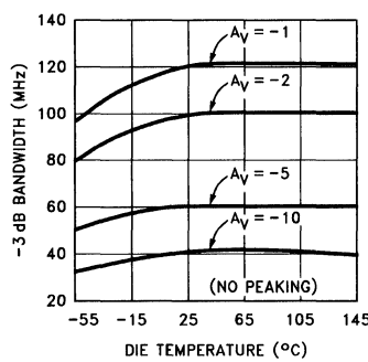
-3 dB Bandwidth vs Die Temperature for Various Inverting Gains
