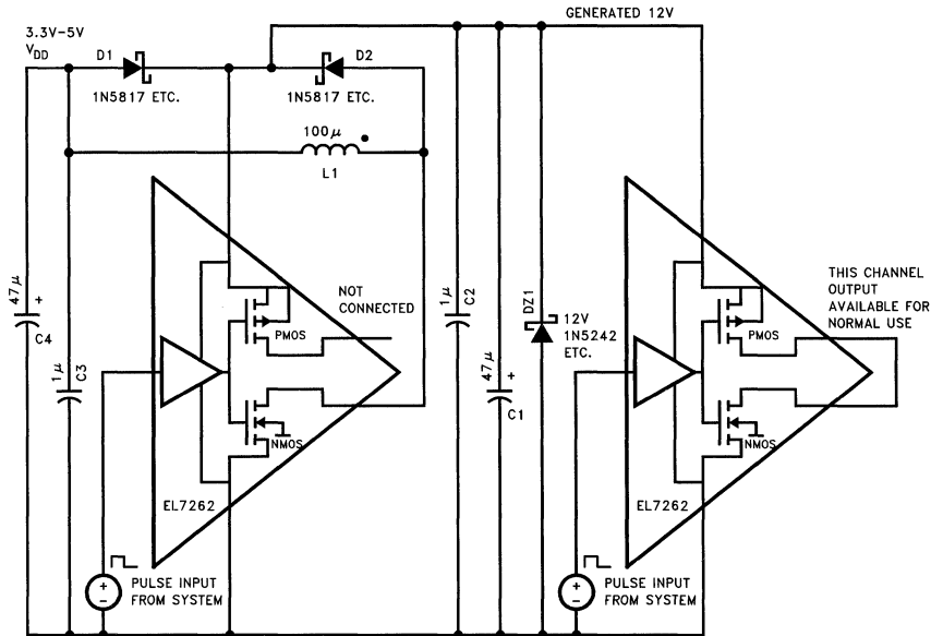
Self Charge Pumping Mosfet Driver
