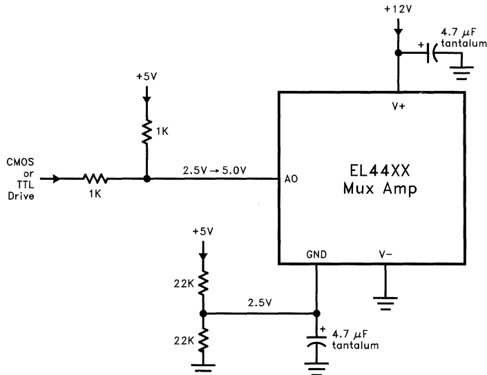
Figure 2. Using the EL44XX Mux Amps with +5\text{V} and +12\text{V} Supplies
