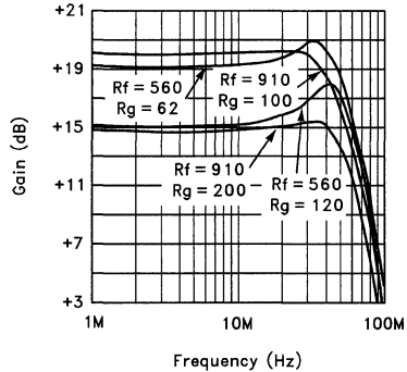
Gain of 5, 10 vs Rf, Rg at ± 15V
