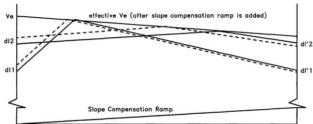
Figure 11. Inductor Current Ramps with Slope Compensation
