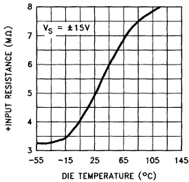
+ Input Resistance vs Die Temperature
