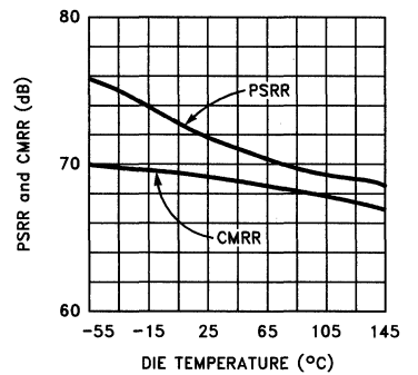
PSSR and CMRR vs Die Temperature
