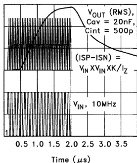
Figure 7. RMS #1 Response to a 10 MHz Signal Burst
