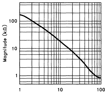
(a) Magnitude
