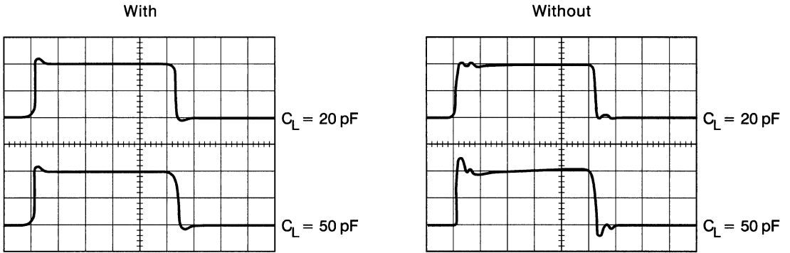
Figure 7. Response with and without a Snubber
