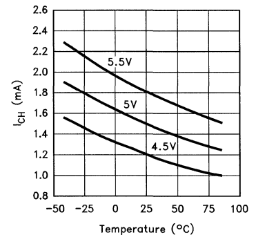
Clamp Charge Current R SET = 681k
