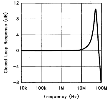
Figure 7. 2044 in Loop with 2002
