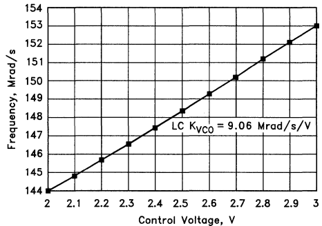
FOSC vs V_C , LC VCO
