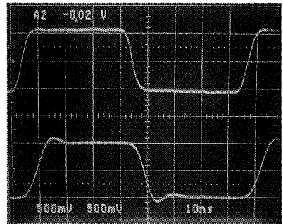
R_L = 50 \Omega , C_L = 10 \text{ pF} , V_S = \pm 15 \text{ V} Top is V_{IN} , Bottom is V_{OUT}
