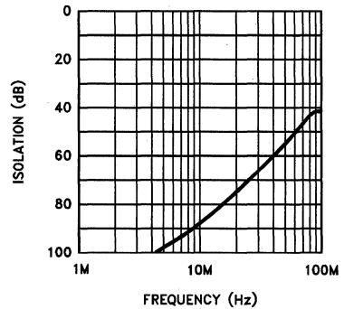
Channel-to-Channel Isolation of Dual EL2120C Multiplexer
