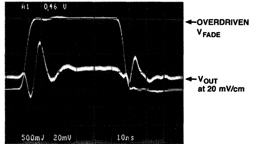
Overdrive Recovery Glitch from V_{FADE} , No Input Signal
