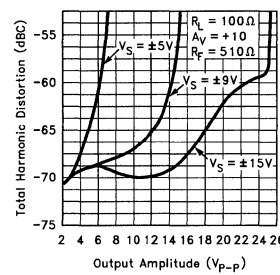
Driver Harmonic Distortion vs Output Amplitude at 2 MHz (Single Amplifier)
