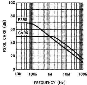
PSRR and CMRR
