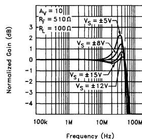
Driver Frequency Response vs ± Supply Voltage
