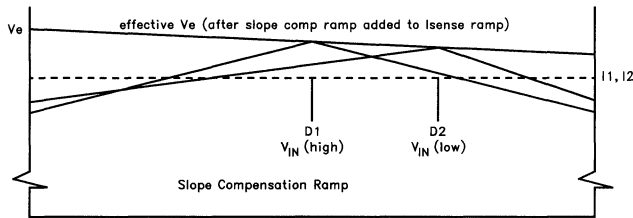
Figure 9. Constant Average Output Current
