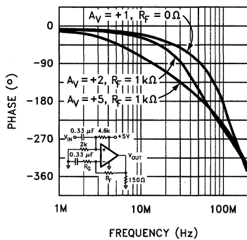
Non-Inverting Frequency Response (Phase)
