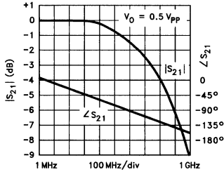
Forward Gain and Phase
