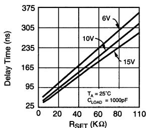
Output Rising Edge Delay vs RSET and Supply Voltage (Detail)
