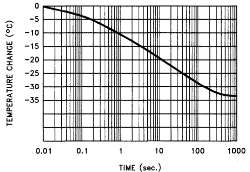
Thermal Relaxation vs. Time of a Mounted Power SO-20 Package
