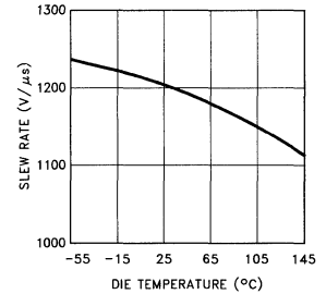
Slew Rate vs Die Temperature
