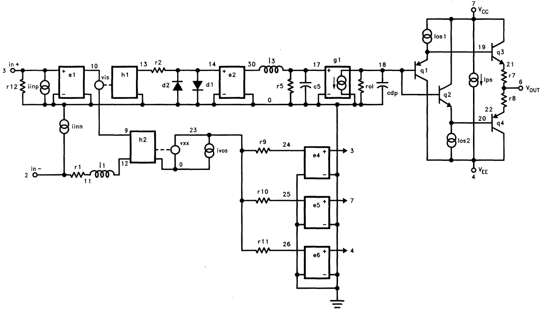
EL2186C/EL2286C Macromodel — Contd.
