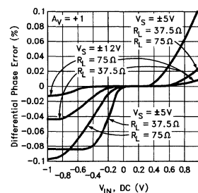
Driver Differential Phase Error vs DC Input Offset Gain = +1
