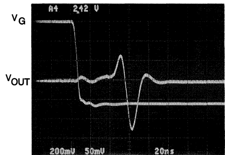
V_{GAIN} Overload Recovery Response
