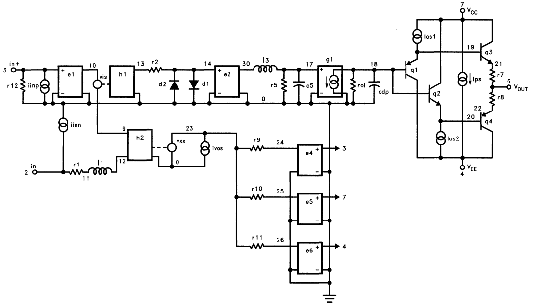
EL2180C/EL2280C/EL2480C Macromodel — Contd.
