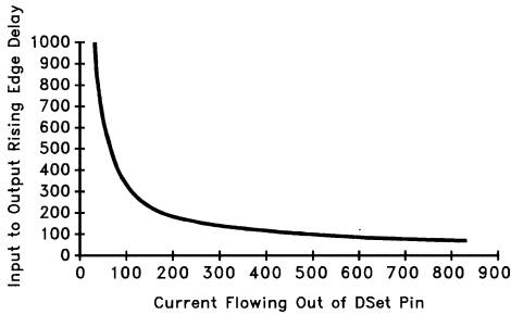
Figure 3. Rising Edge Delay vs Current Out of the DSet Pin
