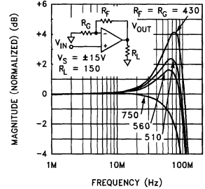
Frequency Response for Various R_F and R_G
