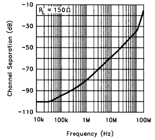
Channel Separation vs Frequency (EL2286)
