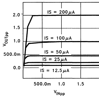
Figure 14. AGC Circuit Output Level Regulation vs Input Level at Several Values of I_{SET}
