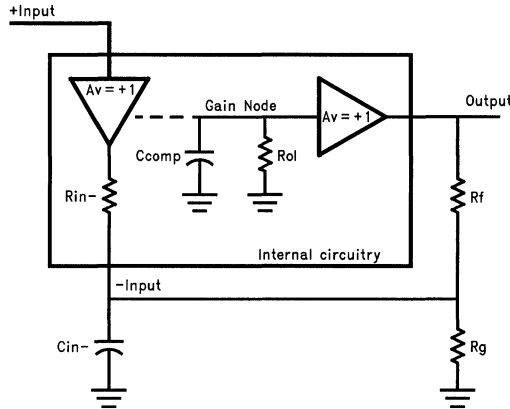
Figure 7. Small-Signal Equivalent Circuit of the Current-Feedback Amplifier
