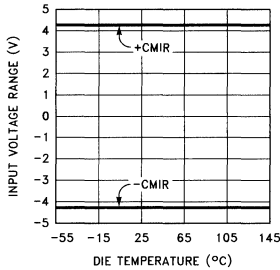
Input Voltage Range vs Die Temperature
