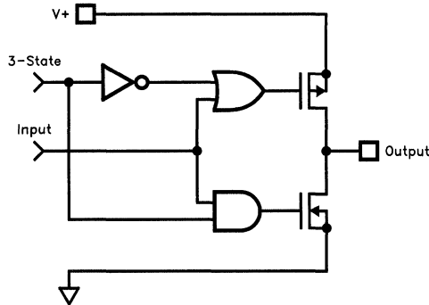
Simplified Schematic
