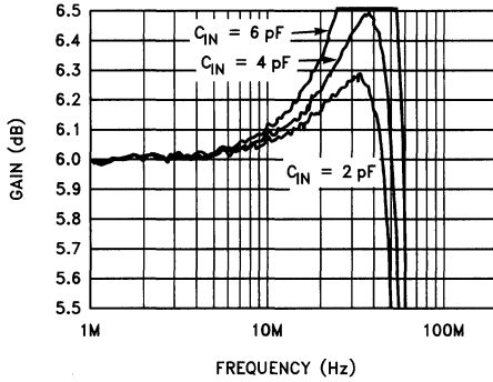
Frequency Response Flatness vs C_{IN-} ; A_V = 2 ; R_F = 300
