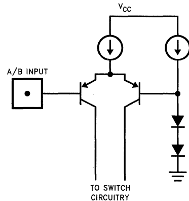
Figure 2a. Simplified Logic Input Stage
