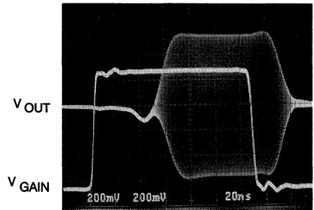
V_{GAIN} Overload Recovery Delay
