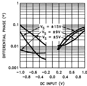
Differential Phase vs DC Input Offset; A_V = 2 ; F_O = 3.58 \text{ MHz} ; R_L = 150\Omega
