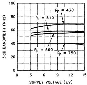
3 dB Bandwidth vs Supply Voltage for A_V = +10
