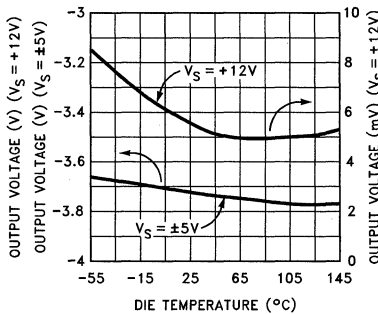
Negative Output Voltage Swing vs Die Temperature, R_L = 150Ω to GND
