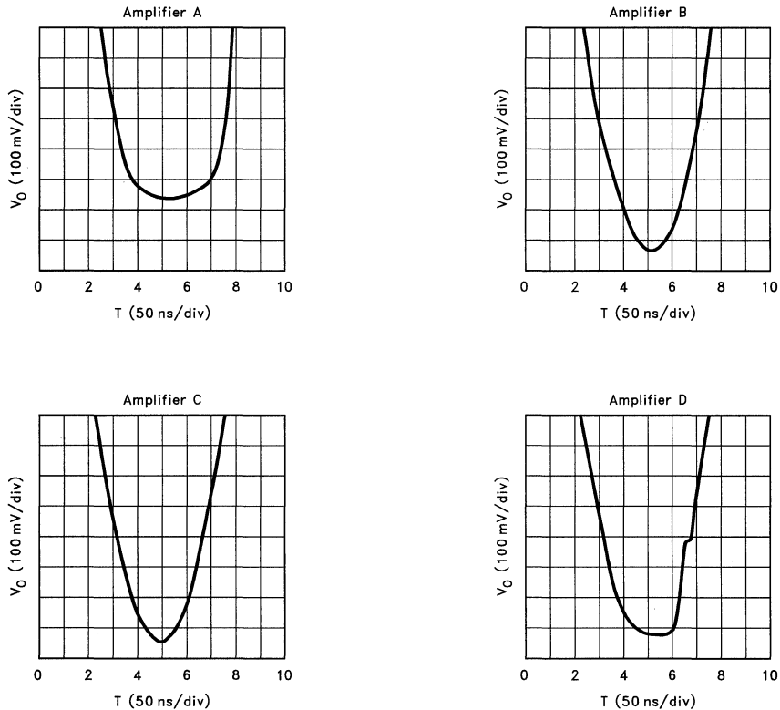
Figure 6. Transient Response, A_V = 1 , R_L = 150
