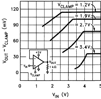
Clamp Accuracy R_L = 1\text{ k}\Omega
