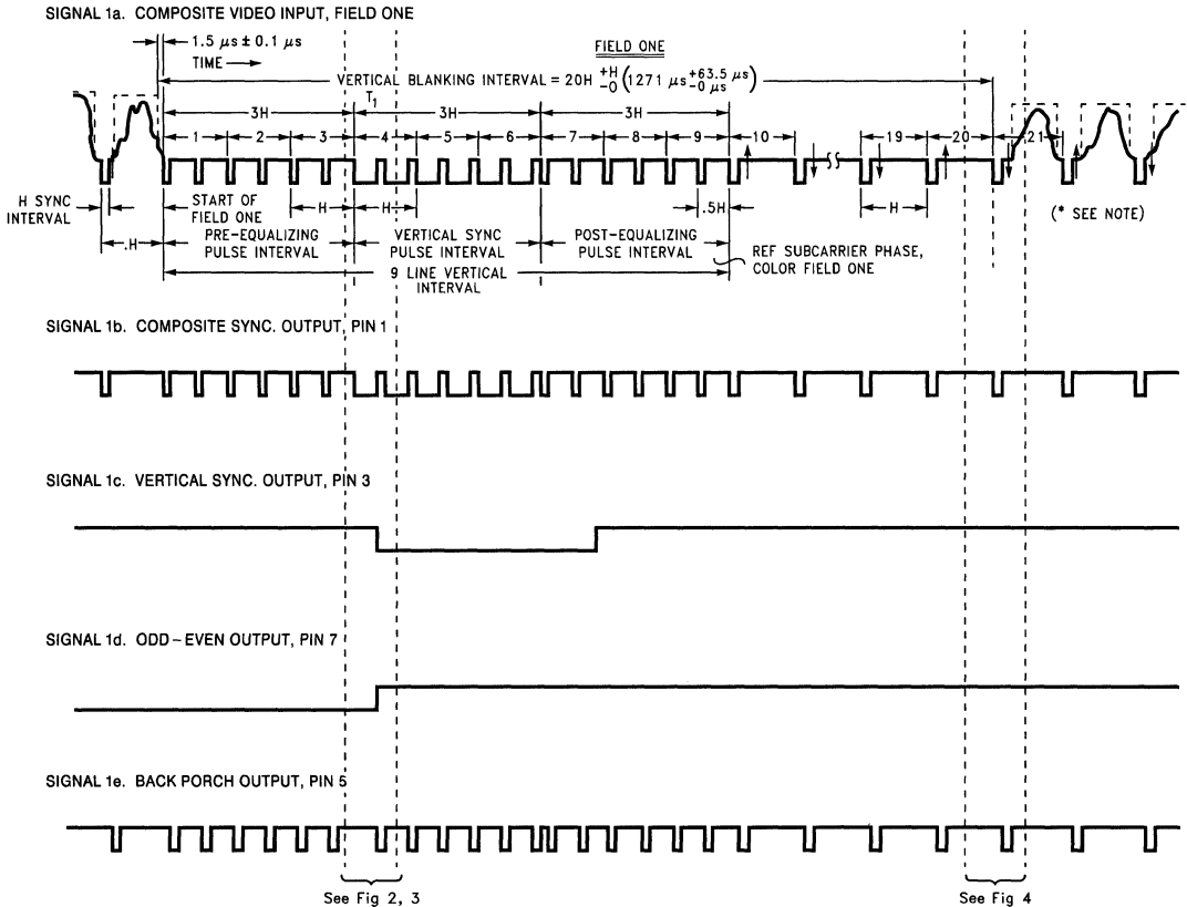
Figure 1. Standard (NTSC Input) Timing
