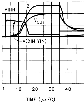
Figure 9. RMS #2 Signal Burst Response
