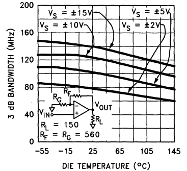
3 dB Bandwidth vs Temperature for A_v = +2
