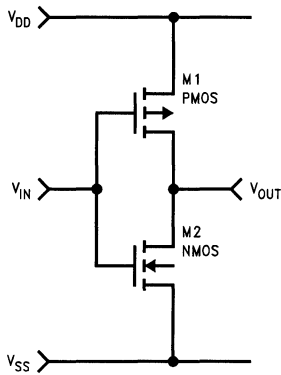
Figure 2A. Standard CMOS Inverter
