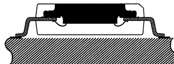
Figure 2. 28 PSOP 2 Board Mounting Options
