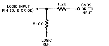
Alternate Logic Interface Figure 1
