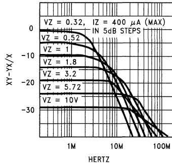
Figure 2. I_Z Divider Frequency Response of XIN for 5 dB D.C. Steps of V_Z
