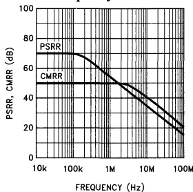
PSRR and CMRR vs Frequency
