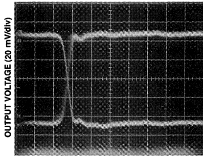
V_S = \pm 5V R_F = R_G = 750\Omega R_L = 150\Omega A_V = +2 TIME (10 ns/div)
