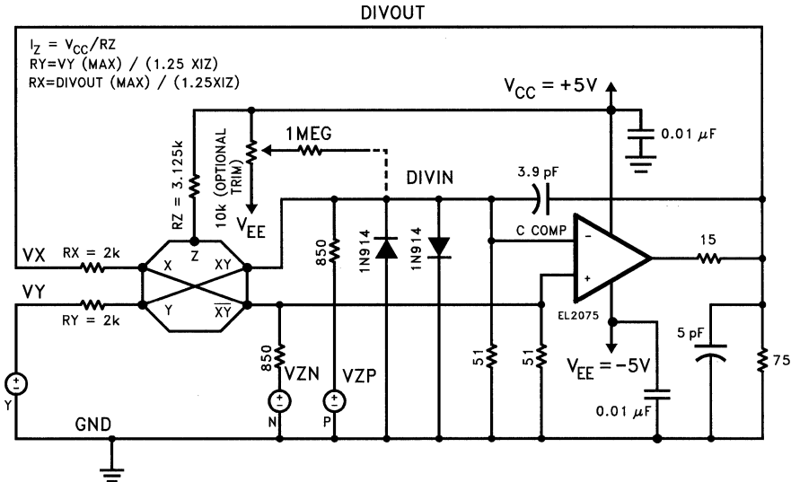
Figure 18. Fast Feedback Divider (with Inverting and Non-inverting Inputs)
