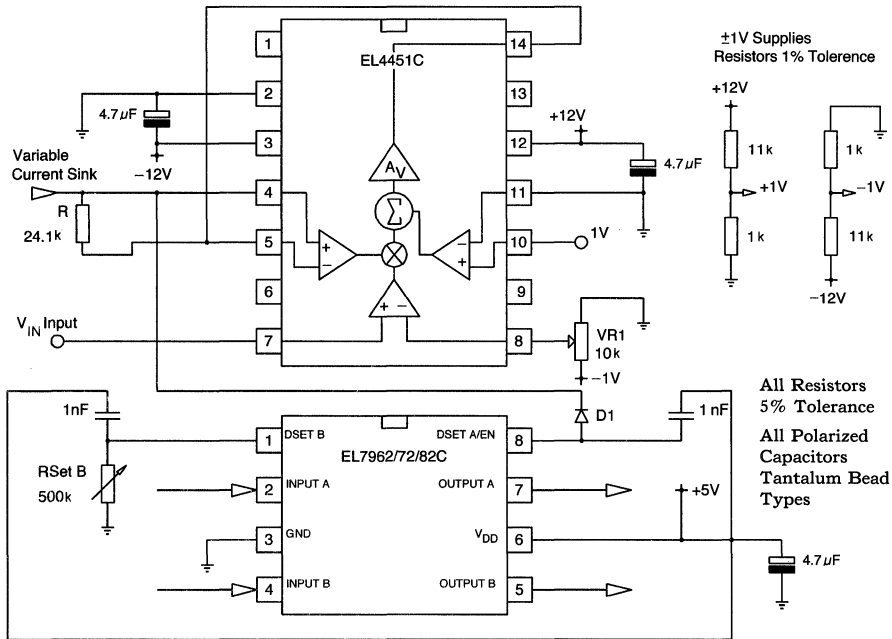
Figure 9. Standalone Variable Current Source
