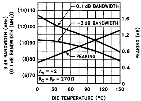
-3 dB Bandwidth, 0.1 dB Bandwidth, and Peaking vs Temperature at V_S \pm 5V
