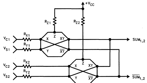
Figure 15. Controlled Signal Summer
