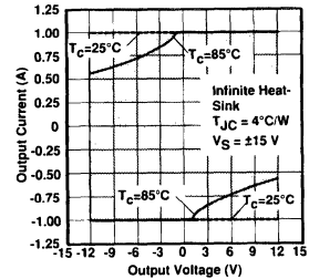
Active operating area
