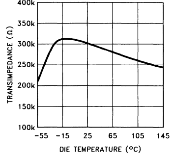
Transimpedance (RO L ) vs Die Temperature
