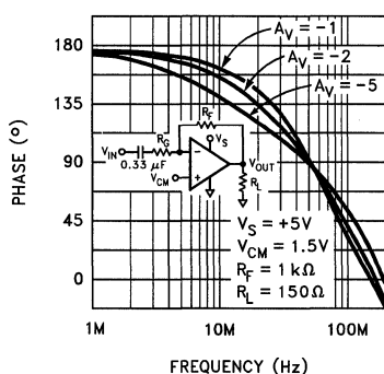
Inverting Frequency Response (Phase)
