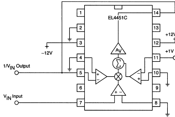
Figure 5. 1/V Converter Using The EL4451C
