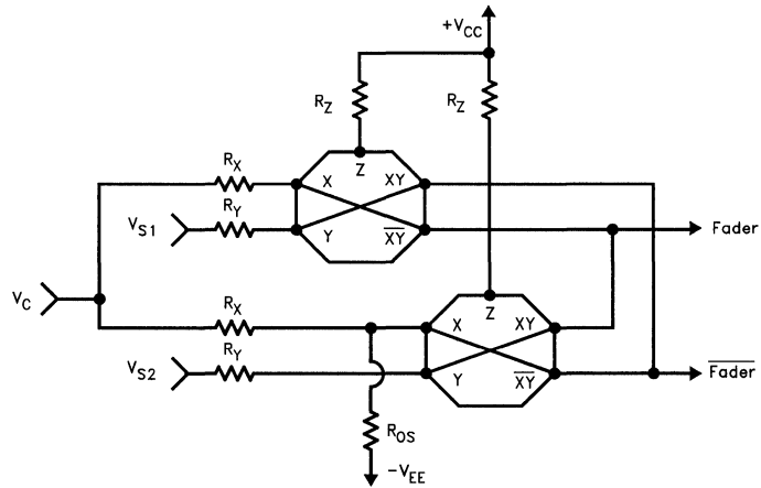
Figure 16. Fader
