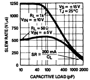
Slew Rate vs Capacitive Load
