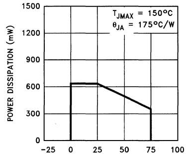
8-Lead SO Maximum Power Dissipation vs Ambient Temperature
