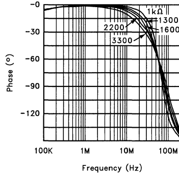
Phase vs Rf at ± 15V
