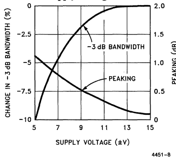
-3 dB Bandwidth and Peaking vs Supply Voltage
