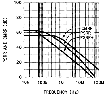
PSRR and CMRR vs Frequency
