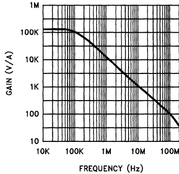
Transimpedance ( R_{OL} )
