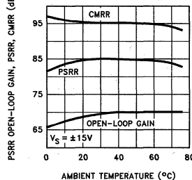
Open-Loop Gain PSRR and CMRR vs Temperature
