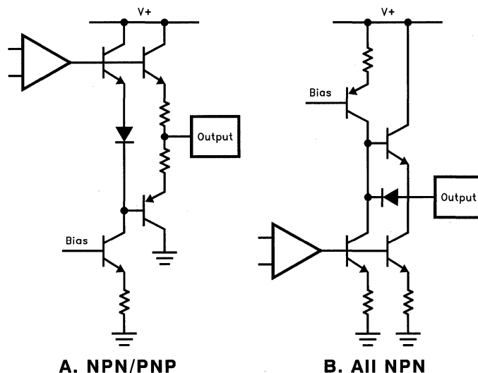
Figure 2. Typical Single-Supply Output Stages
