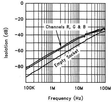
Disabled Isolation Test at \pm 15V
