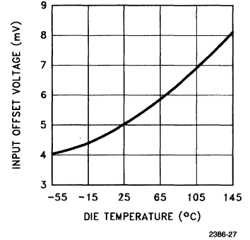
Input Offset Voltage vs Die Temperature
