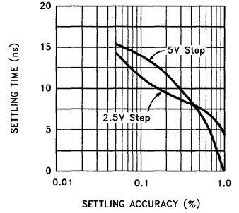
Settling Time vs Settling Accuracy
