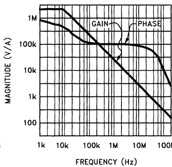
Transimpedance ( R_{OL} ) vs Frequency
