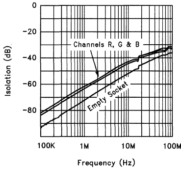
Disabled Isolation Test at \pm 5V
