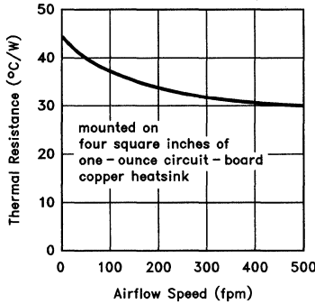
Mounted Thermal Resistance of Package vs Airflow Speed
