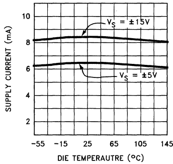
Supply Current vs Die Temperature
