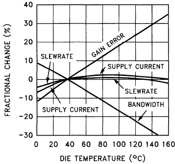
Change in 100% Gain Error, Supply Current, Slewrate and Bandwidth over Temperature
