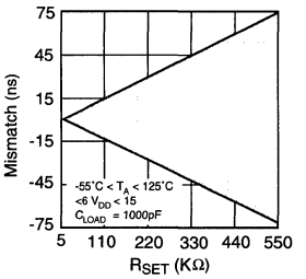
Output Rising Edge Delay Channel to Channel Mismatch
