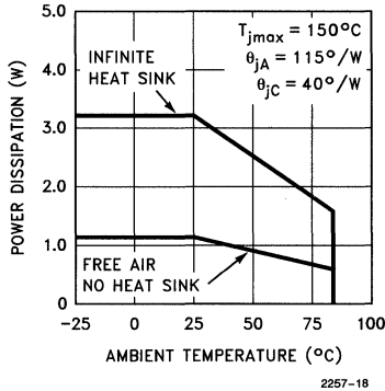
16-Lead Plastic SO Maximum Power Dissipation vs Ambient Temperature
