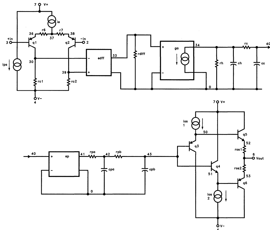
EL2044C Model
