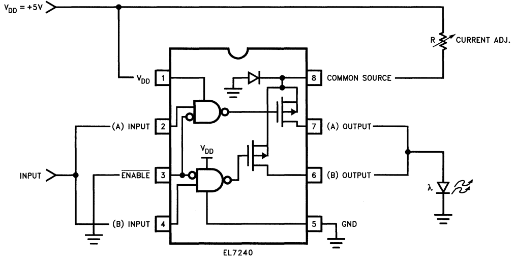
High Current LED/Laser Diode Driver
