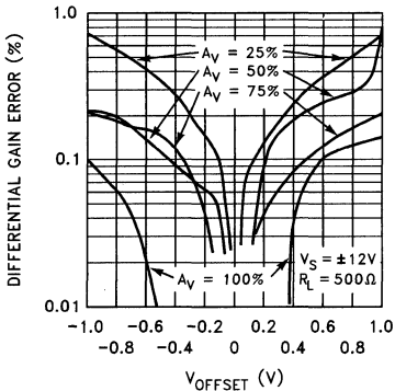
Differential Gain Error vs V_{offset} for Gain = 100%, 75%, 50% and 25%. F = 3.58 MHz
