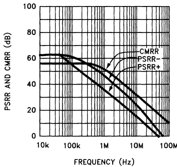
PSRR and CMRR vs Frequency
