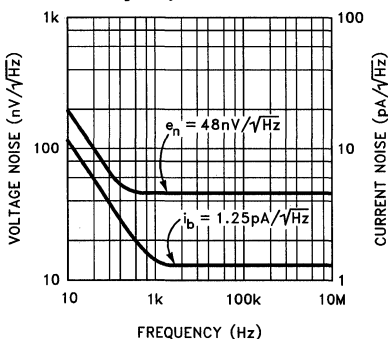
Voltage and Current Noise vs Frequency
