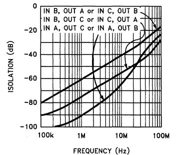
Channel to Channel Isolation vs Frequency
