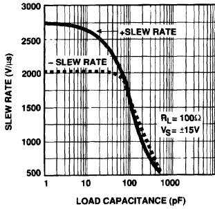
Slew Rate vs Load Capacitance
