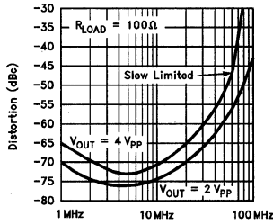
3rd Harmonic Distortion
