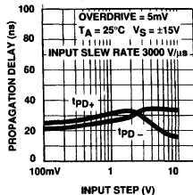
Propagation Delay vs Input Step
