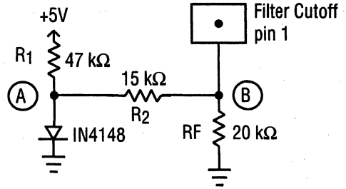
Figure 3. EL4583C Compensation Network
