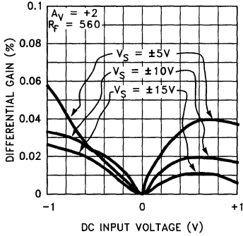
Differential Gain vs DC Input Voltage, R_L = 150
