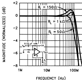
Frequency Response for Various R_L
