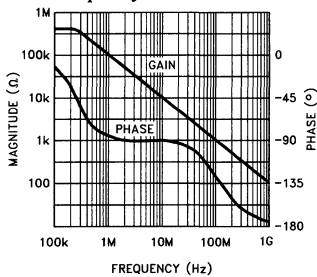
Transimpedance ( R_{OL} ) vs Frequency
