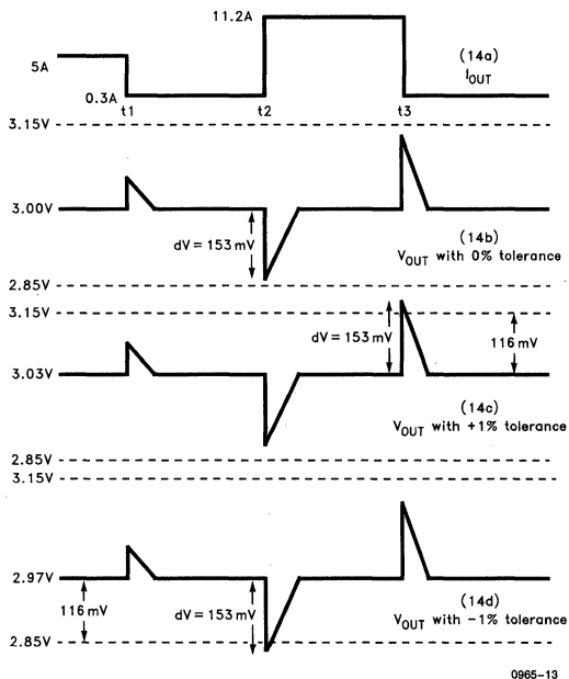
Figure 14. Output Voltage Variation with Traditional Control Scheme
