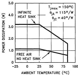
16-Pin Plastic DIP Maximum Power Dissipation vs Ambient Temperature
