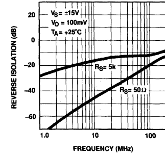
Reverse Isolation vs Frequency
