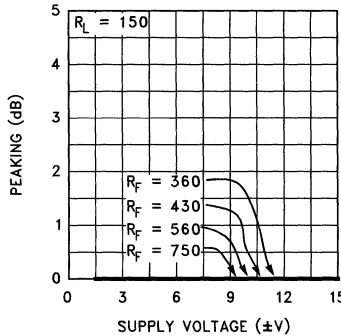
Peaking vs Supply Voltage for A_V = +10
