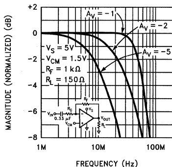
Inverting Frequency Response (Gain)
