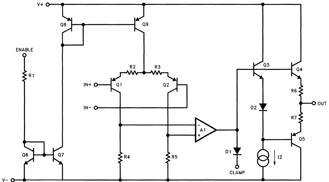
Simplified Schematic (one channel)
