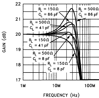
Frequency Response for Various R_L , C_L , V_S = \pm 5\text{ V}
