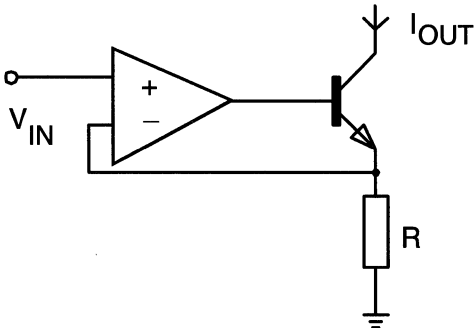
Figure 6. Voltage To Current Converter
