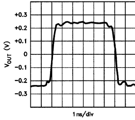
Small Signal Pulse Response
