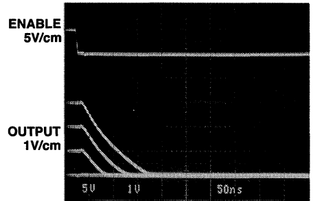
Disable Response for a Family of DC Inputs
