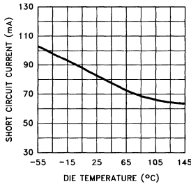
Short Circuit Current vs Die Temperature
