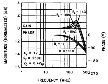
Frequency Response for Various R_L s
