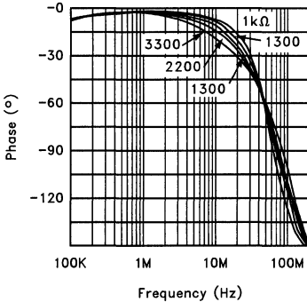
Phase vs Rf at ± 5V
