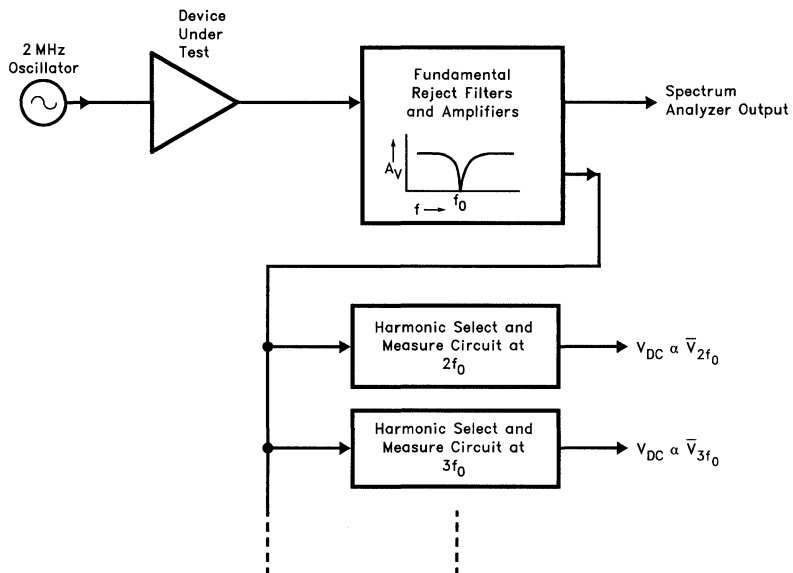
Figure 1. Block Diagram of Distortion Measurement System
