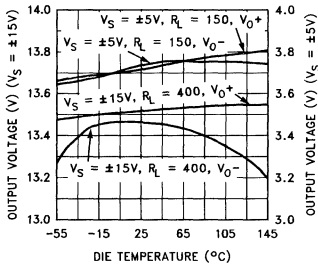
Output Voltage Swing vs Die Temperature
