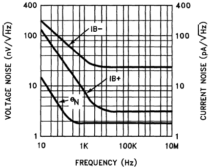
Voltage and Current Noise vs Frequency
