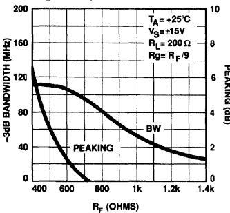
Bandwidth and Peaking vs R_F for A_V = +10
