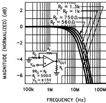
Frequency Response for A_V = +10 and for Various R_F Values
