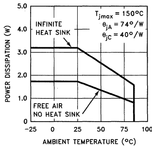
16-Lead SO Maximum Power Dissipation vs Ambient Temperature
