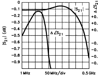
Gain Flatness & Deviation from Linear Phase
