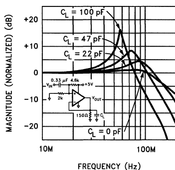
Frequency Response for Various C_L
