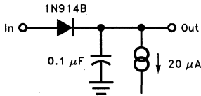
Figure 1. Simple Diode Peak Detector
