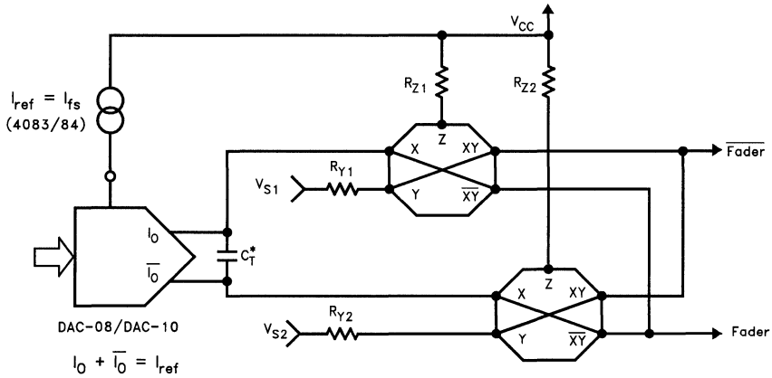
Figure 17. Digitally Controlled Fader
