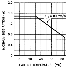
Maximum Power Dissipation vs Ambient Temperature—16-Pin PDIP
