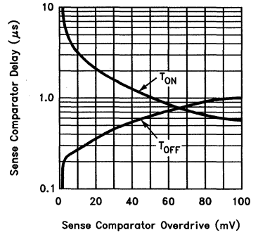
Sense Comparator Delay vs Overdrive
