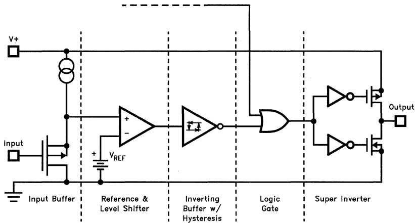
Simplified Schematic
