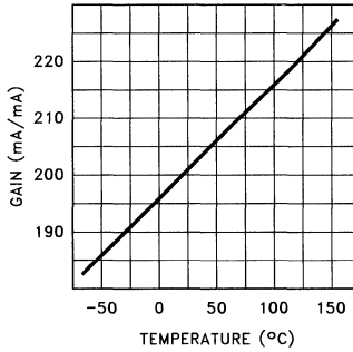
Write Current Gain vs Temperature (VWRPWR = 2.88V, RWRDOUT = 3.6 kΩ)
