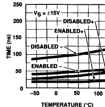
Enabled/Disabled Time vs Temperature
