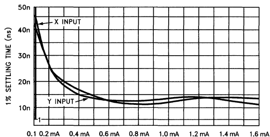
Figure 7. ( I_X , I_Y 1% Settling Time vs I_Z )
