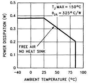
5-Lead Plastic SOT23 Maximum Power Dissipation vs Ambient Temperature
