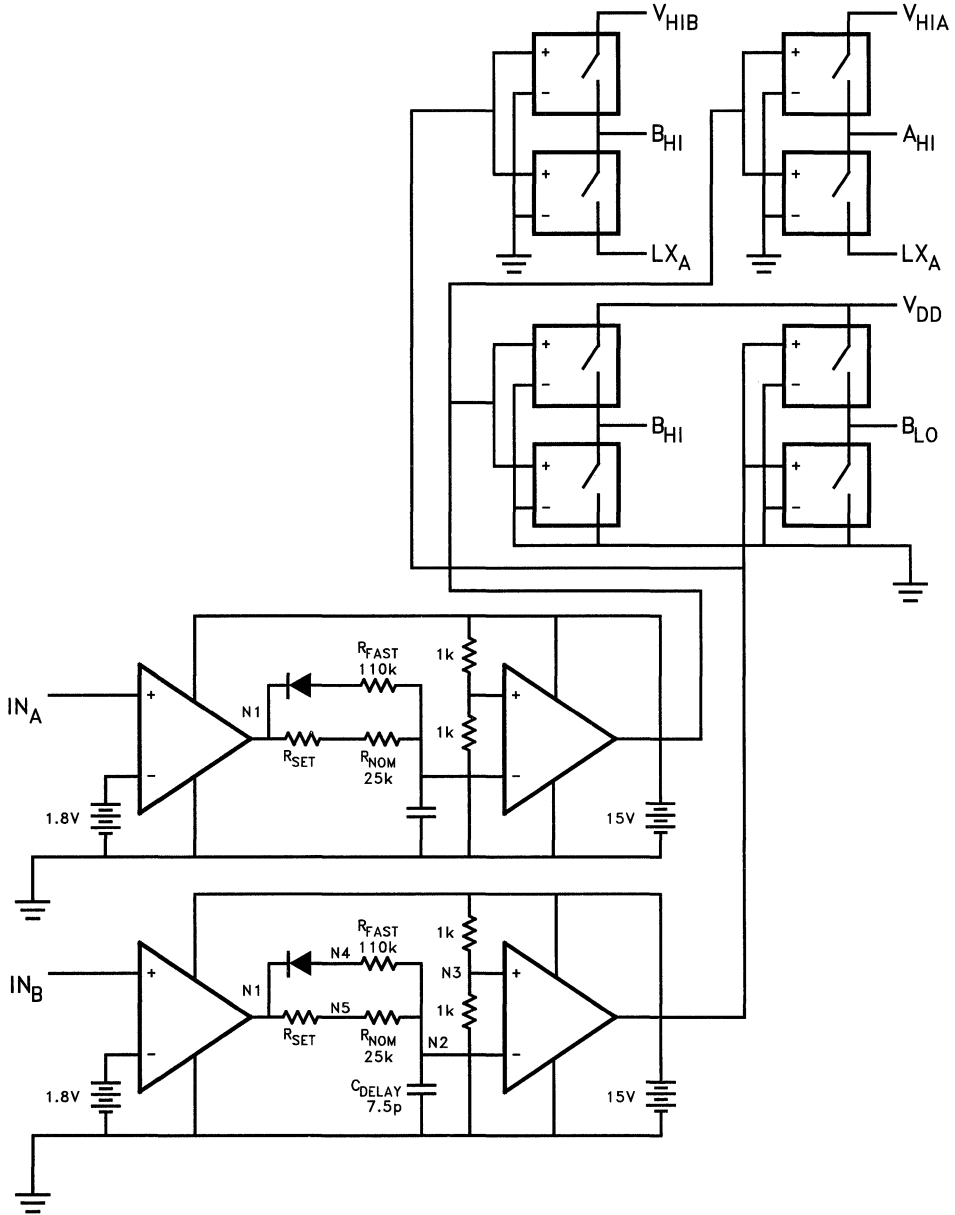
EL7661C Macromodel Schematic
