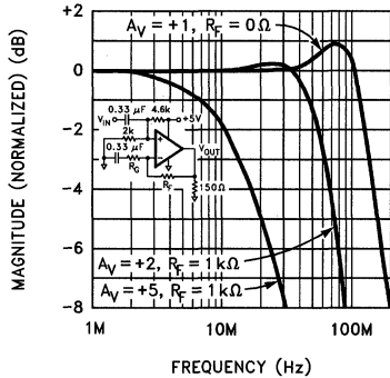
Non-Inverting Frequency Response (Gain)
