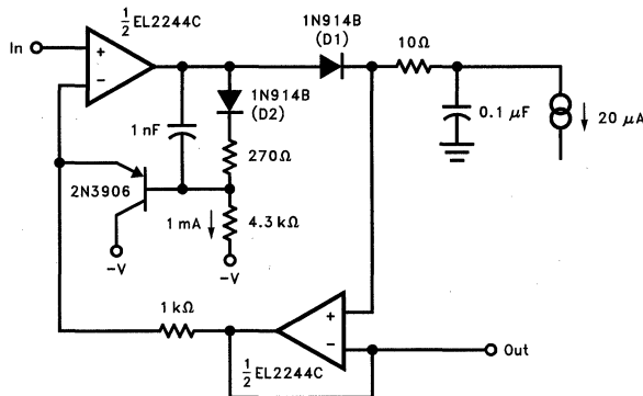
Figure 3. Diode with Feedback
