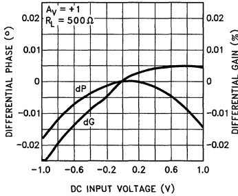
Differential Gain and Phase vs DC Input Voltage at 3.58 MHz
