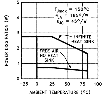
8-Lead Plastic SO Maximum Power Dissipation vs Ambient Temperature
