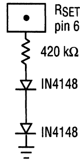
Figure 1. EL4581C Compensation Network
