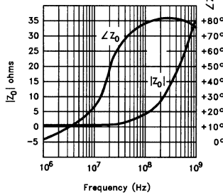
Output Impedance
