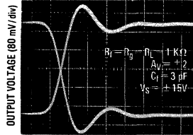
TIME (5 ns/div)
