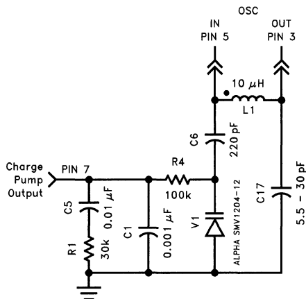
(3) LC Tank
