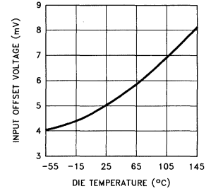
Input Offset Voltage vs Die Temperature
