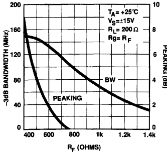
Bandwidth and Peaking vs R_F for A_V = +2
