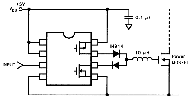
Resonant Gate Driver
