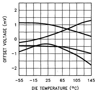
Offset Voltage vs Die Temperature (4 Samples)
