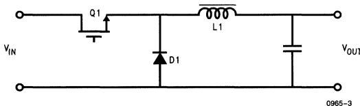
Figure 3. Basic Buck Converter Topology
