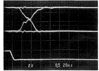
2021-8 Family of output waveshapes from high-impedance H, L to active H, L.
