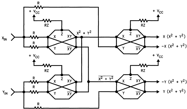
Figure 12. CRT Geometry Correction
