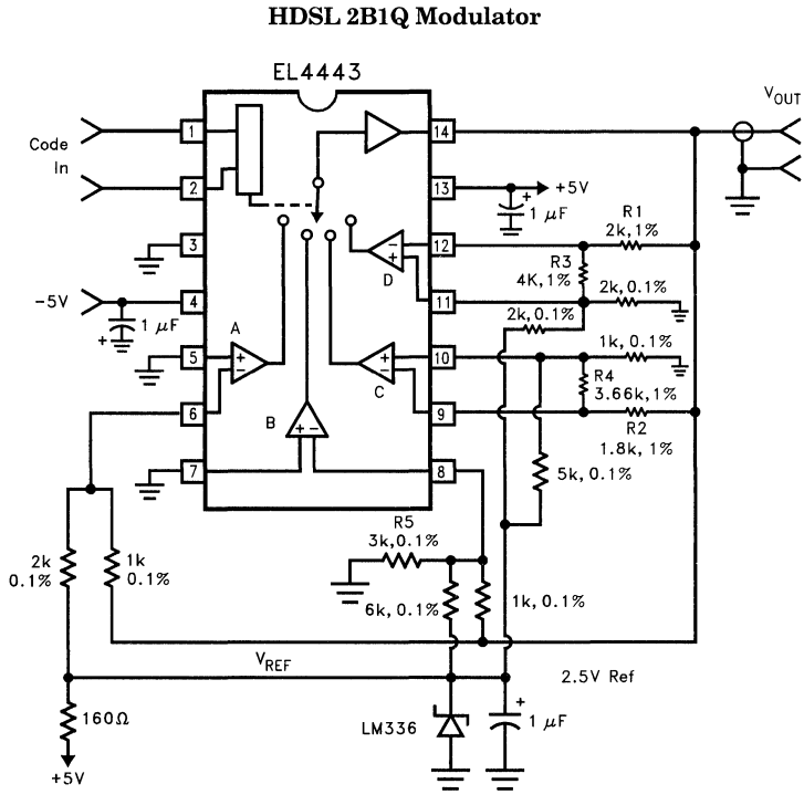
Figure 3. More Accurate 2B1Q Modulator with EL4443
