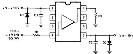
EL2033 DIP
