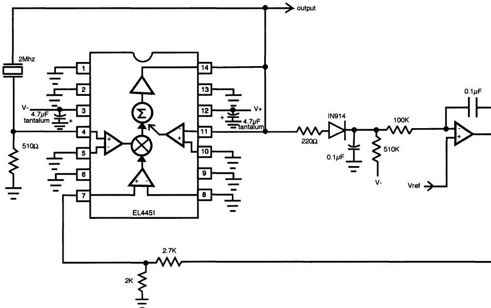
Basic Oscillator with Amplitude Stabilization Loop
