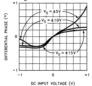
Differential Phase vs DC Input Voltage RL = 150
