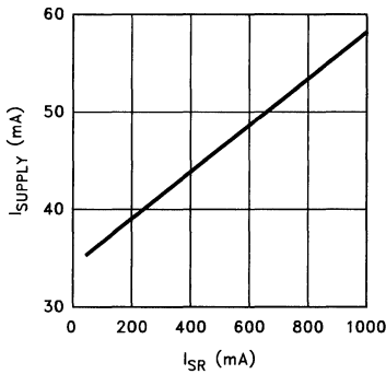
Supply Current vs I_{SR}
