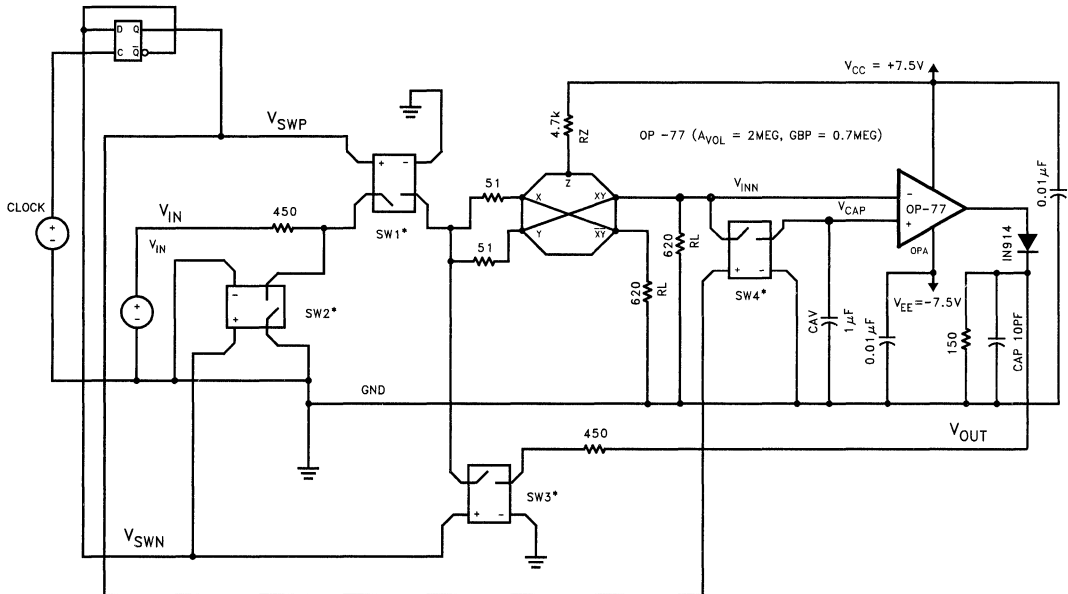
Figure 10. Single Multiplier Switched RMS Circuit RMS #3 (SW1-4 are Siliconix SD5000 Series Quad DFETS for F IN > 10 MHz)
