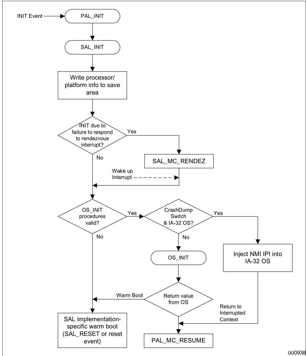
Figure 13-5. INIT Flow
