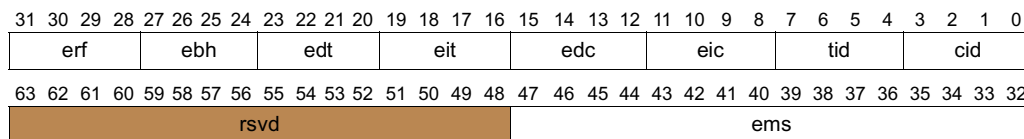
Figure 11-36. level_index Layout
