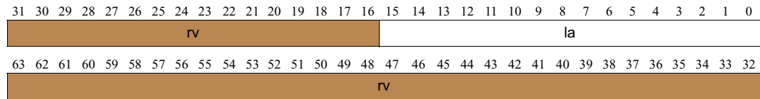
Figure 11-34. Layout of proc_n_log_info2 Return Value
