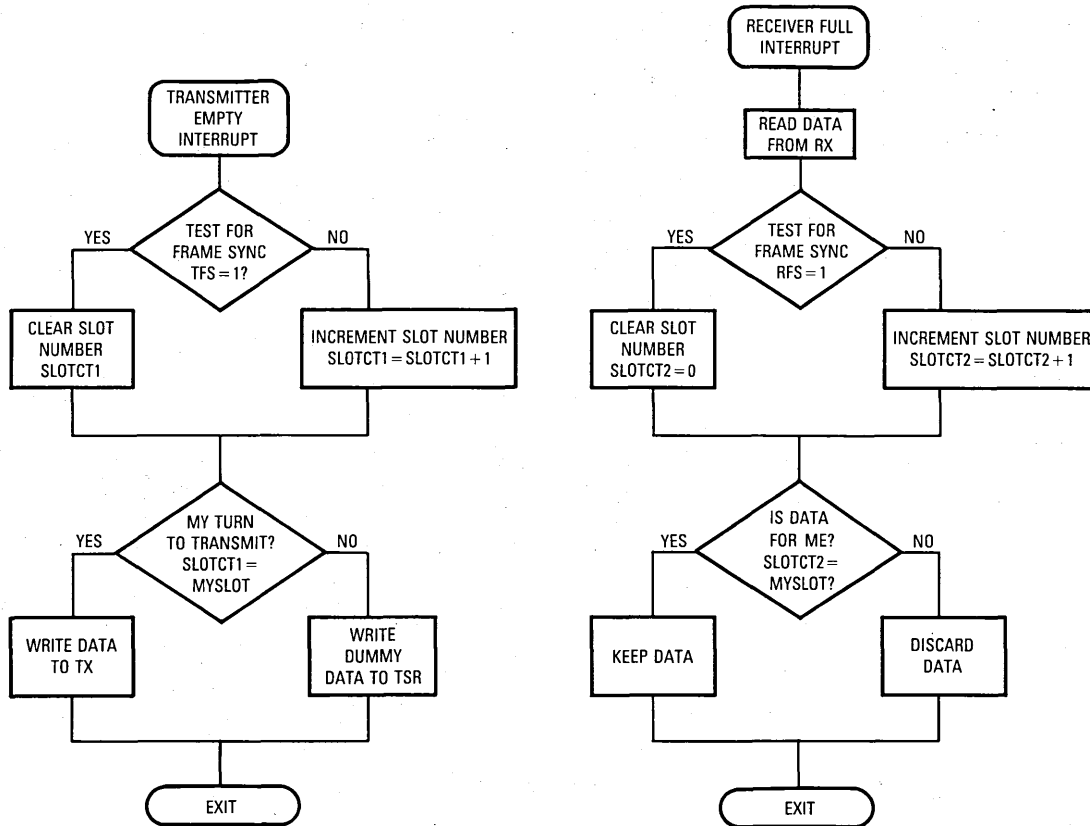
Figure 11-75. TDM Network Software Flowchart
