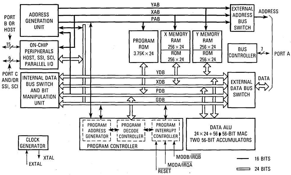
Figure 1-5. DSP56000 Block Diagram
