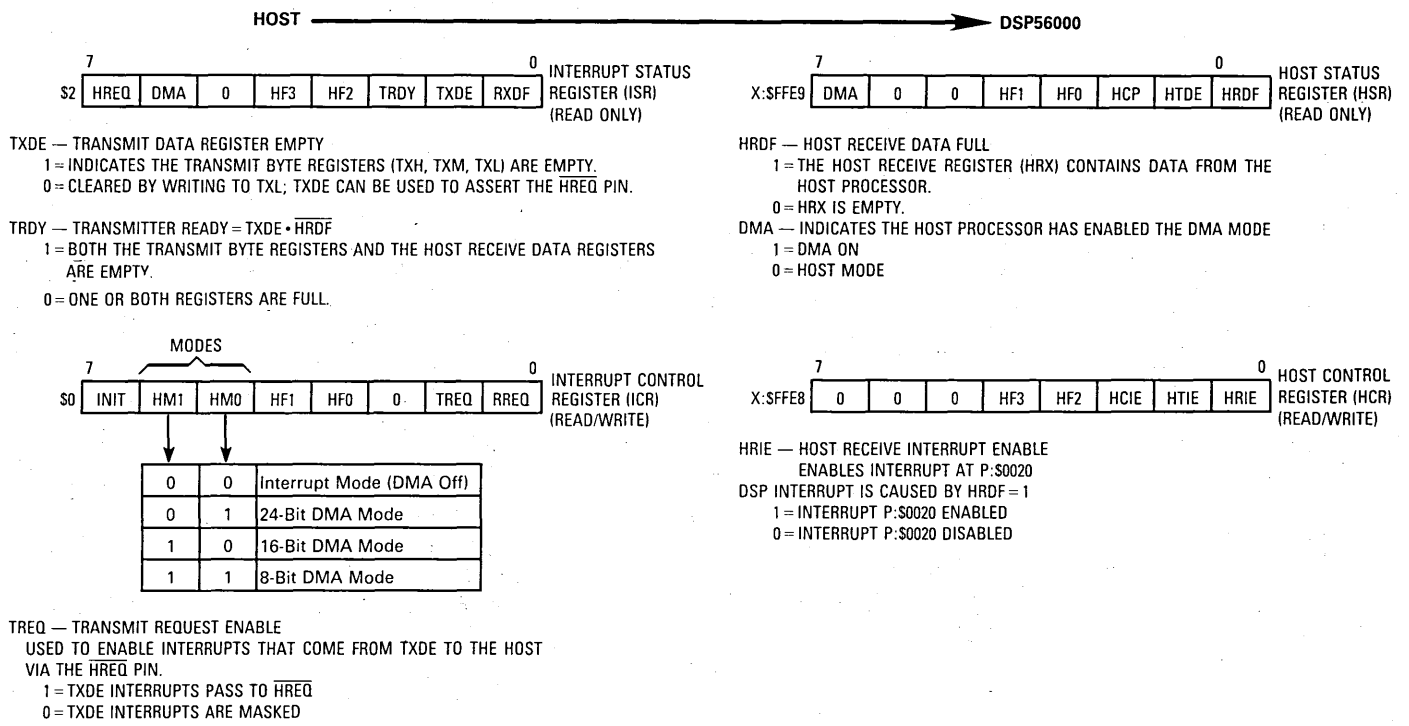
Figure 10-23. Bits Used for Host-to-DSP Transfer
