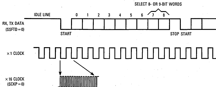
Figure 11-12. 16× Serial Clock
