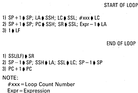
Figure 7-13. Hardware DO Loop
