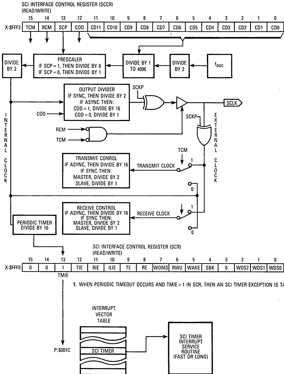
Figure 11-36. SCI Timer Operation
