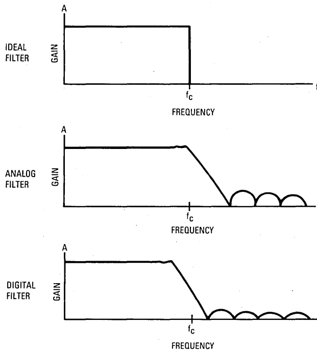
Figure 1-2. Digital Signal Processing
