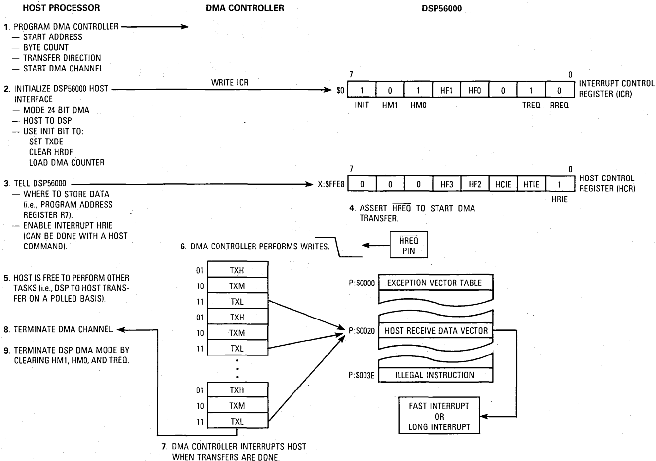
Figure 10-38. Host-to-DSP DMA Procedure
