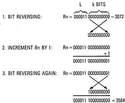
Figure 5-14. Bit-Reverse Address Calculation Example
