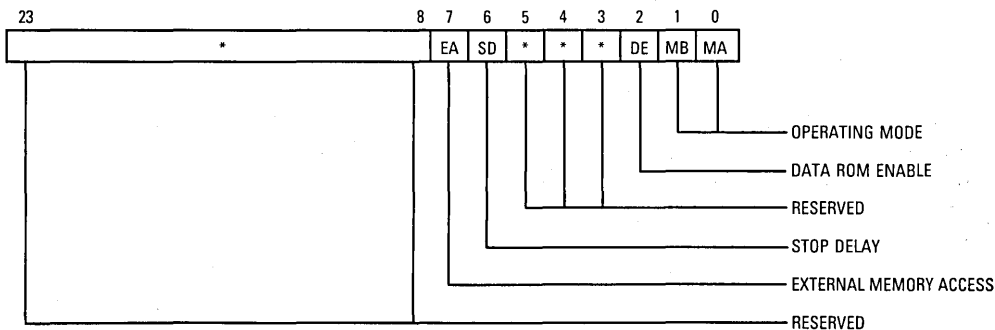
Figure 6-7. OMR Format
