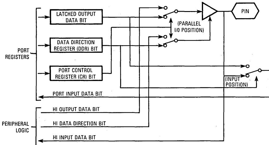
Figure 10-4. Port B I/O Pin Control Logic
