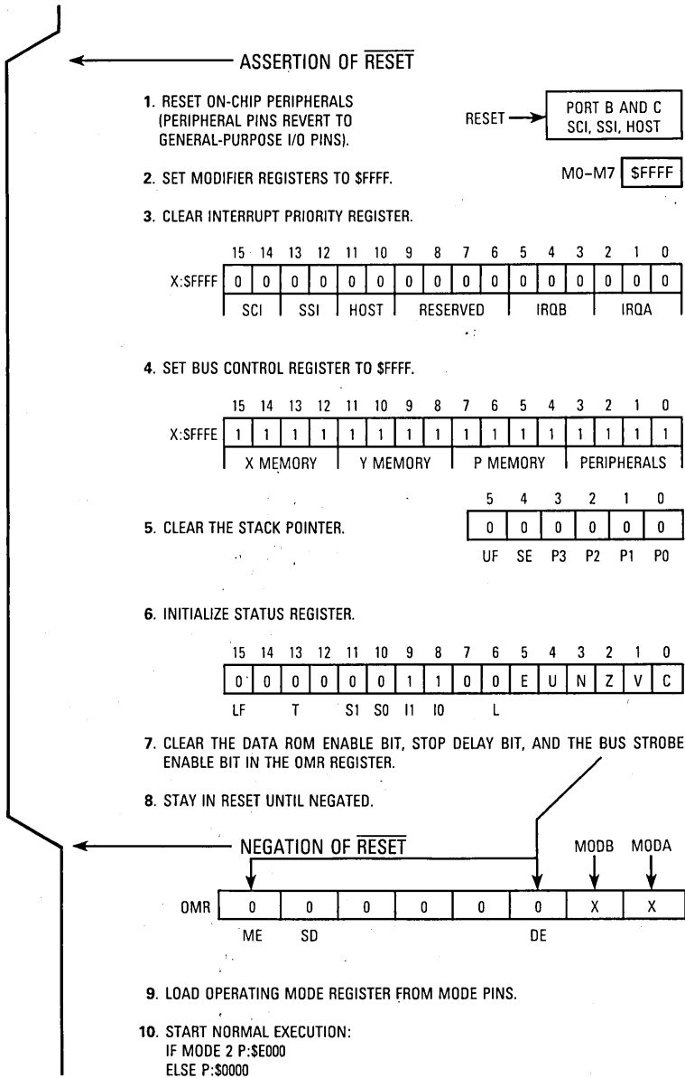
Figure 8-13. Reset Sequence
