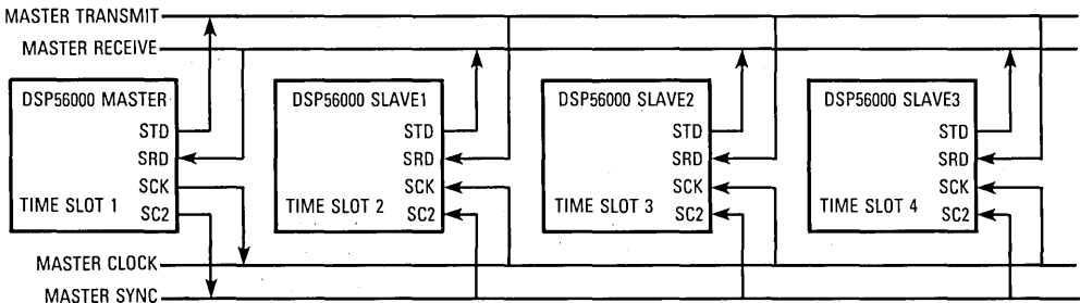
Figure 11-74. Network Mode Example
