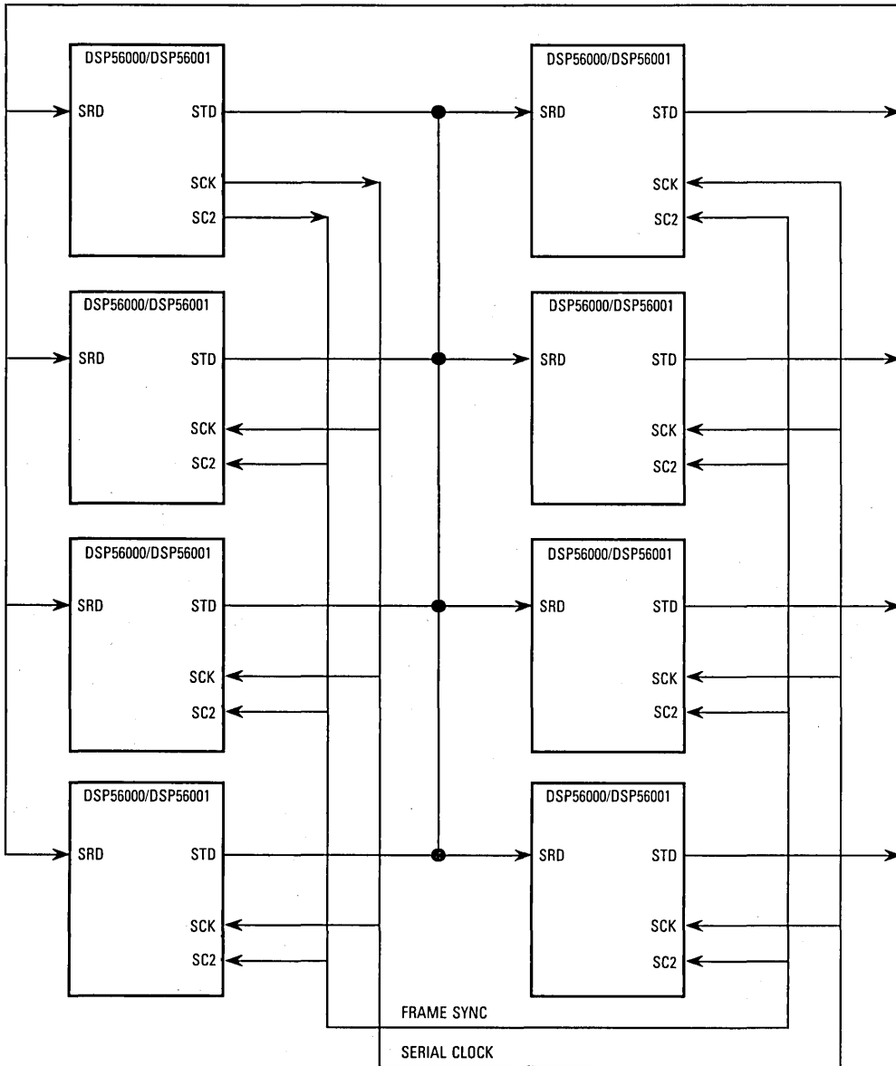
Figure 11-92. SSI TDM Connected Parallel Processing Array
