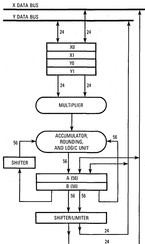
Figure 4-2. Data ALU
