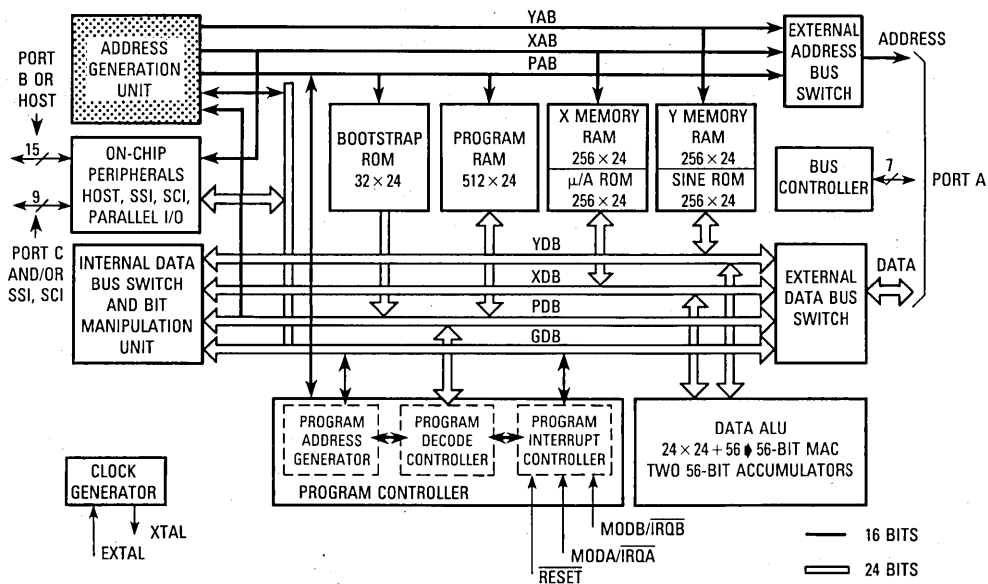
Figure 5-1. DSP56001 Block Diagram
