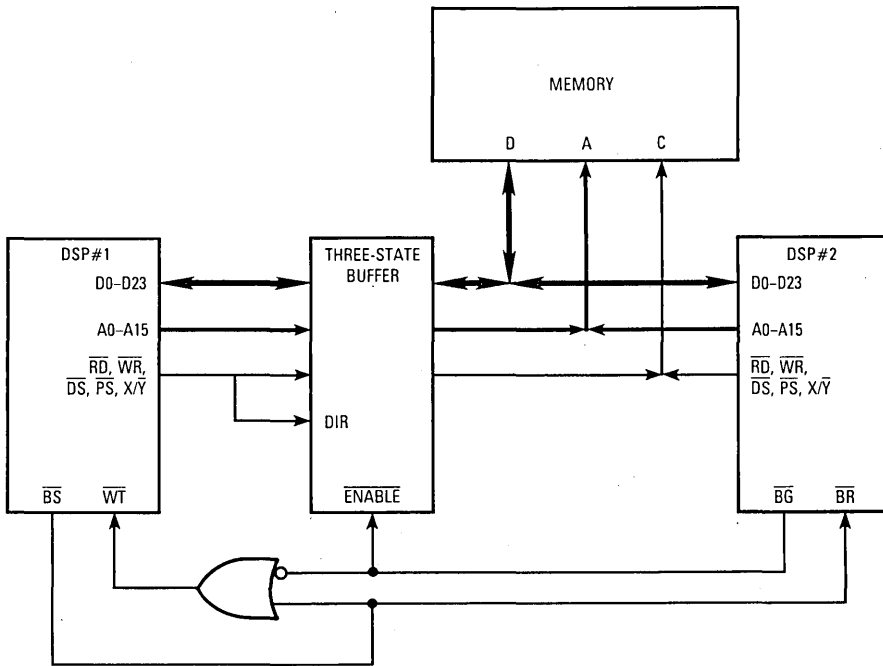
Figure 9-17. Bus Arbitration Using \overline{BR}/\overline{BG} and \overline{BS}/\overline{WT} with No Overhead
