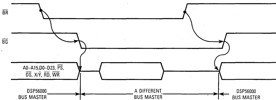
Figure 9-13. Bus Request/Bus Grant Sequence
