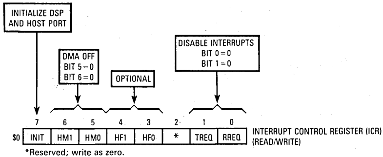
Figure 10-21(b). HI Initialization — Host Side, Polling Mode
