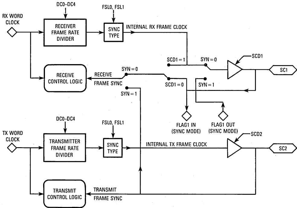
Figure 11-42. SSI Frame Sync Generator Functional Block Diagram
