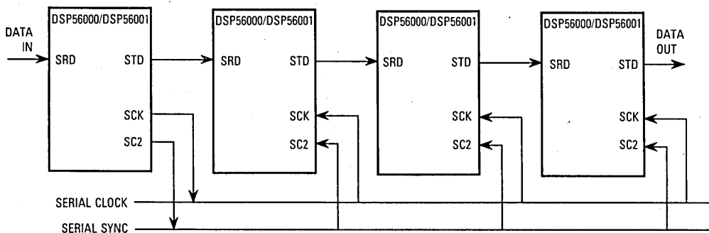
Figure 11-90. SSI Cascaded Multi-DSP System
