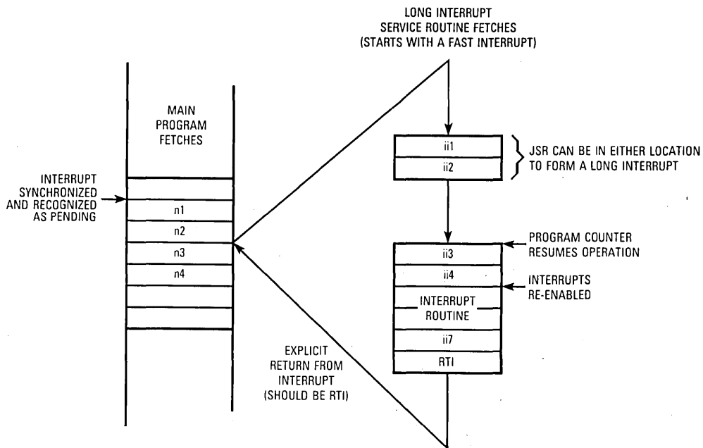
(a) Instruction Fetches from Memory
