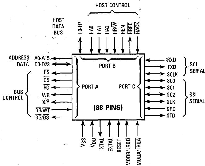
Figure 2-3. DSP56000/DSP56001 Functional Signal Groups
