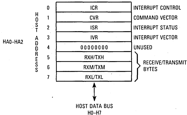
Figure 10-14. HI Register Map
