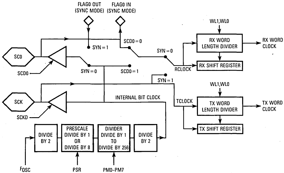
Figure 11-41. SSI Clock Generator Functional Block Diagram
