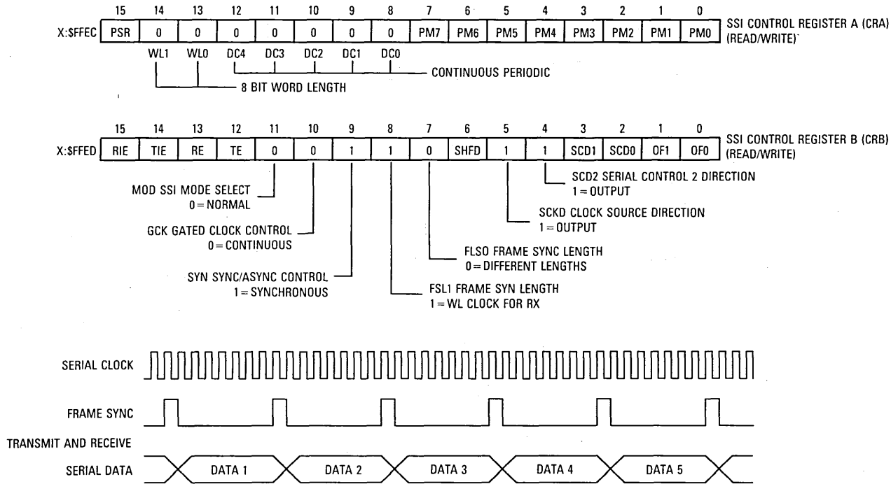
Figure 11-69. Normal Mode Initialization for FSL1 = 1 and FSL0 = 0
