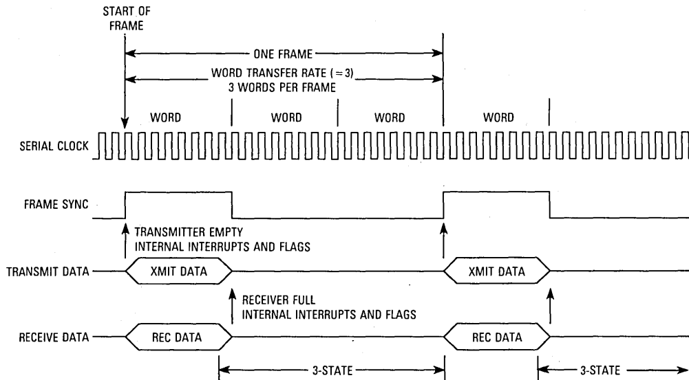
Figure 11-61. Synchronous Communication
