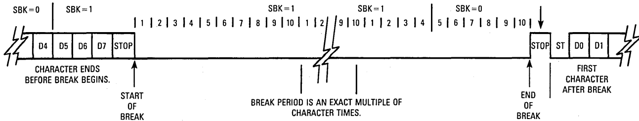
Figure 11-28. Transmitting Marks and Spaces
