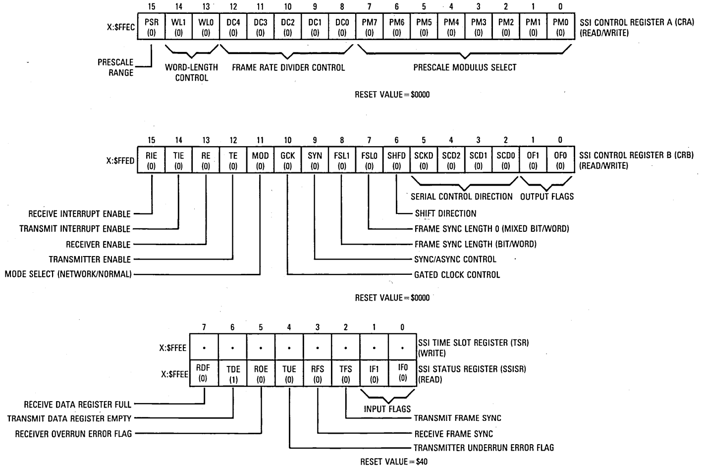
Figure 11-43. SSI Interface Programming Model — Control and Status Registers
