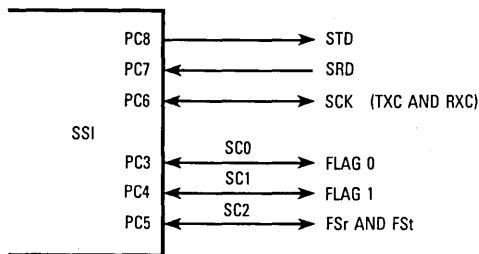
Figure 11-65. Continuous Clock — Synchronous Operation
