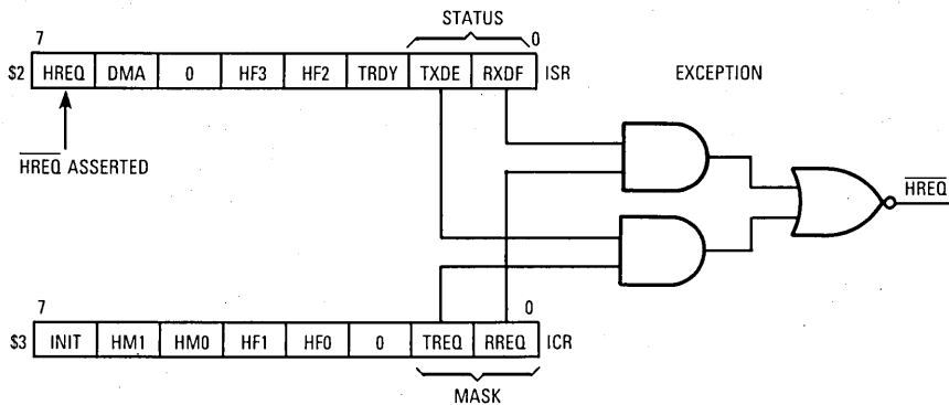
Figure 10-17. HI Interrupt Structure
