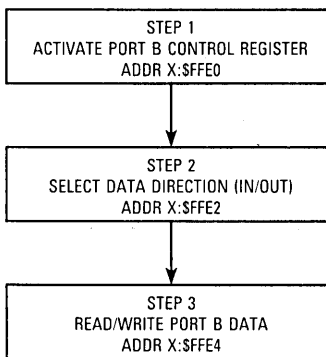
Figure 10-7. Port B Configuration Flowchart
