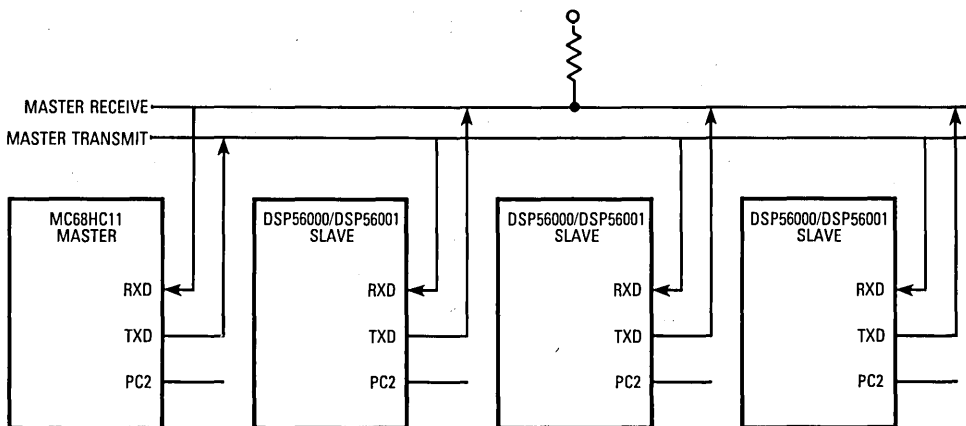
Figure 11-40. Master-Slave System Example
