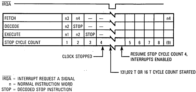
Figure 8-17. STOP Instruction Sequence
