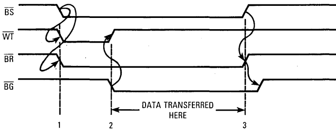
Figure 9-18. Two DSPs with External Bus Arbitration Timing
