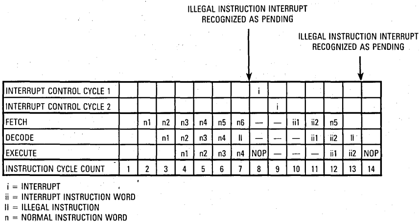
(b) Program Controller Pipeline
