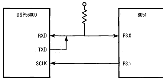
Figure 11-38. Synchronous Mode Example
