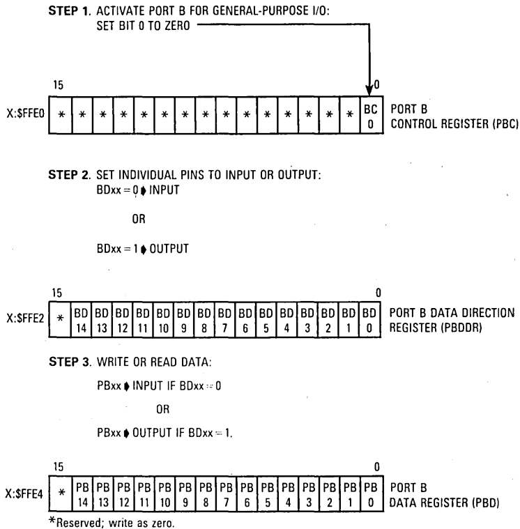
Figure 10-8. I/O Port B Configuration
