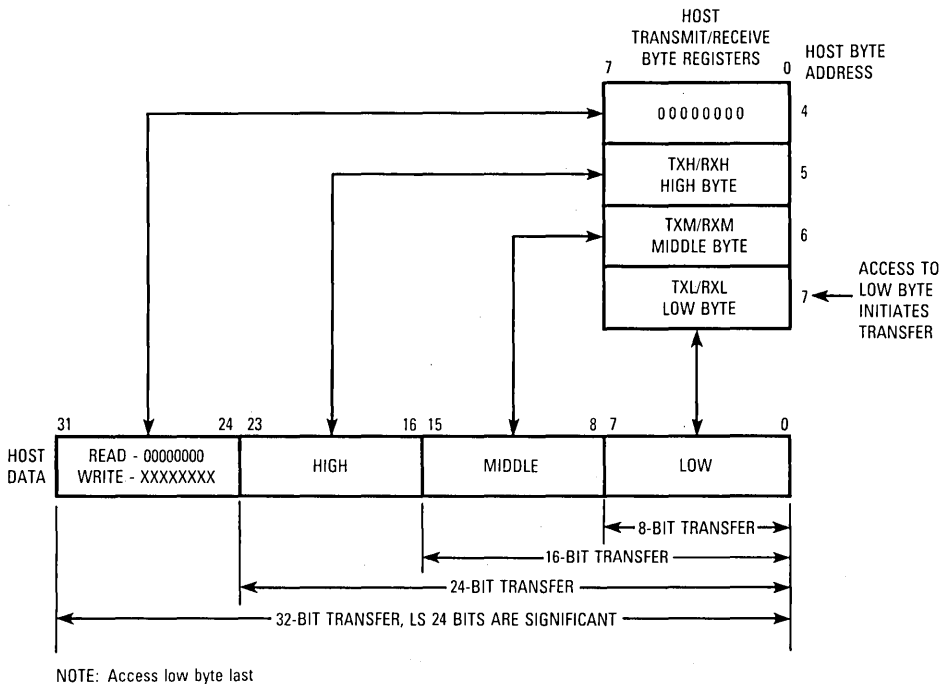
Figure 10-30. Transmit/Receive Byte Registers
