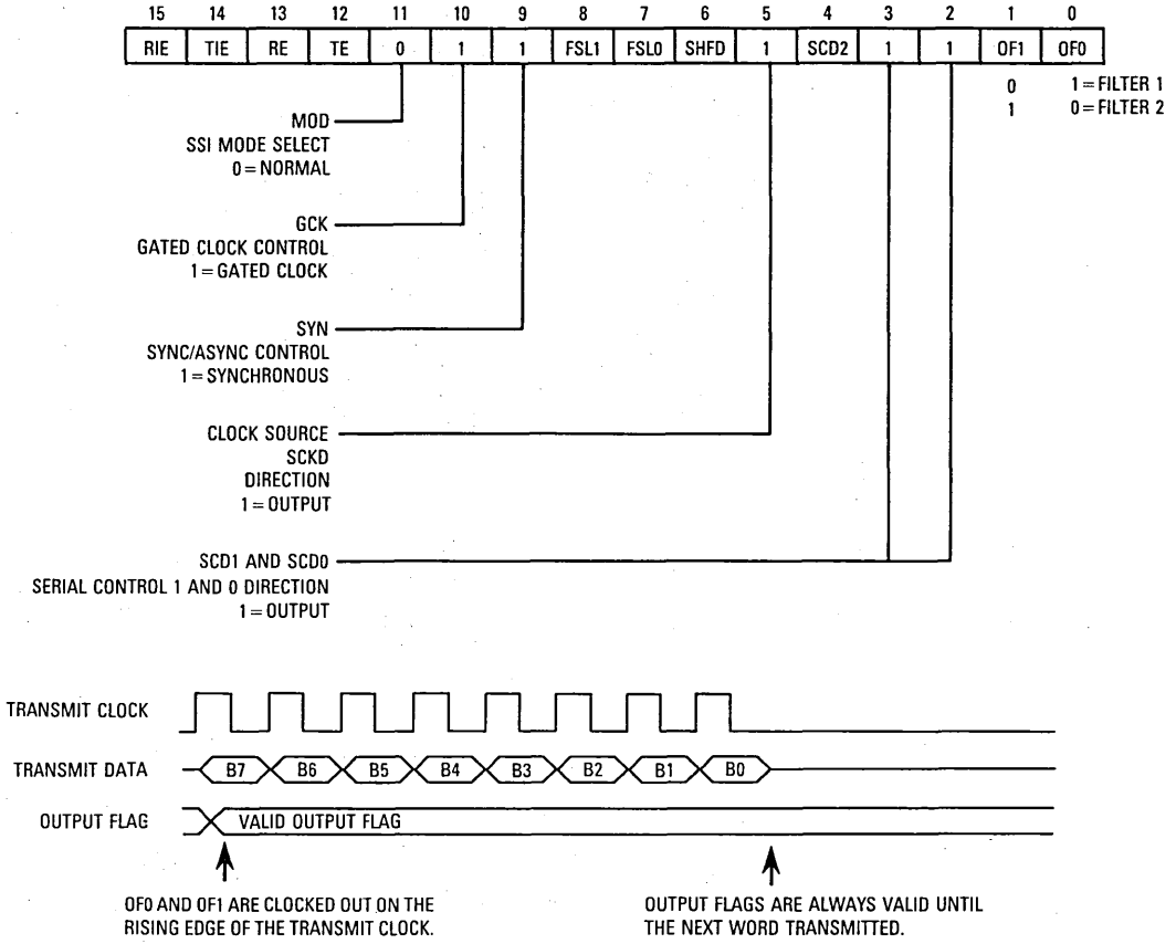
Figure 11-88. Output Flag Initialization
