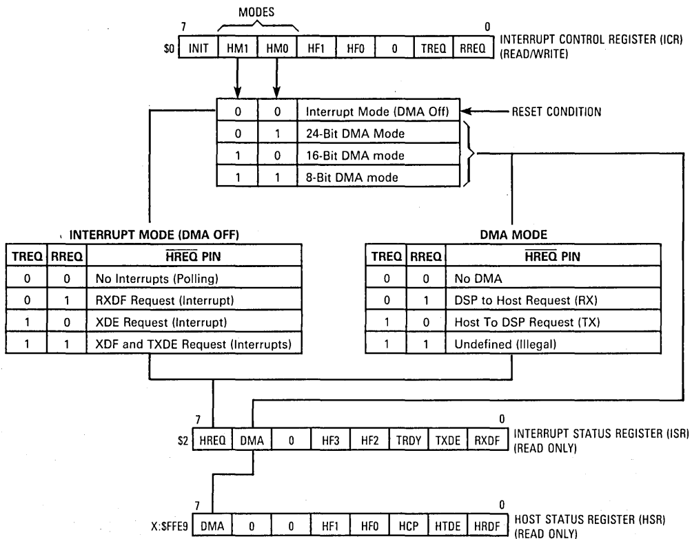
Figure 10-39. Host Bits with TREQ and RREQ
