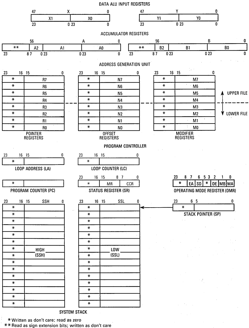
Figure 7-1. DSP56000/DSP56001 Central Processor Programming Model
