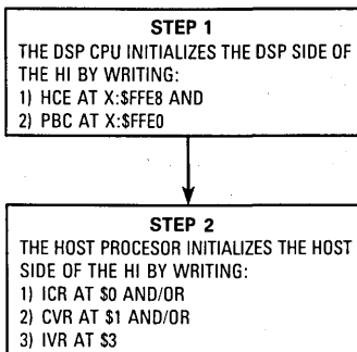
Figure 10-19. HI Initialization Flowchart
