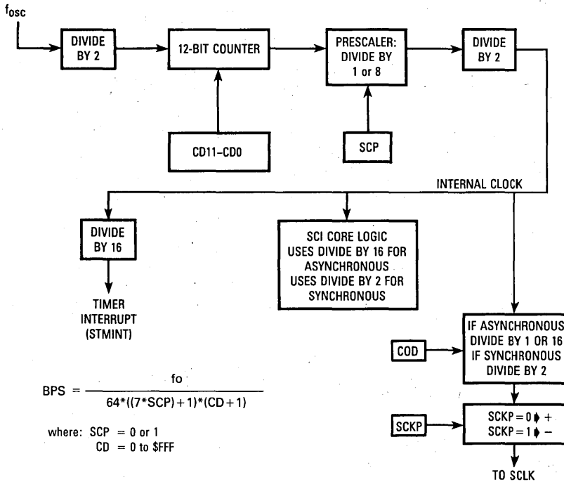
Figure 11-13. SCI Baud Rate Generator
