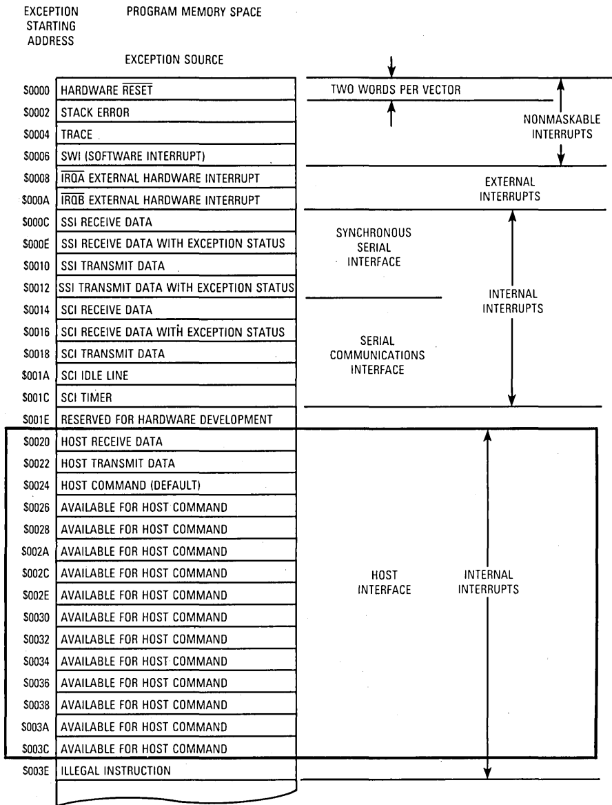
Figure 10-27. Vector Table of Exception Sources
