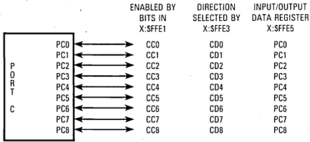
Figure 11-2. Parallel Port C Pinout
