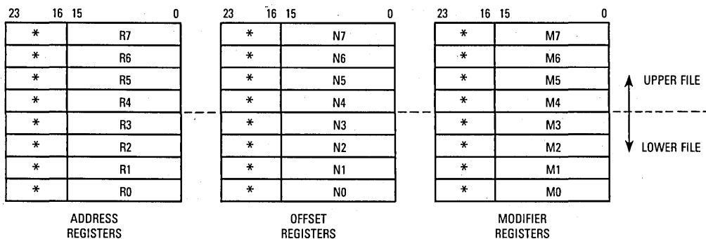
Figure 5-3. AGU Programming Model
