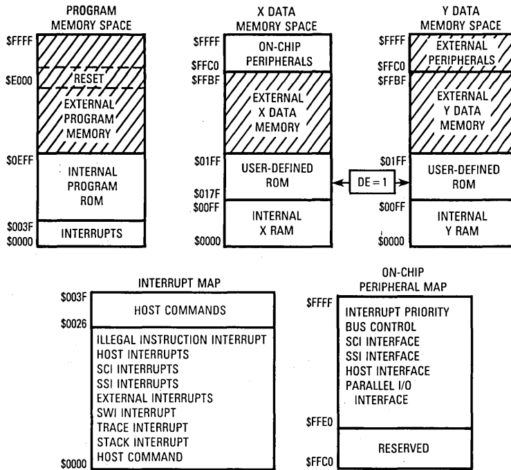
Figure 3-3. Memory Map for DSP56000 Mode 2: Normal Expanded Mode
