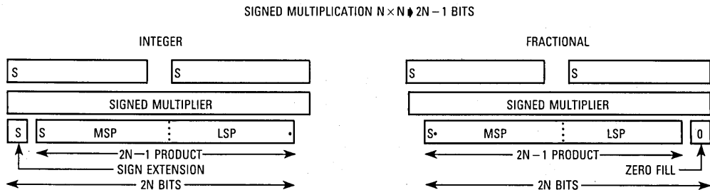
Figure 4-8. Integer/Fractional Multiplication Comparison
