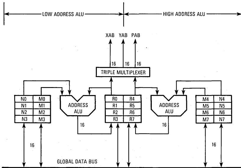
Figure 5-2. AGU Block Diagram
