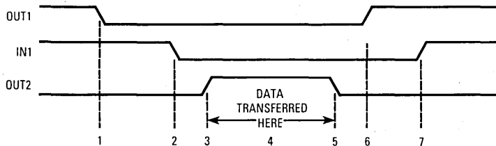
Figure 9-15. Two DSPs with External Bus Arbitration Timing
