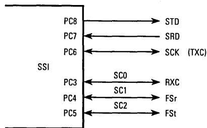
Figure 11-66. Continuous Clock — Asynchronous Operation
