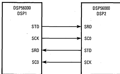
Figure 11-79. On-Demand Example
