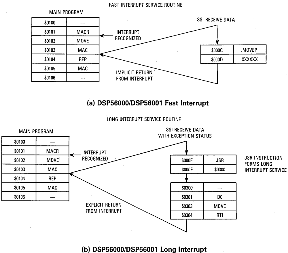
Figure 6-3. Fast and Long Interrupt Examples
