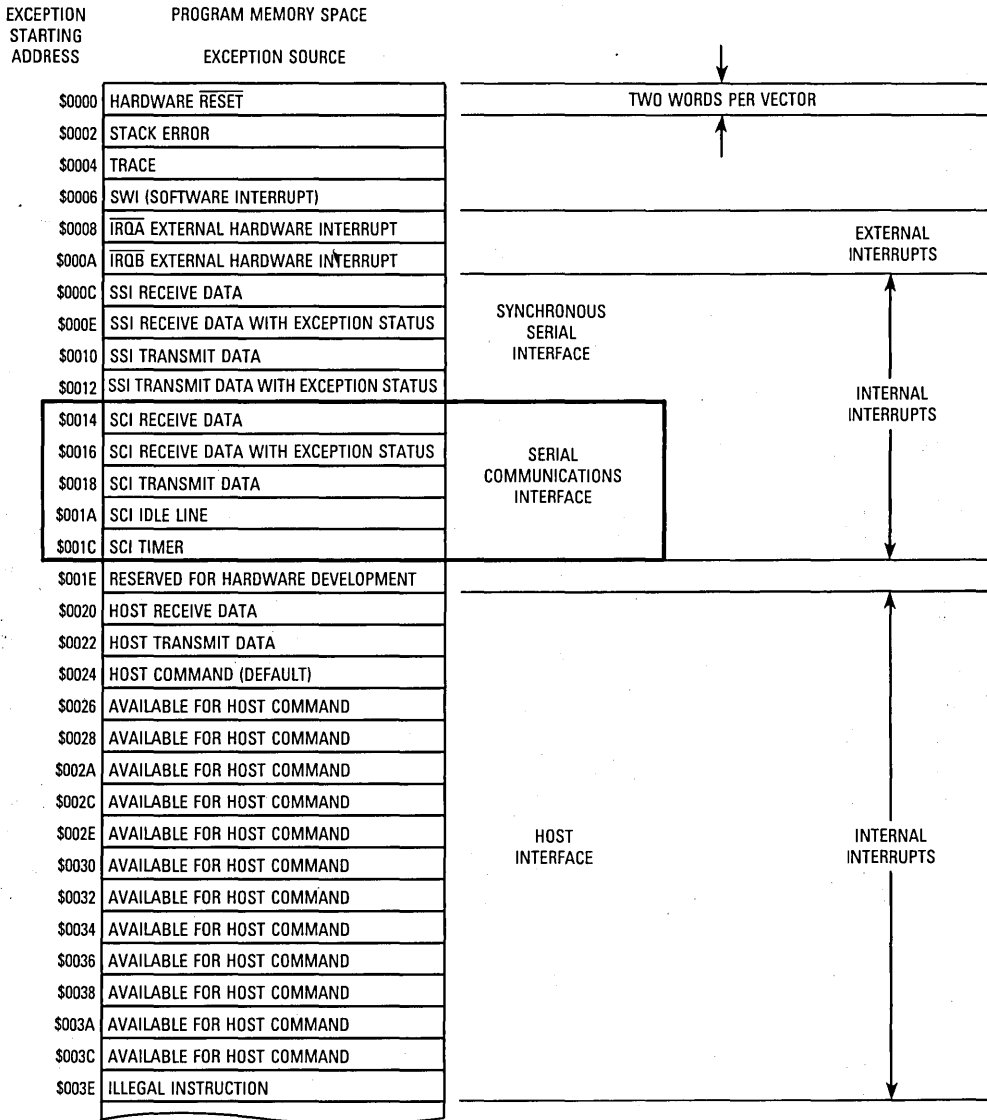
Figure 11-17. SCI Exception Vector Locations
