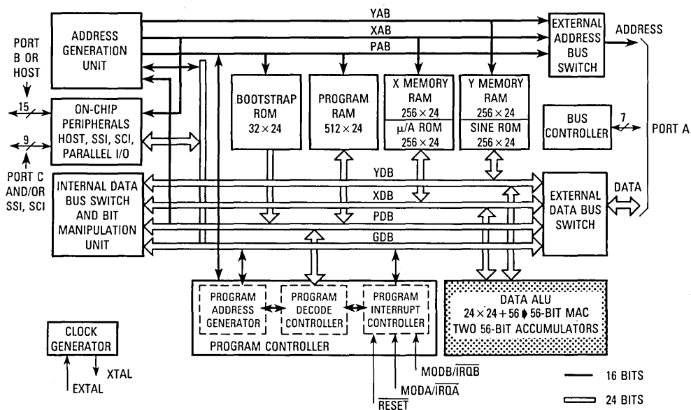
Figure 4-1. DSP56001 Block Diagram
