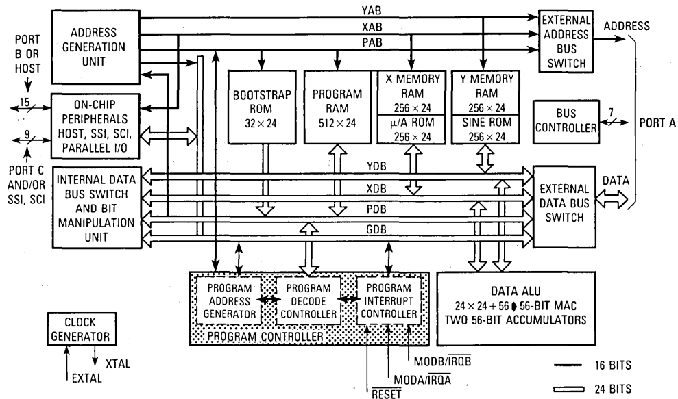
Figure 6-1. DSP56001 Block Diagram
