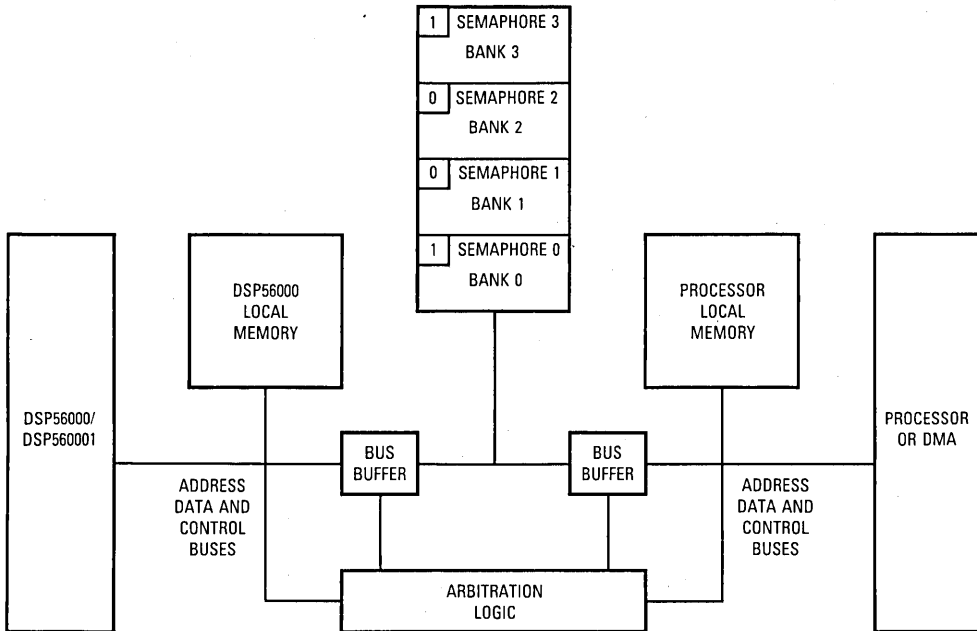
Figure 9-19. Signaling Using Semaphores
