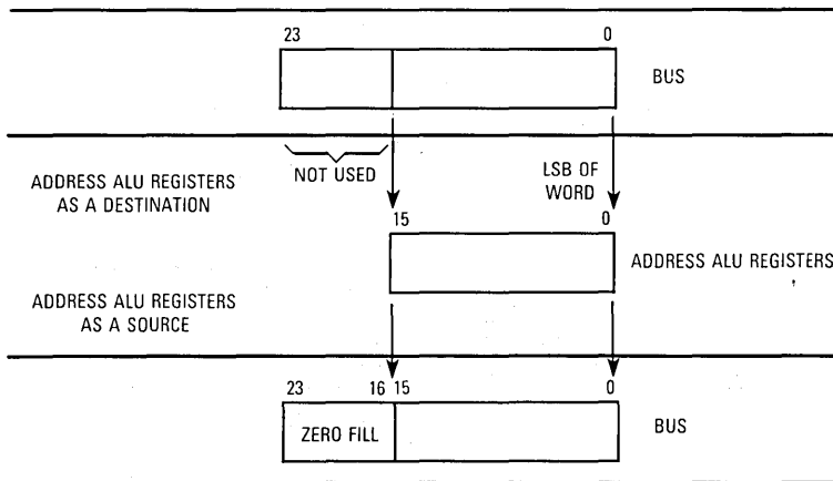
Figure 7-5. Reading and Writing the Address ALU Registers
