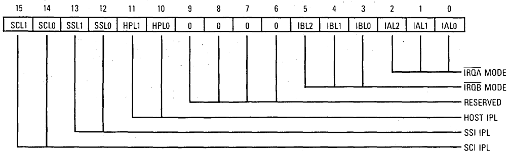
Figure 8-5. Interrupt Priority Register (Addr X:$FFFF)
