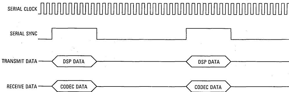
Figure 11-71. Normal Mode Example
