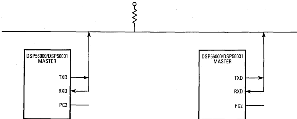
Figure 11-39. Multimaster System Example
