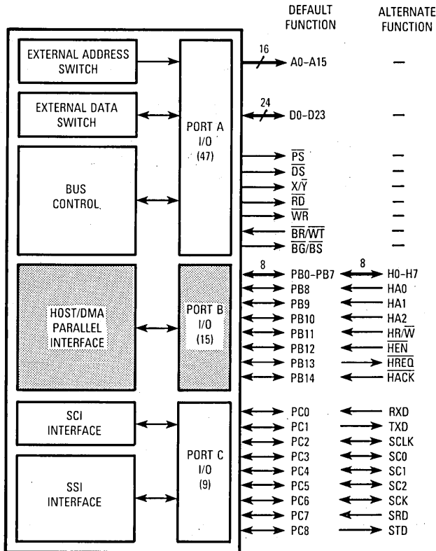
Figure 10-1. Port B Interface
