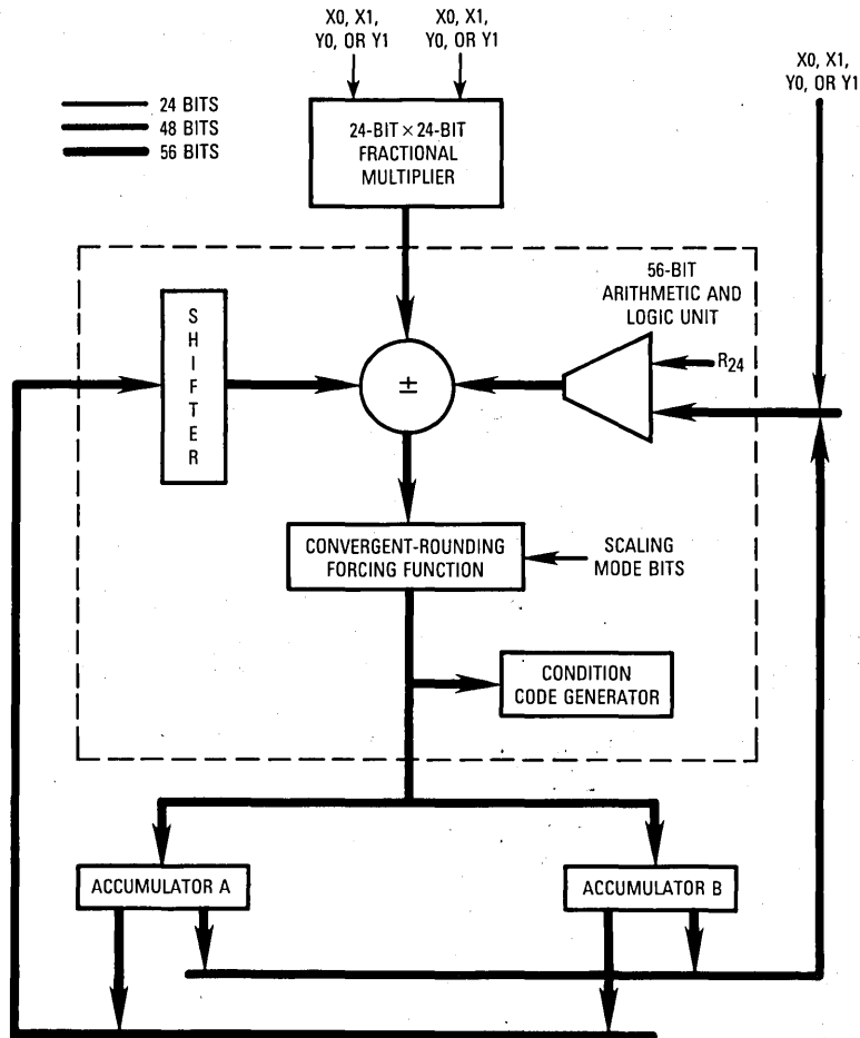
Figure 4-3. MAC Unit
