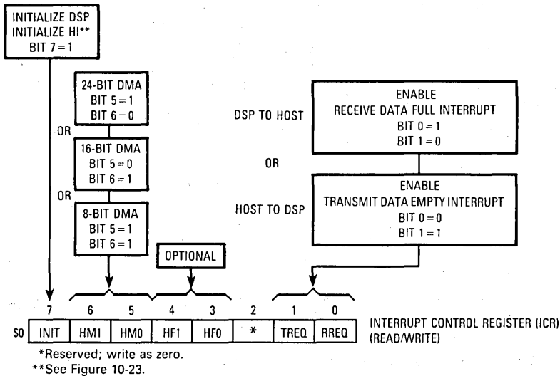
Figure 10-21(d). HI Initialization — Host Side, DMA Mode
