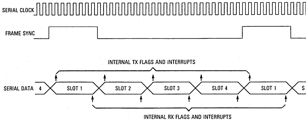
Figure 11-76. Network Mode Initialization
