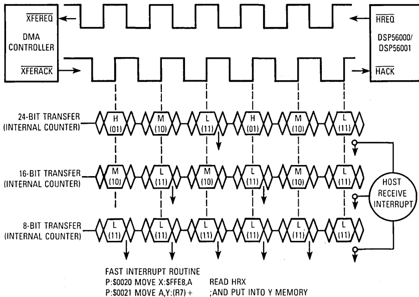
Figure 10-37. DMA Transfer and Host Interrupts
