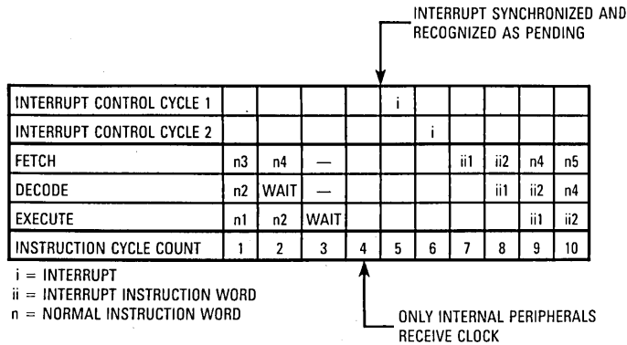
Figure 8-15. Wait Instruction Timing
