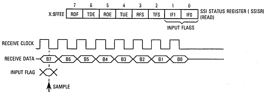
Figure 11-89. Input Flags
