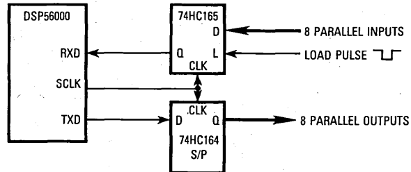
Figure 11-18. Synchronous Master
