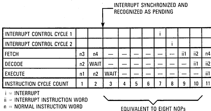
Figure 8-16 Simultaneous Wait Instruction and Interrupt
