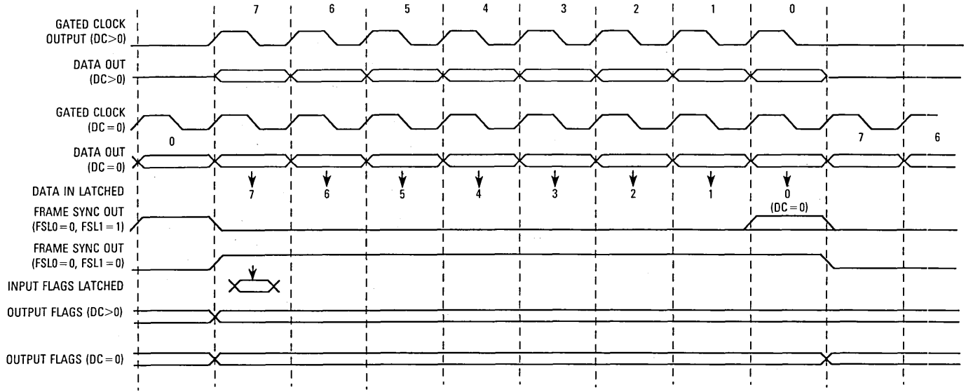
Figure 11-59. Internally Generated Gated Clock Timing (8-Bit Example)
