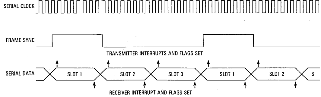
Figure 11-54. CRB MOD Bit Operation
