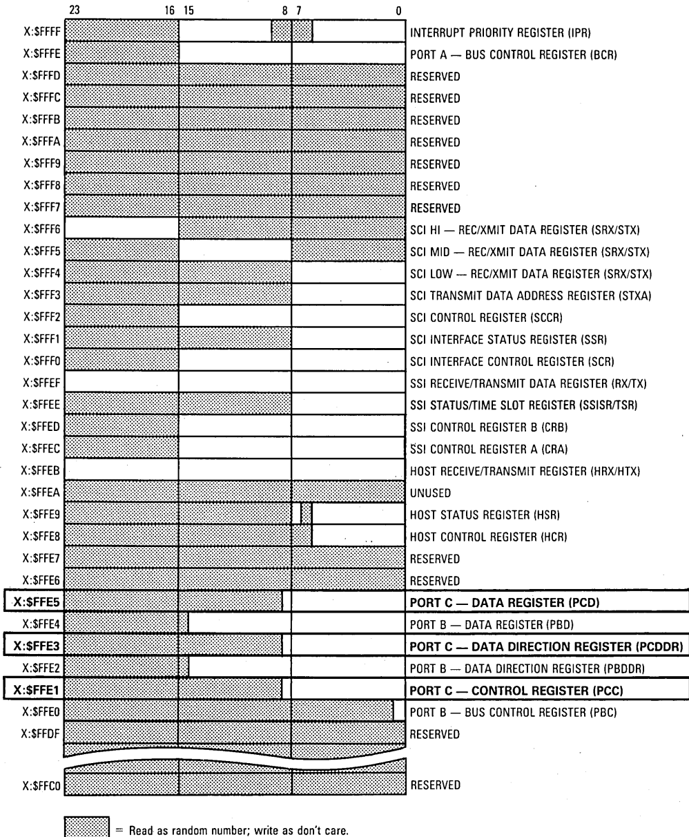
Figure 11-5. On-Chip Peripheral Memory Map
