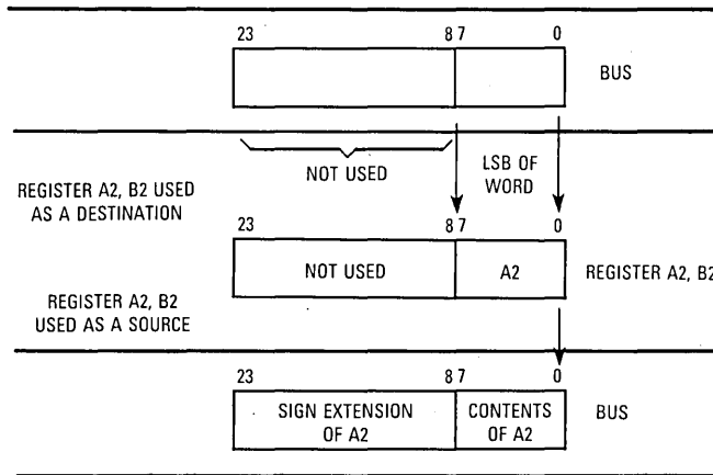
Figure 7-4. Reading and Writing the ALU Extension Registers
