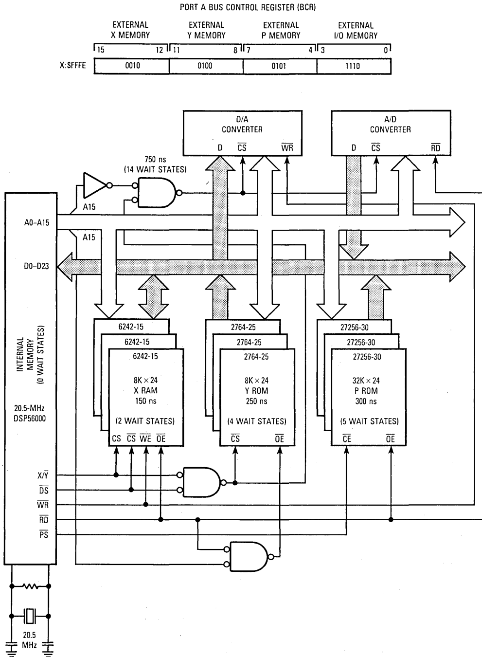
Figure 9-9. Mixed-Speed Expanded System
