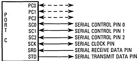
Figure 11-51. SSI Initialization Procedure
