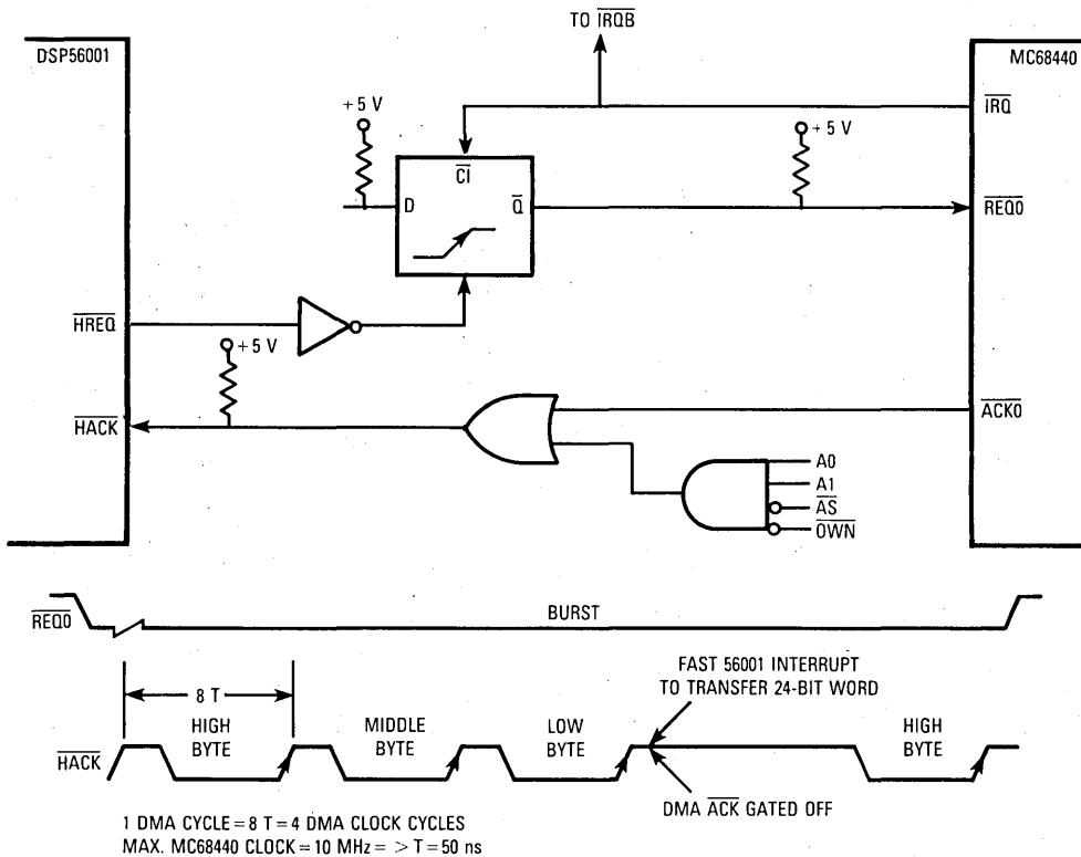
Figure 10-18. DMA Transfer Logic and Timing
