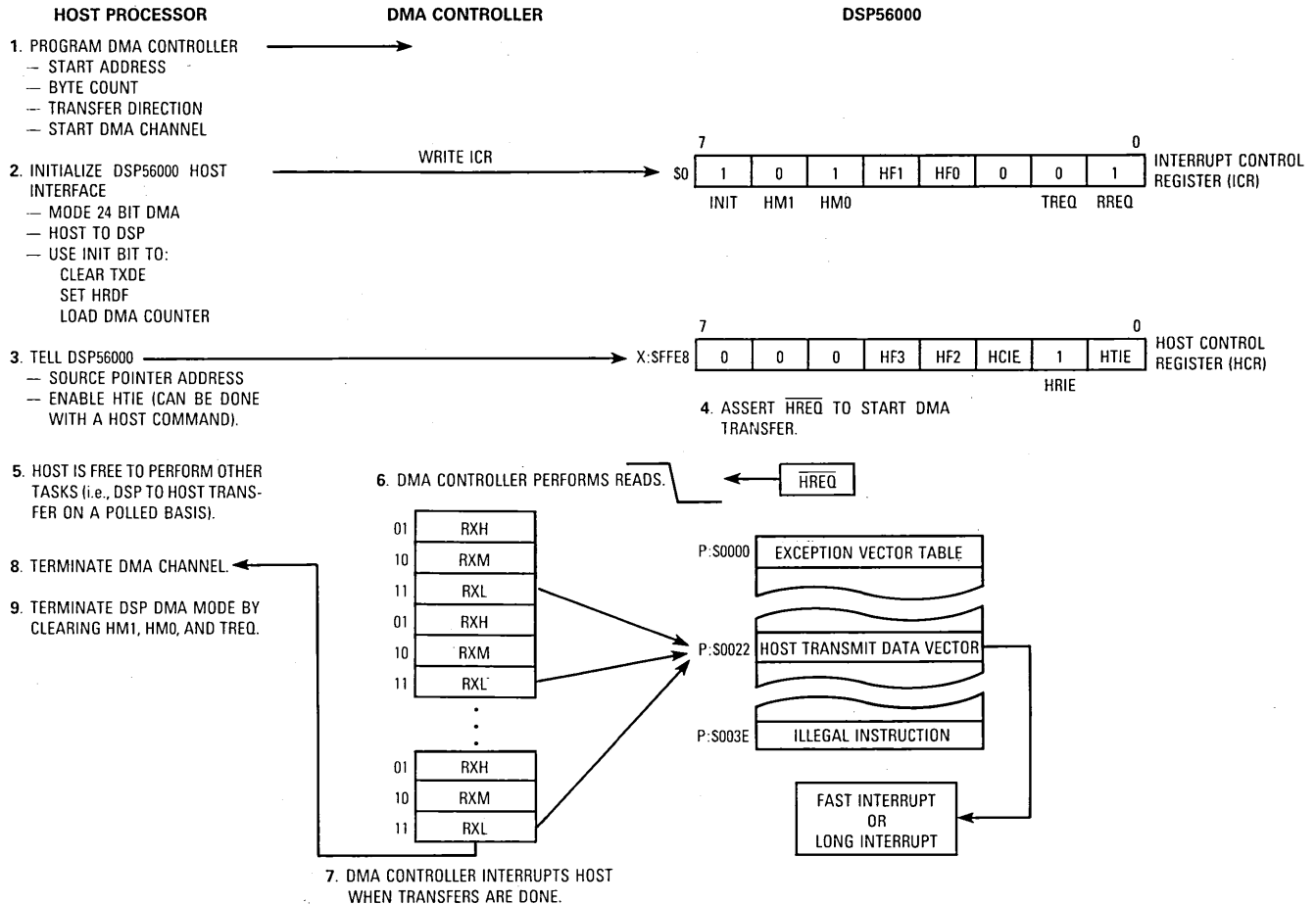
Figure 10-40. DSP-to-Host DMA Procedure
