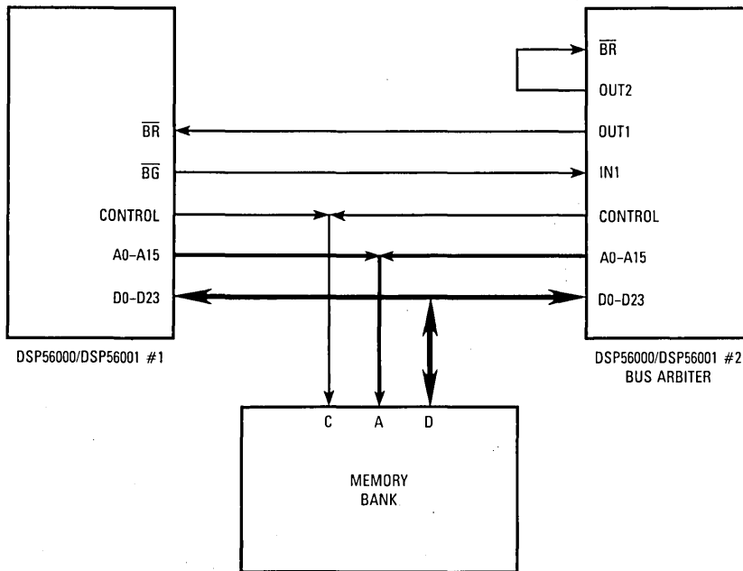
Figure 9-14. Bus Arbitration Using Only \overline{BR}/\overline{BG} with Internal Control
