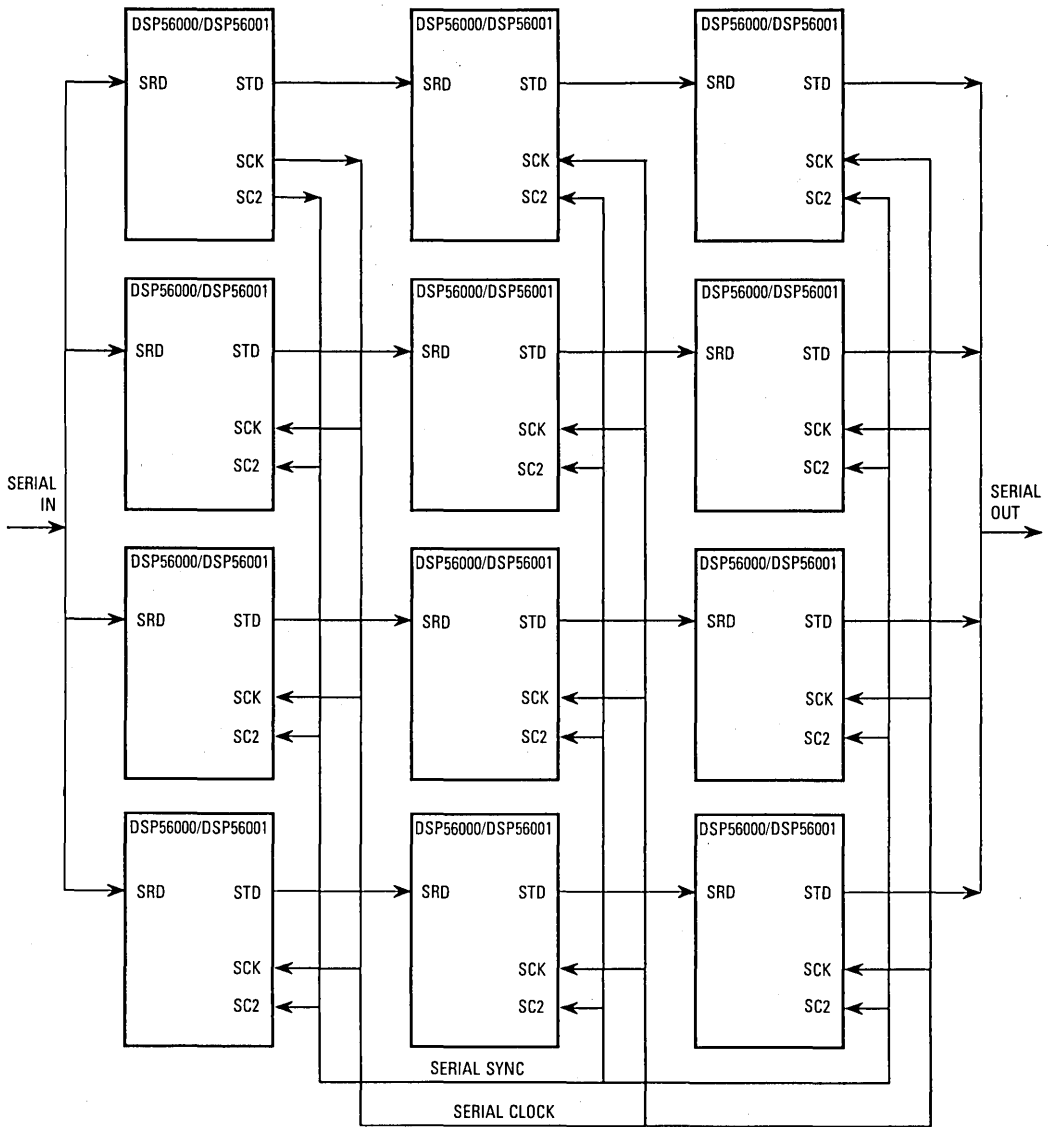
Figure 11-93. SSI TDM Serial/Parallel Processing Array
