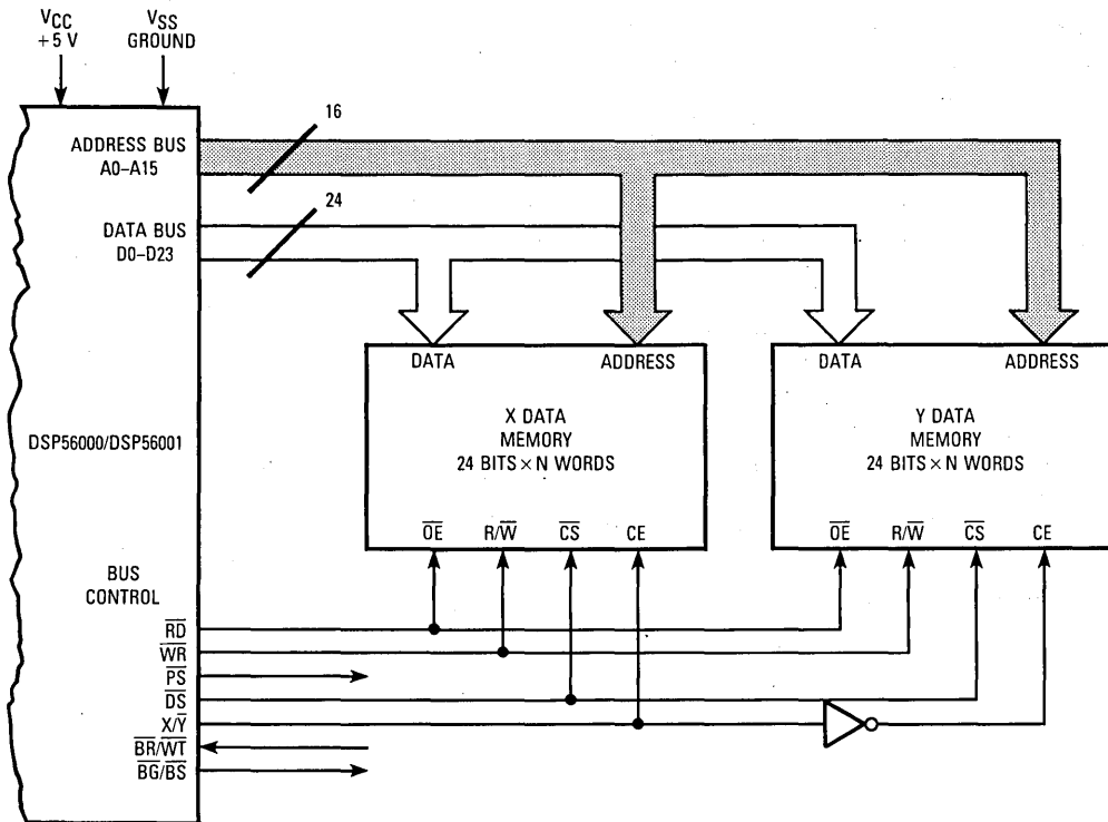
Figure 9-3. External X and Y Data Space
