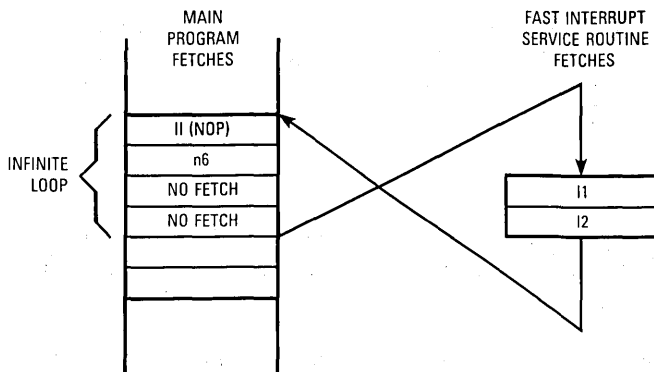
(a) Instruction Fetches from Memory
