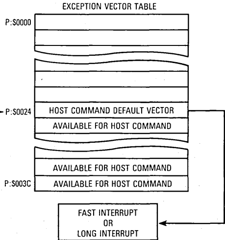
Figure 10-28. Host Command
