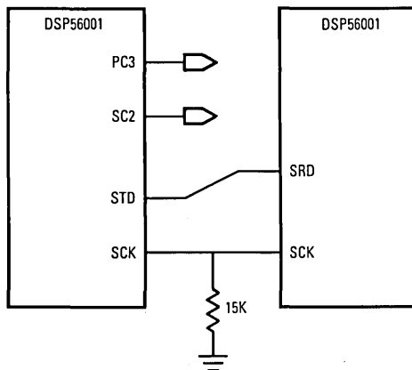
Figure 11-83. On-Demand Mode Example — Hardware Configuration
