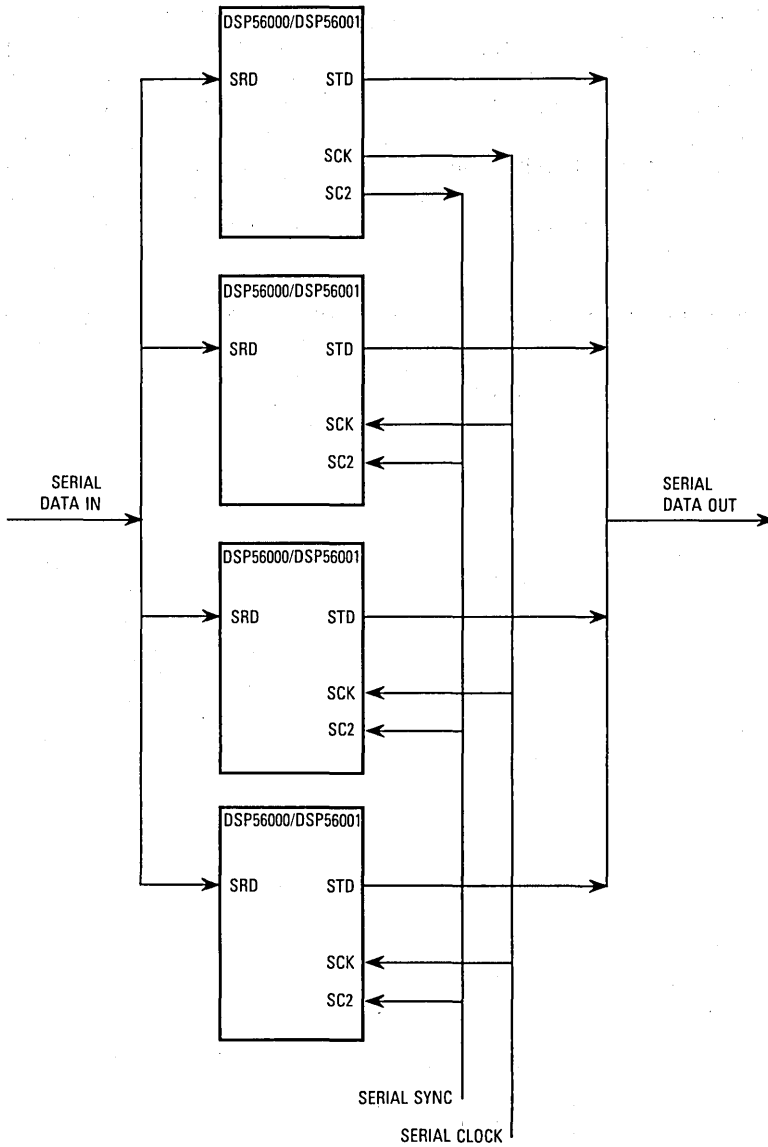
Figure 11-91. SSI TDM Parallel DSP Network
