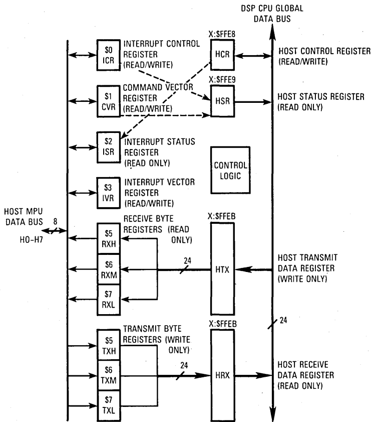
Figure 10-9. HI Block Diagram
