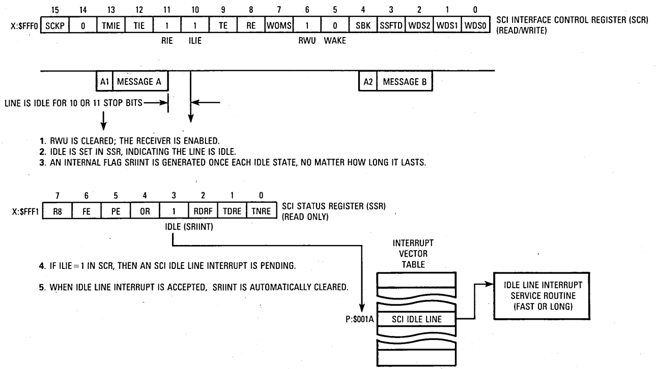
Figure 11-33. Idle Line Wakeup
