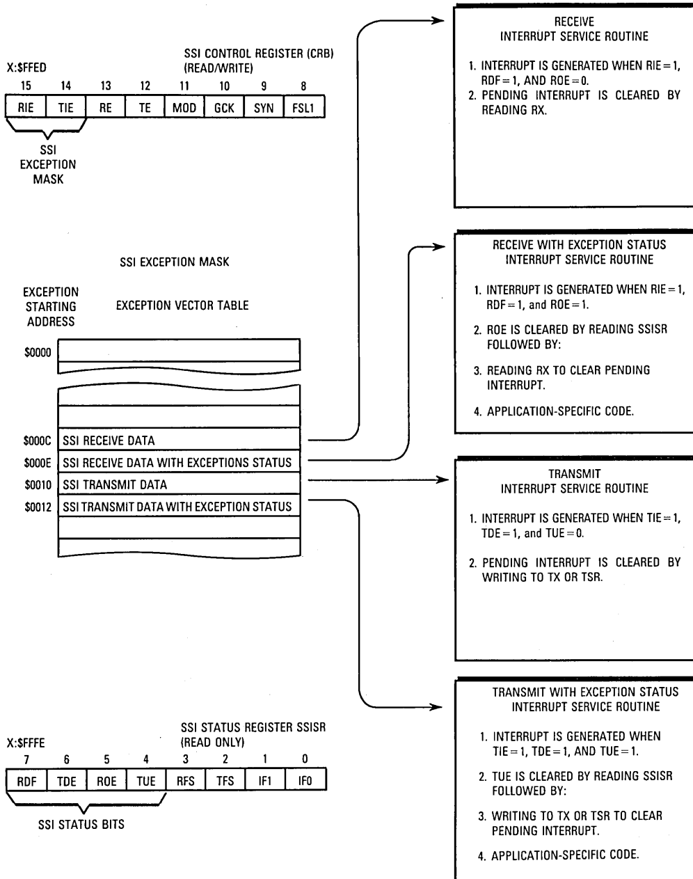
Figure 11-53. SSI Exceptions
