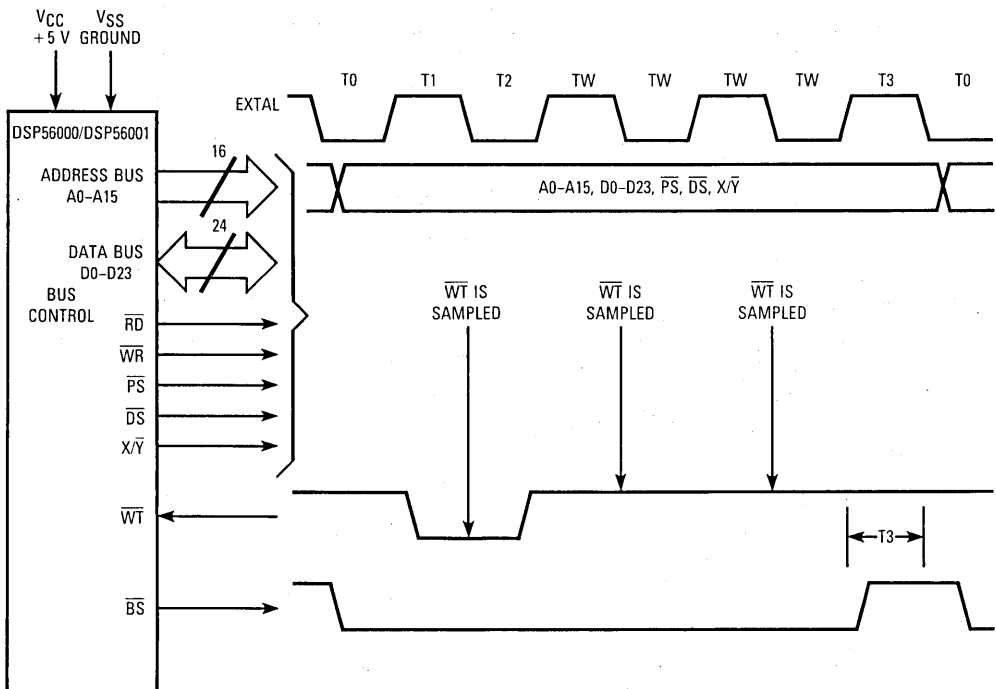
Figure 9-12. Bus Strobe/Wait Sequence
