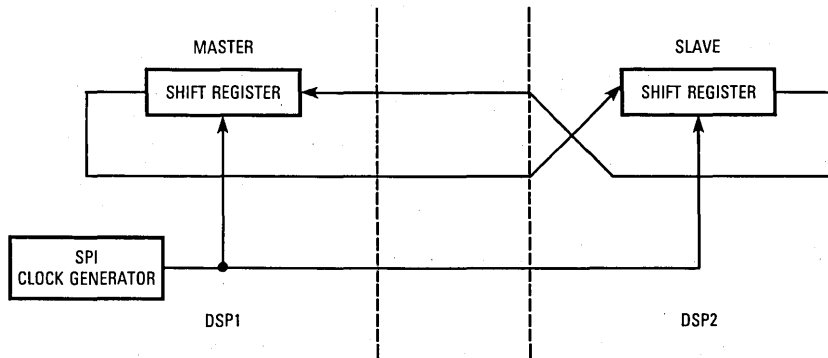
Figure 11-82. SPI Configuration
