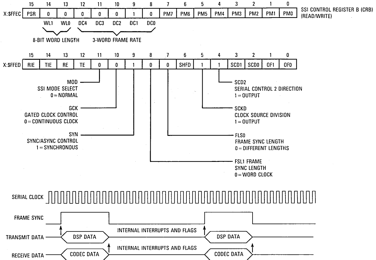
Figure 11-68. Normal Mode Initialization for FSL1=0 and FSL0=0
