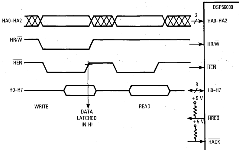
Figure 10-15. Host Processor Transfer Timing
