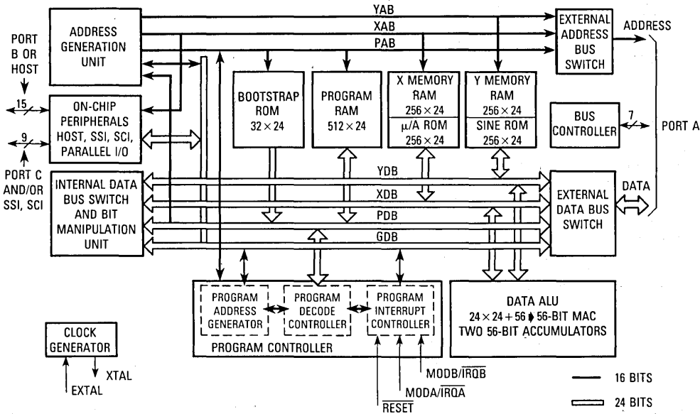
Figure 2-2. DSP56001 Block Diagram
