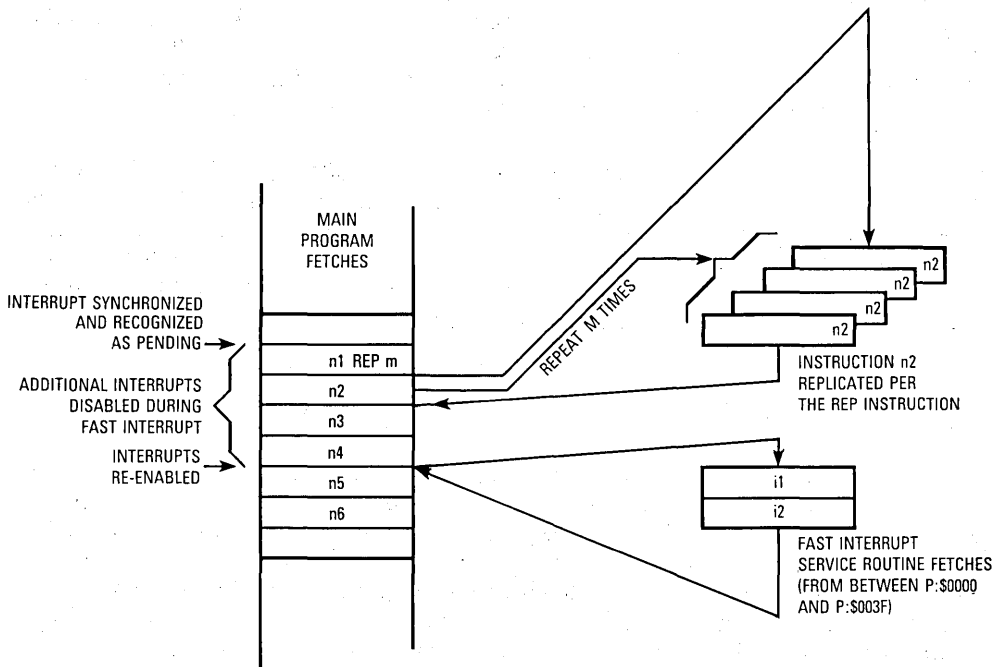
(a) Instruction Fetches from Memory
