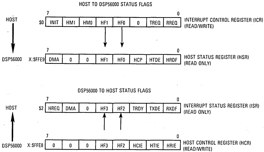
Figure 10-11. Host Flag Operation
