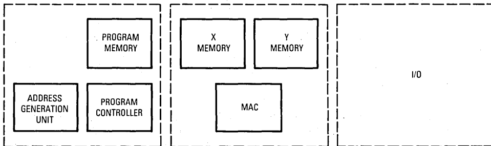
Figure 1-4. DSP Block Diagram
