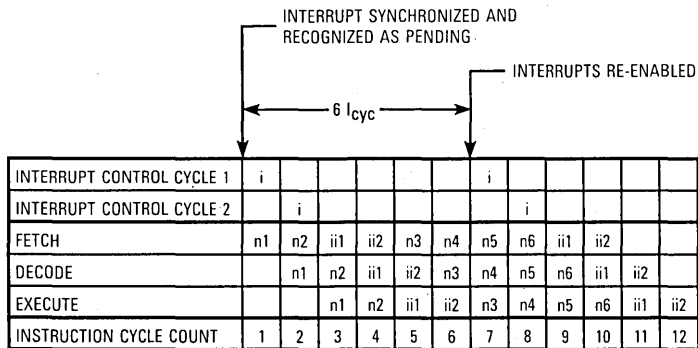
(b) Program Controller Pipeline
