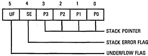
Figure 6-8. SP Register Format
