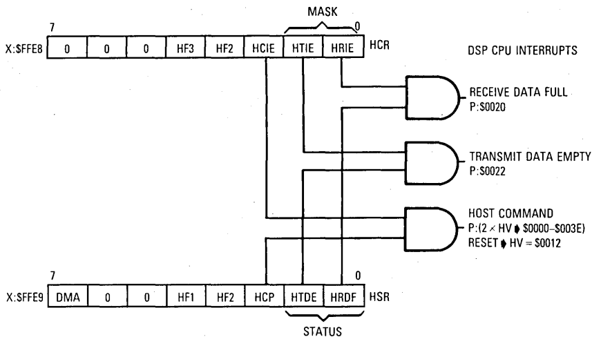
Figure 10-12. HSR-HCR Operation
