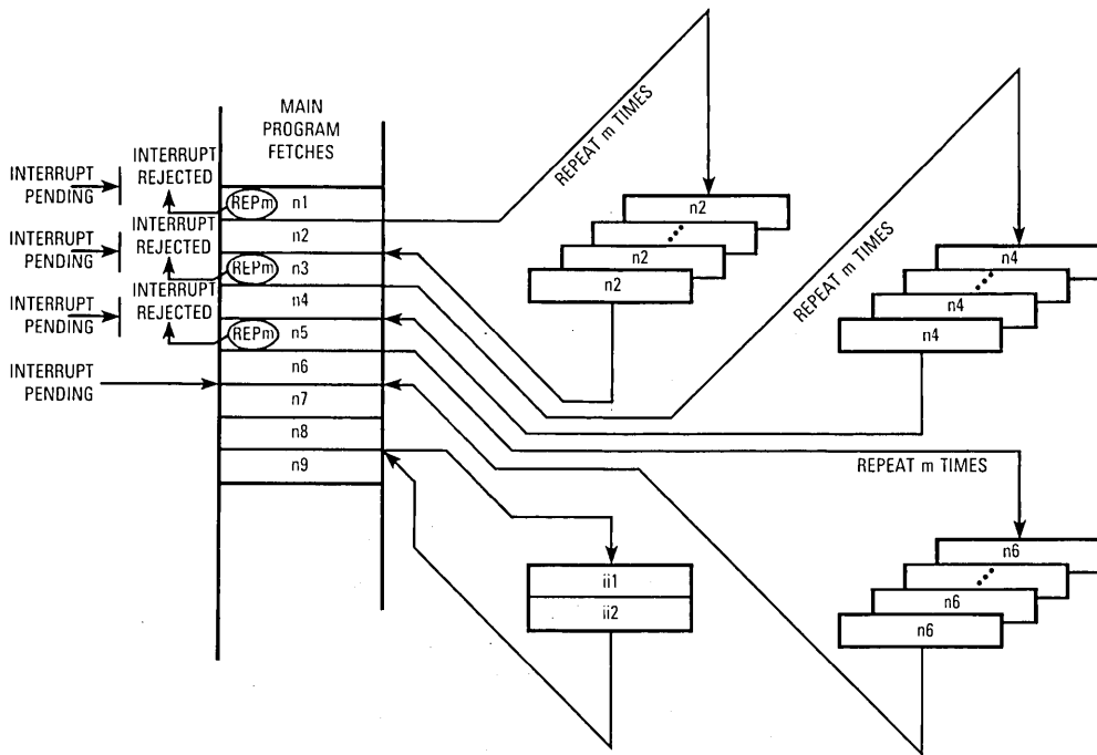
(a) Instruction Fetches from Memory
