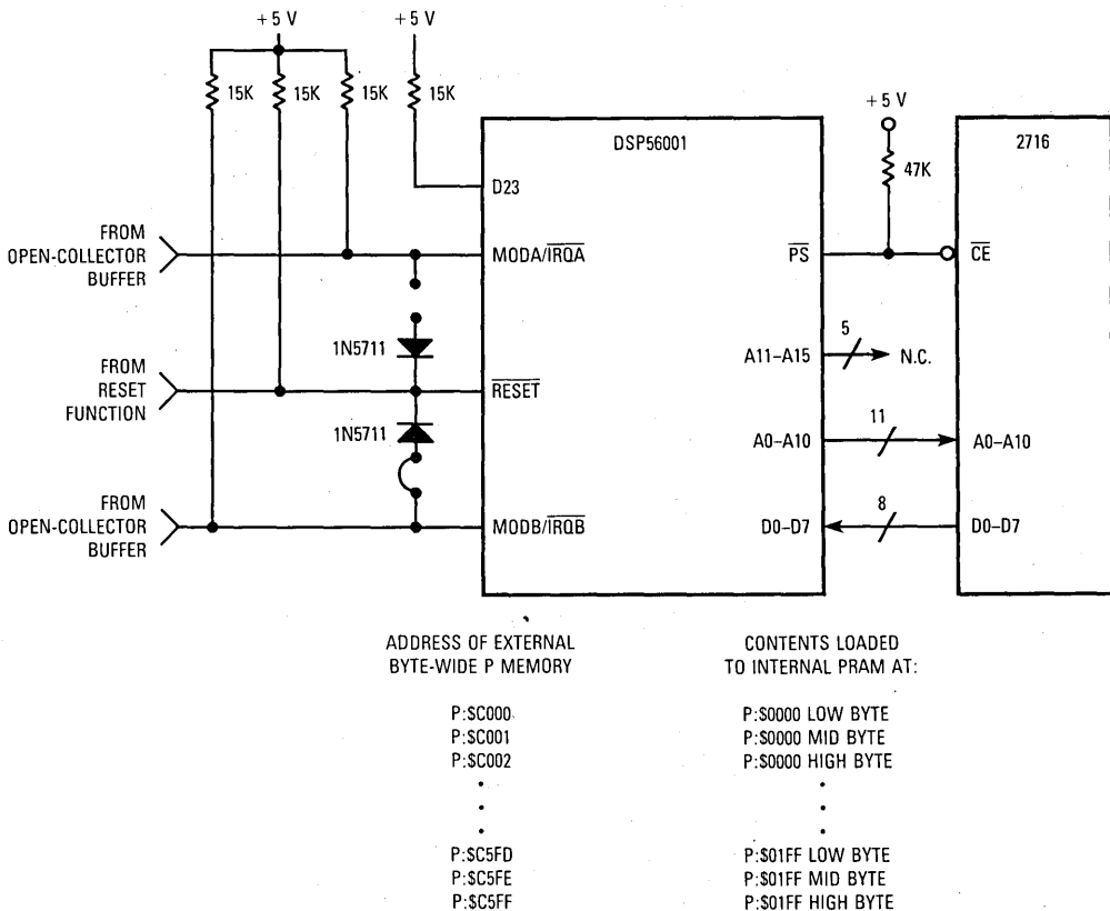
Figure 9-5. Port A Bootstrap Circuit
