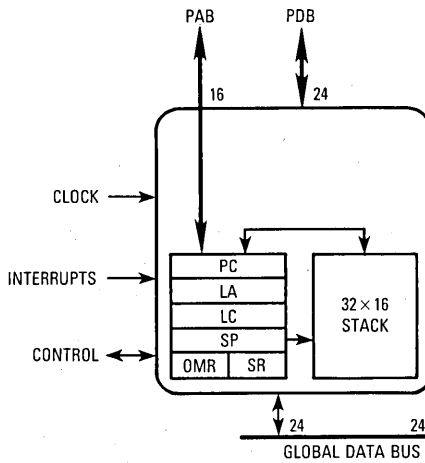
Figure 6-2. DSP56000/DSP56001 Program Controller
