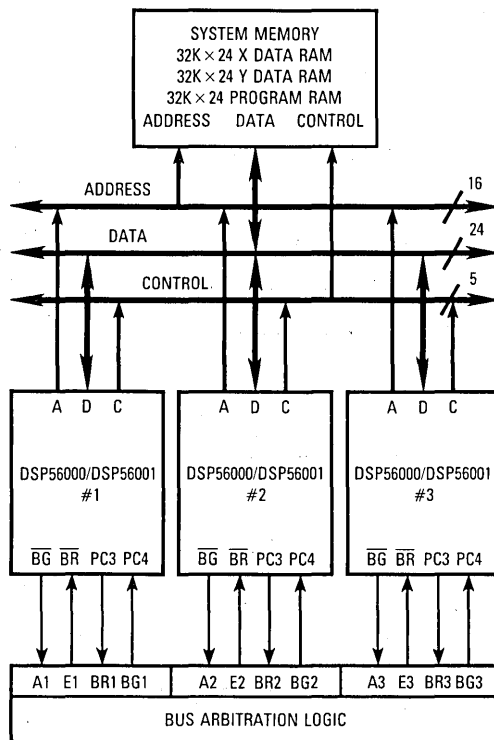
Figure 9-16. Bus Arbitration Using Only \overline{BR}/\overline{BG} with External Control
