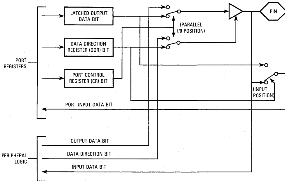
Figure 11-4. Port B I/O Pin Control Logic
