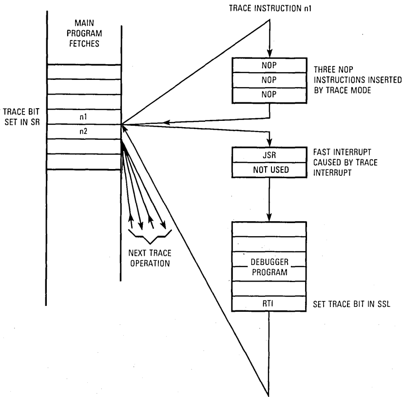
(a) Instruction Fetches from Memory
