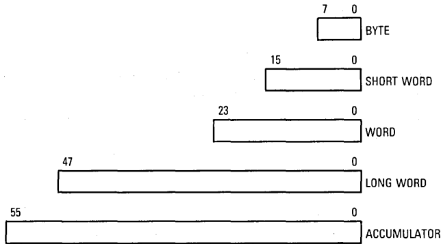
Figure 7-3. Operand Sizes
