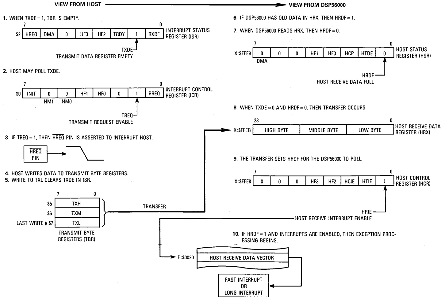
Figure 10-24. Data Transfer from Host to DSP
