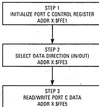
Figure 11-7. Port C Configuration Flowchart
