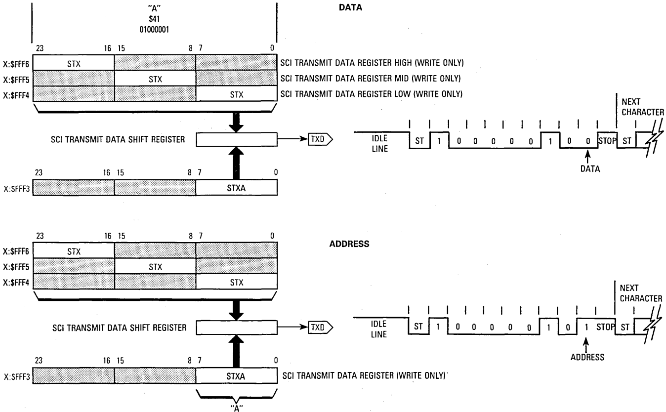
Figure 11-31. Transmitting Data and Address Characters
