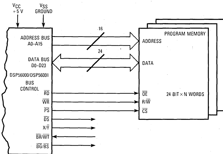
Figure 9-2. External Program Space
