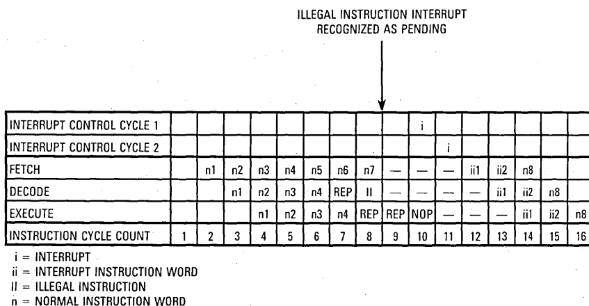
Figure 8-3. Repeated Illegal Instruction
