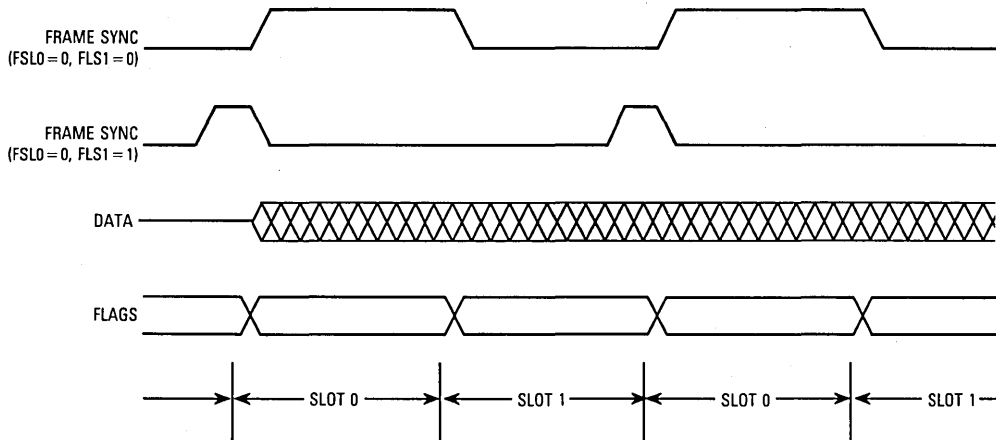
Figure 11-56. Network Mode (8 Bit, 2 Words in Frame)
