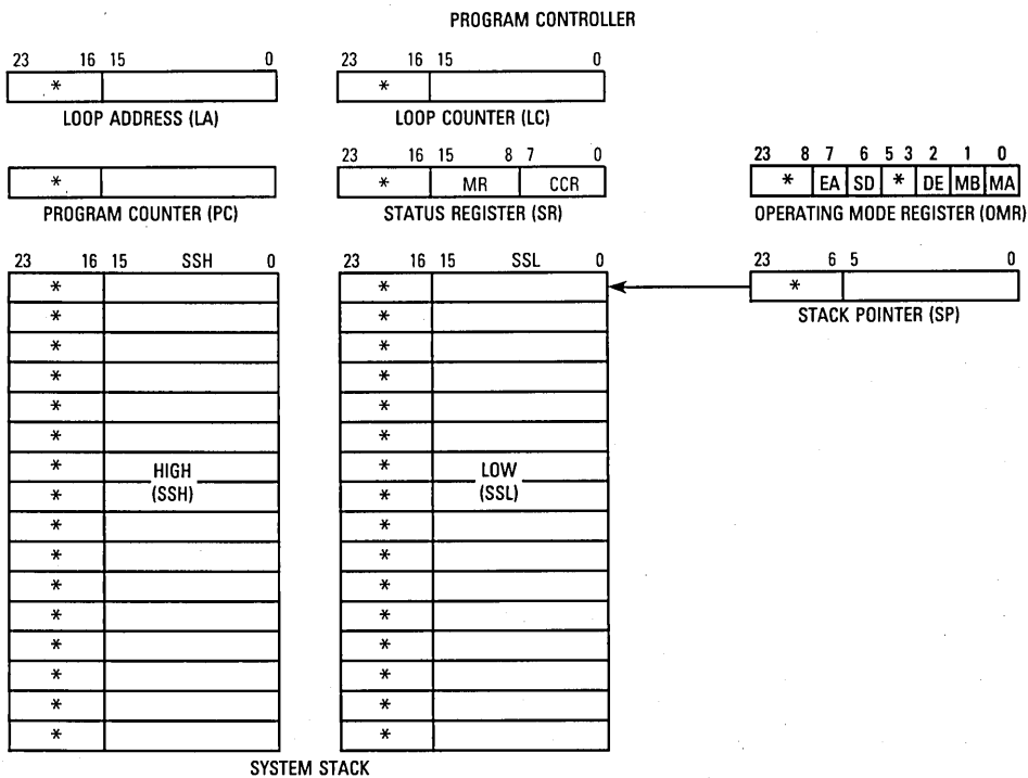
Figure 6-5. Program Controller Programming Model
