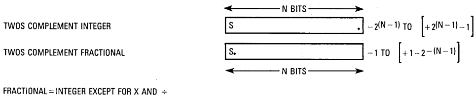
Figure 4-7. Integer/Fractional Number Comparison
