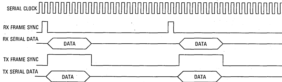
Figure 11-67. CRB FSL0 and FSL1 Bit Operation
