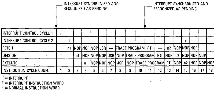
(b) Program Controller Pipeline
