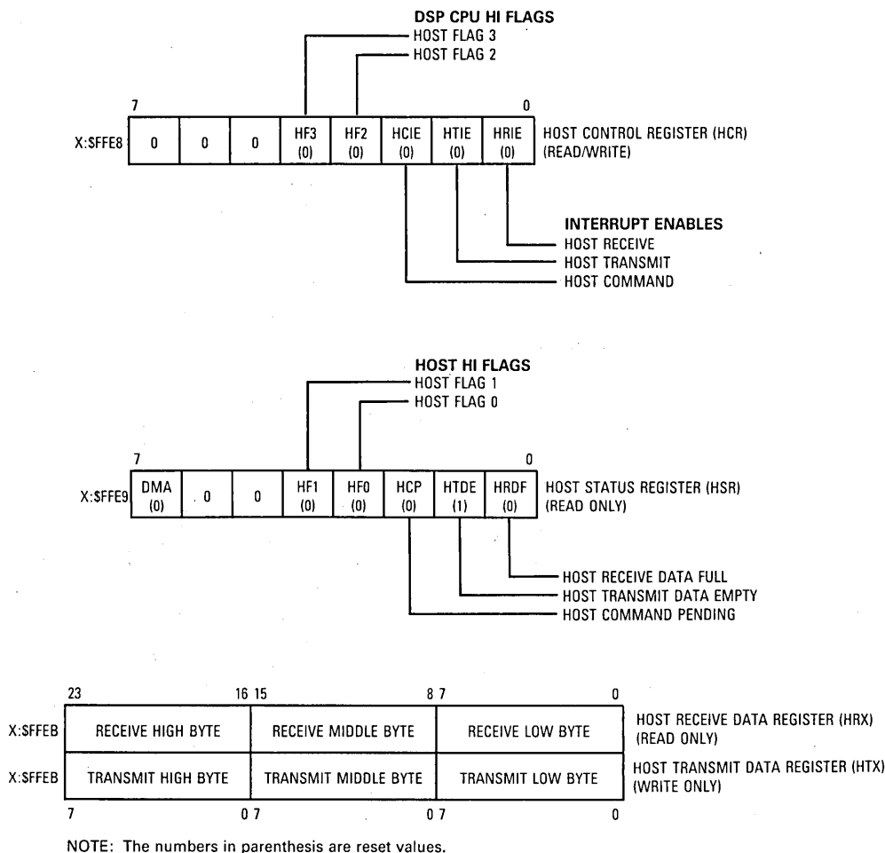
Figure 10-10. Host Interface Programming Model — DSP Viewpoint
