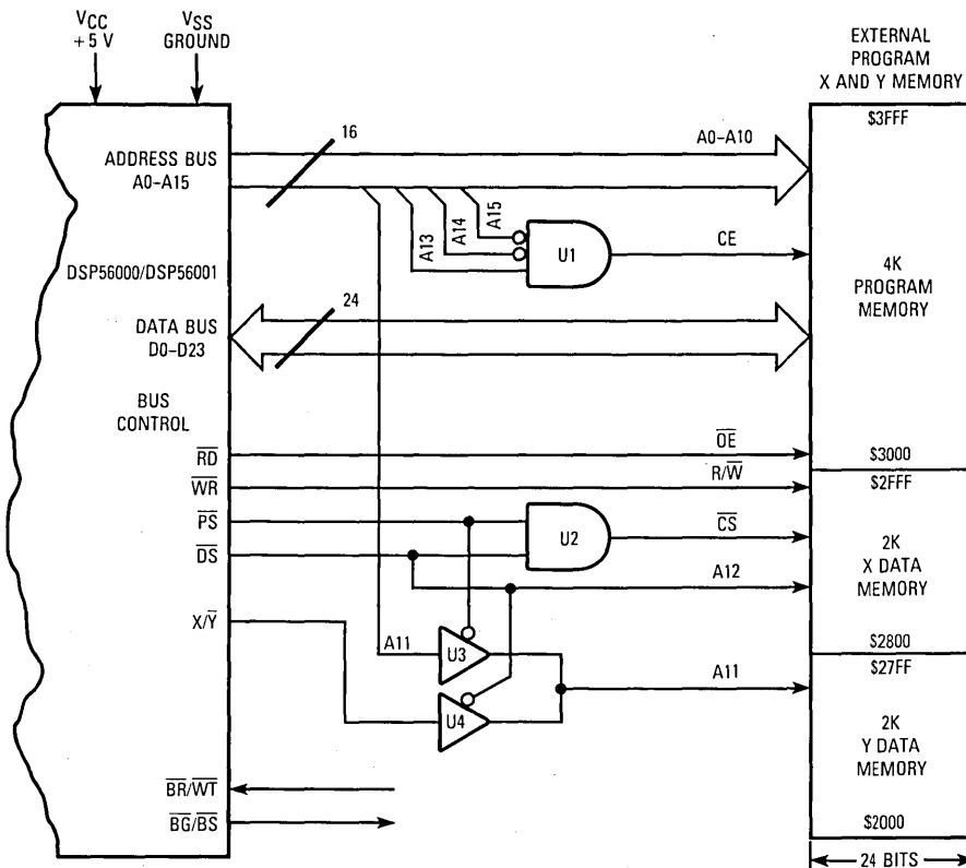
Figure 9-4. Memory Segmentation
