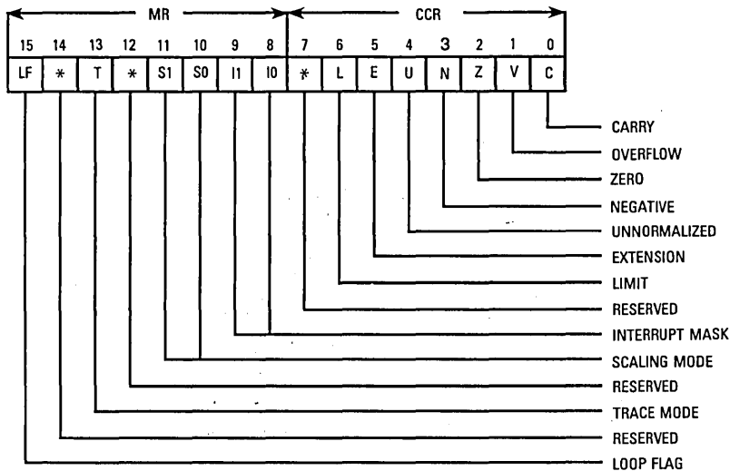
Figure 6-6. Status Register Format
