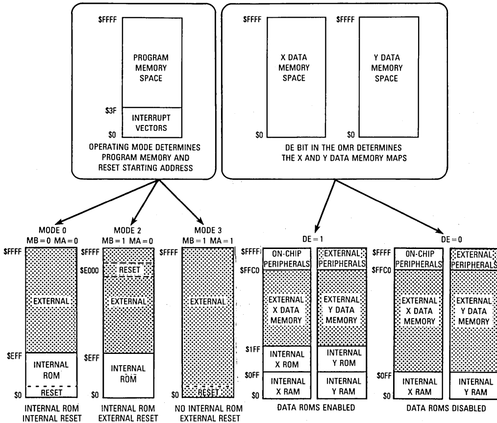
Figure 3-1. DSP56000 Memory Map
