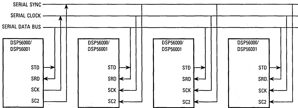
Figure 11-95. SSI TDM Bus DSP Network
