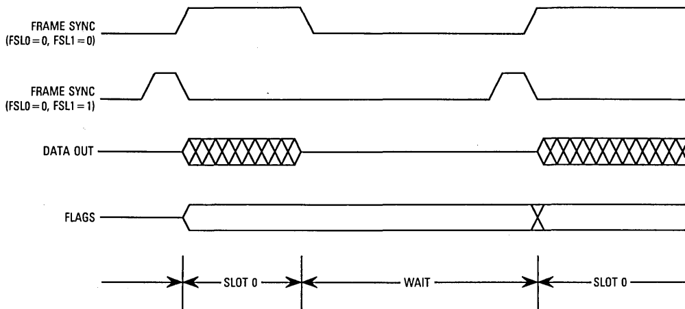
Figure 11-55. Normal Mode, External Frame Sync (8 Bit, 1 Word in Frame)
