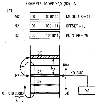
Figure 5-13. Modulo Modifier Example
