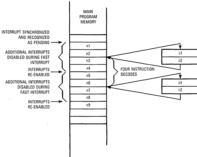
(a) Instruction Fetches from Memory
