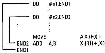
Figure 7-14. Nested DO Loops
