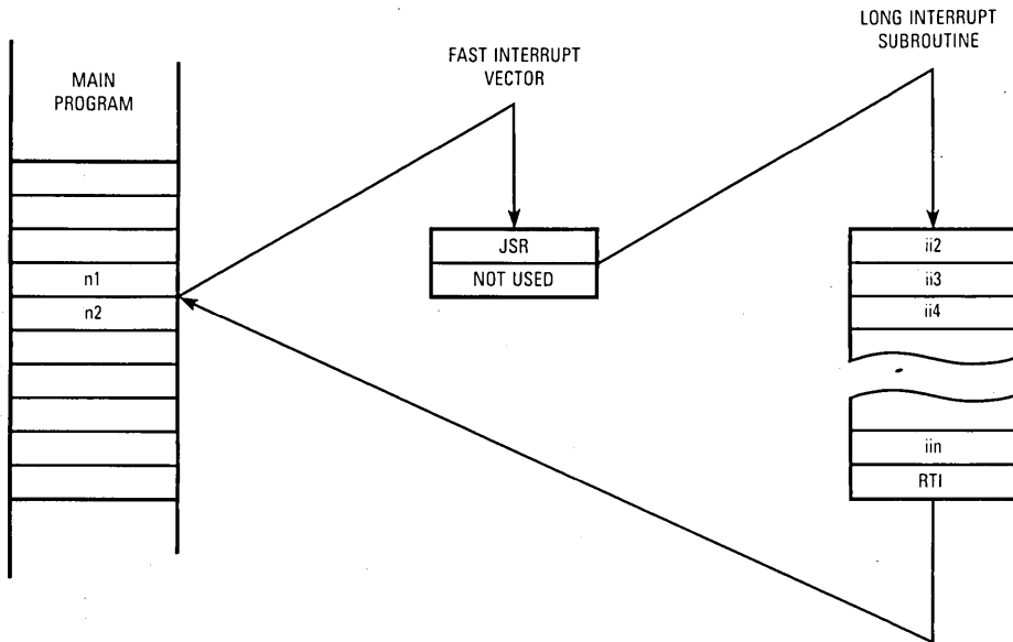
(a) Instruction Fetches from Memory
