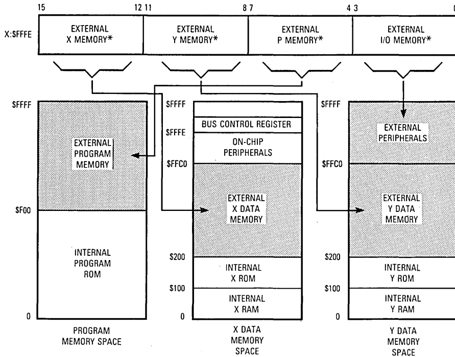
Figure 9-10. Bus Control Register
