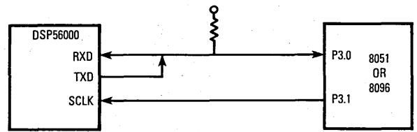
Figure 11-19. Synchronous Slave
