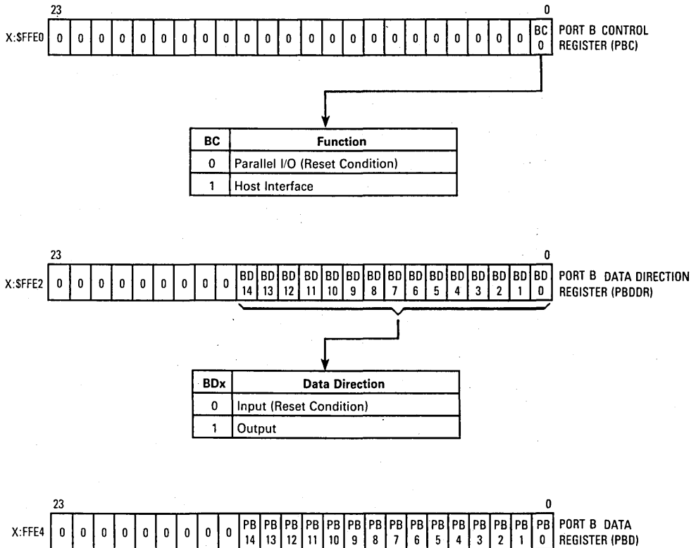
Figure 10-2. Parallel Port B Registers
