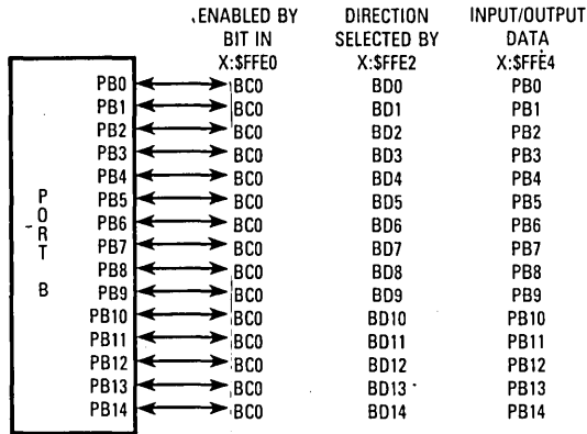
Figure 10-3. Parallel Port B Pinout
