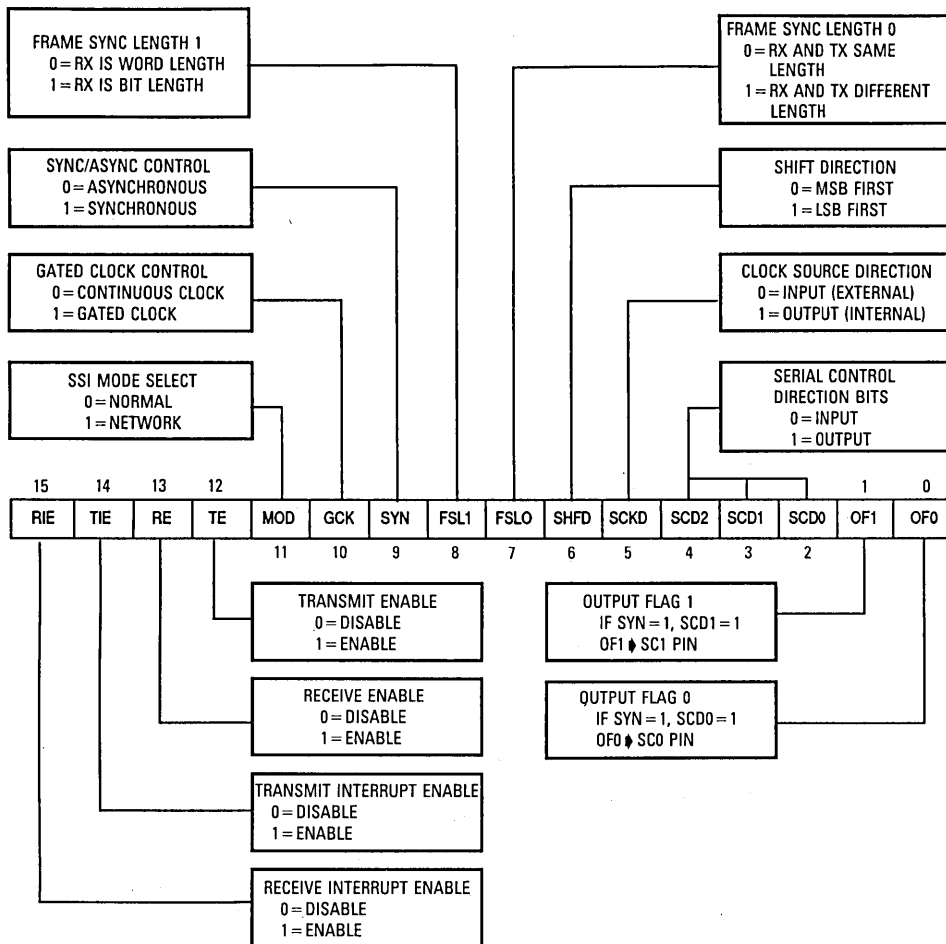
Figure 11-50. SSI CRB Initialization Procedure
