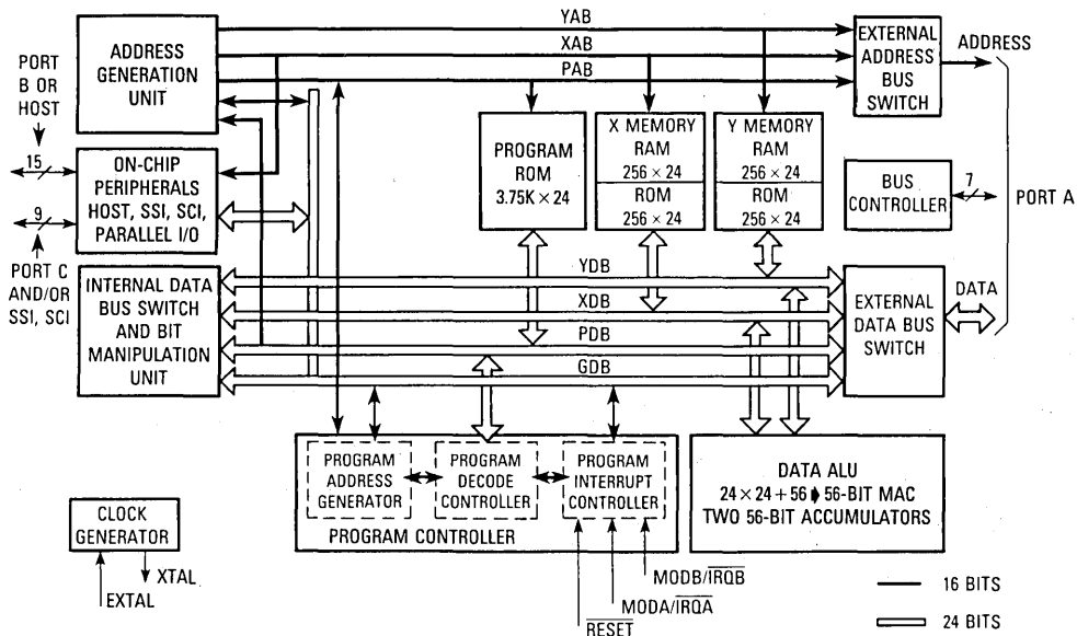
Figure 2-1. DSP56000 Block Diagram
