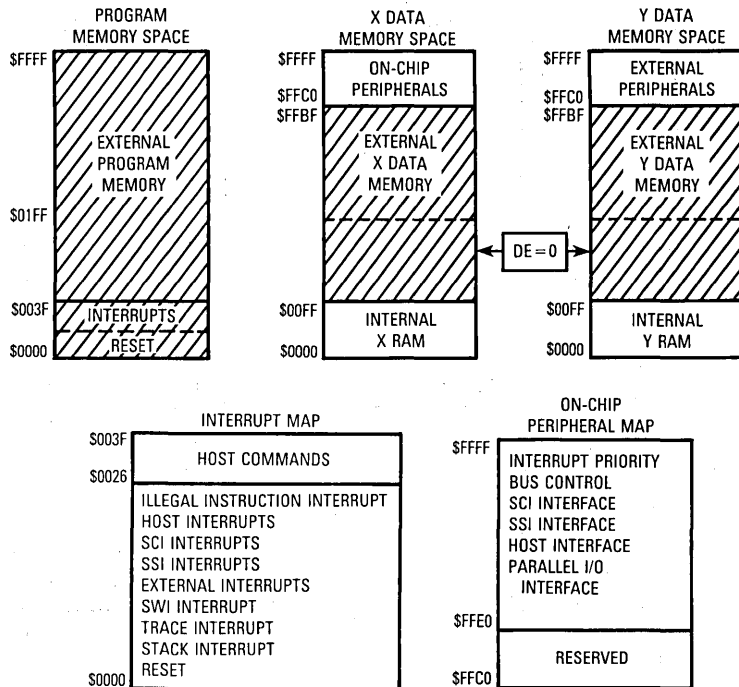
Figure 3-4. Memory Map for DSP56000 Mode 3: Development Mode
