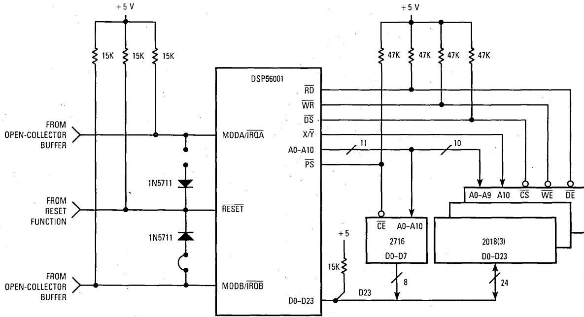
Figure 9-6. Port A Bootstrap ROM with X and Y RAM
