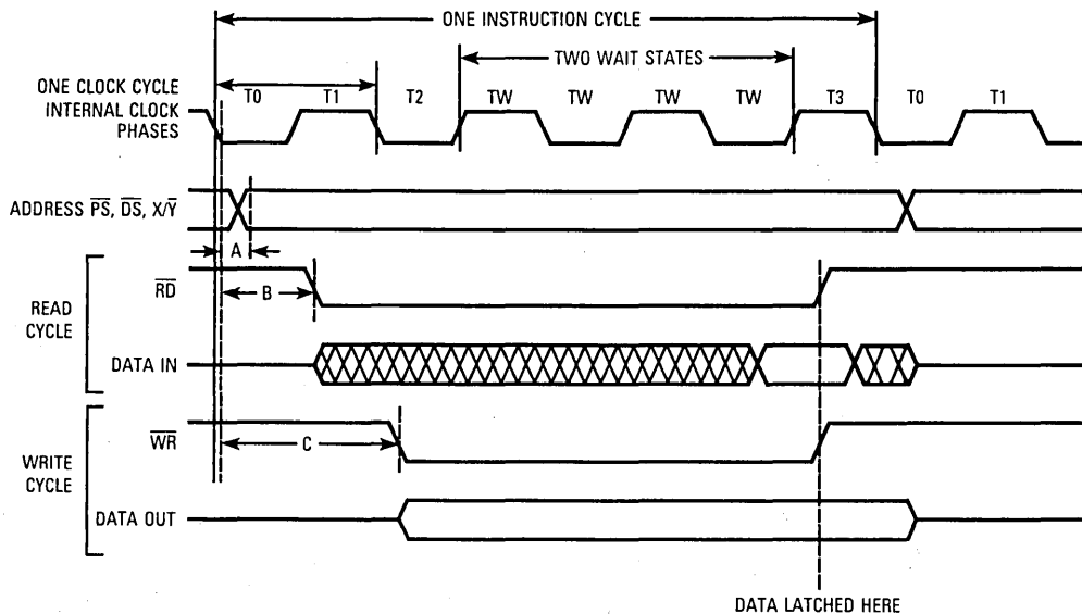
Figure 9-8. Port A Bus Operation with Two Wait States
