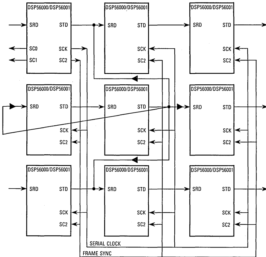
Figure 11-94. SSI Parallel Processing — Nearest Neighbor Array
