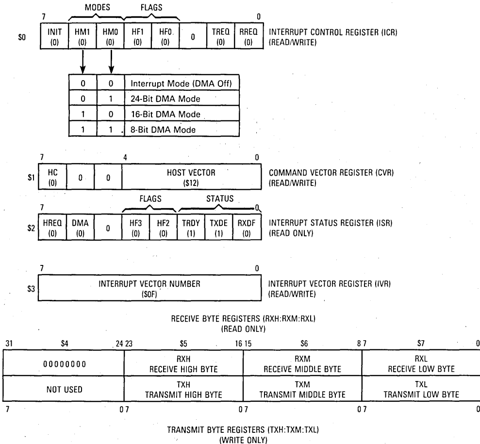
Figure 10-13. Host Processor Programming Model — Host Side
