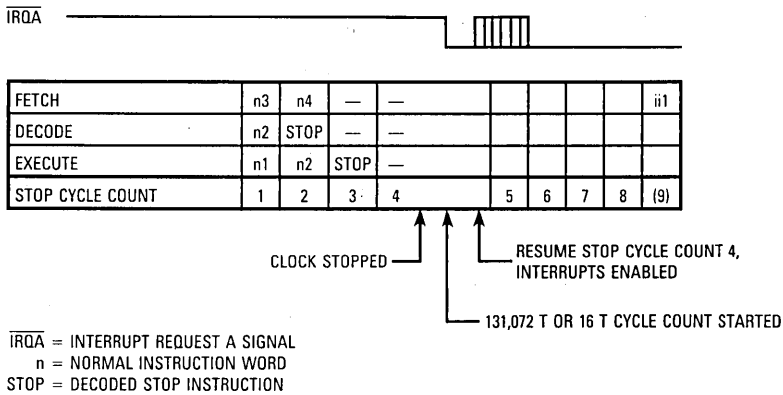
Figure 8-18. STOP Instruction Sequence Followed by \overline{\text{IRQA}}
