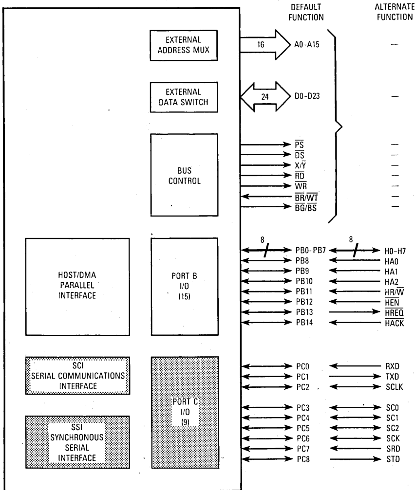
Figure 11-1. Port C Interface
