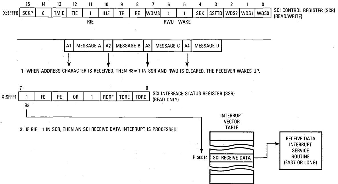
Figure 11-34. Address Mode Wakeup
