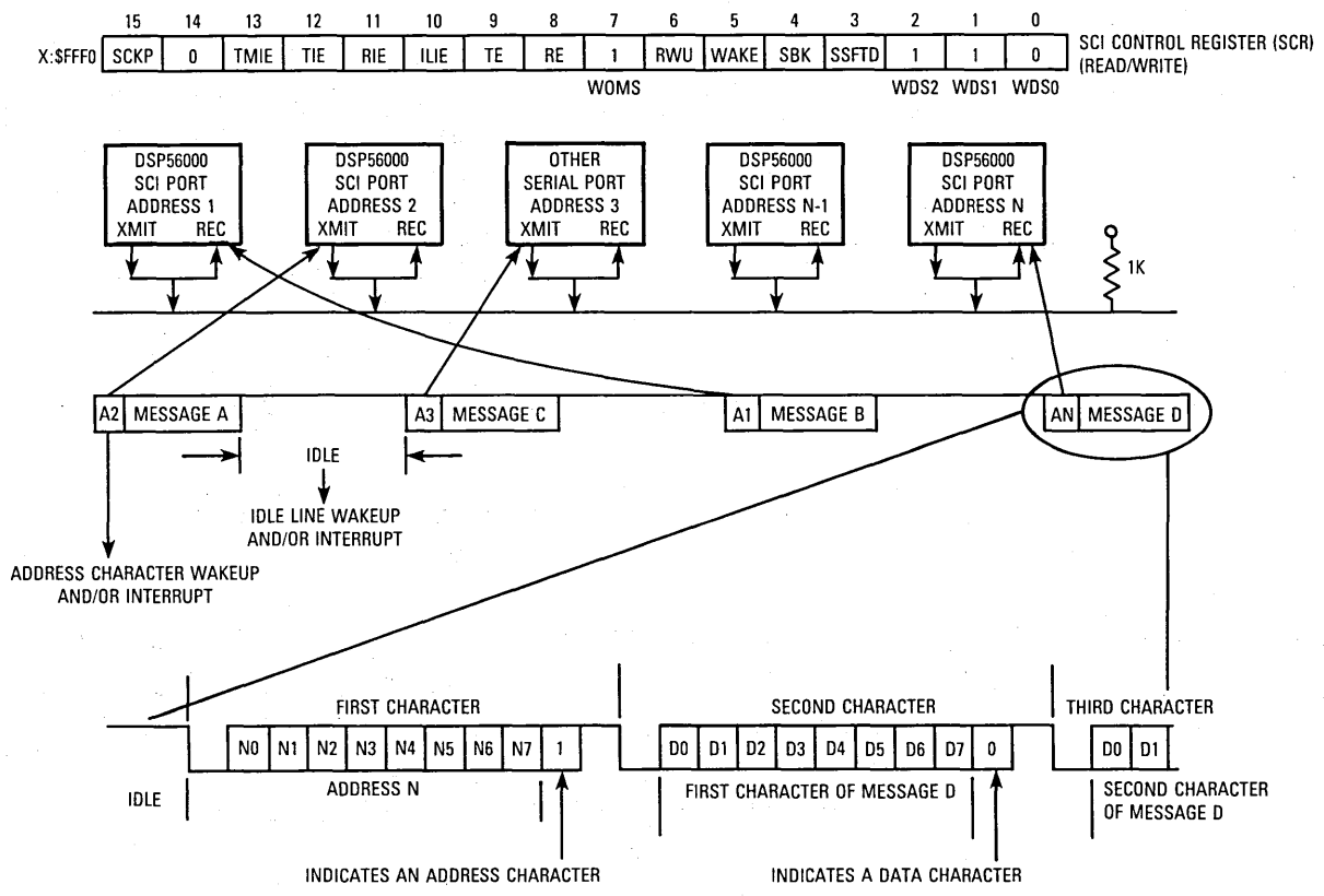
Figure 11-32. Wired-OR Mode
