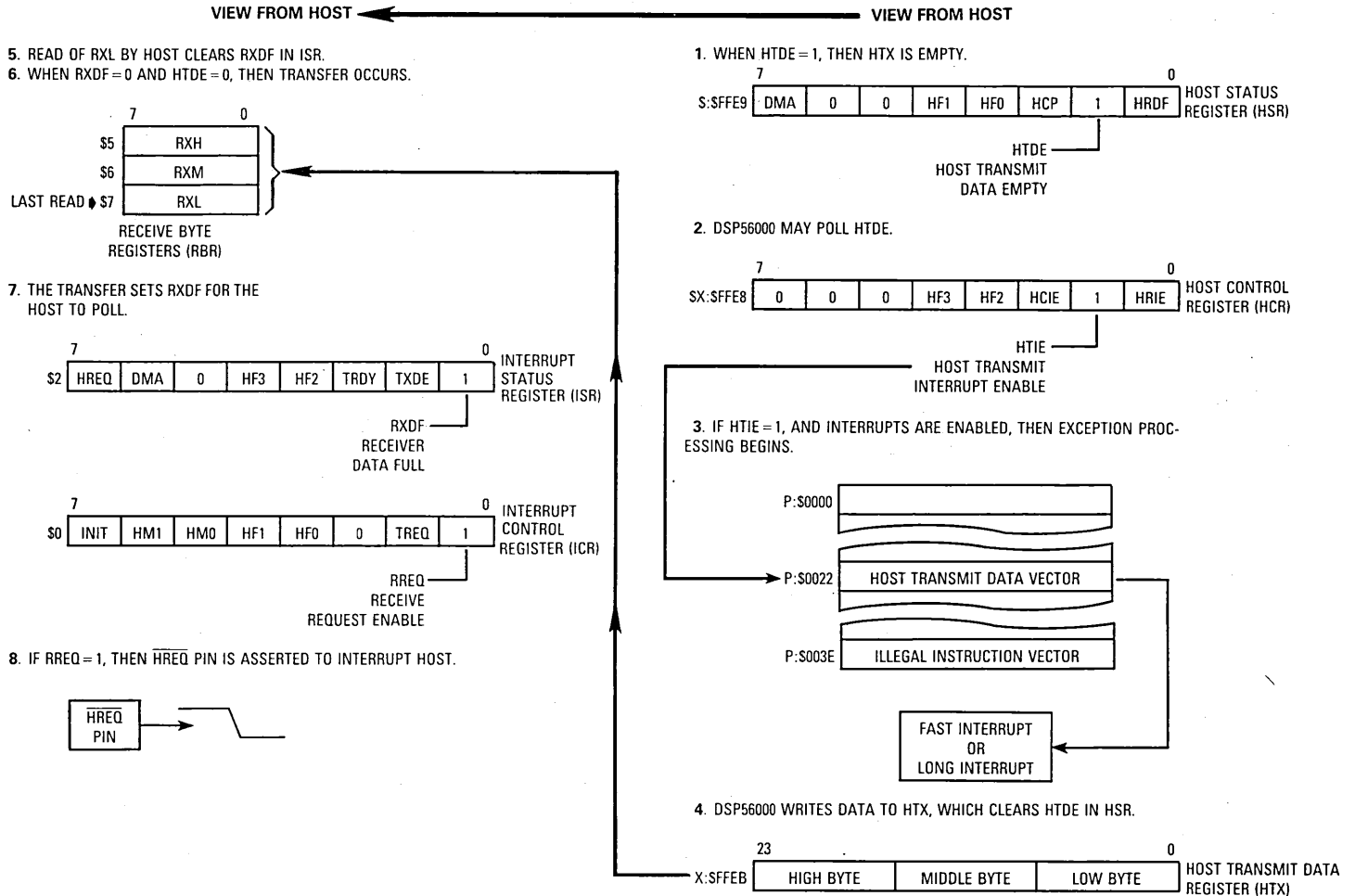
Figure 10-33. Data Transfer from DSP to Host
