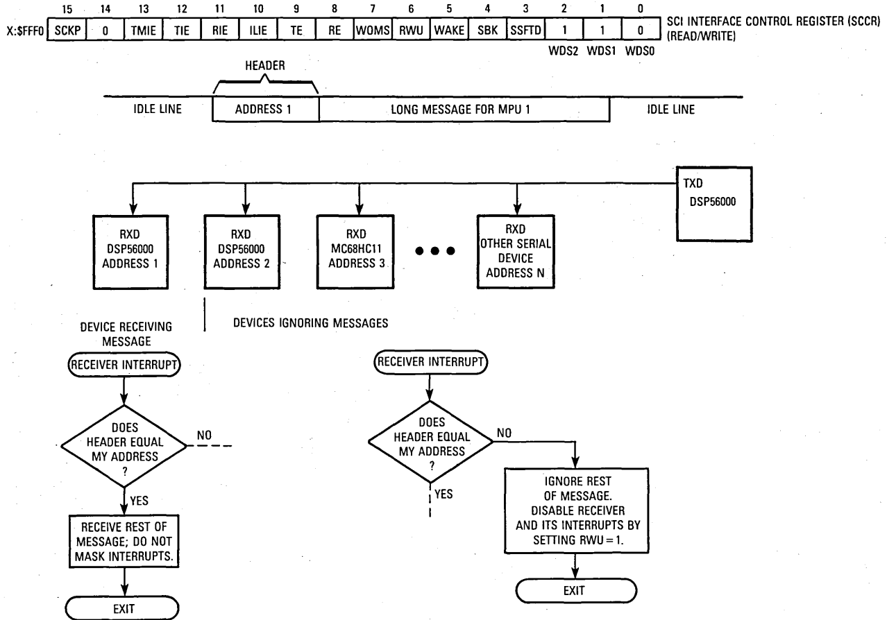
Figure 11-30. 11-Bit Multidrop Mode
