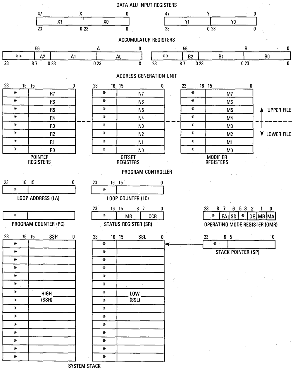
Figure 6-10. DSP56000/DSP56001 Central Processor Programming Model
