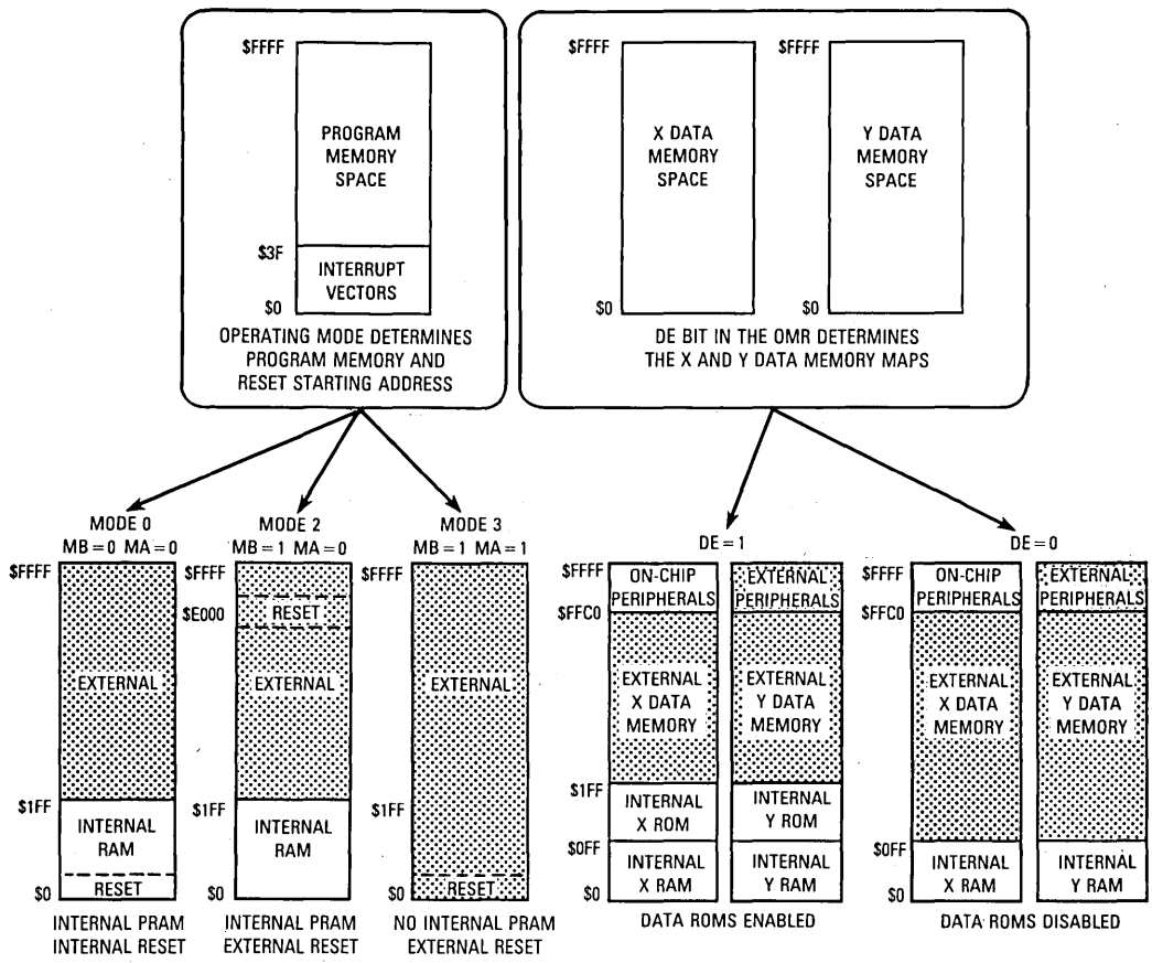
Figure 3-5. DSP56001 Memory Map
