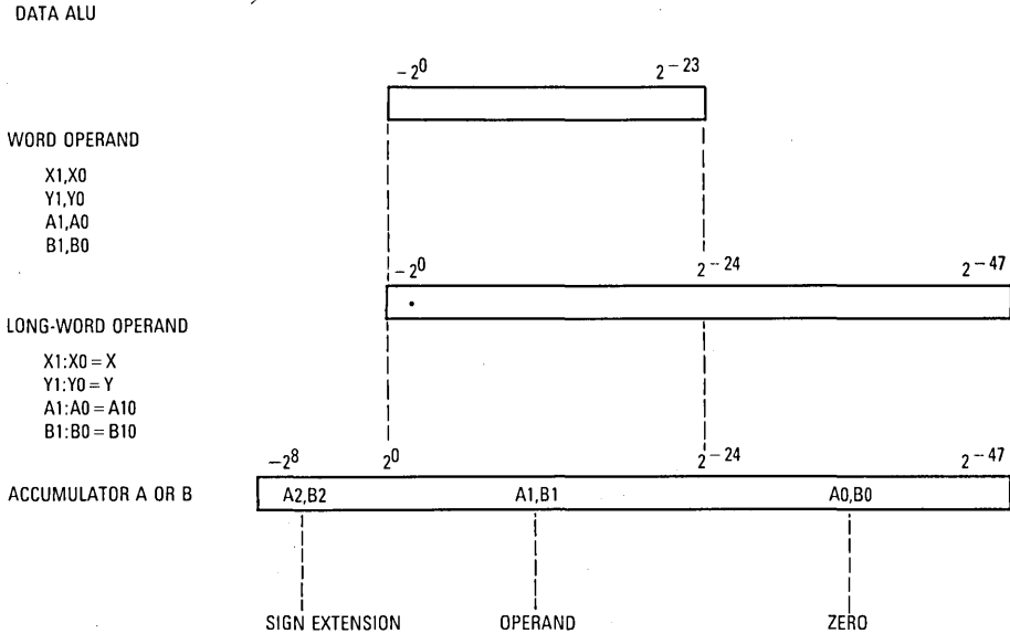
Figure 4-5. Bit Weighting and Alignment of Operands
