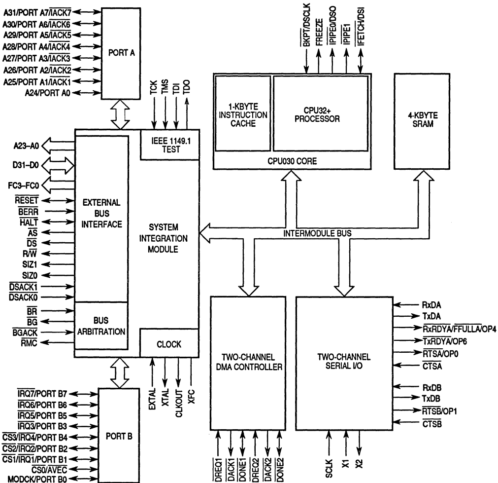
Figure 2-1. Functional Signal Groups
