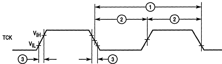
Figure 11-17. Test Clock Input Timing Diagram
