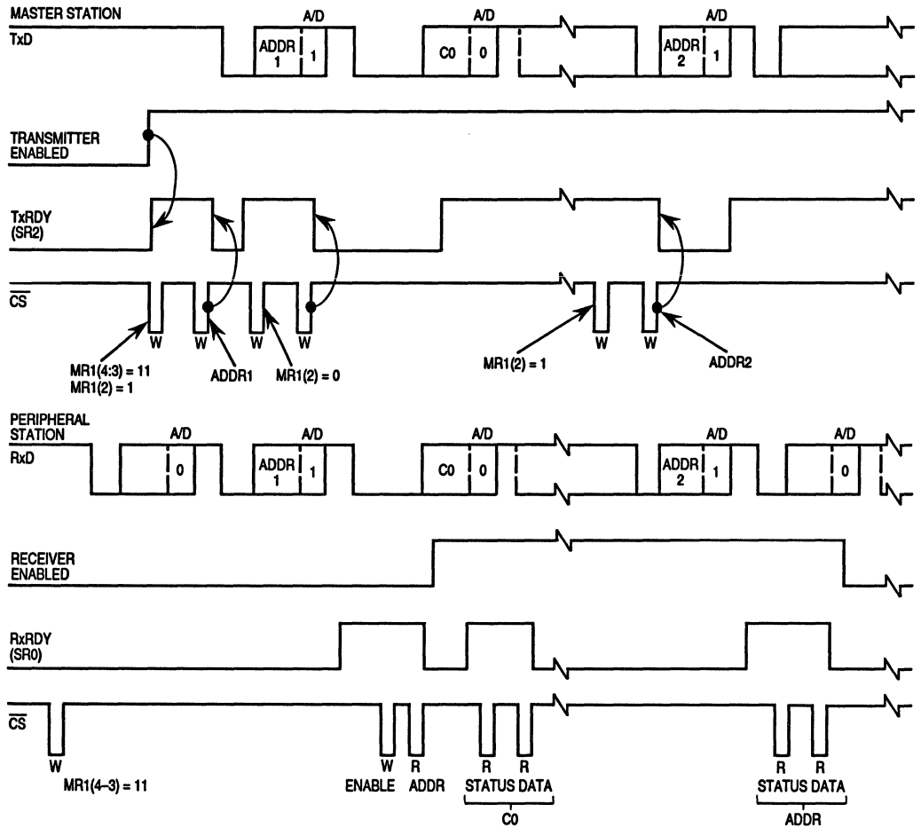
Figure 8-8. Multidrop Mode Timing Diagram
