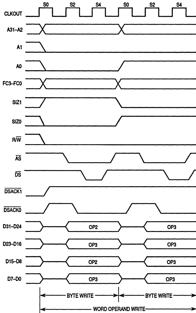
Figure 3-7. Word Operand Write to Byte Port Timing
