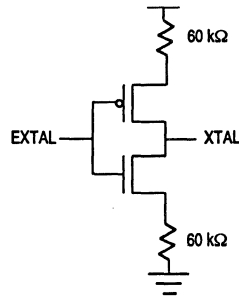
Figure 4-5. MC68349 Crystal Oscillator
