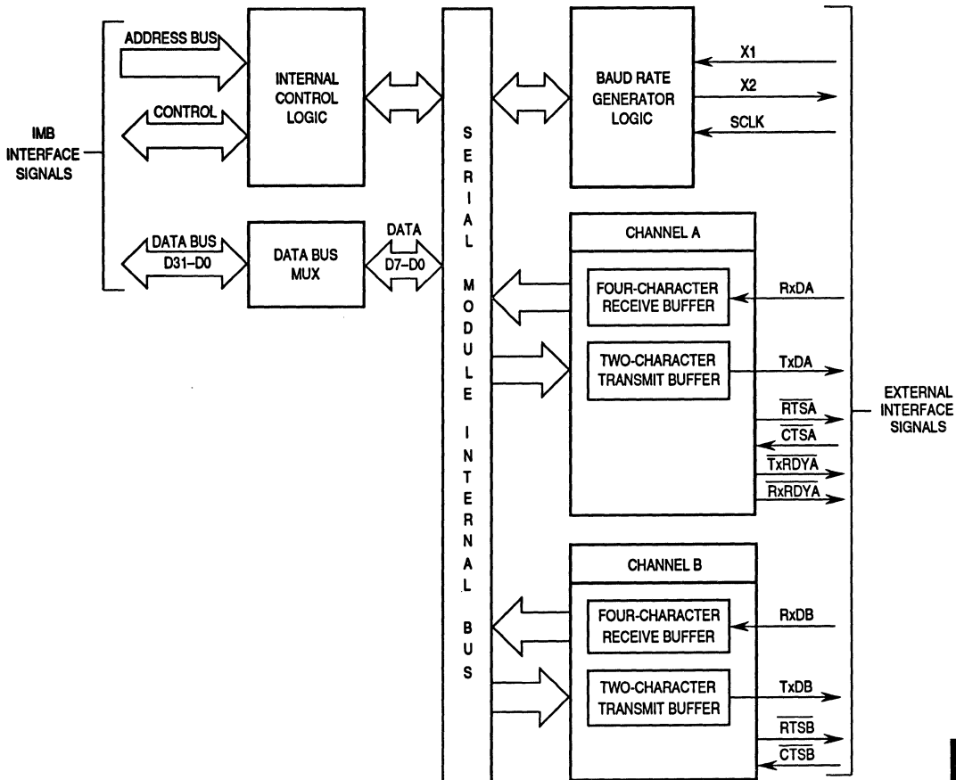
Figure 8-2. External and Internal Interface Signals
