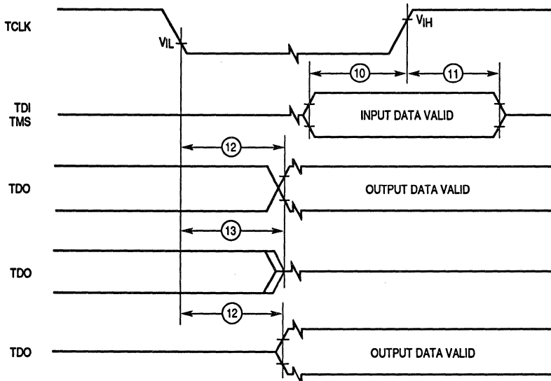
Figure 11-19. Test Access Port Timing Diagram
