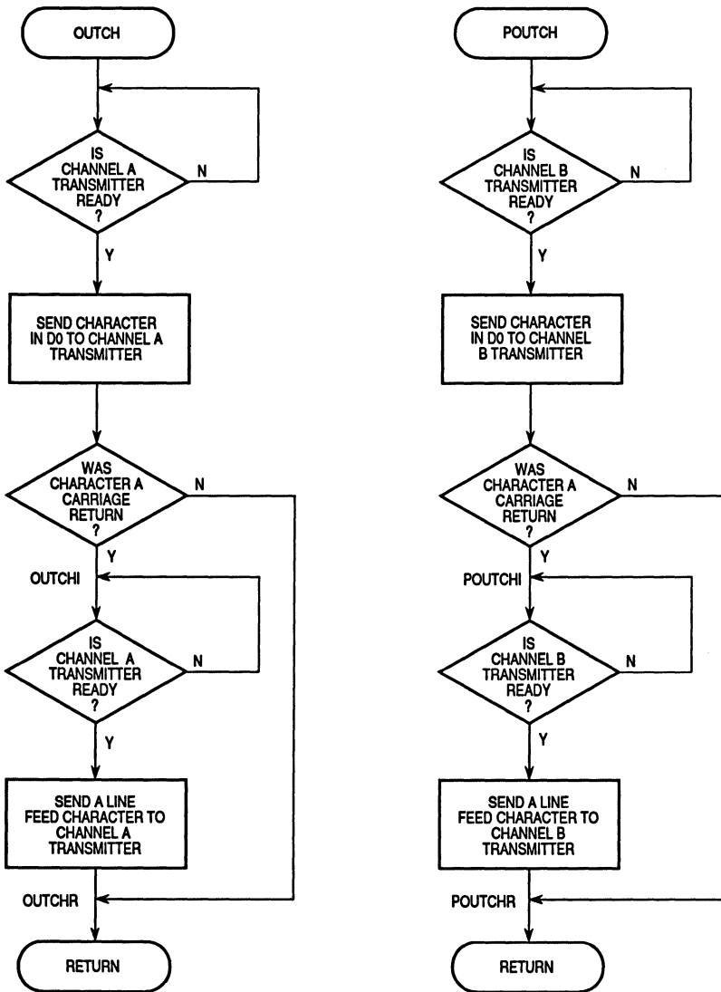
Figure 8-10. Serial Module Programming Flowchart (5 of 5)
