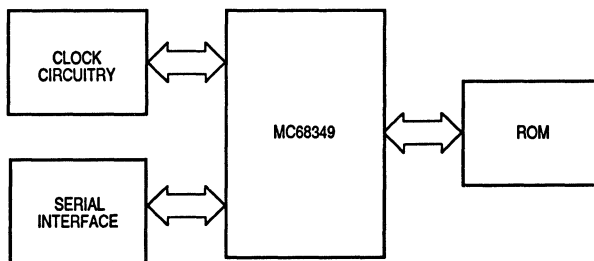
Figure 10-1. Minimum System Configuration Block Diagram
