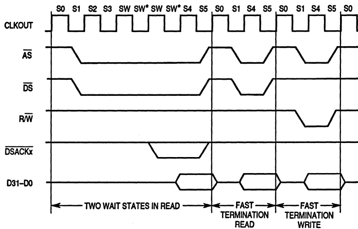
Figure 3-14. Fast Termination Timing
