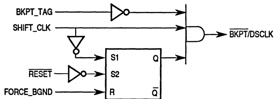
Figure 5-30. \overline{\text{BKPT}}/\text{DSCLK} Logic Diagram
