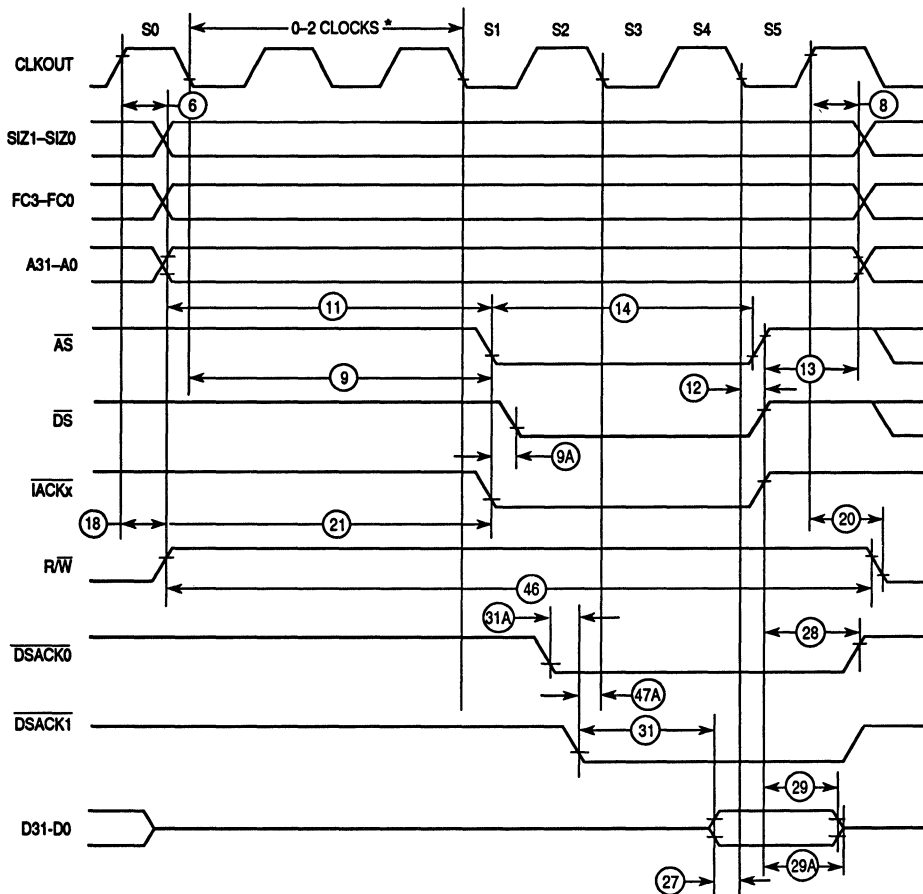
Figure 11-9. \overline{\text{TACK}} Cycle Timing Diagram
