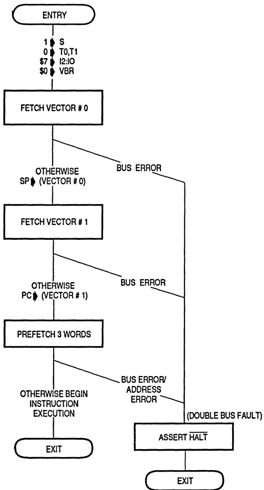
Figure 5-15. Reset Operation Flowchart
