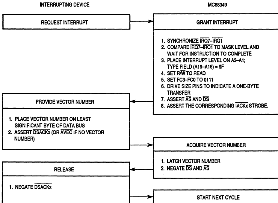
Figure 3-26. Interrupt Acknowledge Cycle Flowchart
