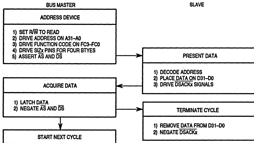
Figure 3-15. Long-Word Read Cycle Flowchart
