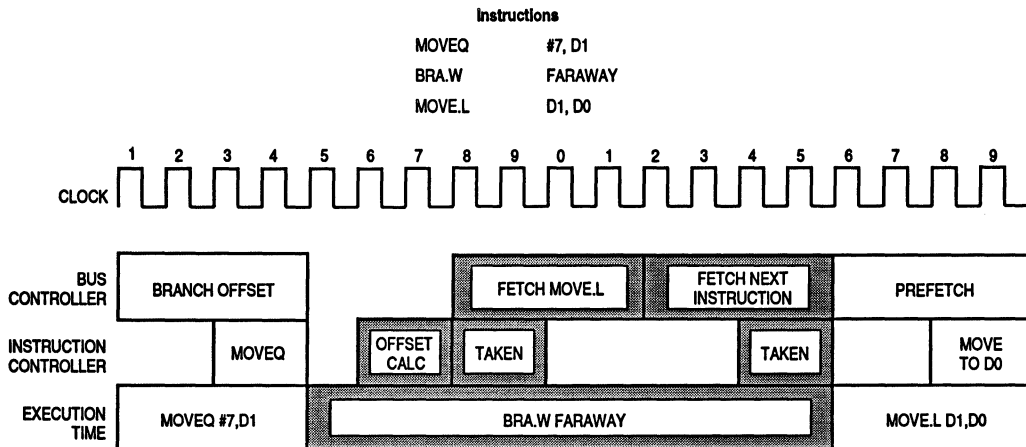
Figure 5-40. Example 3—Branch Negative Tail
