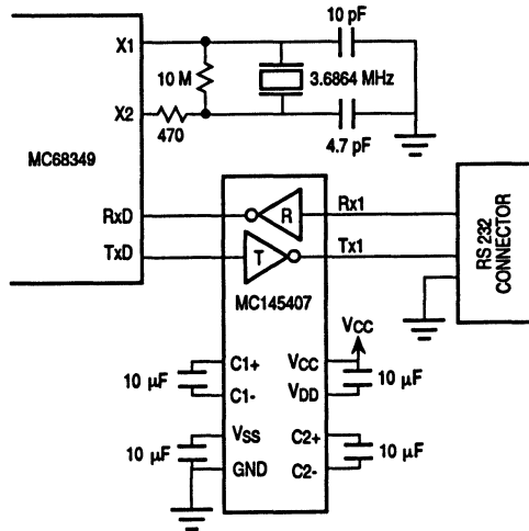
Figure 10-7. Serial Interface
