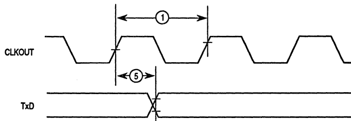
Figure 11-13. Serial Module General Timing Diagram
