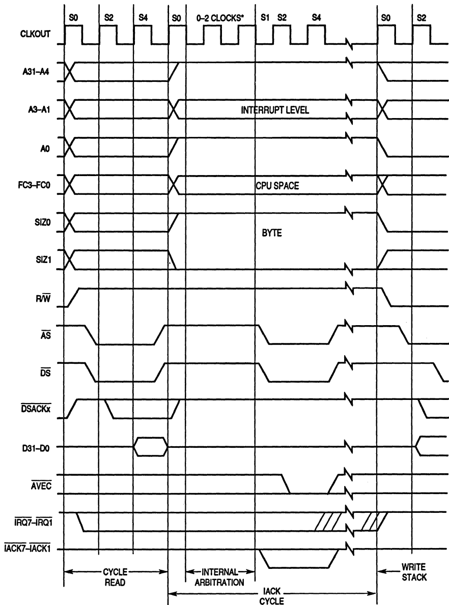
Figure 3-28. Autovector Operation Timing
