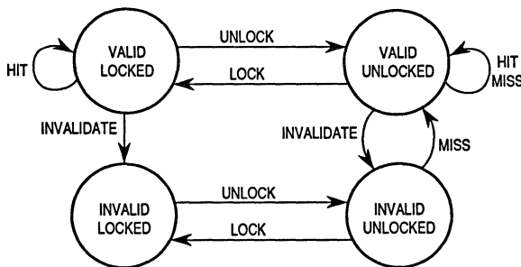
Figure 5-5. Instruction Cache Word State Diagram
