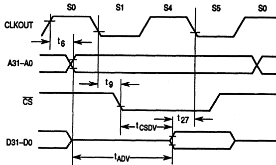
Figure 10-8. Access Time Computation Diagram
