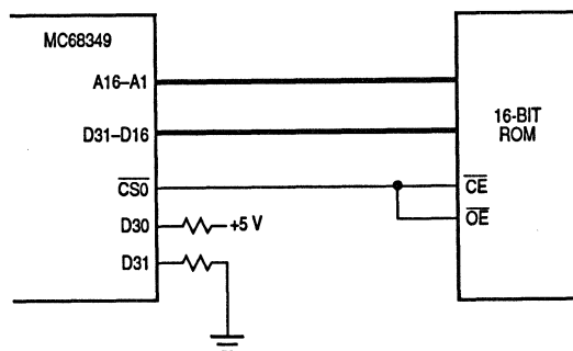
Figure 10-6. ROM Interface
