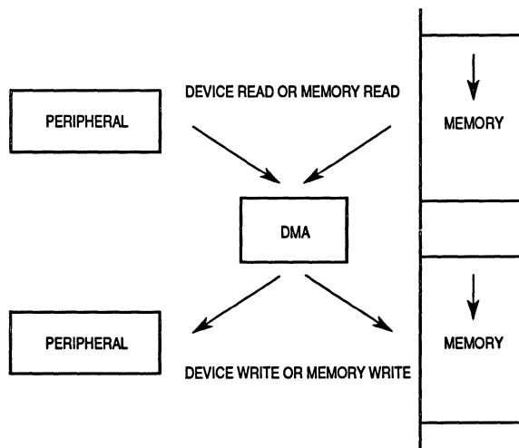
Figure 7-3. Dual-Address Transfer
