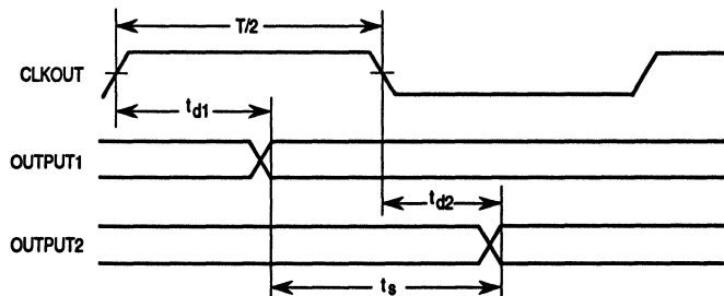
Figure 10-11. Skew between Two Outputs
