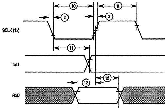
Figure 11-16. Serial Module Synchronous Mode Timing Diagram
