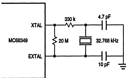
Figure 10-2. Sample Crystal Circuit
