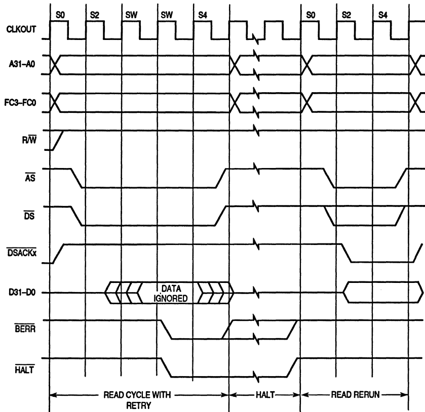
Figure 3-31. Retry Sequence Timing
