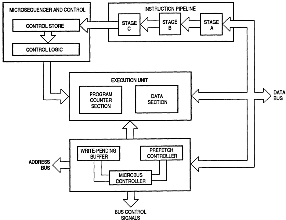
Figure 5-34. Block Diagram of Independent Resources
