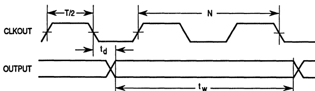
Figure 10-10. Signal Width Specifications
