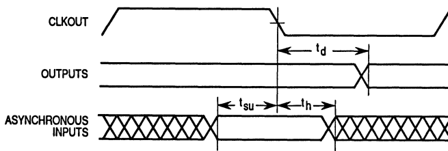
Figure 10-9. Signal Relationships to CLKOUT
