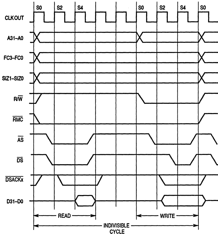
Figure 3-21. Read-Modify-Write Cycle Timing
