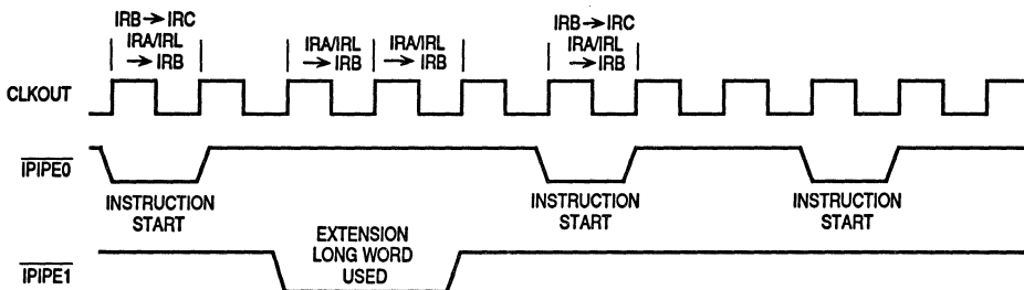
Figure 5-33. Instruction Pipeline Timing Diagram
