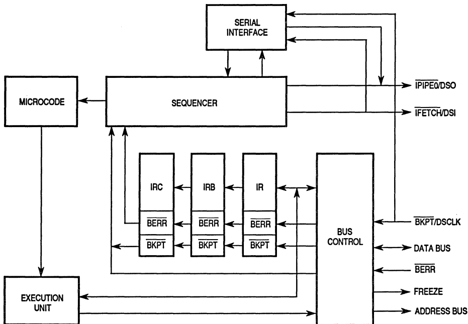
Figure 5-24. BDM Block Diagram
