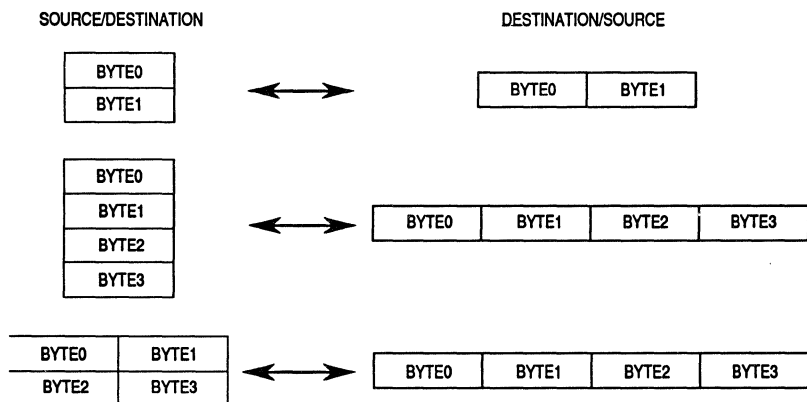
Figure 7-16. Packing and Unpacking of Operands
