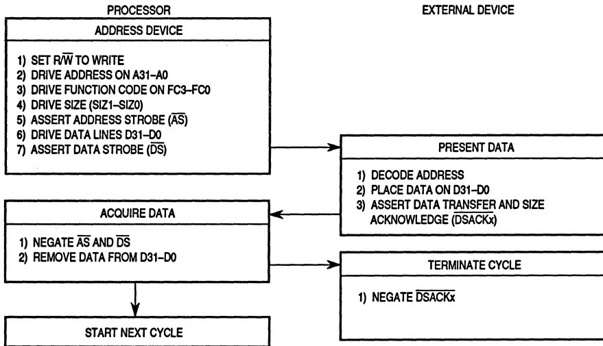
Figure 3-19. Long Word Write Cycle Flowchart
