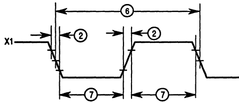
Figure 11-14. Serial Module Asynchronous Mode Timing (X1)
