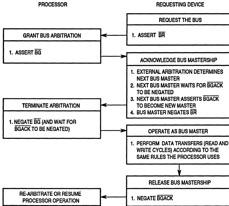
Figure 3-34. Bus Arbitration Flowchart for Single Request
