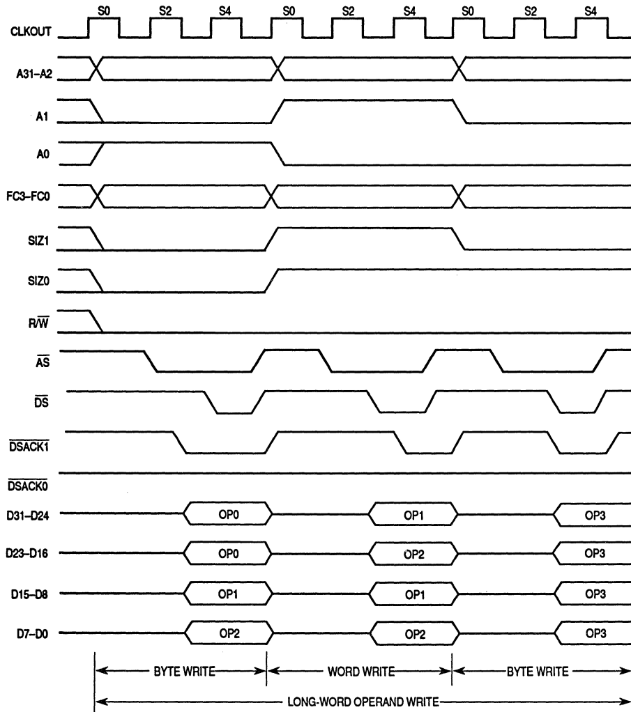
Figure 3-9. Misaligned Long-Word Operand Write to Word Port Timing
