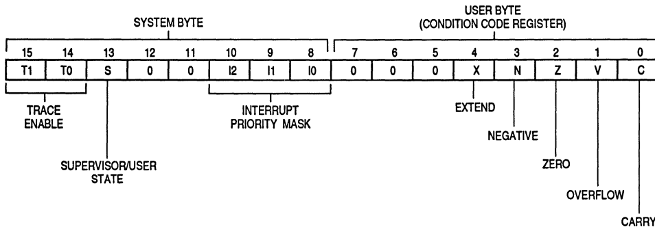
Figure 5-10. Status Register
