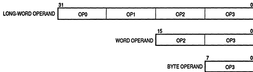
Figure 3-2. Internal Operand Representation
