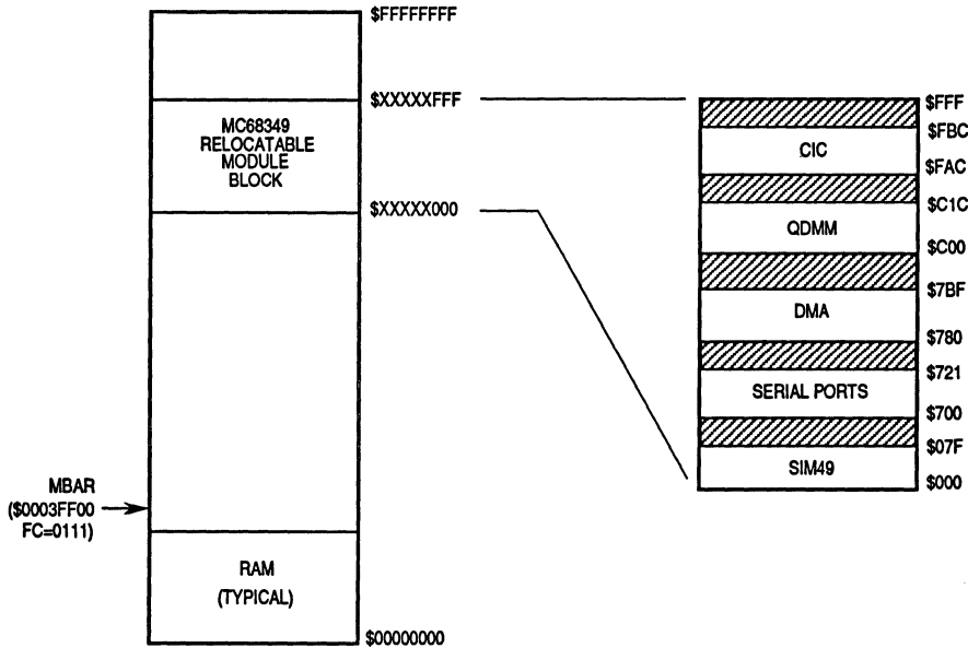
Figure 4-1. SIM49 Module Register Block
