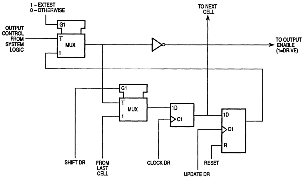
Figure 9-6. Active-Low Output Control Cell (IO.Ct10)
