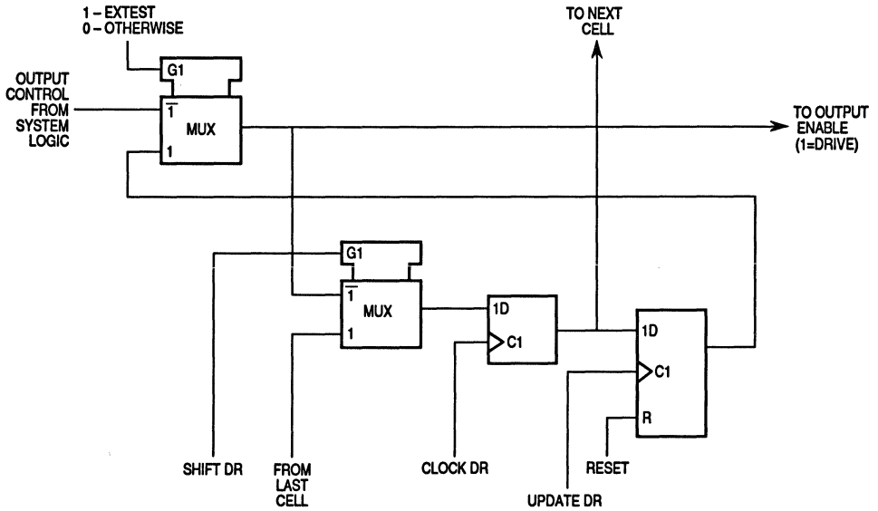
Figure 9-5. Active-High Output Control Cell (IO.Ct11)
