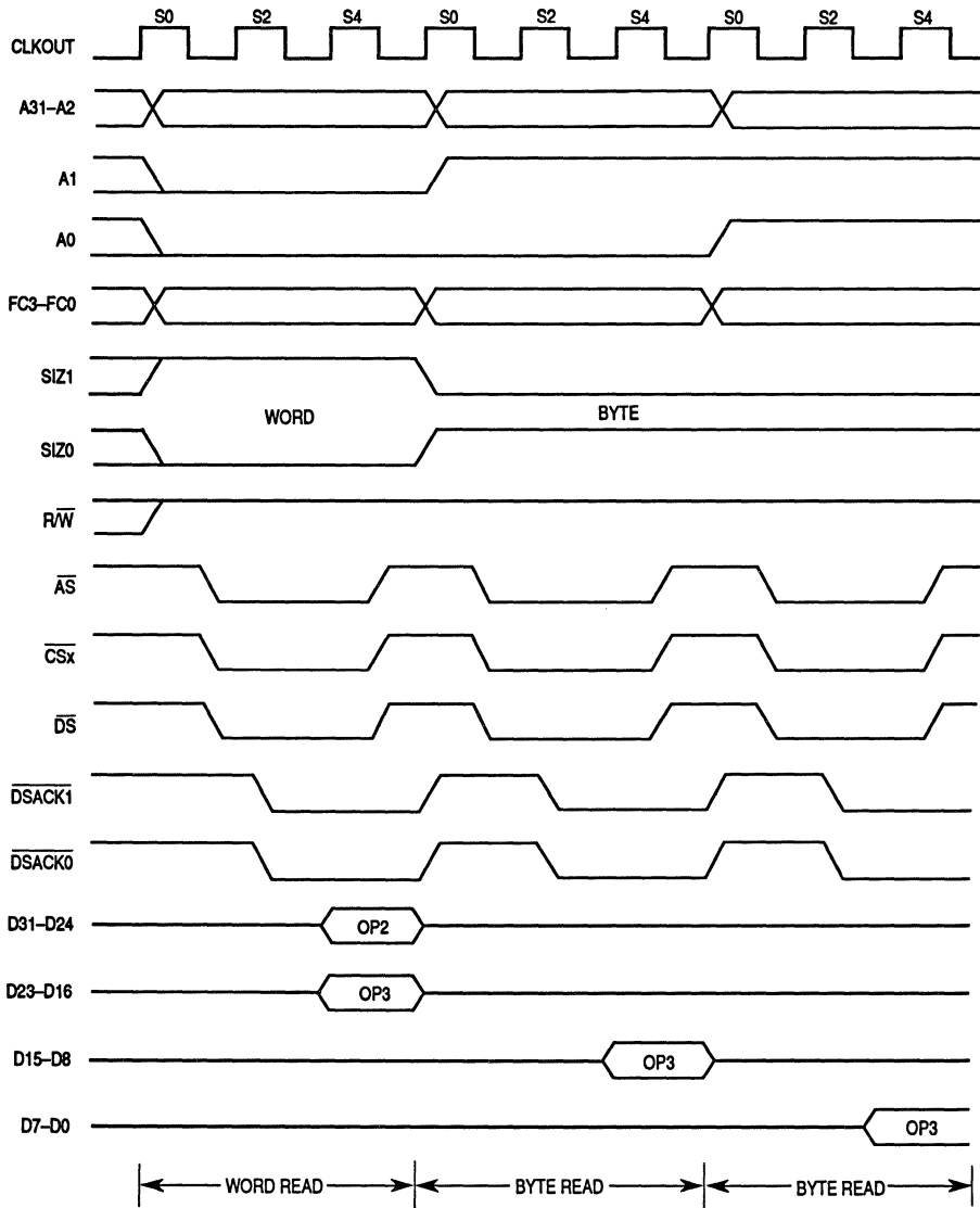
Figure 3-17. Byte and Word Read Cycles—32-Bit Port Timing
