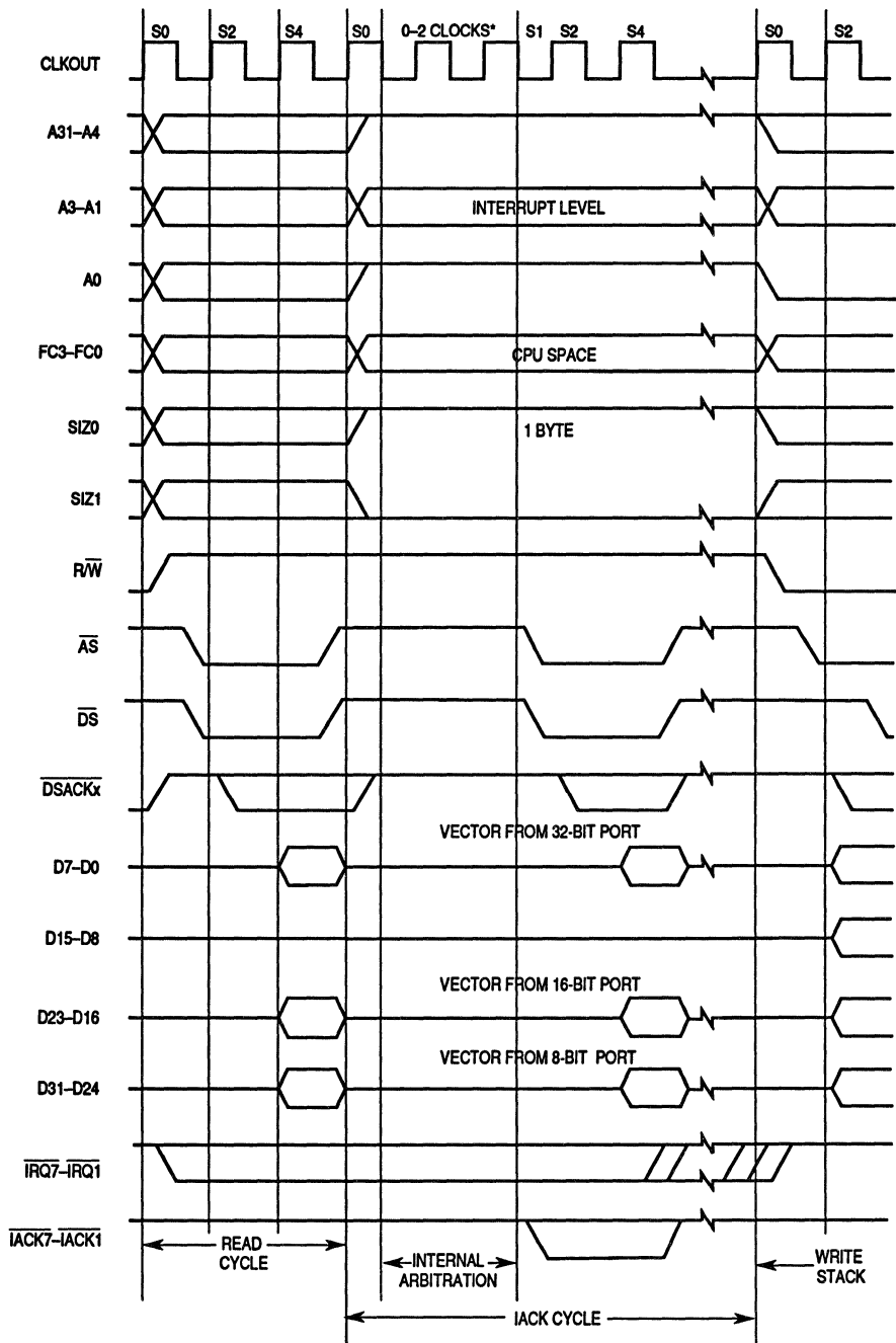
Figure 3-27. Interrupt Acknowledge Cycle Timing
