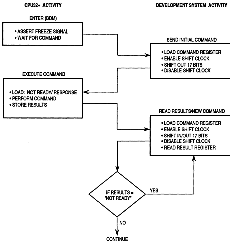
Figure 5-25. BDM Command Execution Flowchart
