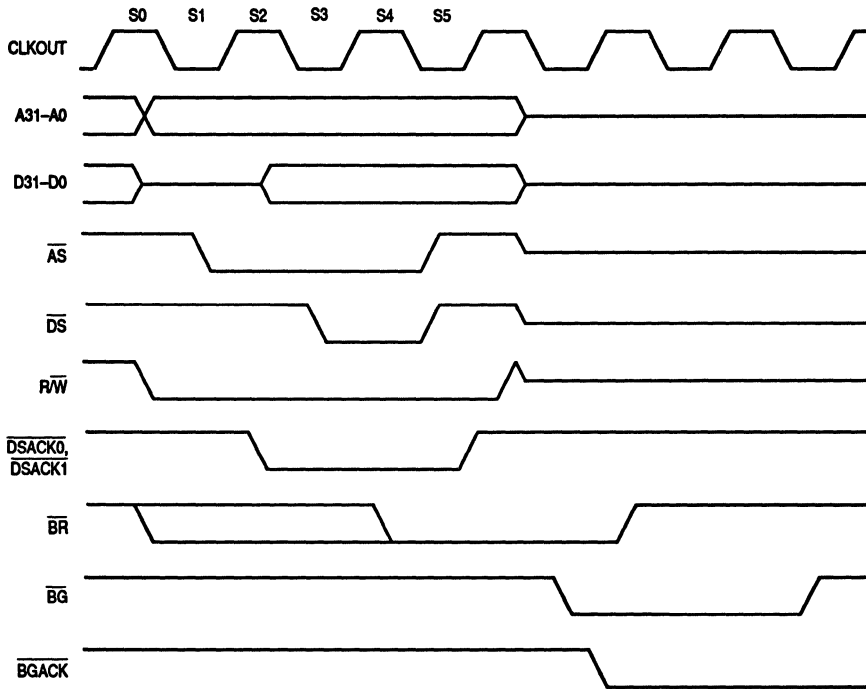
Figure 3-36. Bus Arbitration Timing—Active Bus Case
