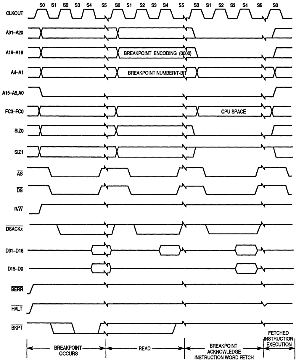
Figure 3-24. Breakpoint Acknowledge Cycle Timing (Opcode Returned)
