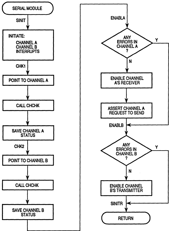
Figure 8-10. Serial Module Programming Flowchart (1 of 5)
