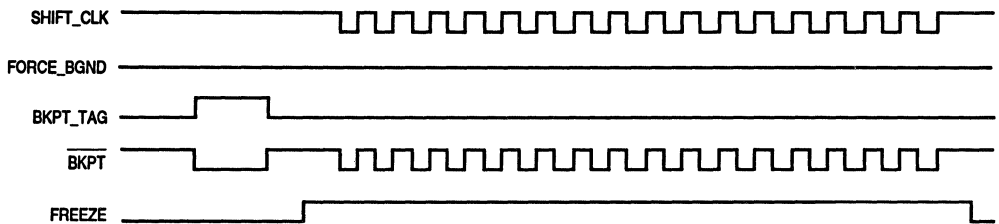
Figure 5-28. \overline{\text{BKPT}} Timing for Single Bus Cycle
