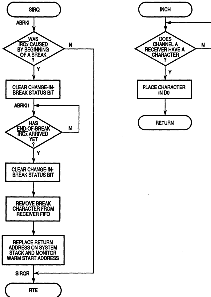
Figure 8-10. Serial Module Programming Flowchart (4 of 5)
