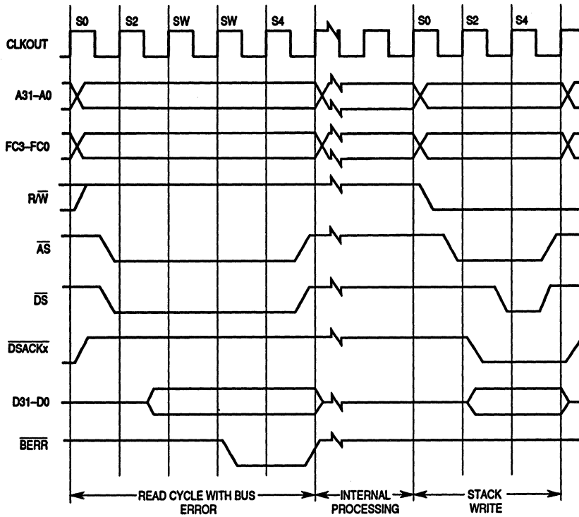
Figure 3-29. Bus Error without \overline{DSACKx} Timing
