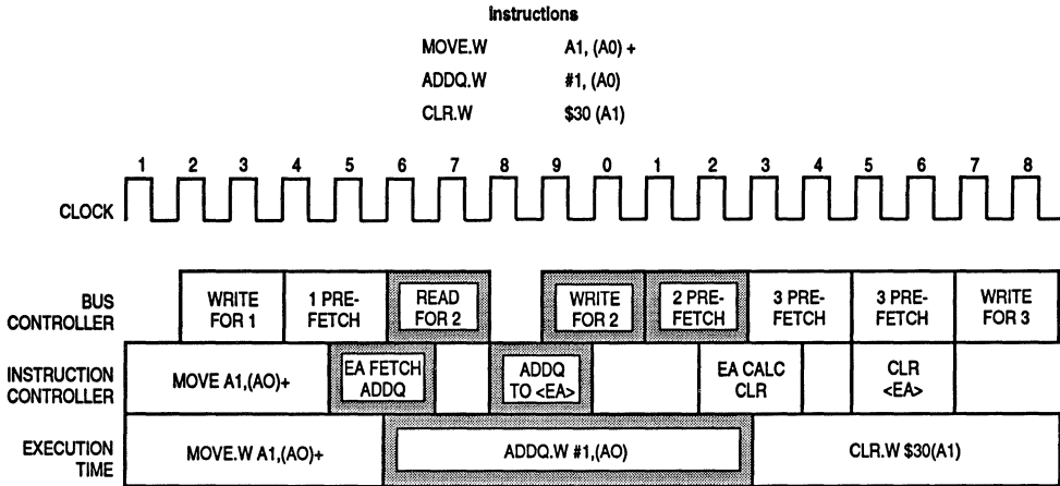
Figure 5-37. Example 1—Instruction Stream
