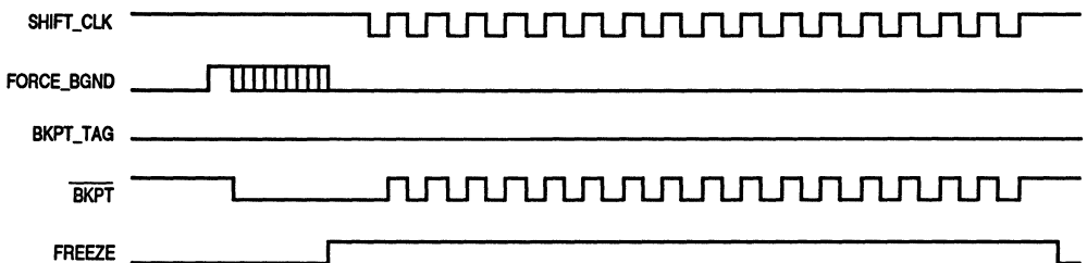
Figure 5-29. \overline{\text{BKPT}} Timing for Forcing BDM
