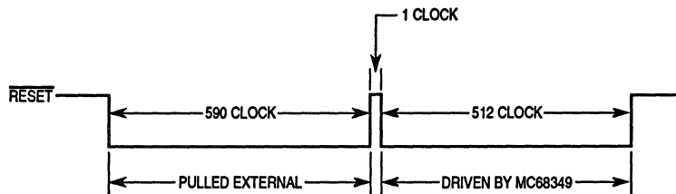
Figure 3-39. Timing for External Devices Driving \overline{RESET}
