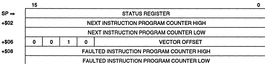
Figure 5-17. Format $2—Six-Word Stack Frame
