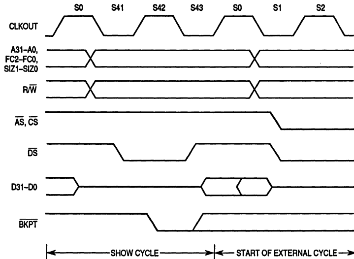
Figure 3-38. Show Cycle Timing
