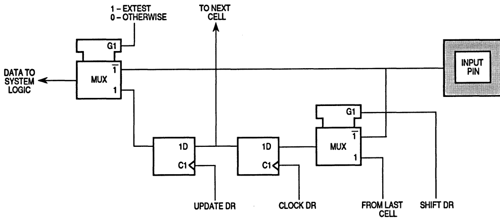
Figure 9-4. Input Pin Cell (I.Pin)
