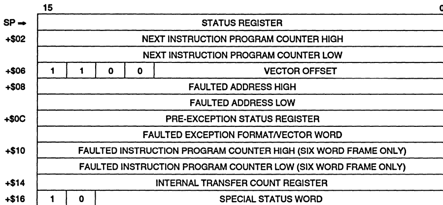
Figure 5-21. Format $C—Four- and Six-Word Bus Error Stack
