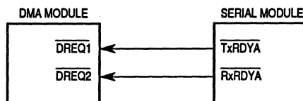
Figure 7-4. DMA External Connections to Serial Module
