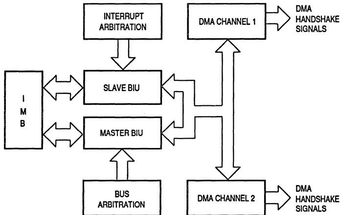
Figure 7-1. DMA Block Diagram
