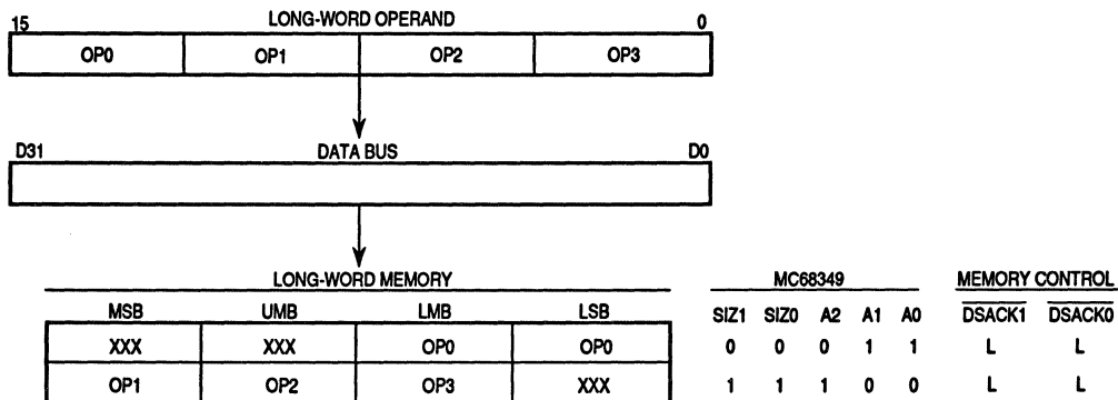
Figure 3-12. Misaligned Long-Word Operand Write to Long-Word Port Example
