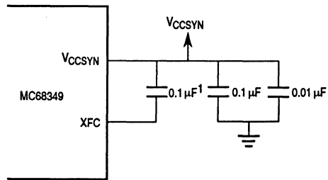
Figure 10-4. XFC and VCCSYN Capacitor Connections
