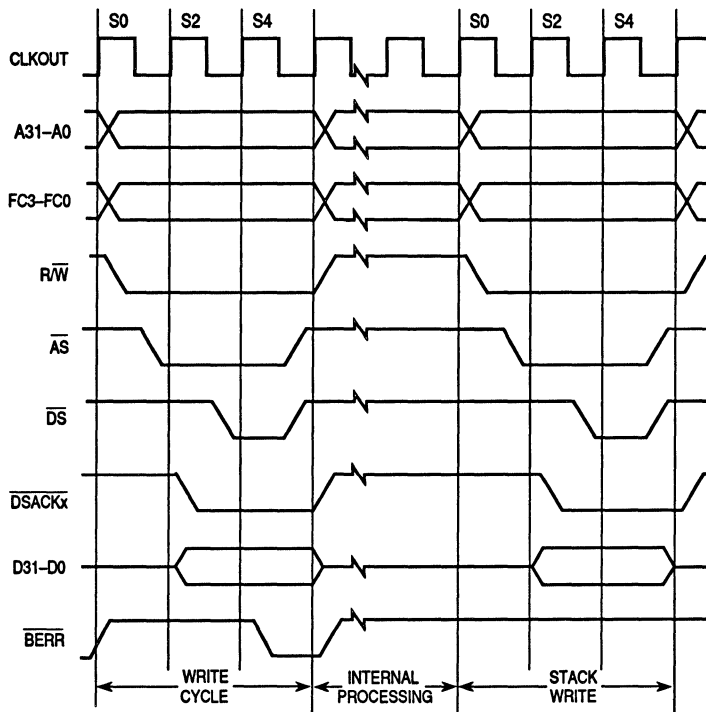
Figure 3-30. Late Bus Error with \overline{DSACKx} Timing
