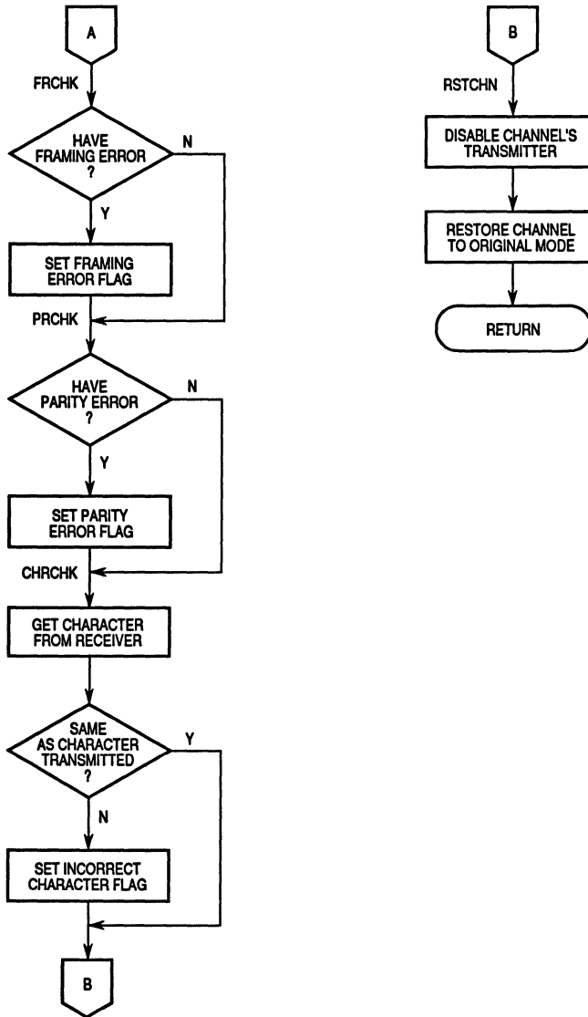
Figure 8-10. Serial Module Programming Flowchart (3 of 5)
