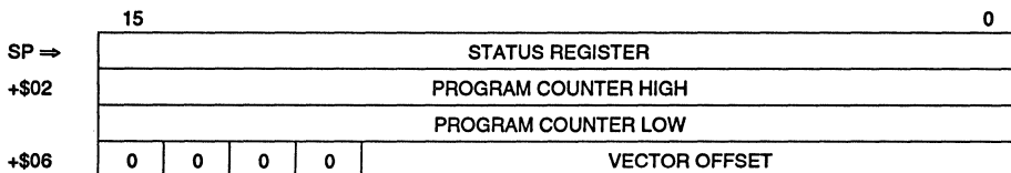
Figure 5-16. Format $0—Four-Word Stack Frame
