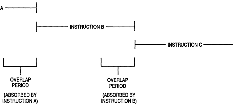
Figure 5-36. Attributed Instruction Times
