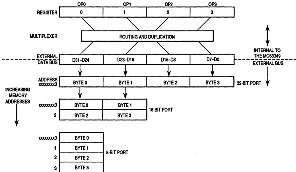
Figure 3-3. MC68349 Interface to Various Port Sizes
