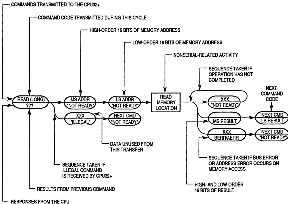
Figure 5-31. Command Sequence Diagram
