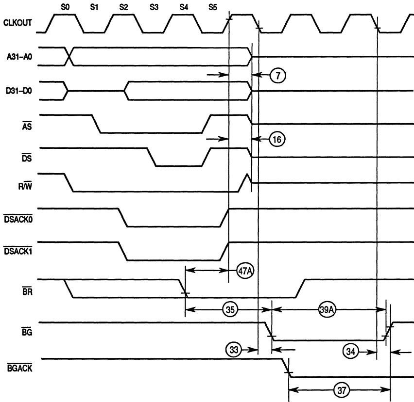
Figure 11-6. Bus Arbitration Timing—Active Bus Case
