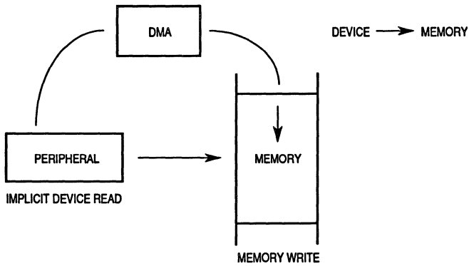
Figure 7-2. Single-Address Transfers
