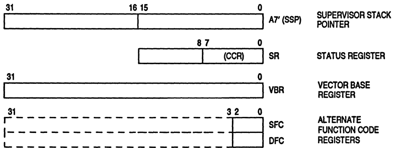
Figure 5-9. Supervisor Programming Model Supplement
