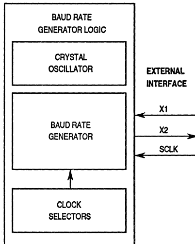
Figure 8-3. Baud Rate Generator Block Diagram
