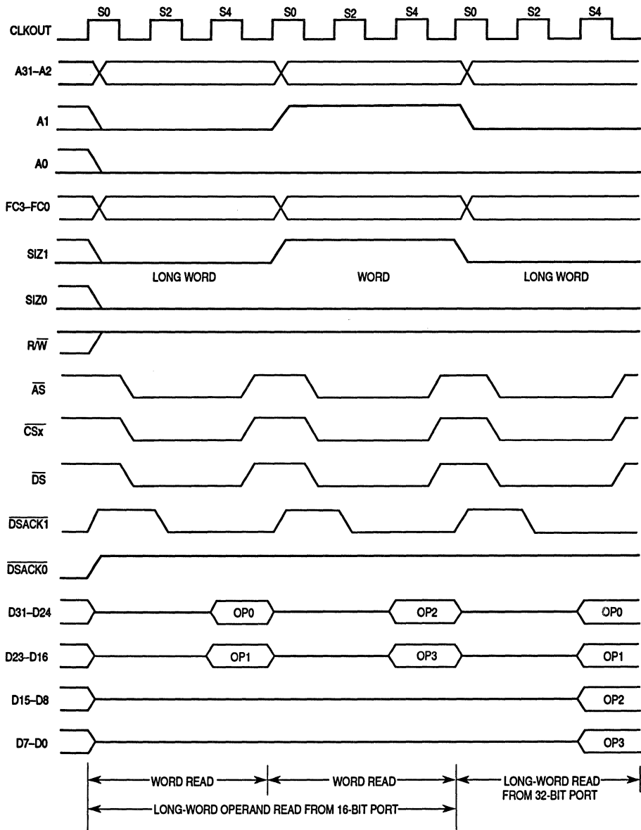
Figure 3-18. Long-Word Read—16-Bit and 32-Bit Port Timing
