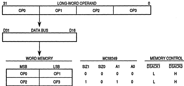
Figure 3-4. Long-Word Operand Write to Word Port Example
