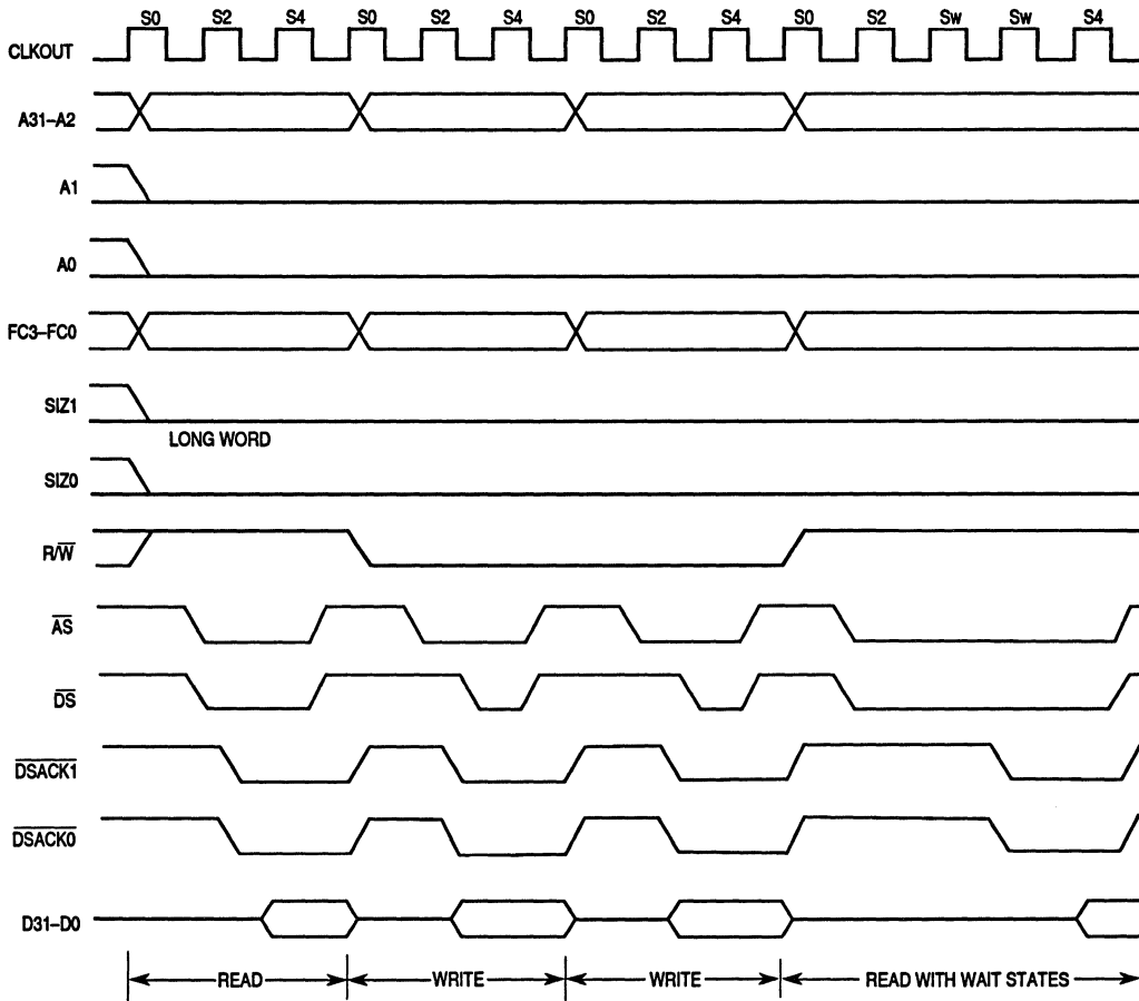
Figure 3-20. Read-Write-Read Cycles—32-Bit Port Timing
