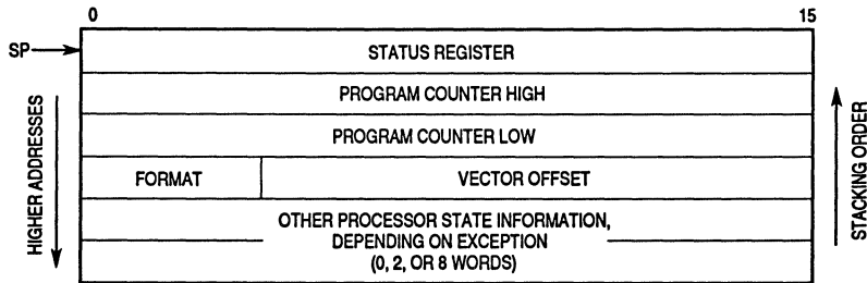
Figure 5-14. Exception Stack Frame
