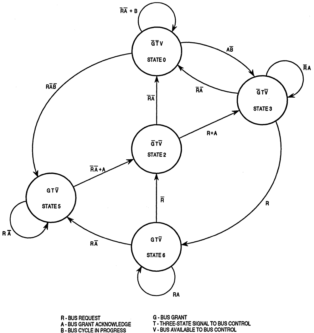
Figure 3-37. Bus Arbitration State Diagram
