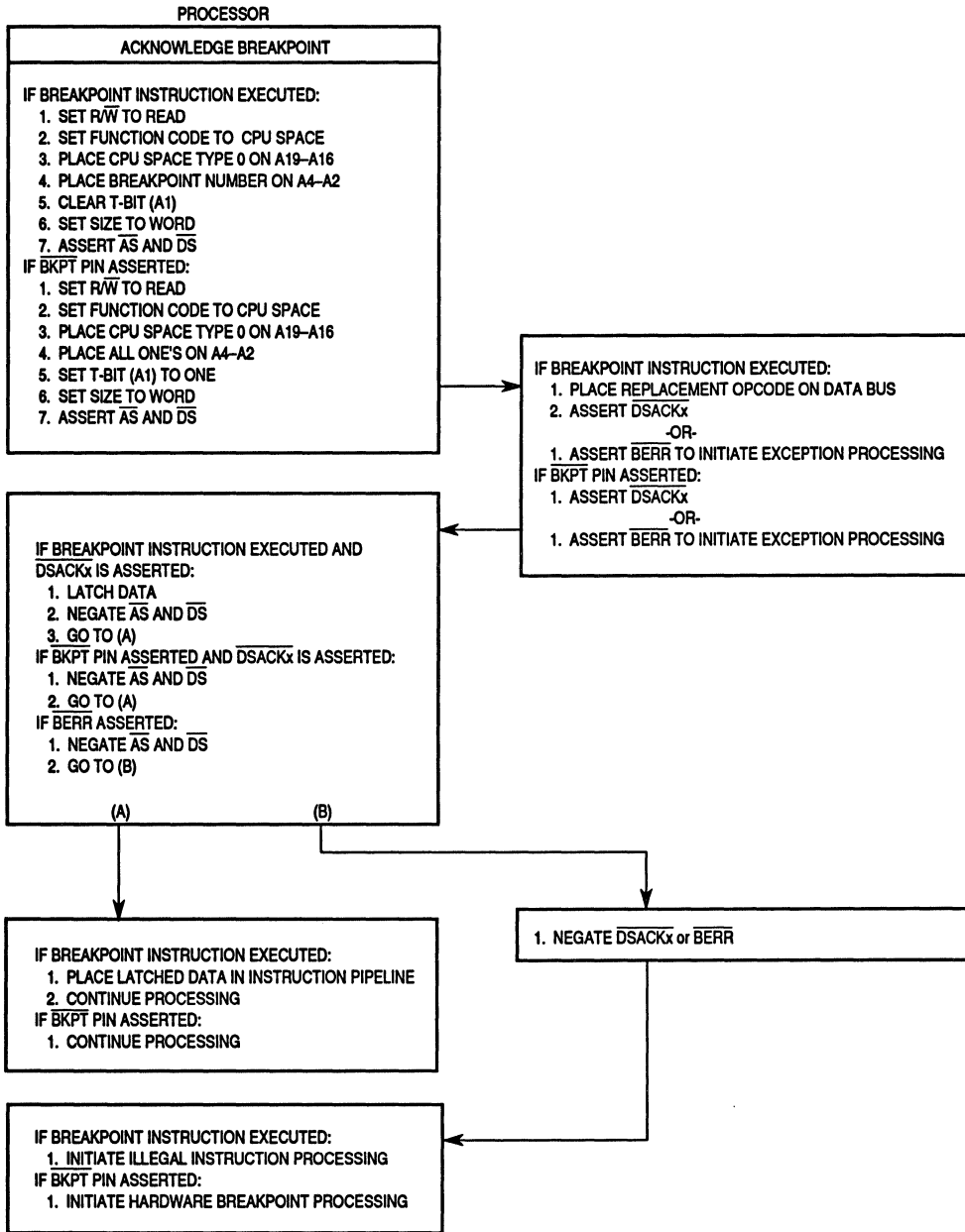
Figure 3-23. Breakpoint Operation Flowchart
