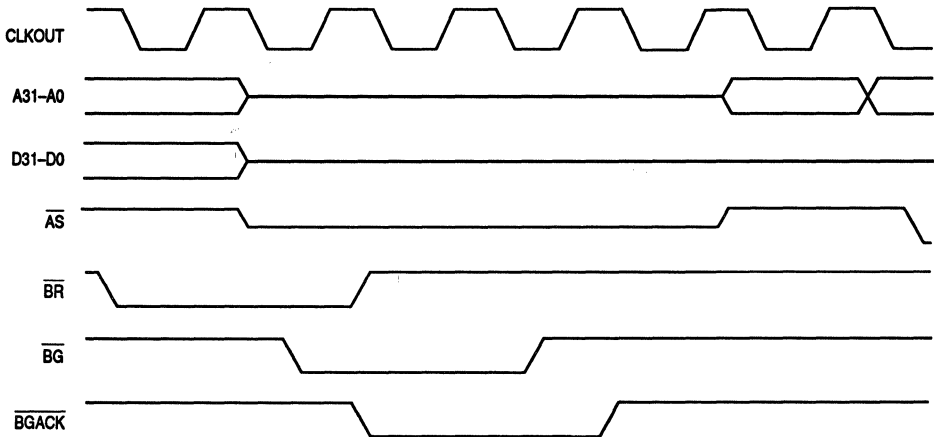
Figure 3-35. Bus Arbitration Timing—Idle Bus Case
