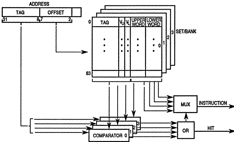
Figure 5-4. Instruction Cache
