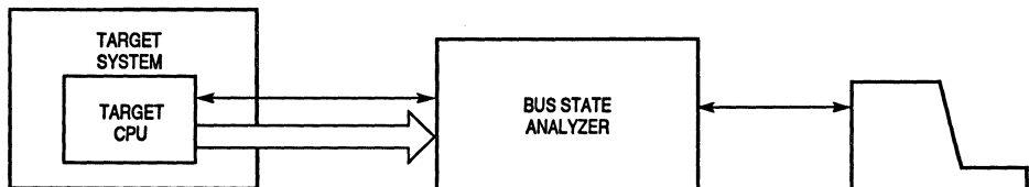
Figure 5-23. Bus State Analyzer Configuration
