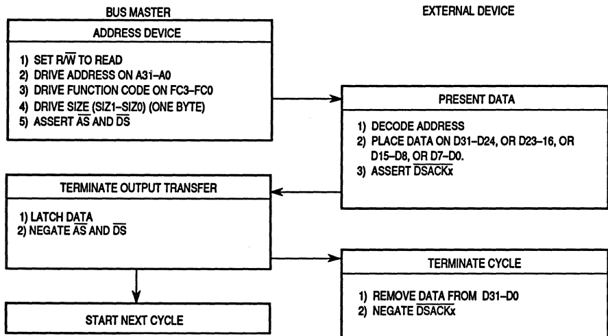
Figure 3-16. Byte Read Cycle Flowchart
