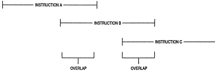
Figure 5-35. Simultaneous Instruction Execution
