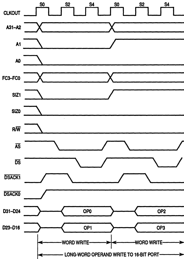
Figure 3-5. Long-Word Operand Write to Word Port Timing
