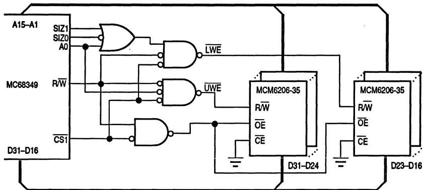
Figure 10-5. SRAM Interface
