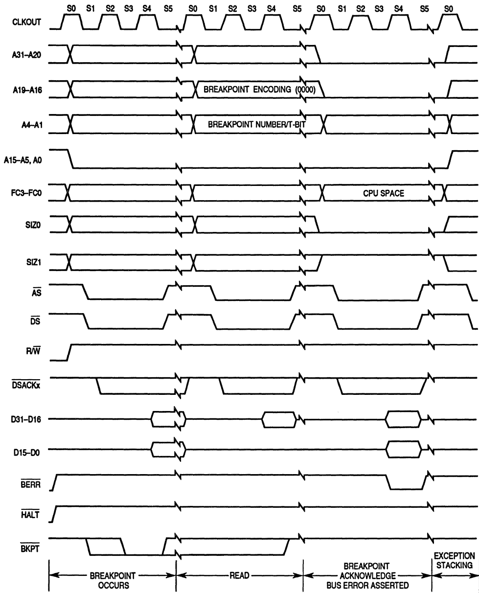
Figure 3-25. Breakpoint Acknowledge Cycle Timing (Exception Signaled)
