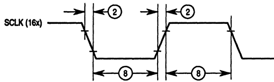
Figure 11-15. Serial Module Asynchronous Mode Timing (SCLK-16X)
