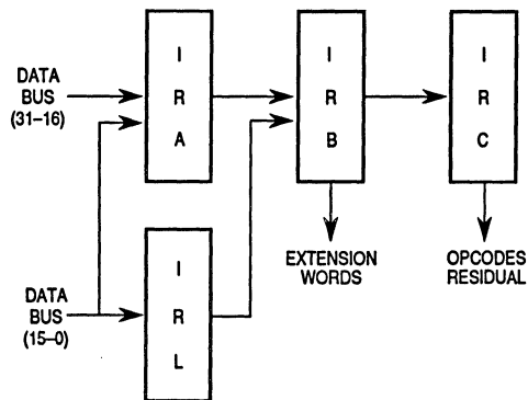
Figure 5-32. Functional Model of Instruction Pipeline
