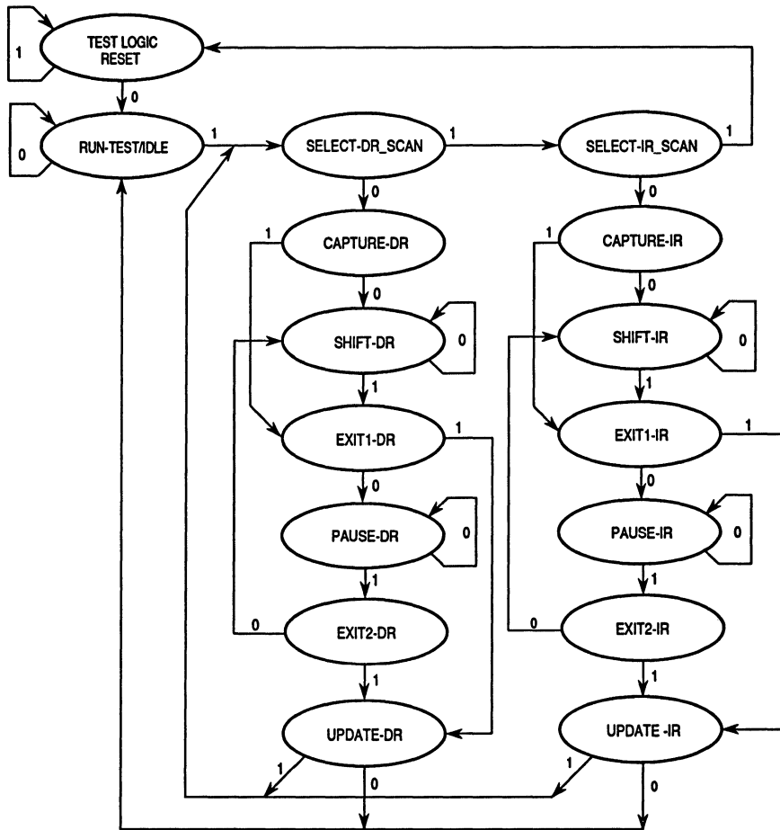
Figure 9-2. TAP Controller State Machine
