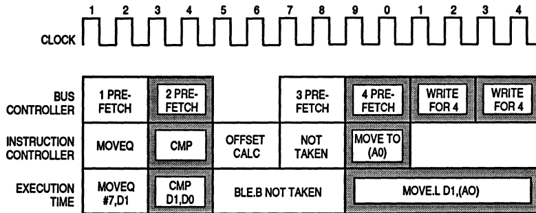
Figure 5-39. Example 2—Branch Not Taken
