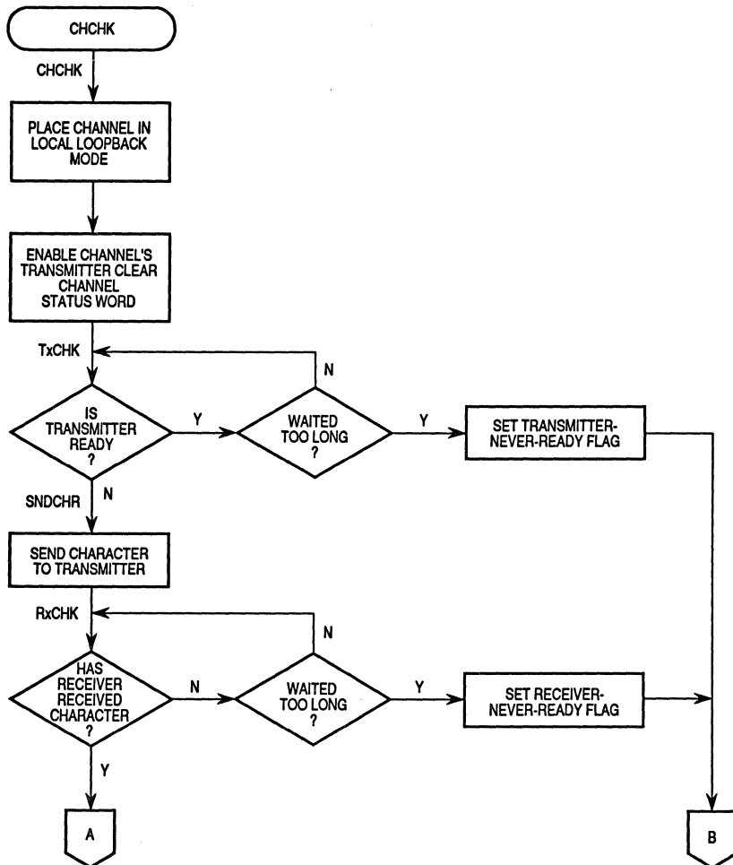
Figure 8-10. Serial Module Programming Flowchart (2 of 5)
