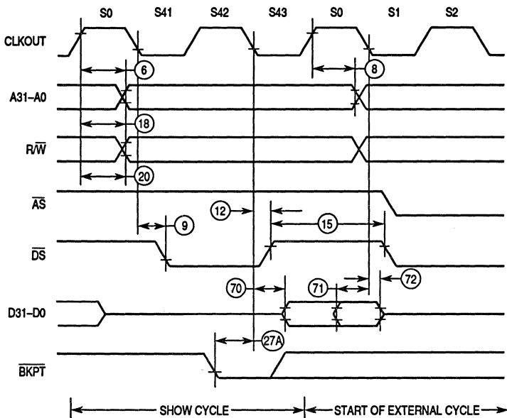
Figure 11-8. Show Cycle Timing Diagram
