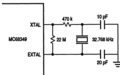
Figure 10-3. Statek Corporation Crystal Circuit
