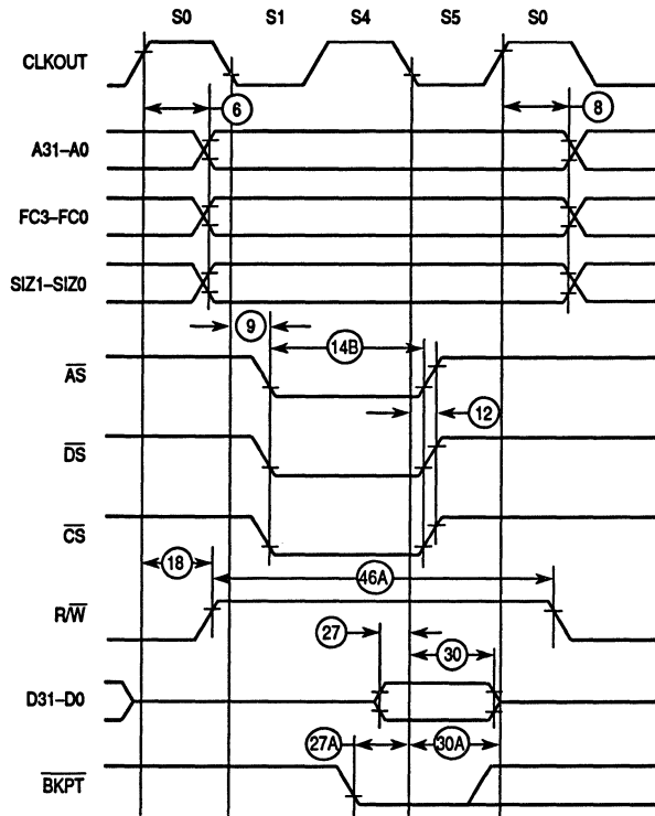
Figure 11-4. Fast Termination Read Cycle Timing Diagram
