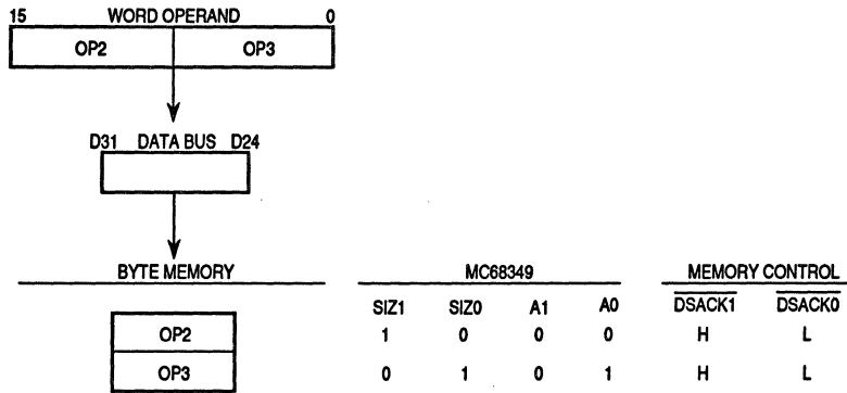
Figure 3-6. Word Operand Write to Byte Port Example
