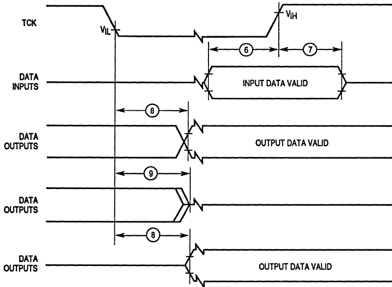
Figure 11-18. Boundary Scan Timing Diagram
