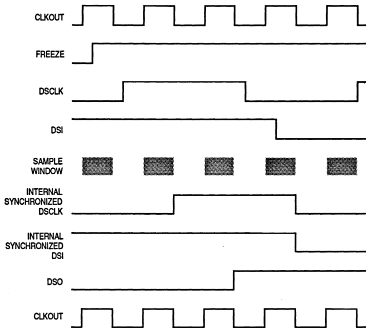
Figure 5-27. Serial Interface Timing Diagram
