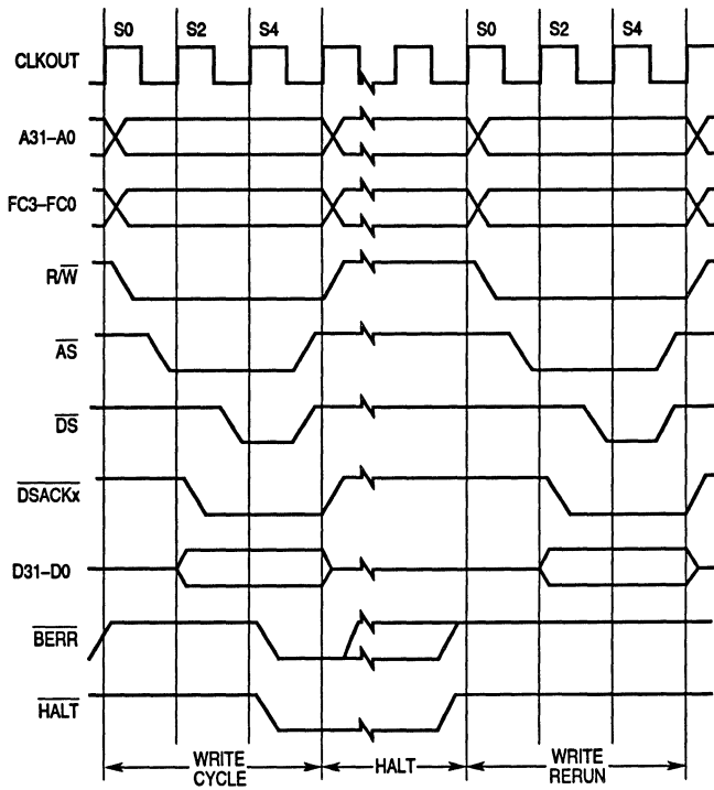
Figure 3-32. Late Retry Sequence Timing
