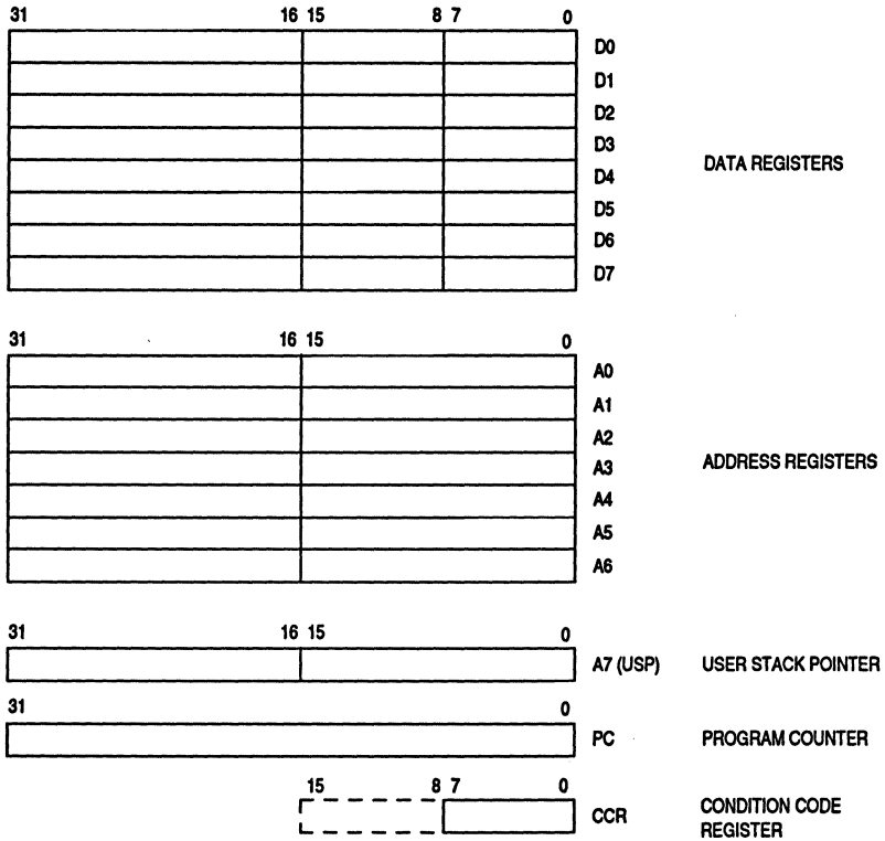
Figure 5-8. User Programming Model
