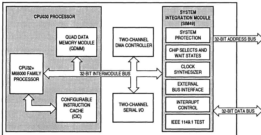
Figure 1-1. MC68349 Block Diagram
