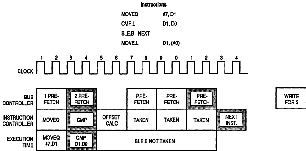
Figure 5-38. Example 2—Branch Taken
