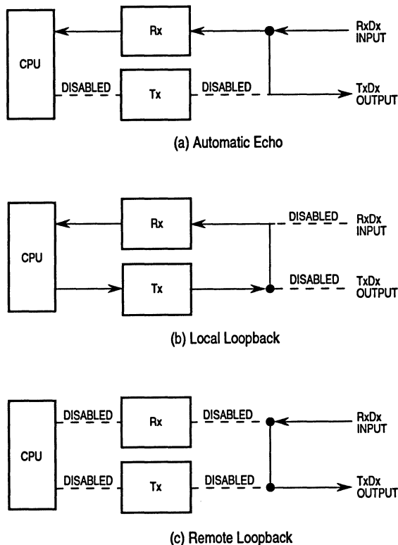
Figure 8-7. Looping Modes Functional Diagram
