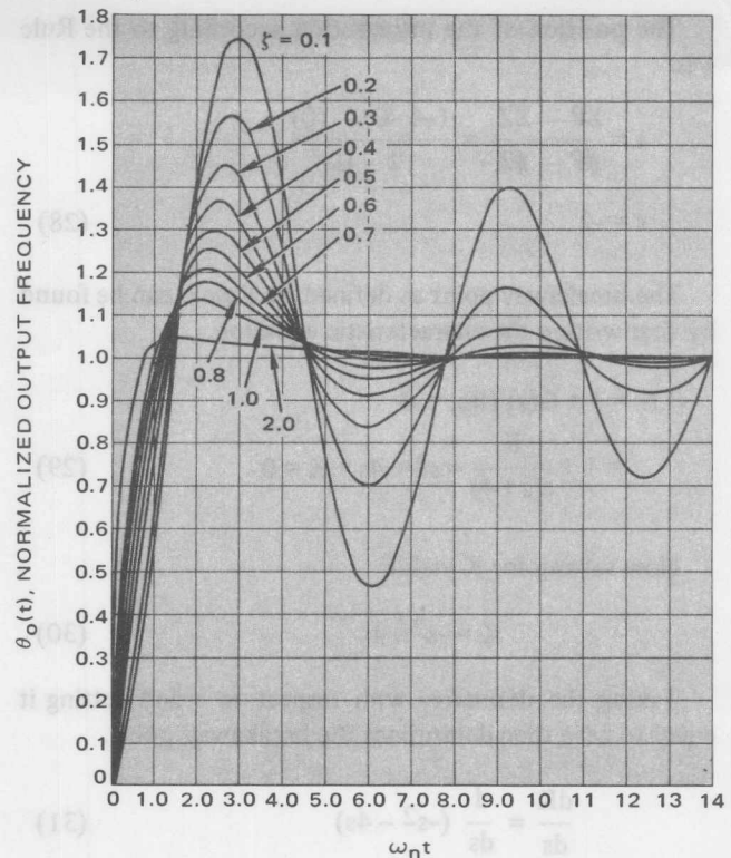
FIGURE 6 – Type 2 Second Order Step Response
