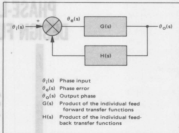
FIGURE 1 – Feedback System
