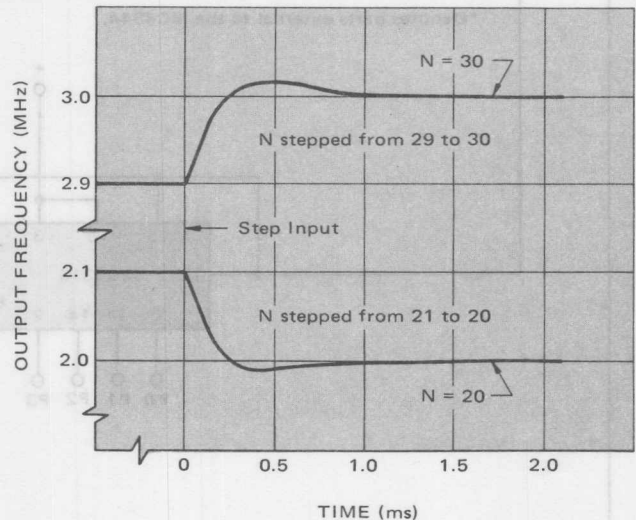
FIGURE 13 – Frequency-Time Response
