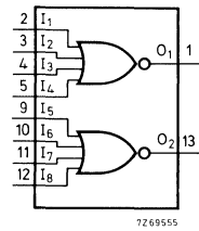
Dual 4-input NOR gate.
