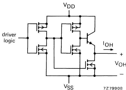
Fig. 3 Schematic diagram of output stage.
