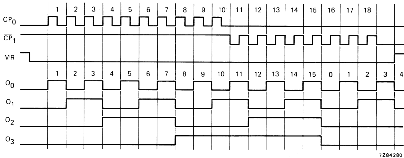
Fig. 6 Timing diagram.
