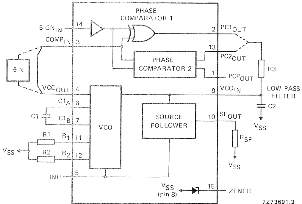
Fig. 1 Functional diagram.
