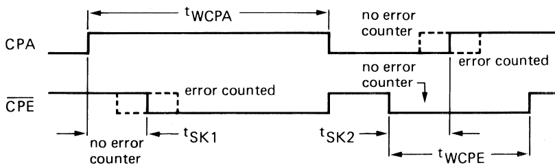
Fig. 4 Skew times timing diagram; t_{WCPA} > t_{SK1} ; t_{WCE} > t_{SK2} .
