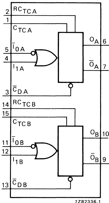
Fig. 1 Functional diagram.
