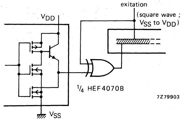
Fig. 14 Connection to liquid crystal (LCD) display readout. Direct d.c. drive of LCDs not recommended for life of LCD readouts.
