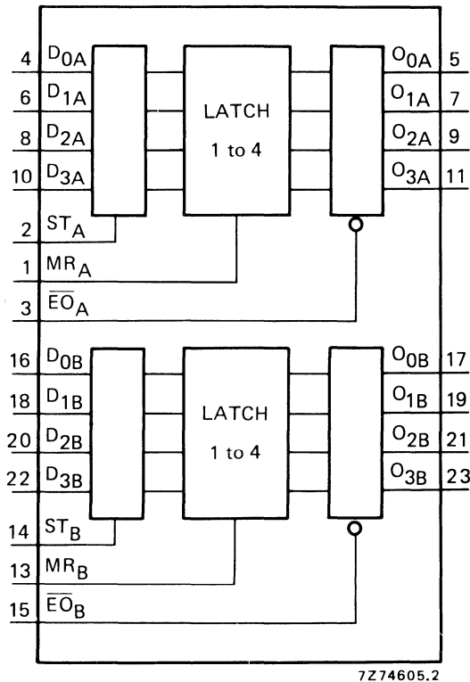
Fig. 1 Functional diagram.
