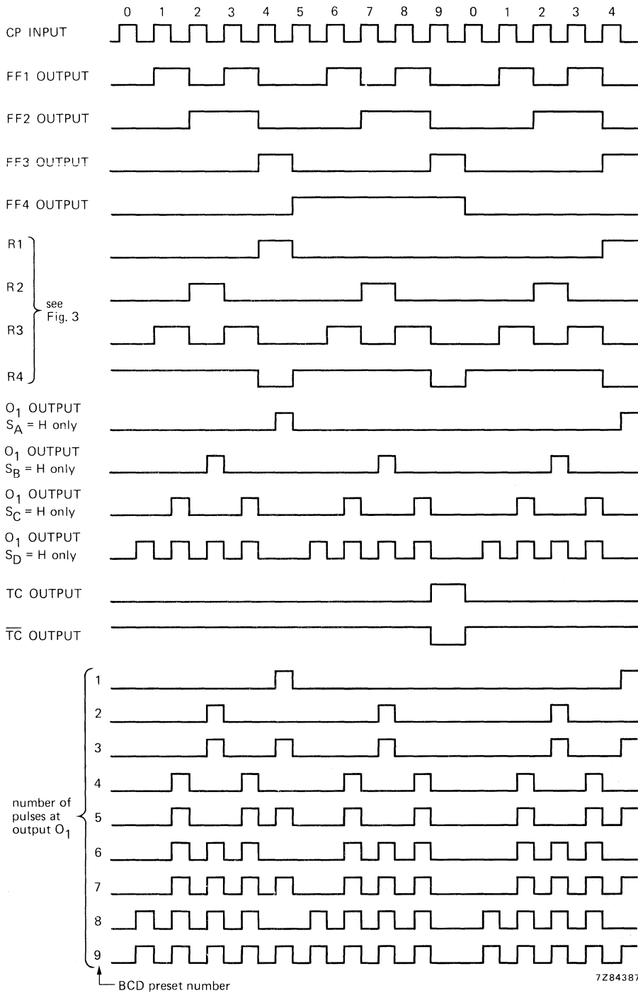
Fig. 4 Timing diagram.
