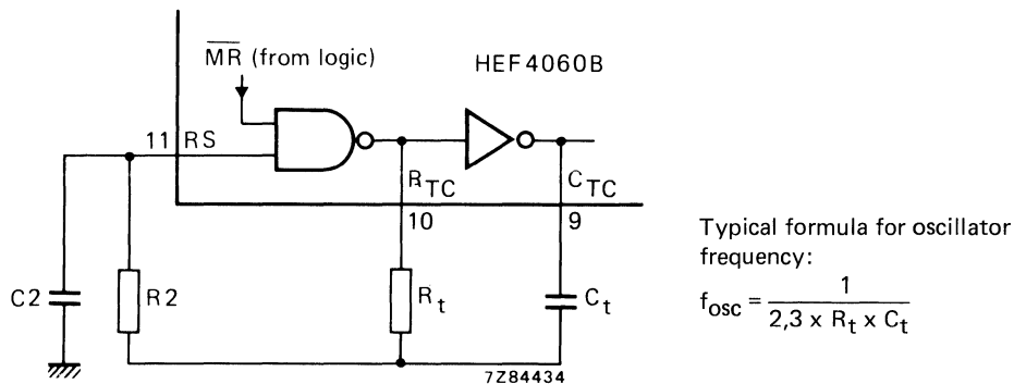
Fig. 4 External component connection for RC oscillator.
