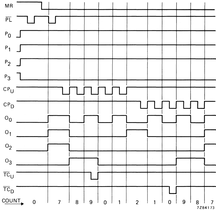
Fig. 6 Timing diagram.
