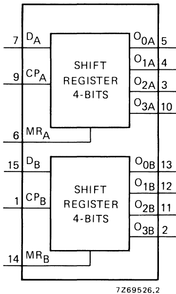
Fig. 1 Functional diagram.
