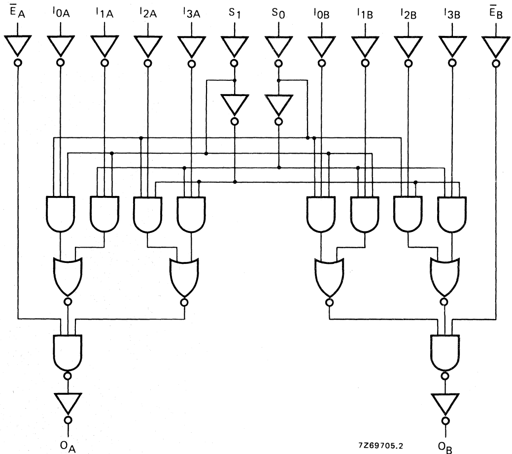
Fig. 3 Logic diagram.
