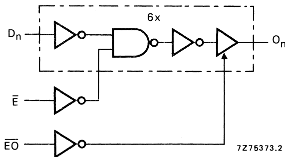
Fig. 3 Logic diagram.
