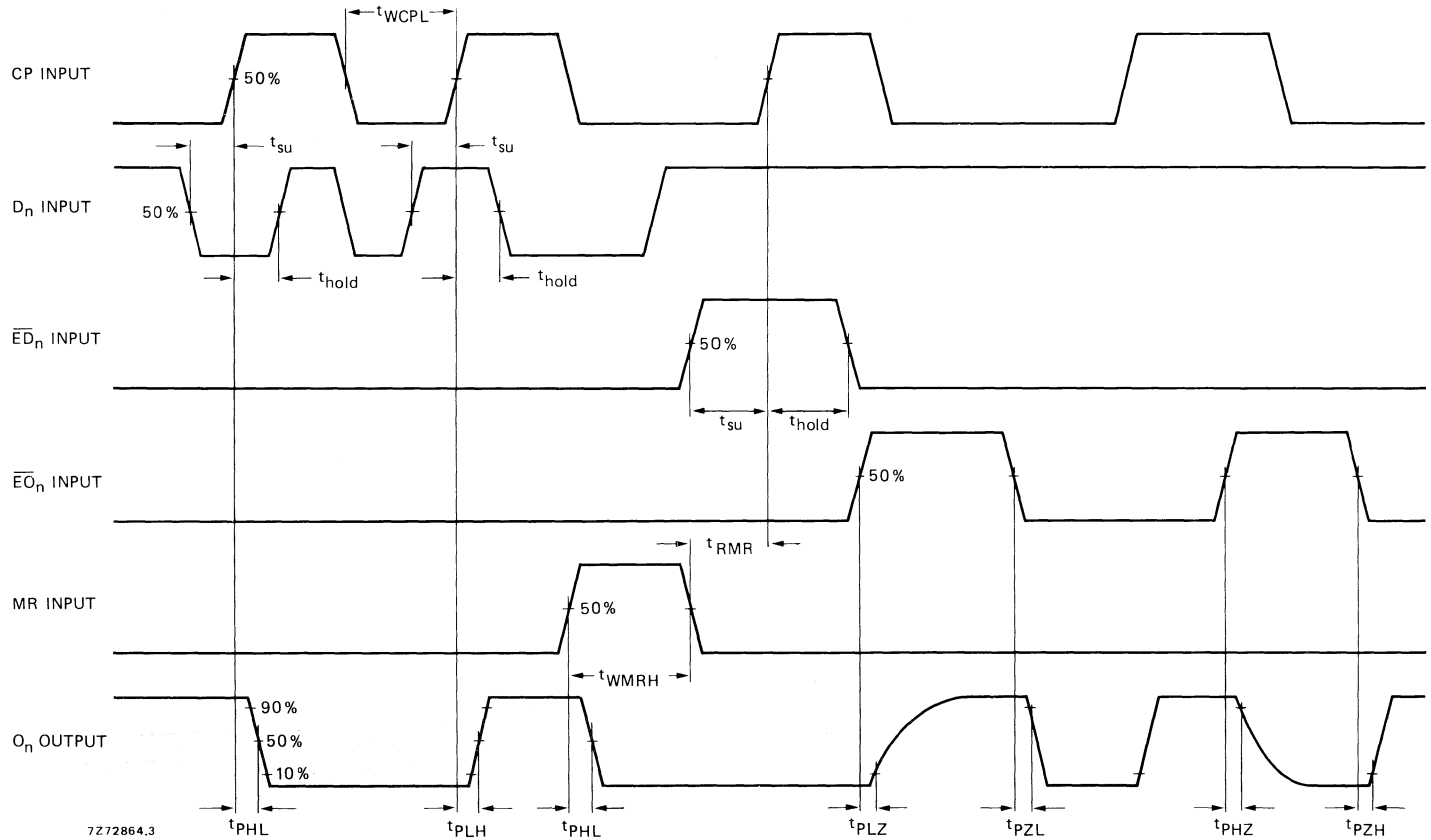
Fig. 4 Waveforms showing propagation delays, output disable/enable times, minimum CP and MR pulse widths, set-up and hold times for D_n to CP and \overline{E}D_n to CP, and recovery time for MR. Set-up and hold times are shown as positive values but may be specified as negative values.
