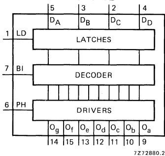
BCD to 7-segment latch/decoder/driver.
