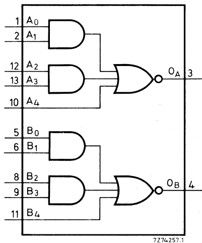
Fig. 1 Functional diagram.
