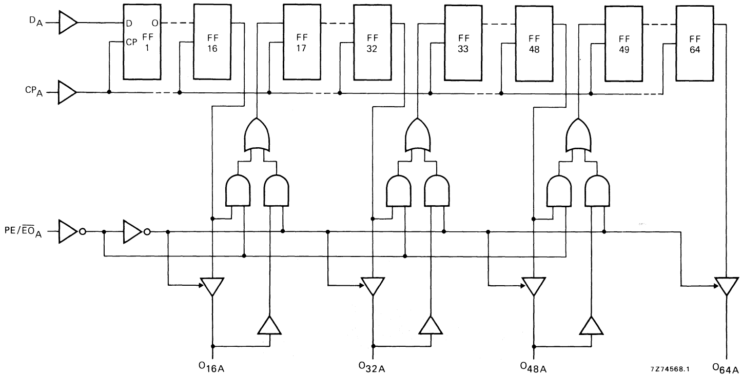
Fig. 3 Logic diagram (one shift register).
