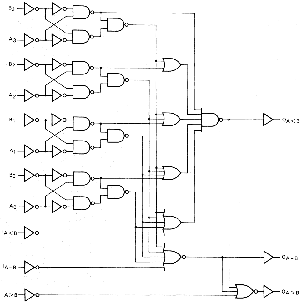
Fig. 3 Logic diagram.
