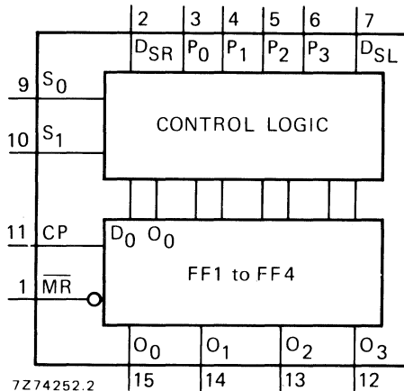
Fig. 1 Functional diagram.
