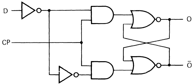
Fig. 6 Logic diagram (one latch); see also Fig. 5. 7Z79901
