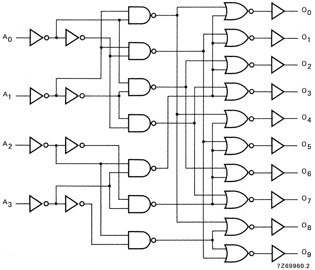
Fig. 3 Logic diagram.
