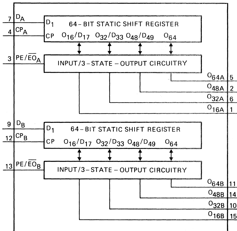
Fig. 1 Functional diagram.
