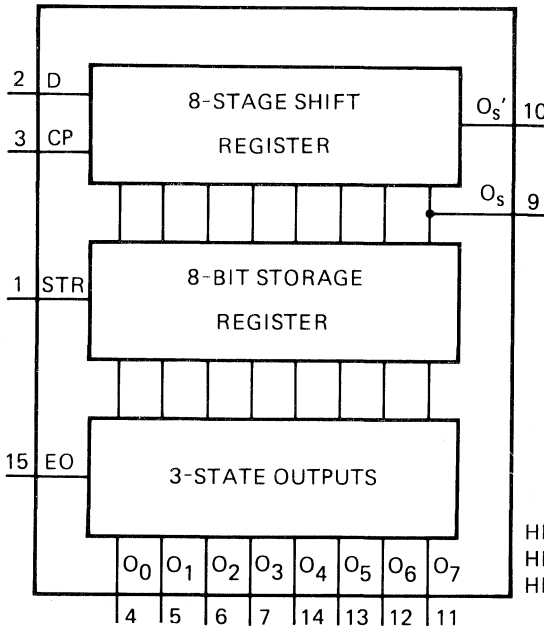
Fig. 1 Functional diagram.
