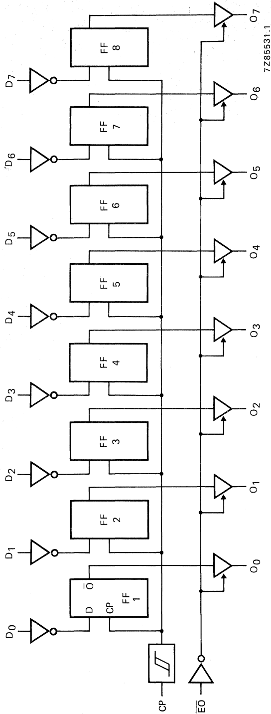
Fig. 3 Logic diagram.
