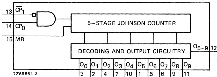
Fig. 1 Functional diagram.
