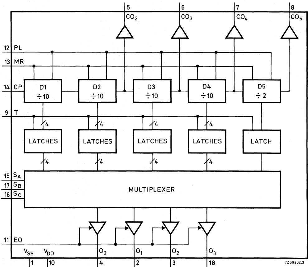
Fig. 2 Block diagram.
