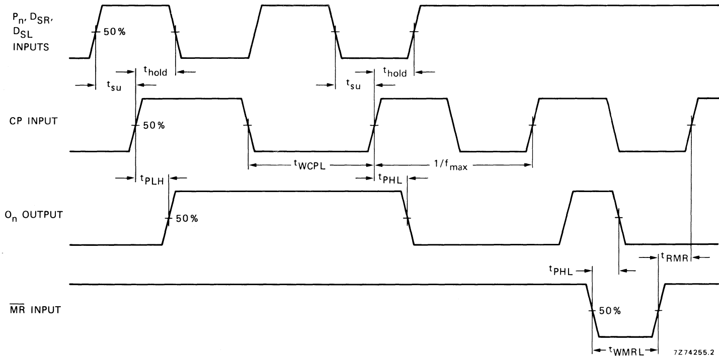
Fig. 4 Waveforms showing set-up times, hold times for D_{SR} , D_{SL} and P_n inputs; minimum \overline{MR} pulse width, \overline{MR} to output delays and \overline{MR} to CP recovery time; minimum CP pulse width and CP to output delays. Set-up and hold times are shown as positive values but may be specified as negative values.
