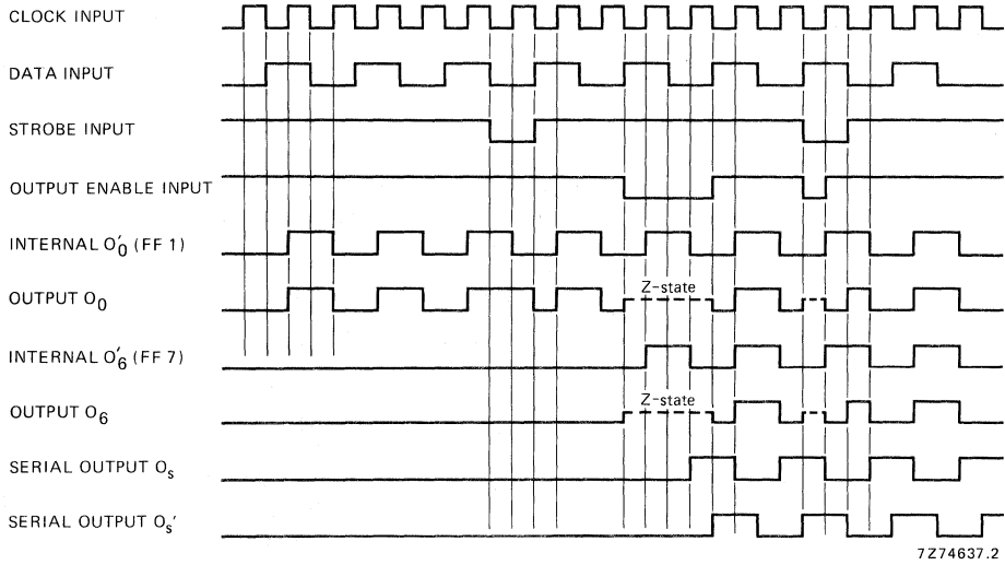
Fig. 4 Timing diagram.
