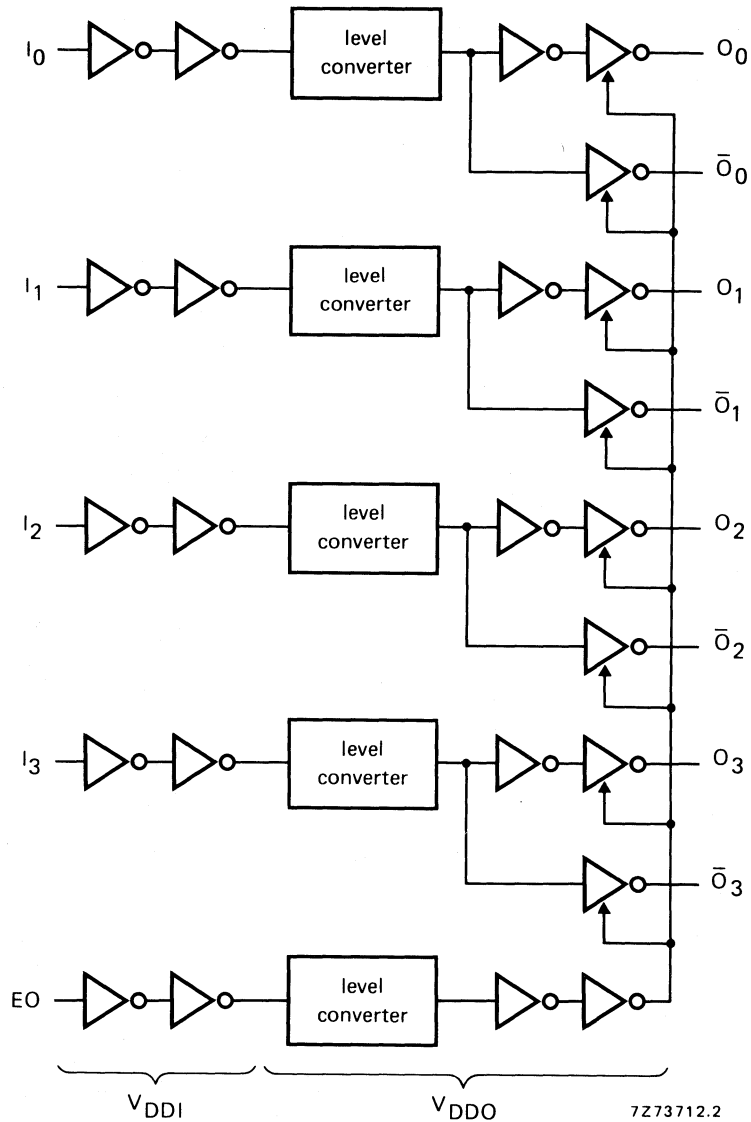
Fig. 3 Logic diagram.
