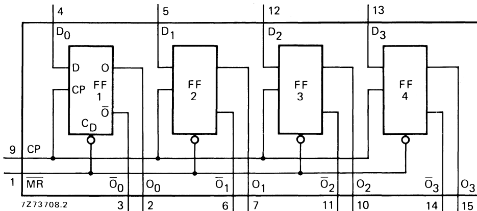
Fig. 1 Functional diagram.
