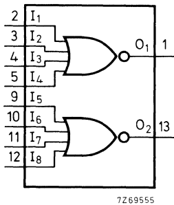
Fig. 1 Functional diagram.
