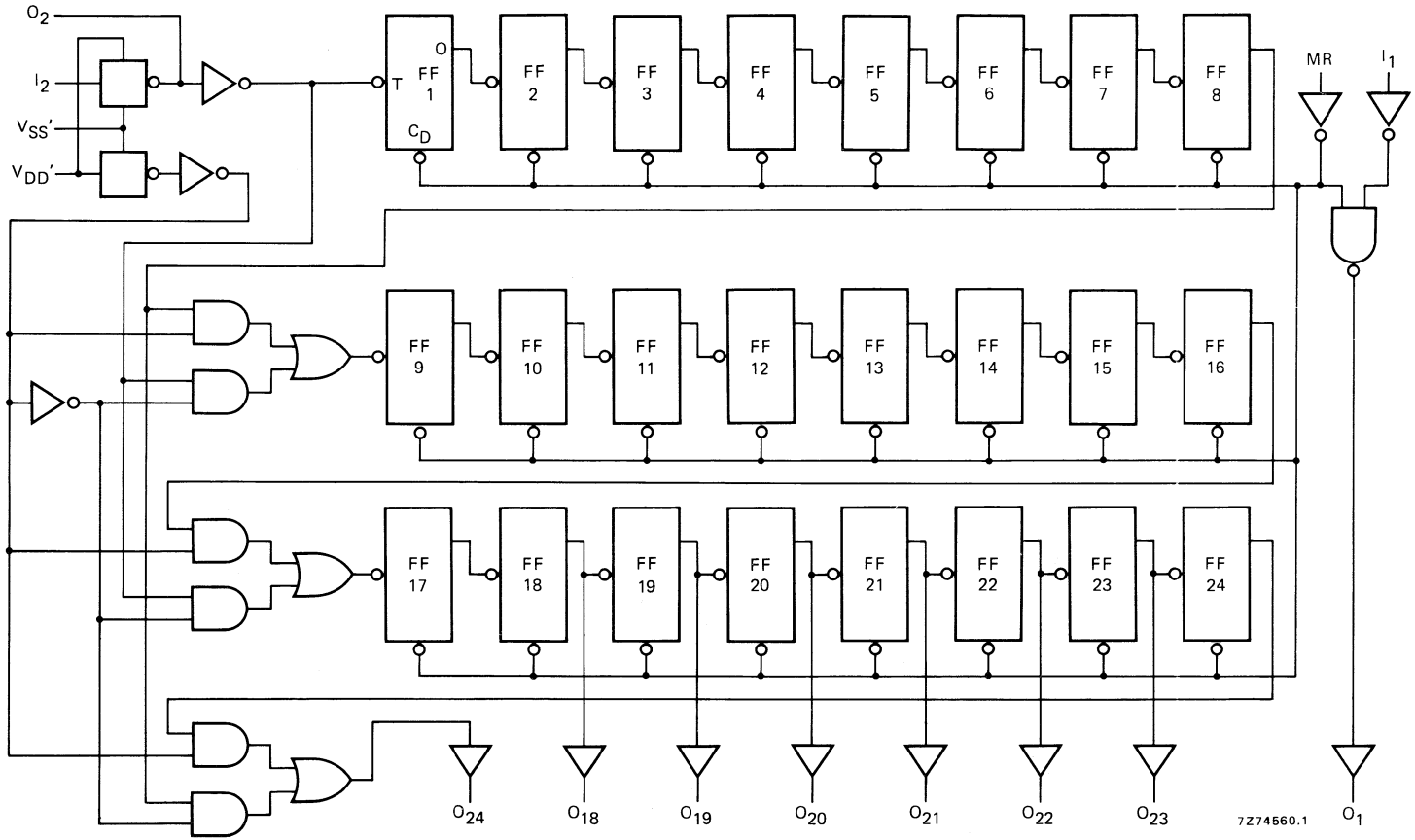
Fig. 3 Logic diagram; for schematic diagram of clock circuit see Fig. 4.
