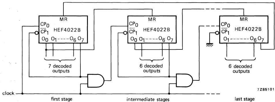
Fig. 7 Counter expansion.
