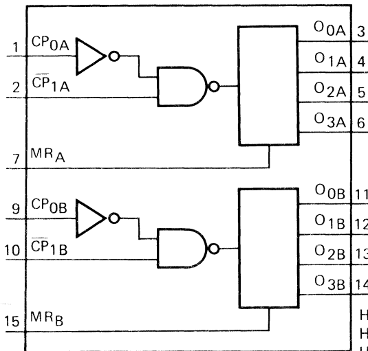
Fig. 1 Functional diagram.
