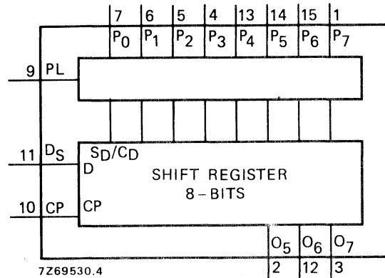
Fig. 1 Functional diagram.
