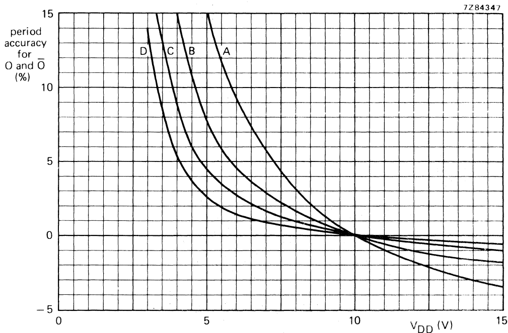
Fig. 6 Typical O and \bar{O} period accuracy as a function of supply voltage; astable mode; T_{amb} = 25^\circ\text{C} .
