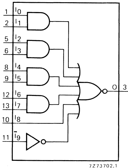
Fig. 1 Functional diagram.
