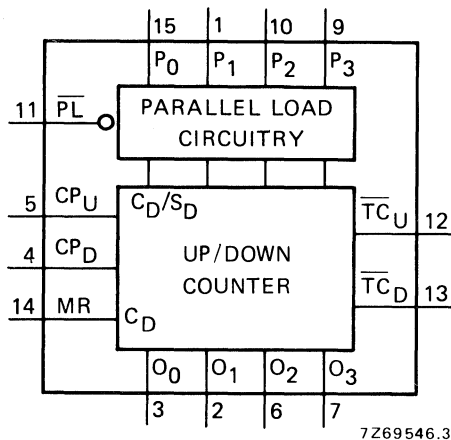
Fig. 1 Functional diagram.
