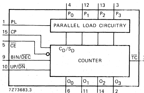
Fig. 1 Functional diagram.
