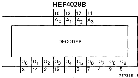
1-of-10 decoder.
