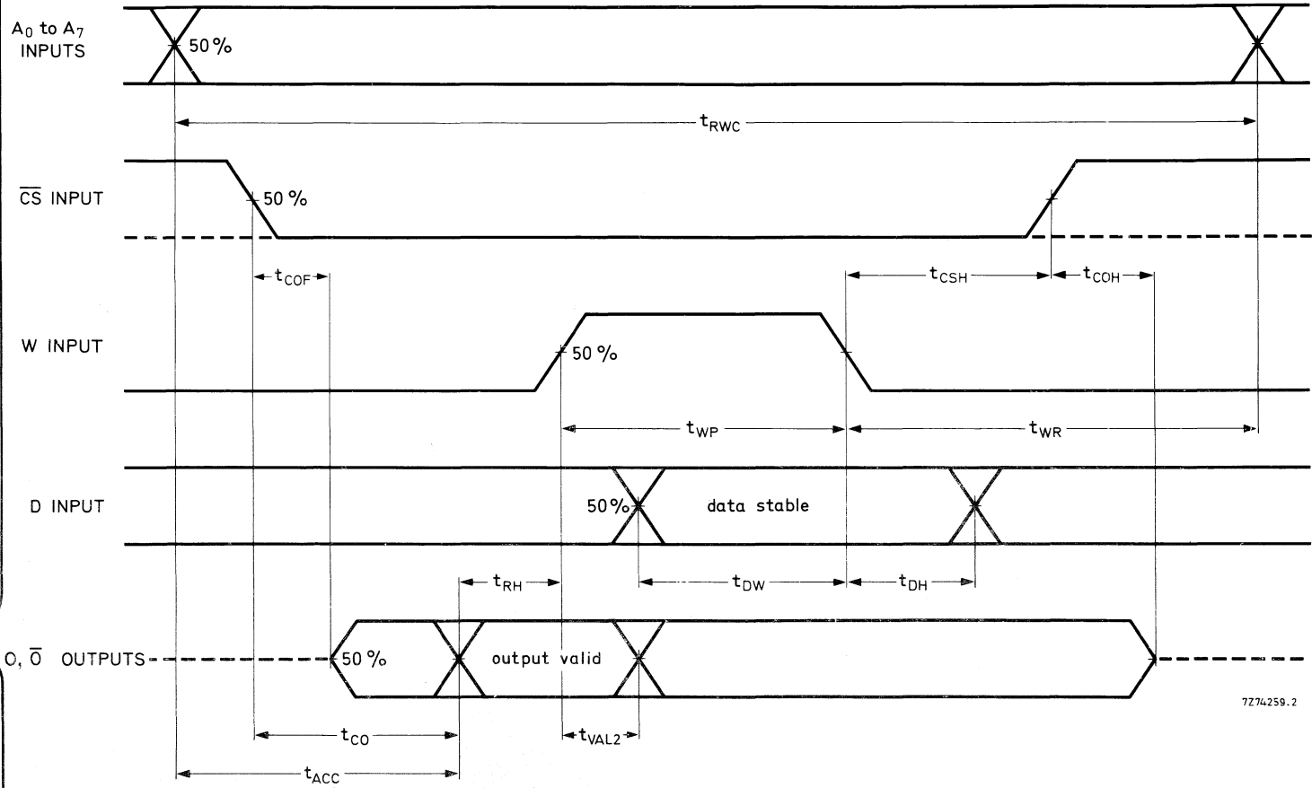
Fig. 5 Read-modify-write cycle timing diagram.
