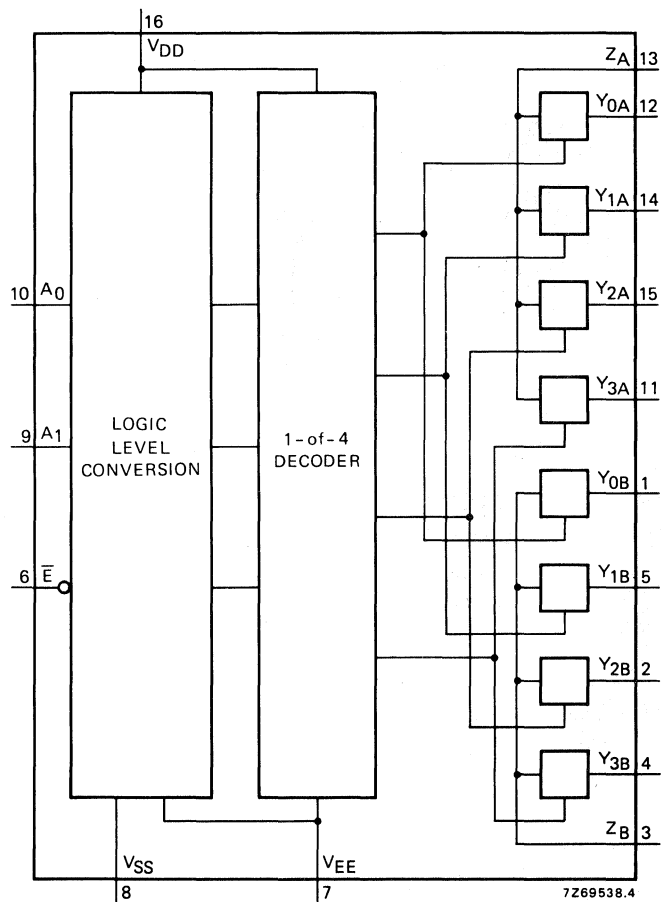
Fig. 1 Functional diagram.
