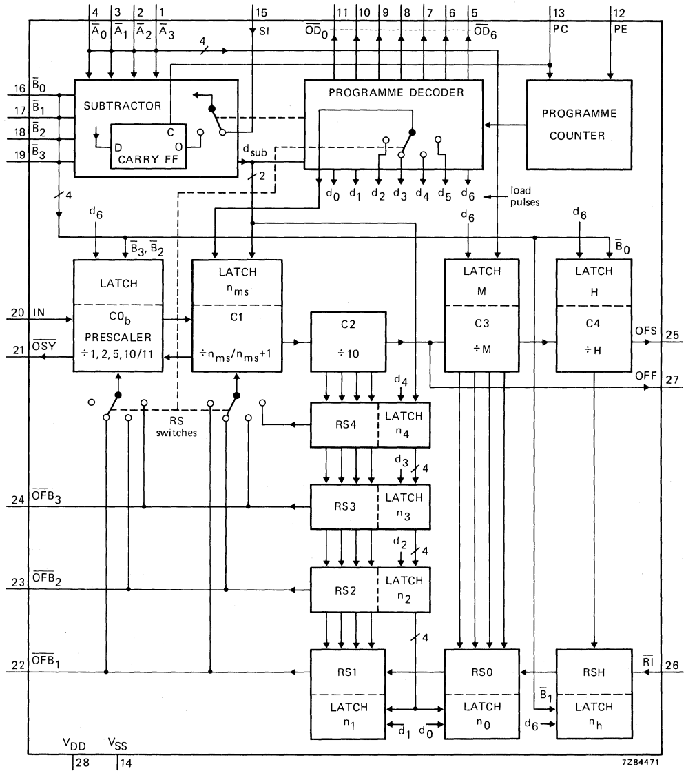
Fig. 2 Block diagram.
