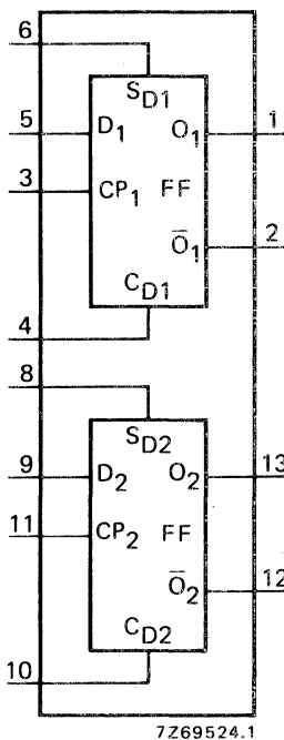
Fig. 1 Functional diagram.
