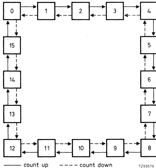
Fig. 4 State diagram.
