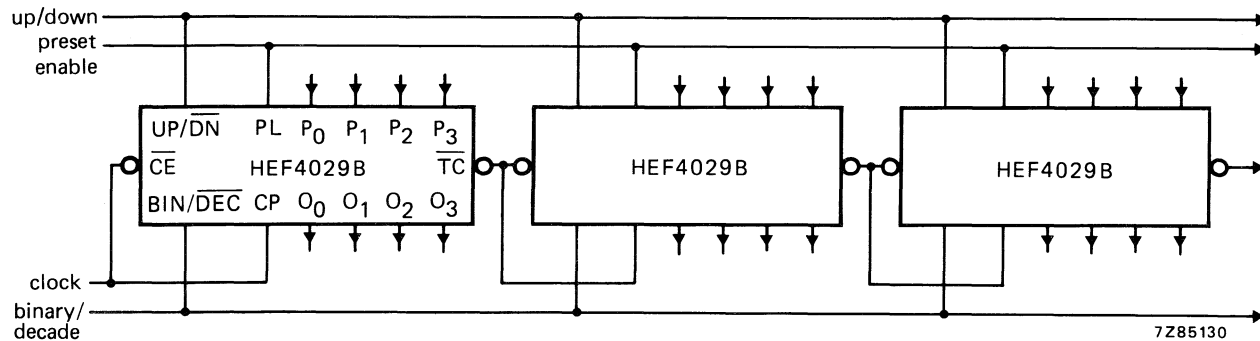
Fig. 11 Example of ripple clocking when cascading HEF4029B ICs. Ripple clocking mode: the up/down control can be changed at any count; the only restriction on changing the up/down control is that the clock input to the first counting stage must be HIGH.
