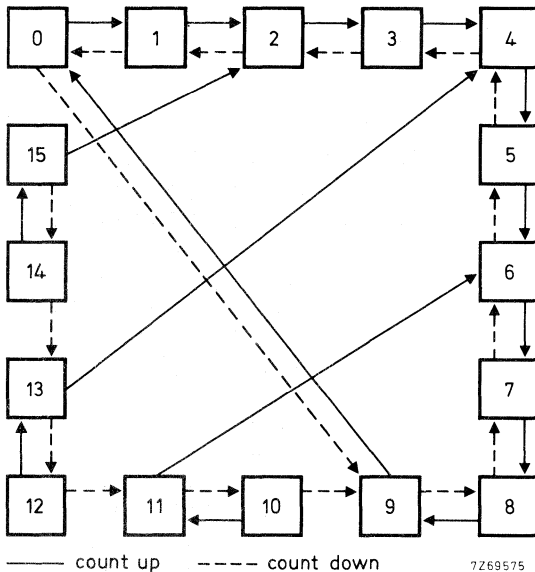
Fig. 4 State diagram.
