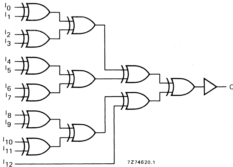
Fig. 3 Logic diagram.
