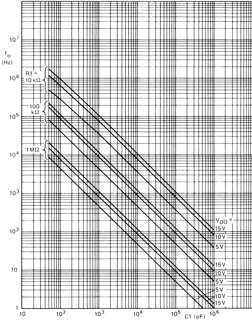
Fig. 7 Typical centre frequency as a function of capacitor C_1 ; T_{amb} = 25\text{ }^\circ\text{C} ; V_{CO\text{IN}} at \frac{1}{2} V_{DD} ; \text{INH} at V_{SS} ; R_2 = \infty .
