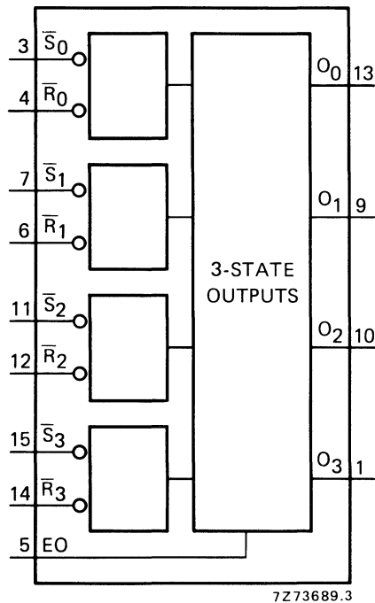
Fig. 1 Functional diagram.
