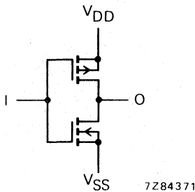
Fig. 3 Schematic diagram (one inverter).
