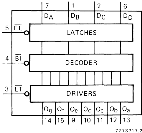
Fig. 1 Functional diagram.
