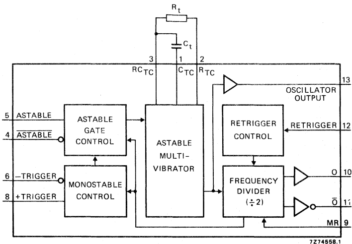
Monostable/astable multivibrator.
