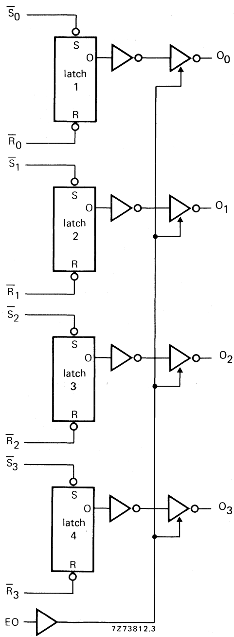
Fig. 3 Logic diagram.
