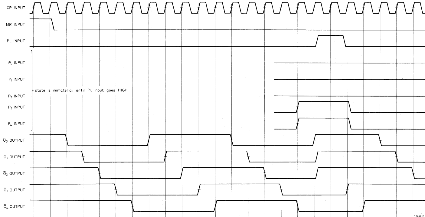
Fig. 7 Timing diagram.
