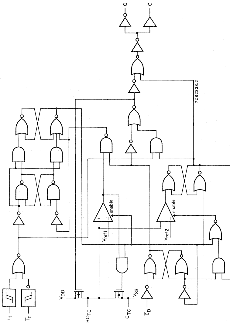
Fig. 3 Logic diagram.
