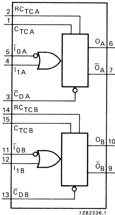
Fig. 1 Functional diagram.
