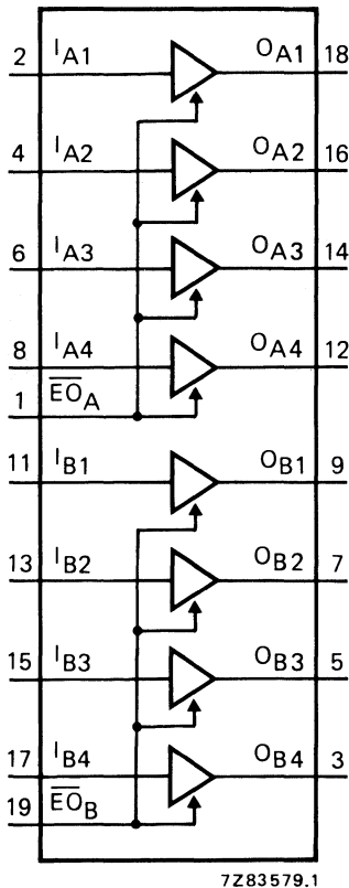
Fig. 1 Functional diagram.
