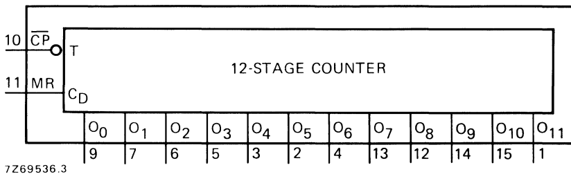
Fig. 1 Functional diagram.
