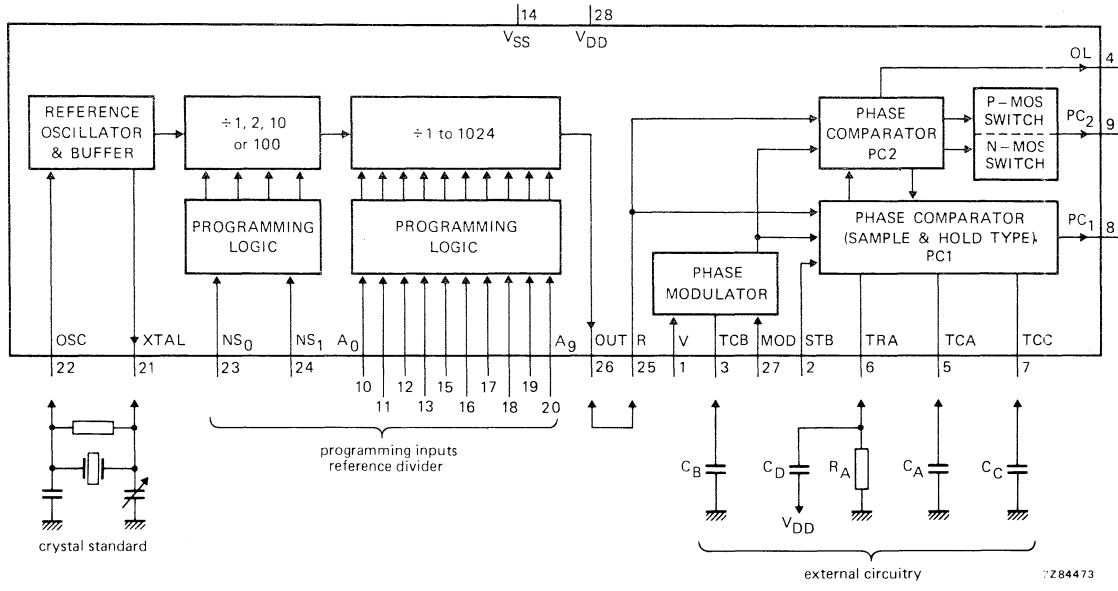
Frequency synthesizer.
