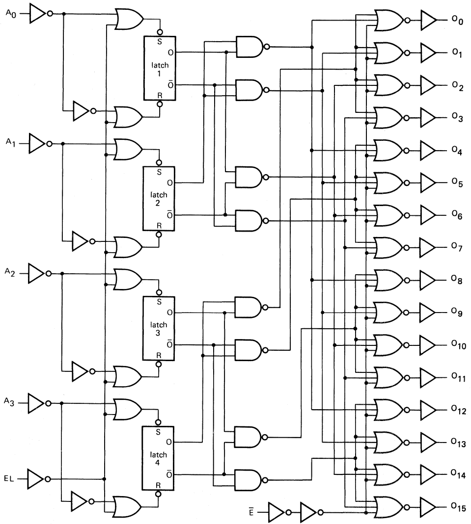
Fig. 3 Logic diagram.
