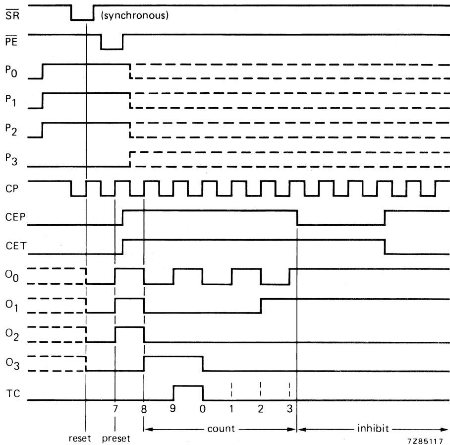
Fig. 9 Timing diagram.
