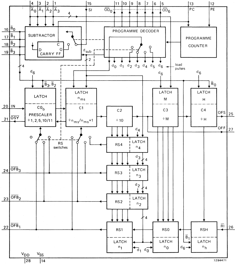
Universal divider.
