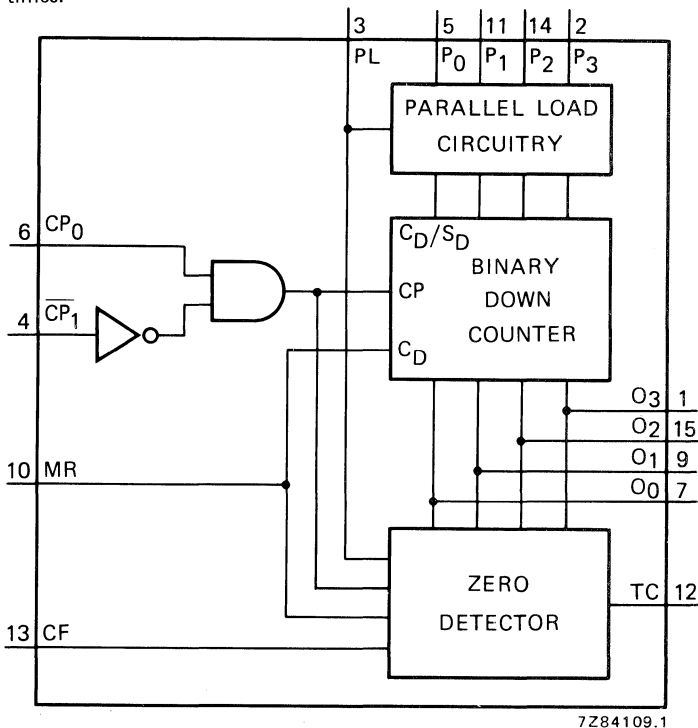
Fig. 1 Functional diagram.
