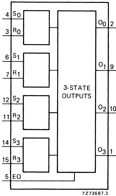
Fig. 1 Functional diagram.
