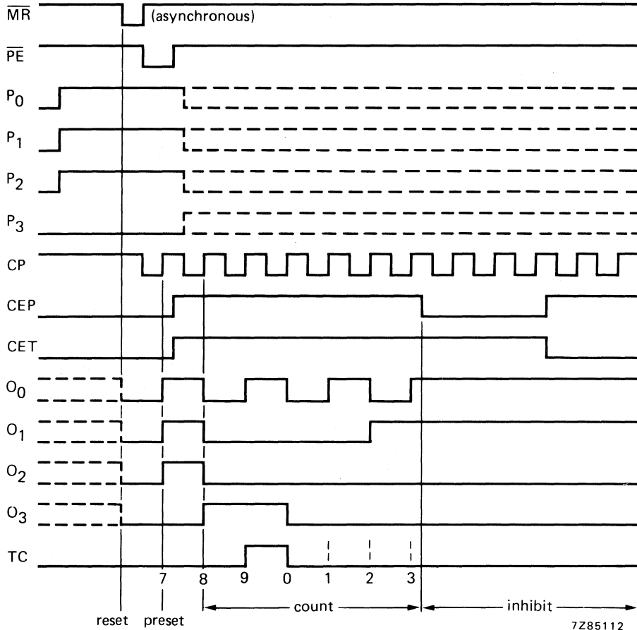
Fig. 9 Timing diagram.
