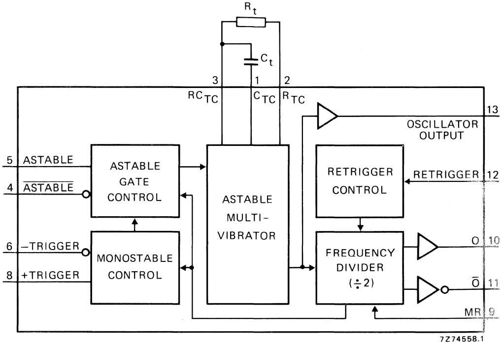
Fig. 1 Functional diagram.
