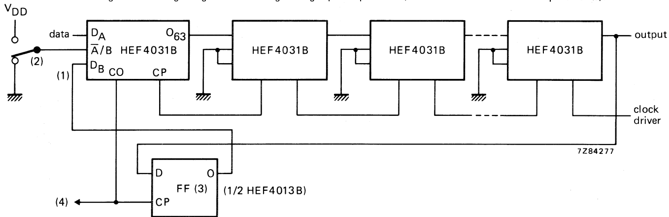
Fig. 5 Cascading using direct clocking for high speed operation (see clock rise and fall time requirements).
