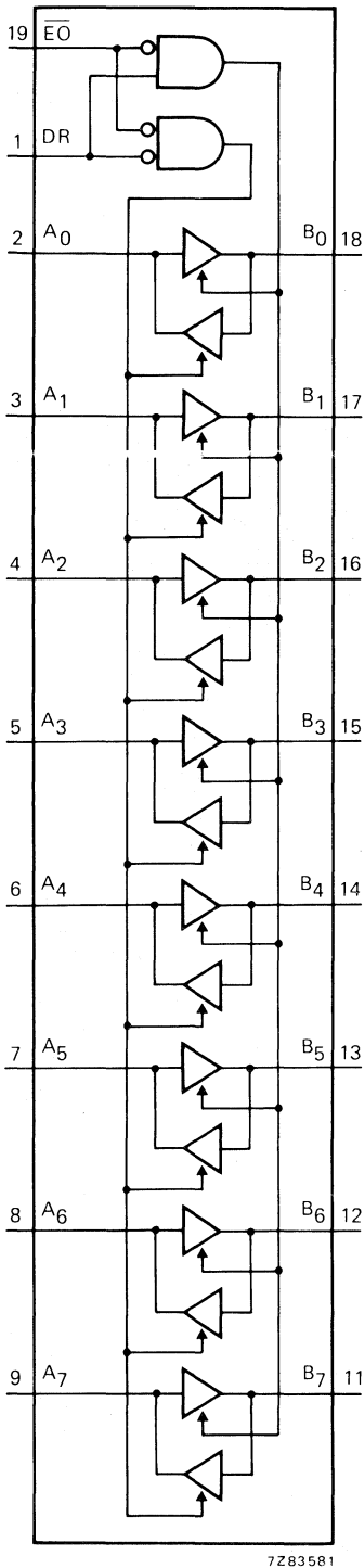
Fig. 3 Functional diagram.
