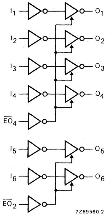
Fig. 3 Logic diagram.
