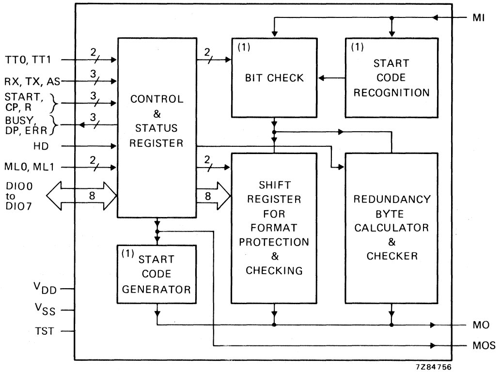
Fig. 2 Block diagram.
