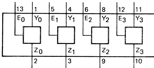
Fig. 1 Functional diagram.
