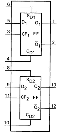
Dual D-type flip-flop.
