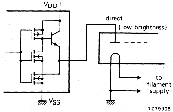
Fig. 12 Connection to fluorescent display readout.
