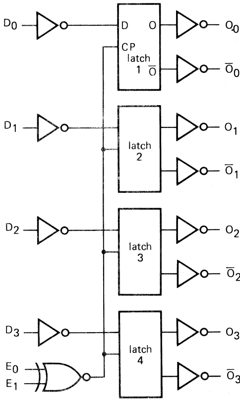
Fig. 3 Logic diagram.
