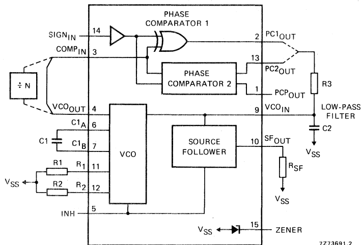
Phase-locked loop.
