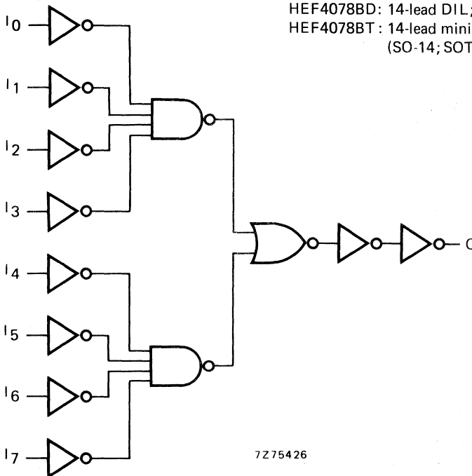
Fig. 3 Logic diagram.
