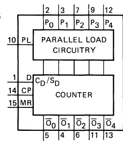
Presetable divide-by-n counter.
