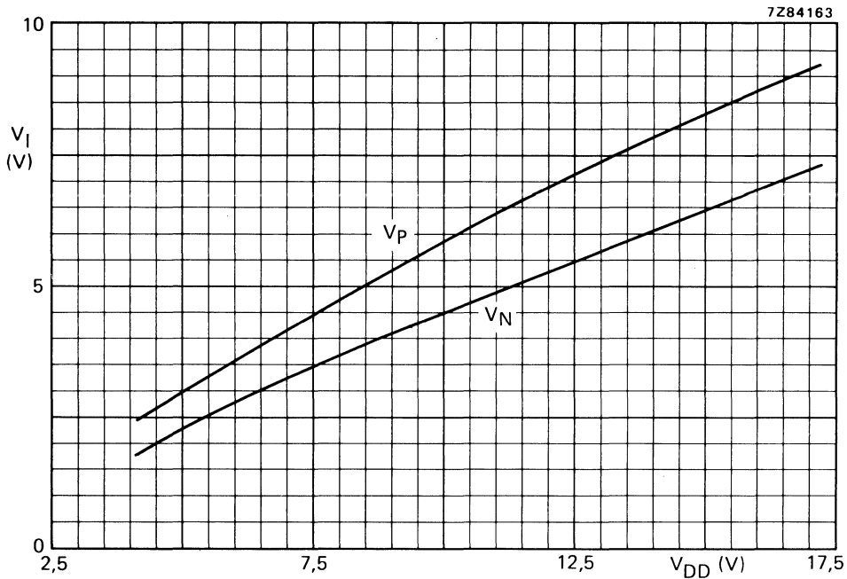
Fig. 9 Typical switching levels as a function of supply voltage V_{DD} ; T_{amb} = 25^\circ C .
