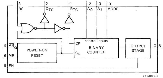
Programmable timer.
