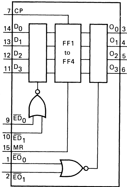
Fig. 1 Functional diagram.
