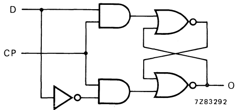
Fig. 3b One D-latch.
