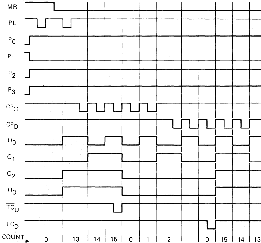
Fig. 6 Timing diagram.
