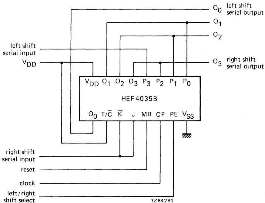
Fig. 6 Shift-left/shift-right register.
