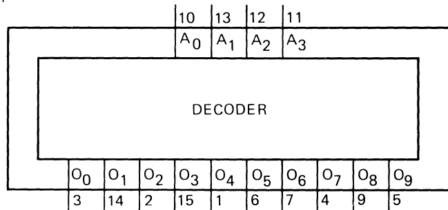
Fig.1 Functional diagram.
