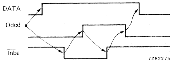
Fig. 4 Waveforms showing data exchange in talker function.
