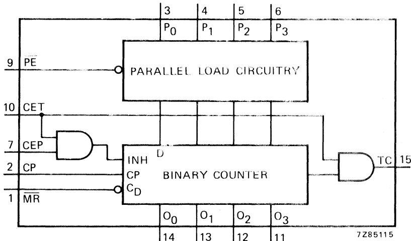
Fig. 1 Functional diagram.
