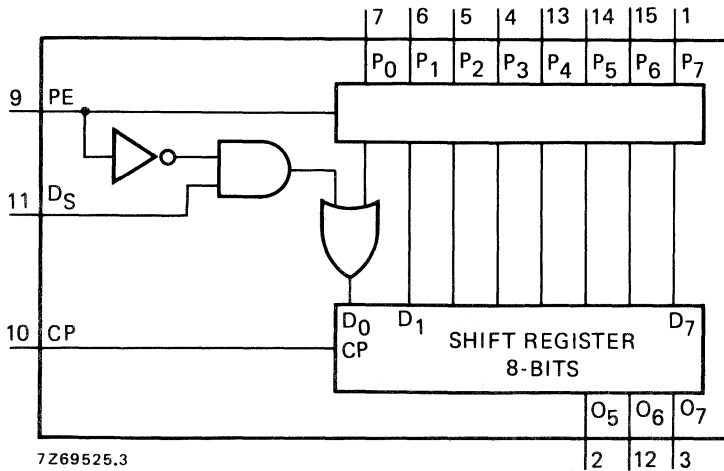
Fig. 1 Functional diagram.
