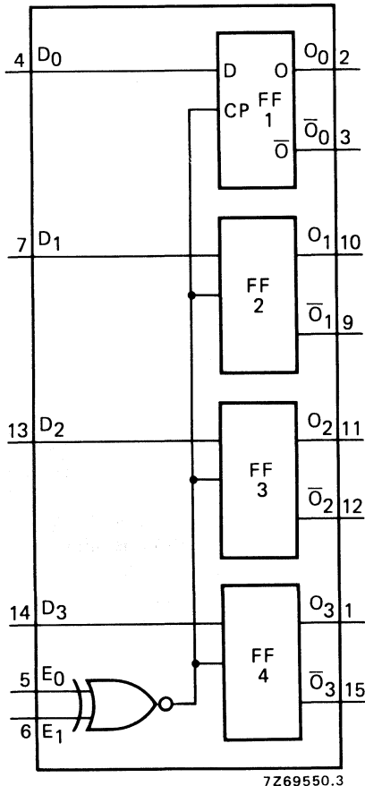
Fig. 1 Functional diagram.
