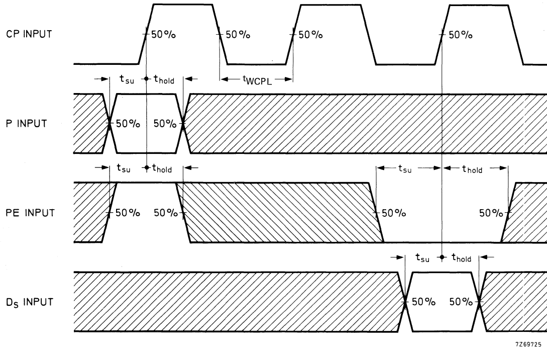
Fig. 4 Waveforms showing minimum clock pulse width, and set-up and hold times for PE to CP, D S to CP, and P to CP. Set-up and hold times are shown as positive values but may be specified as negative values.
