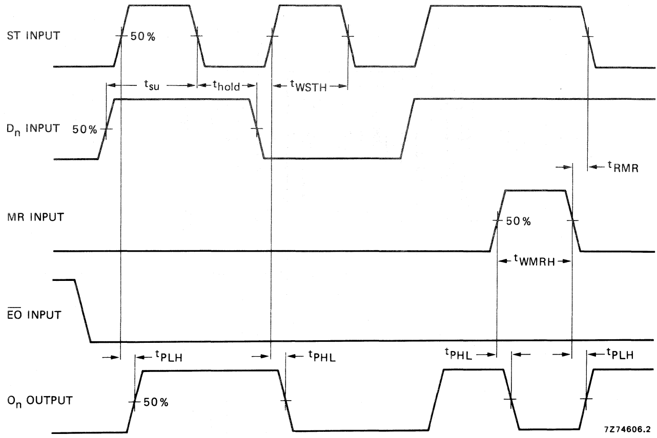
Fig. 4 Waveforms showing minimum ST and MR pulse widths, set-up and hold times for D n to ST, recovery time for MR and propagation delays from ST to O n , D n to O n and MR to O n .
