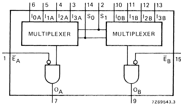
Fig. 1 Functional diagram.
