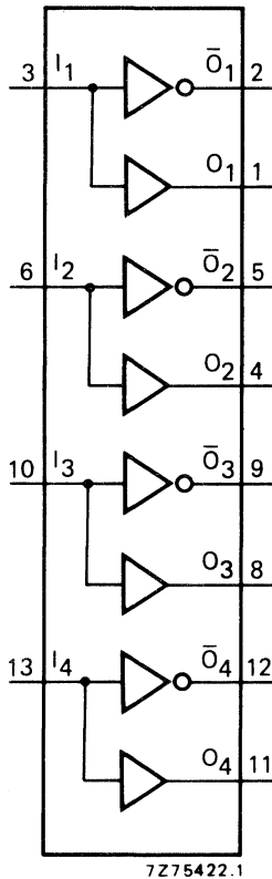
Fig. 1 Functional diagram.
