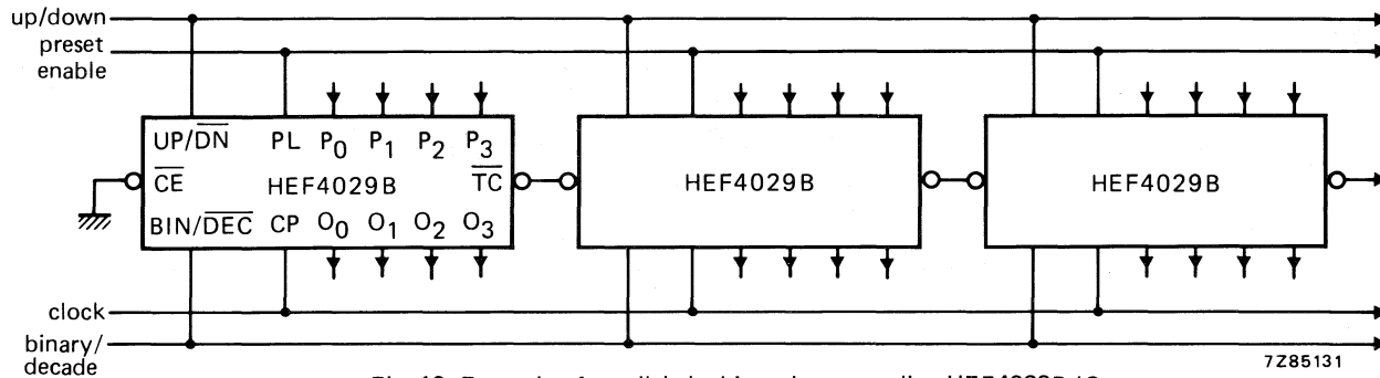
Fig. 10 Example of parallel clocking when cascading HEF4029B ICs.
