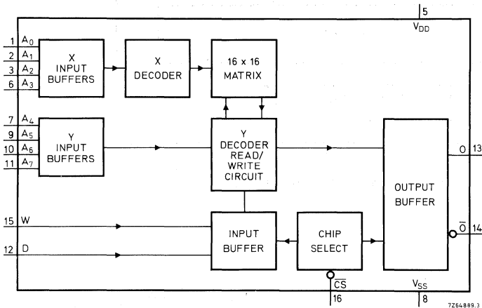
256-bit, 1-bit per word RAM.
