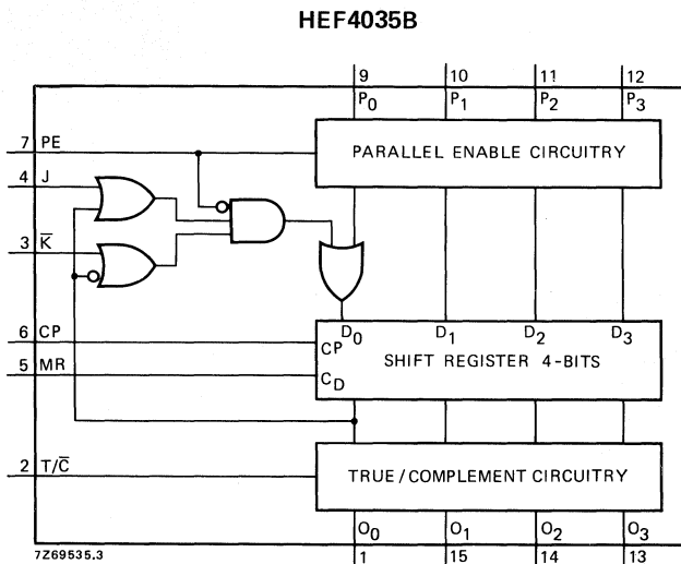
4-bit universal shift register.
