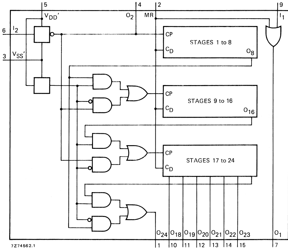
Fig. 1 Functional diagram.
