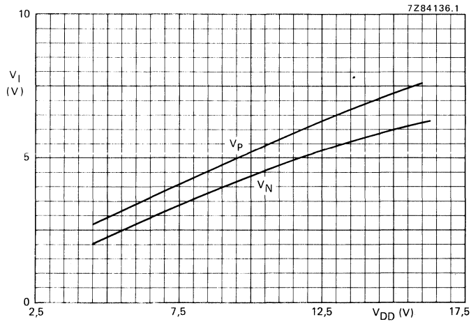
Fig. 9 Typical switching levels as a function of supply voltage V_{DD} ; T_{amb} = 25^\circ\text{C} .
