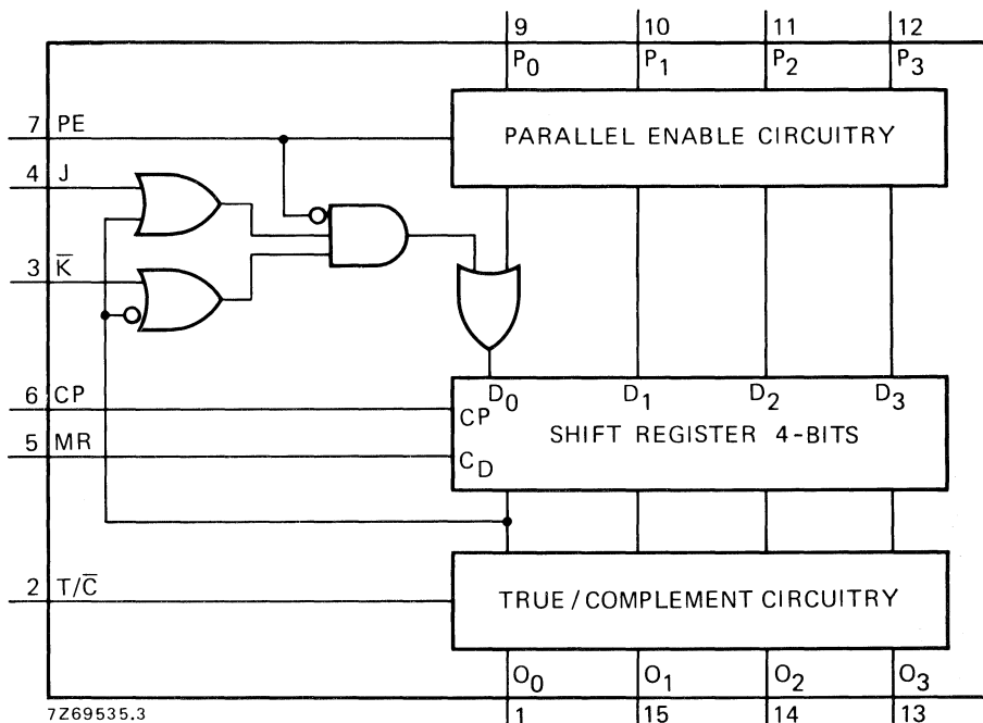
Fig. 1 Functional diagram.
