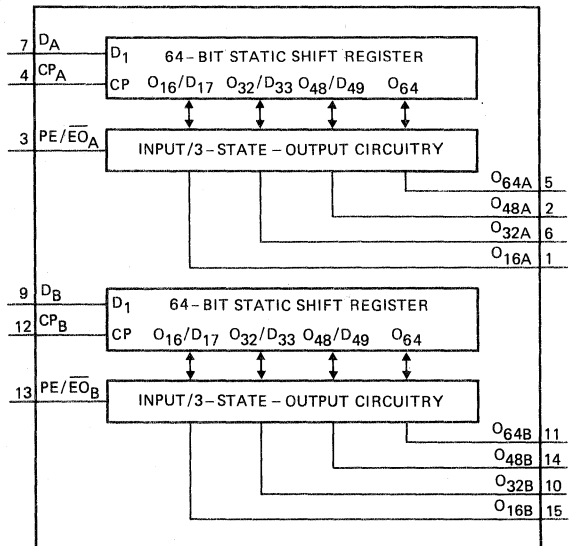
Dual 64-bit static shift register.
