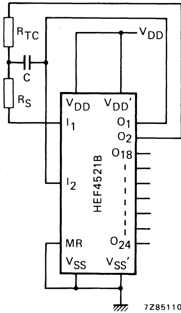
Fig. 7 RC oscillator circuit;
