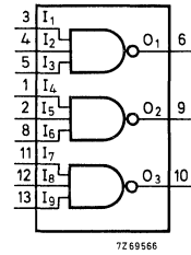
Triple 3-input NAND gate.
