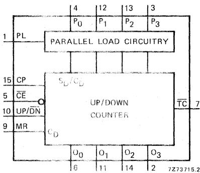
Binary up/down counter.
