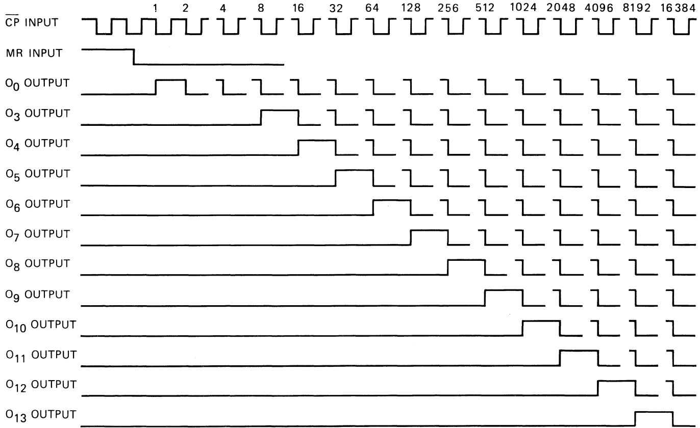
Fig. 5 Timing diagram.
