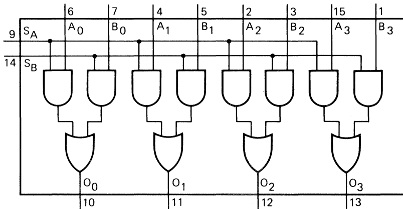
Fig. 1 Functional diagram.
