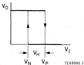
Fig. 4 Transfer characteristic.
