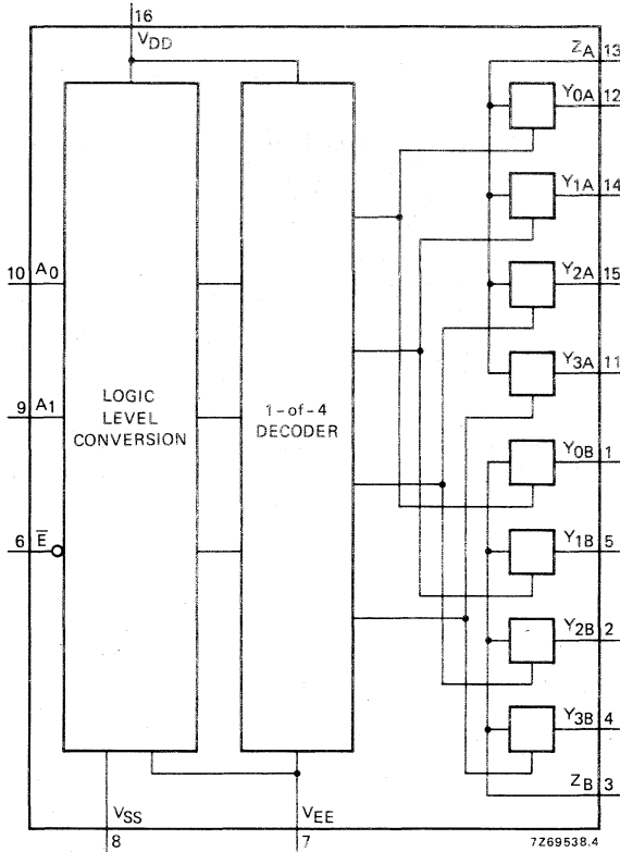
Dual 4-channel analogue multiplexer/demultiplexer.
