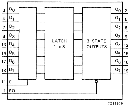
Fig. 1 Functional diagram.
