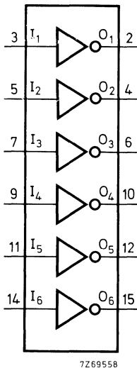
Fig. 1 Functional diagram.
