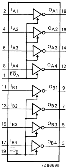
Fig. 1 Functional diagram.
