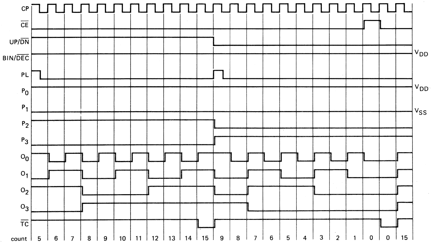
Fig. 9 Timing diagram; binary mode; P 0 = HIGH; P 1 = LOW; BIN/ \overline{DEC} = HIGH.
