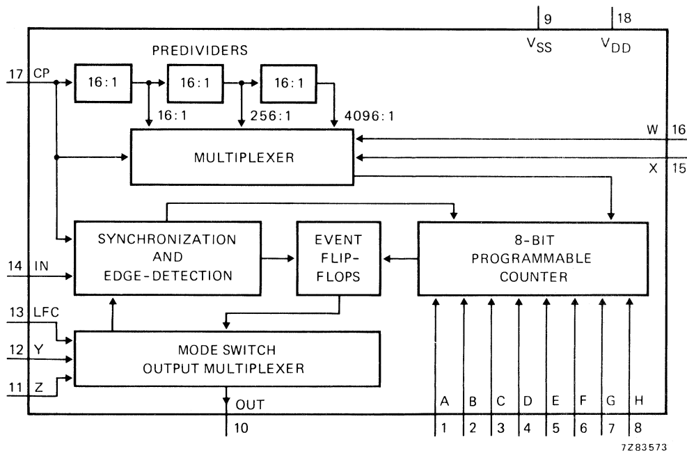
Fig. 1 Functional diagram.
