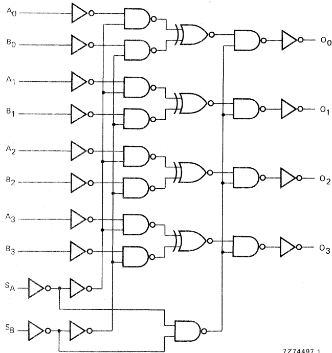
Fig. 3 Logic diagram.
