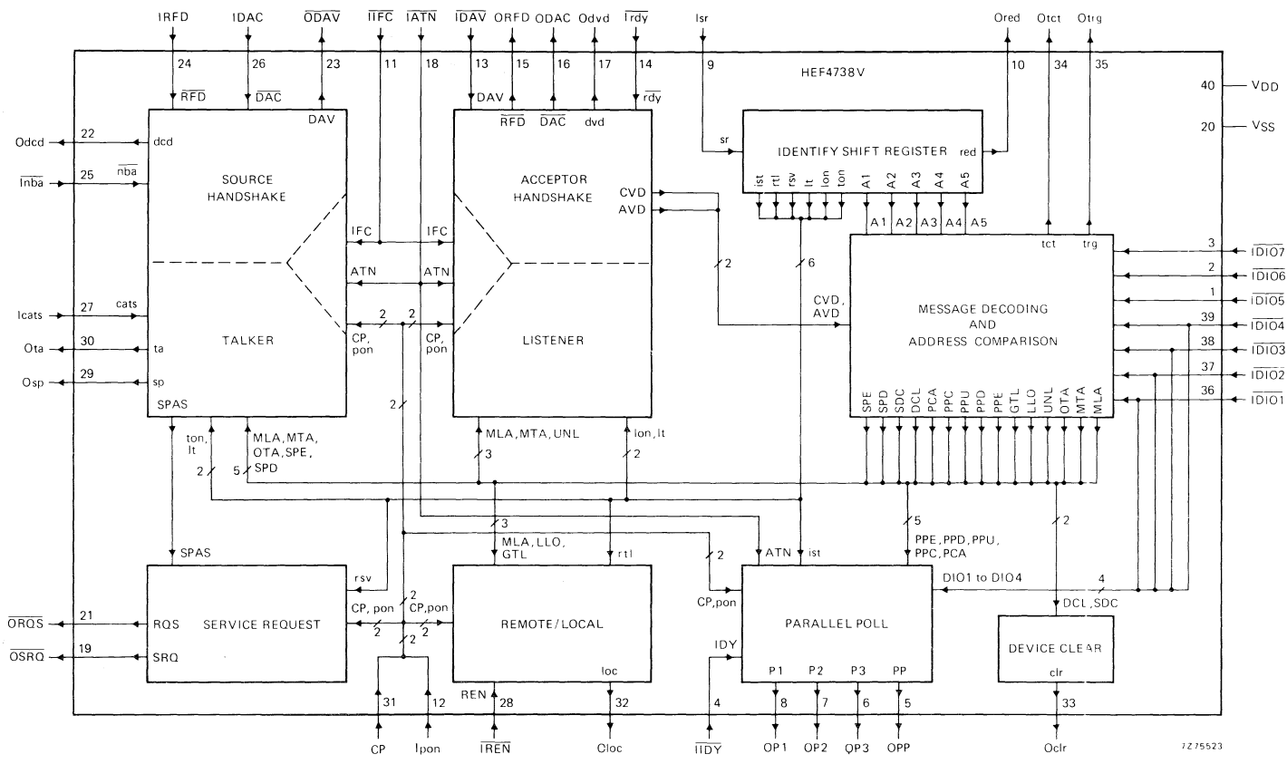
Fig. 3 Block diagram.
