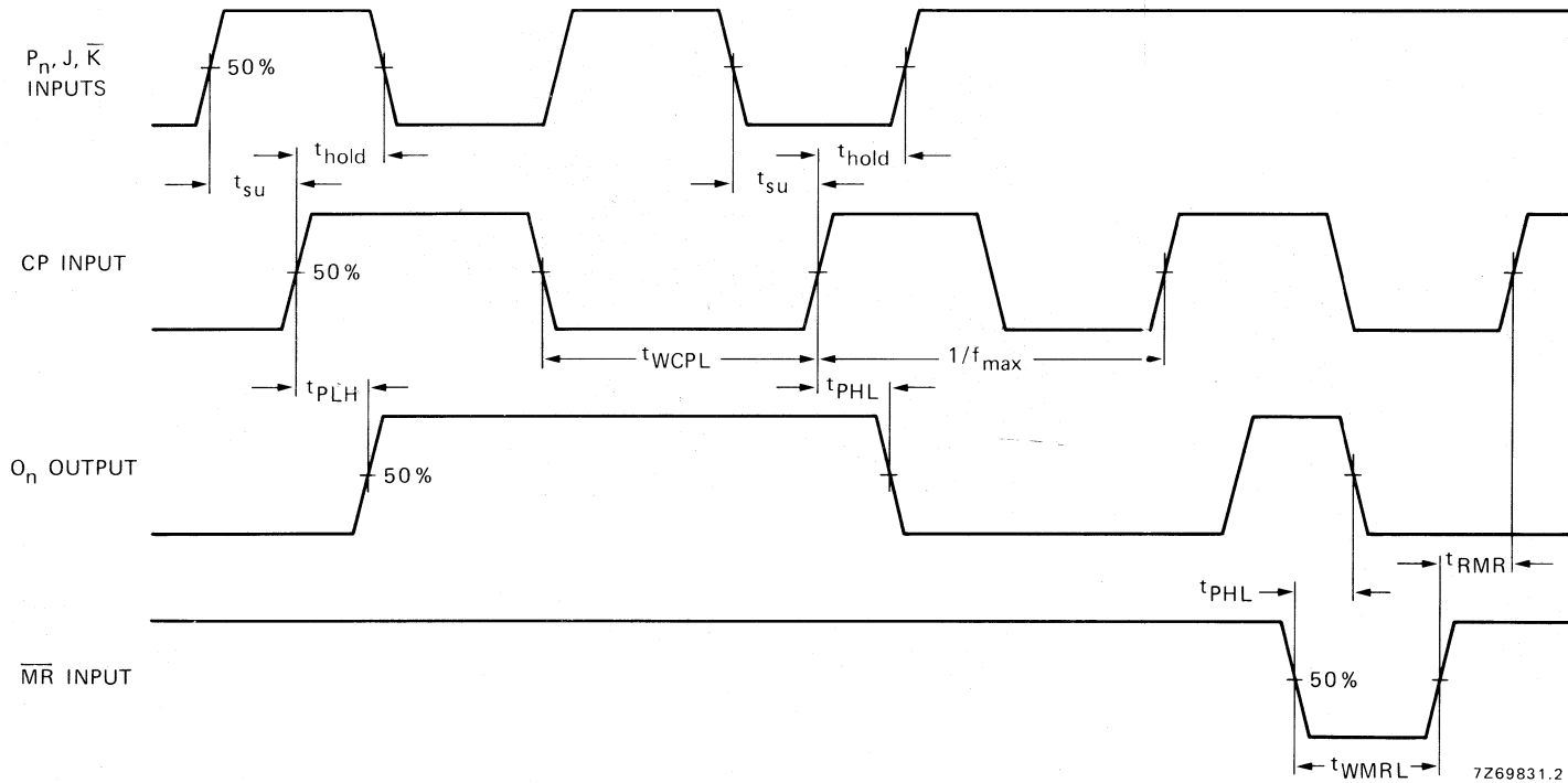
Fig. 4 Waveforms showing set-up times, hold times for J , \bar{K} and P_n inputs; minimum \bar{MR} pulse width, \bar{MR} to output delays and \bar{MR} to CP recovery time; minimum CP pulse width and CP to output delays. Set-up and hold times are shown as positive values but may be specified as negative values.
