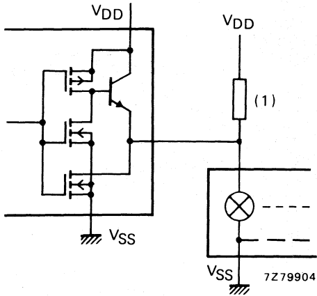
(1) A filament pre-warm resistor is recommended to reduce filament thermal shock and increase the effective cold resistance of the filament. Fig. 11 Connection to incandescent display readout.
