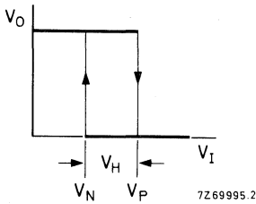
Fig. 4 Transfer characteristic.
