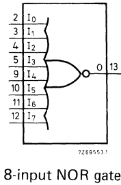
8-input NOR gate.
