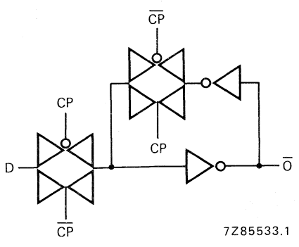
Fig. 4 Logic diagram (one latch).
