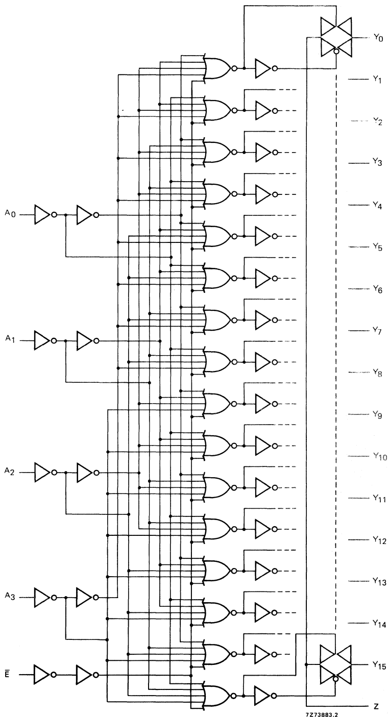
Fig. 4 Logic diagram.
