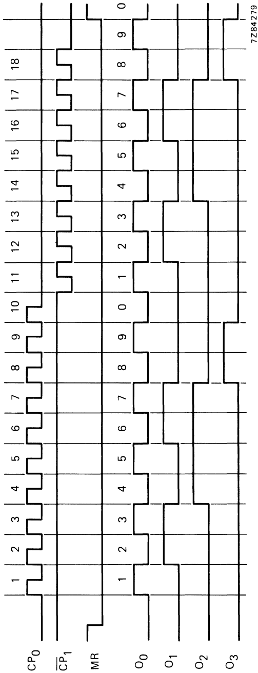
Fig. 6 Timing diagram.
