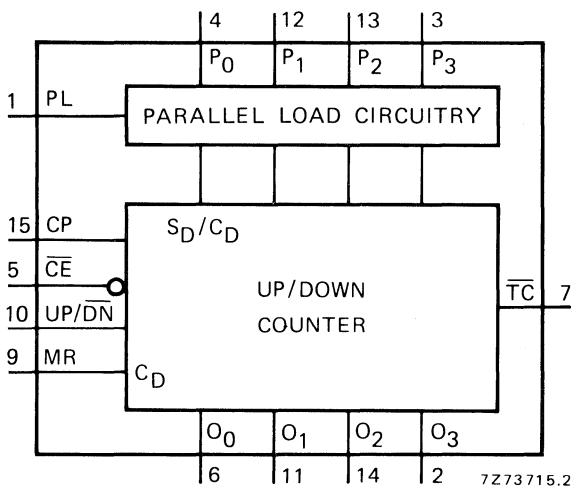
Fig. 1 Functional diagram.
