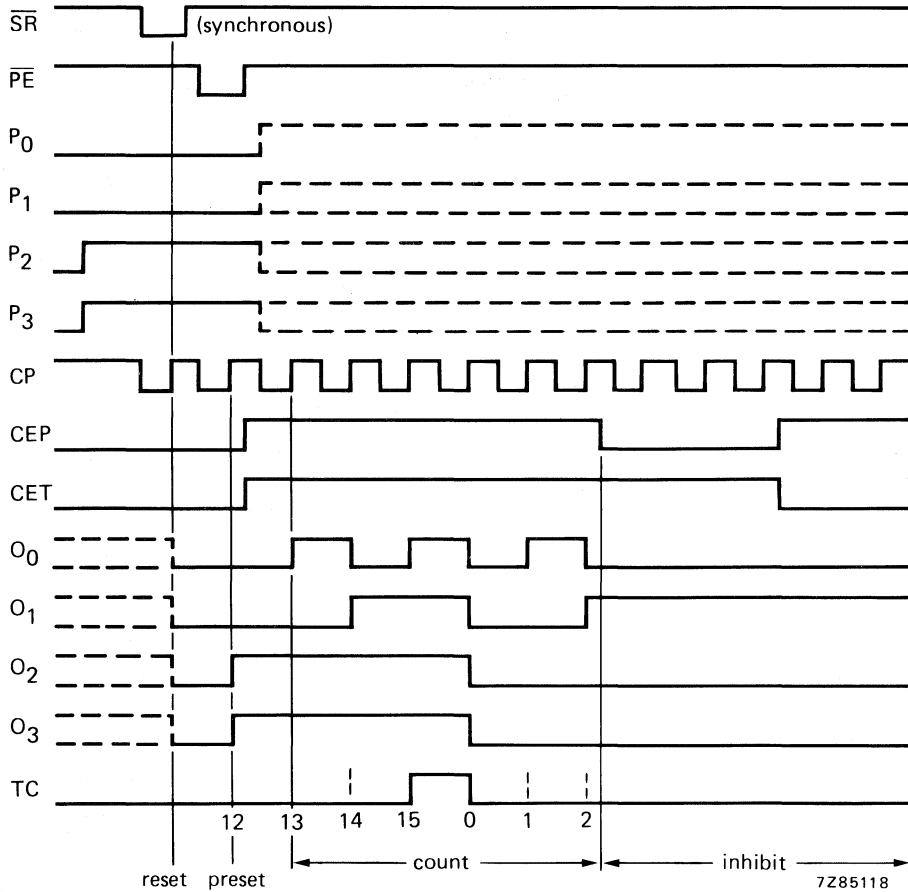
Fig. 9 Timing diagram.
