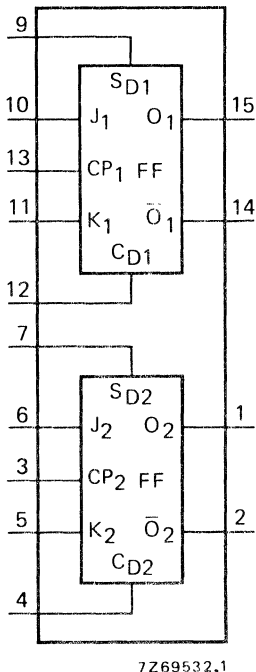
Fig. 1 Functional diagram.
