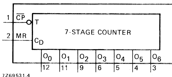
Fig. 1 Functional diagram.
