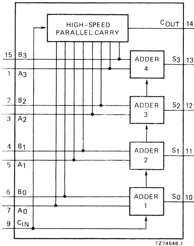
Fig. 1 Functional diagram.
