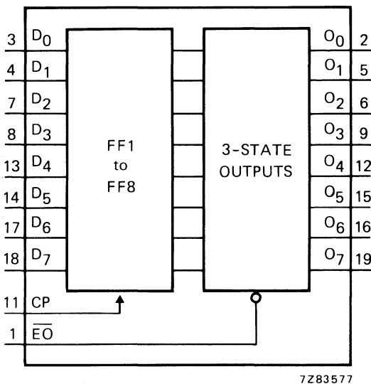
Fig. 1 Functional diagram.
