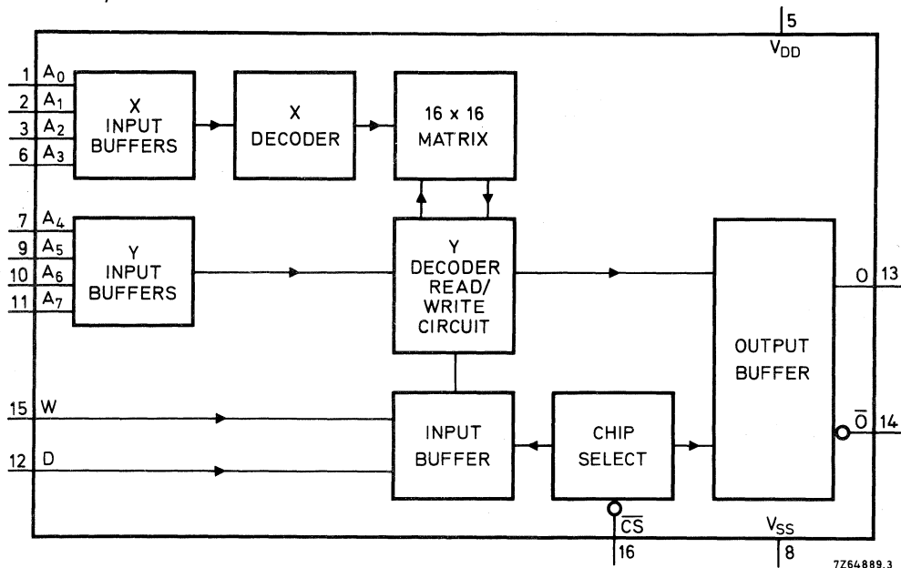
Fig. 1 Functional diagram.
