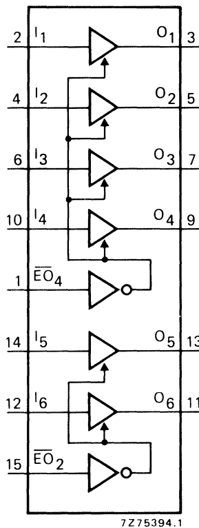
Fig. 1 Functional diagram.
