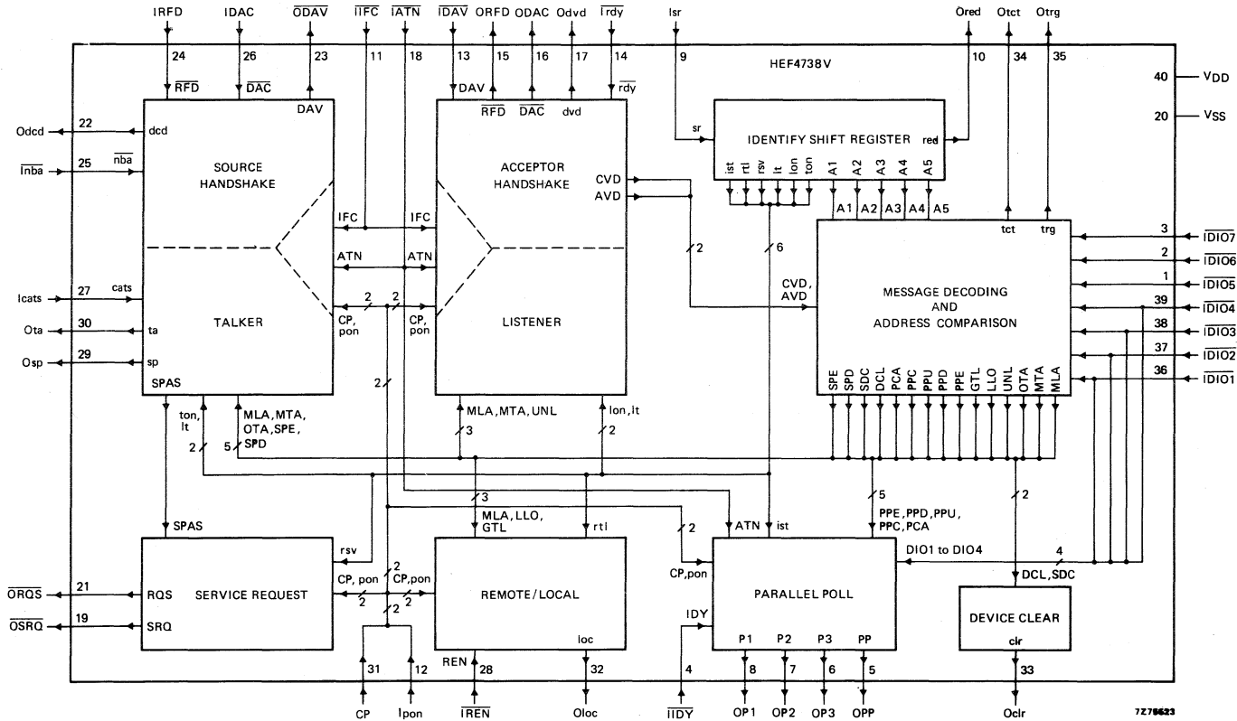
IEC/IEEE bus interface.
