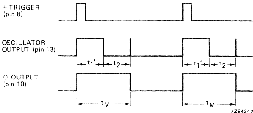
Fig. 7 Monostable waveforms.
