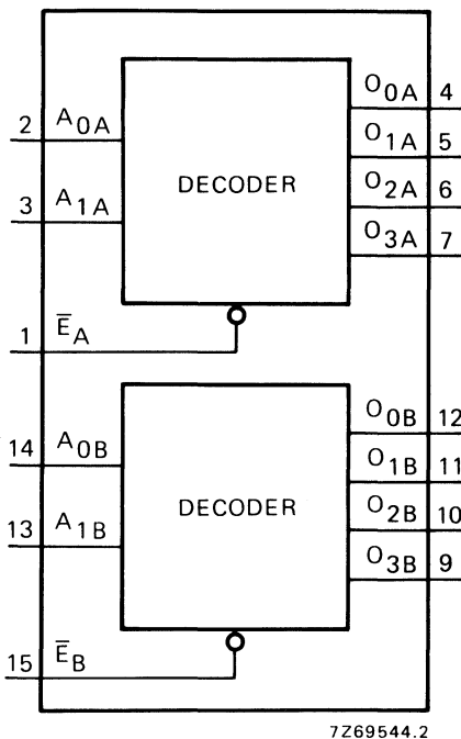
Fig. 1 Functional diagram.
