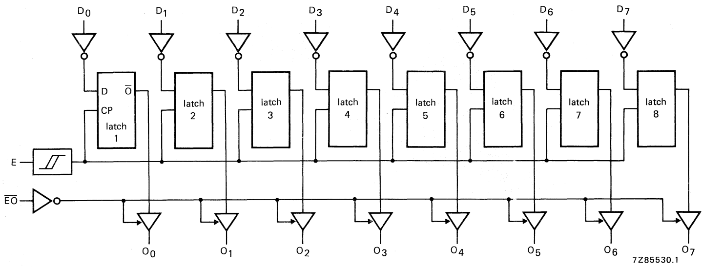
Fig. 3 Logic diagram.
