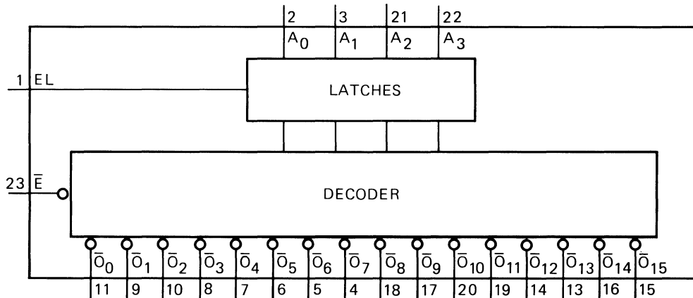
Fig. 1 Functional diagram.
