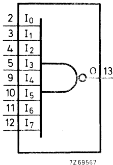
Fig. 1 Functional diagram.
