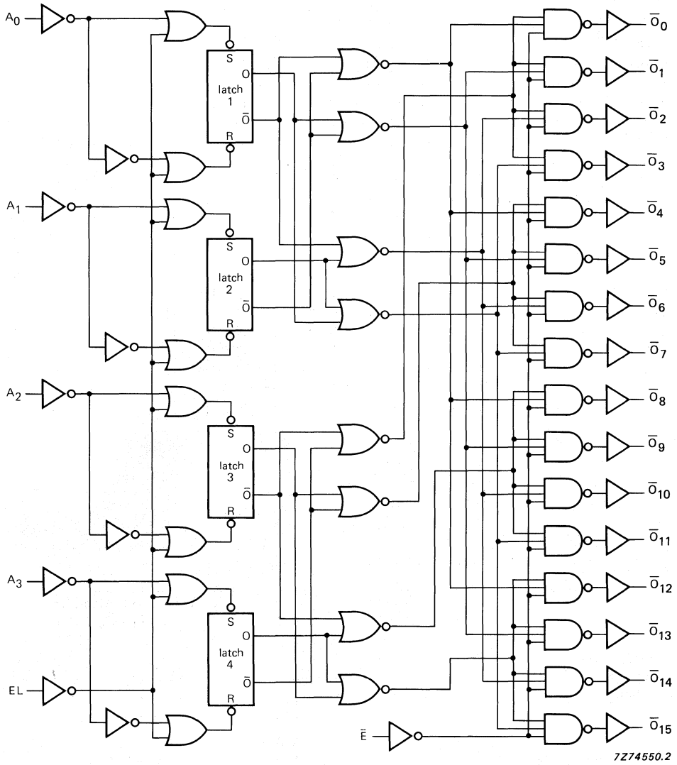
Fig. 3 Logic diagram.
