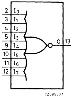
Fig. 1 Functional diagram.
