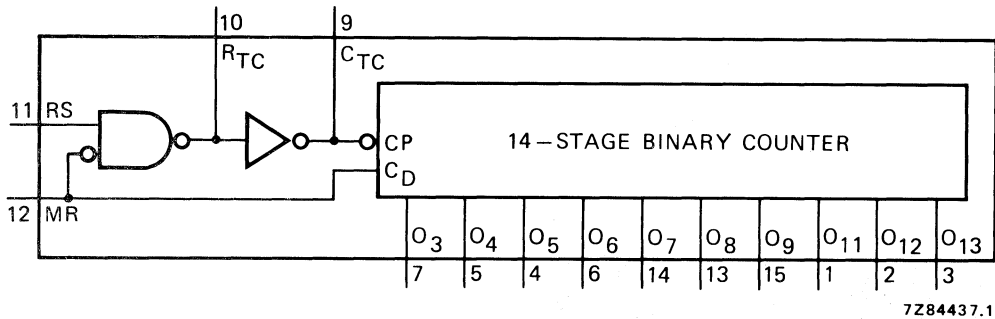
Fig. 1 Functional diagram.
