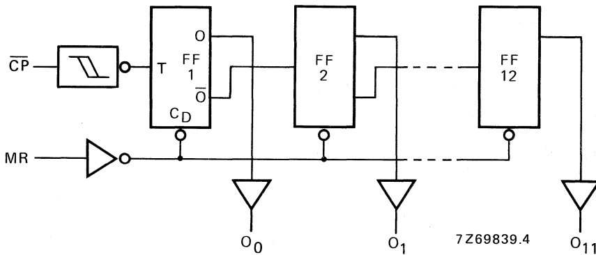
Fig. 3 Logic diagram.
