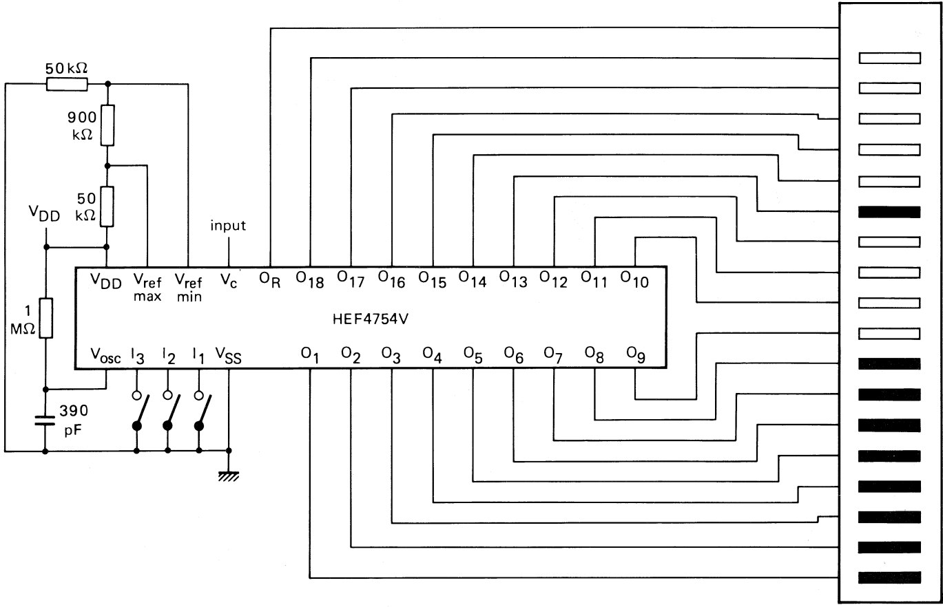
Fig. 3 Typical operating set-up.
