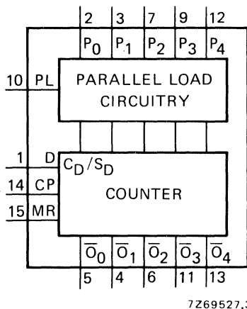
Fig. 1 Functional diagram.
