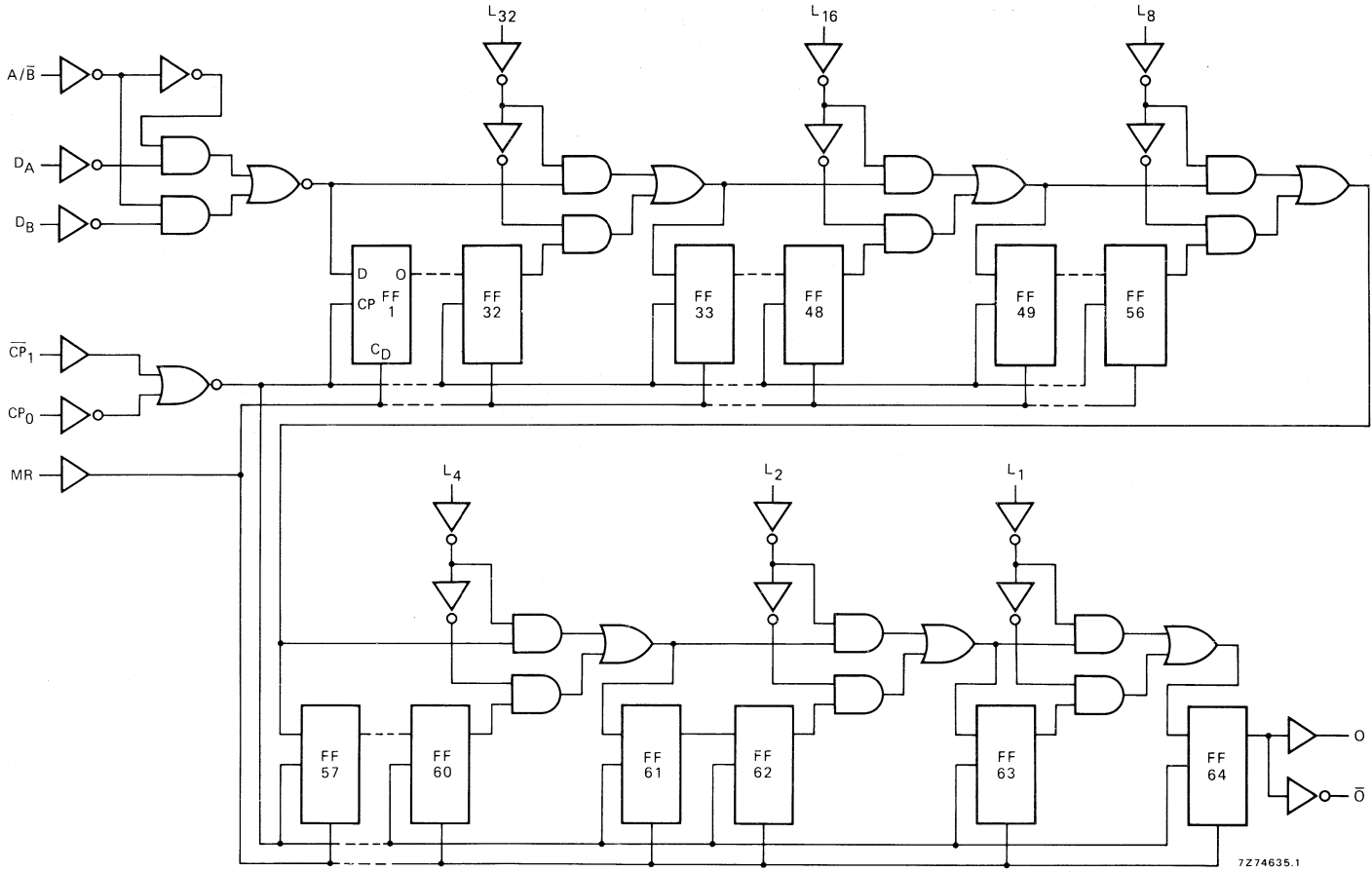
Fig. 3 Logic diagram.
