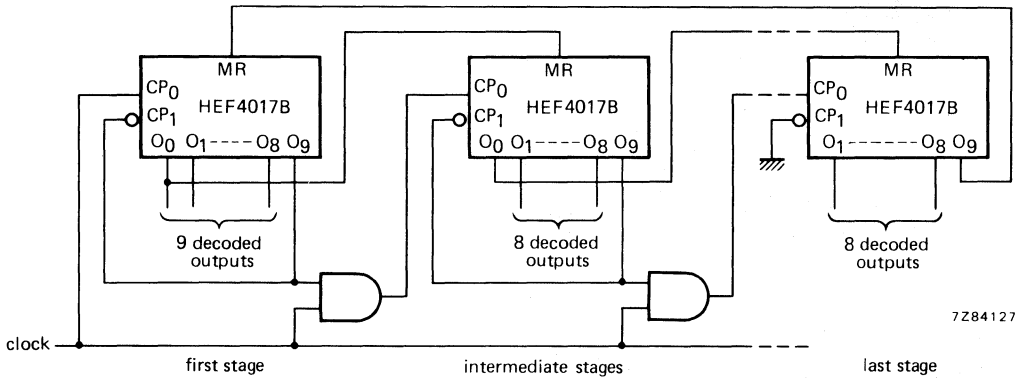
Fig. 7 Counter expansion.
