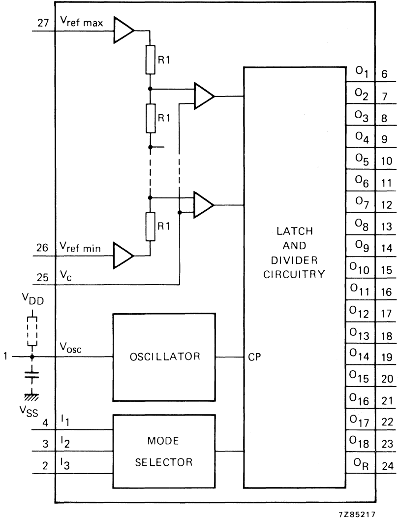
Fig. 1 Functional diagram.
