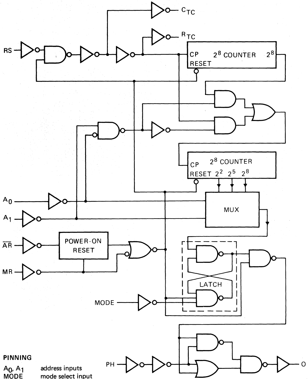
Fig. 3 Logic diagram.
