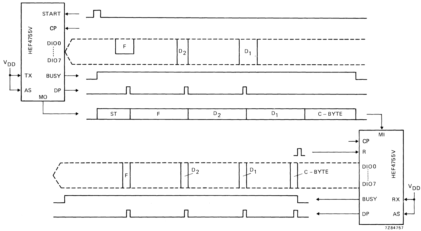
Fig. 6 Function/timing diagram when using the HEF4755V in the asynchronous mode where the byte number per message is variable and the hamming distance is 4.
