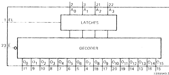
1-of-16 decoder/demultiplexer with input latches.
