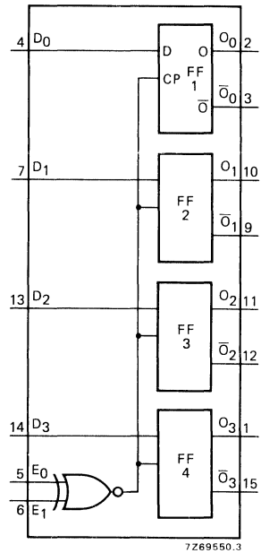
Quadruple D-latch.
