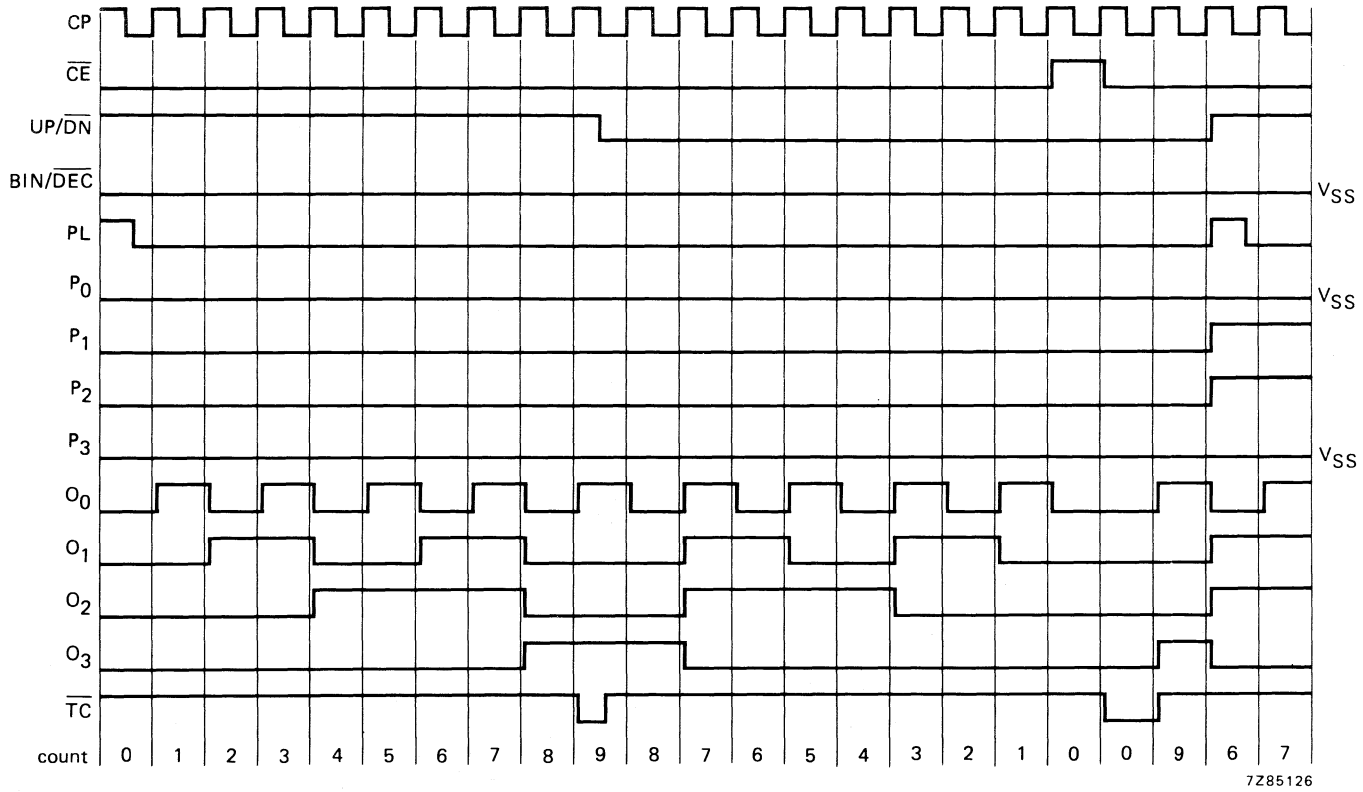
Fig. 8 Timing diagram; decade mode; P_0 = \text{LOW} ; P_3 = \text{LOW} ; \overline{BIN/DEC} = \text{LOW} .
