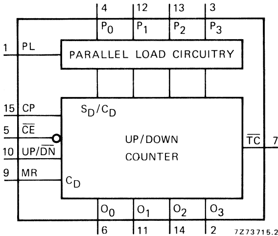
Fig. 1 Functional diagram.
