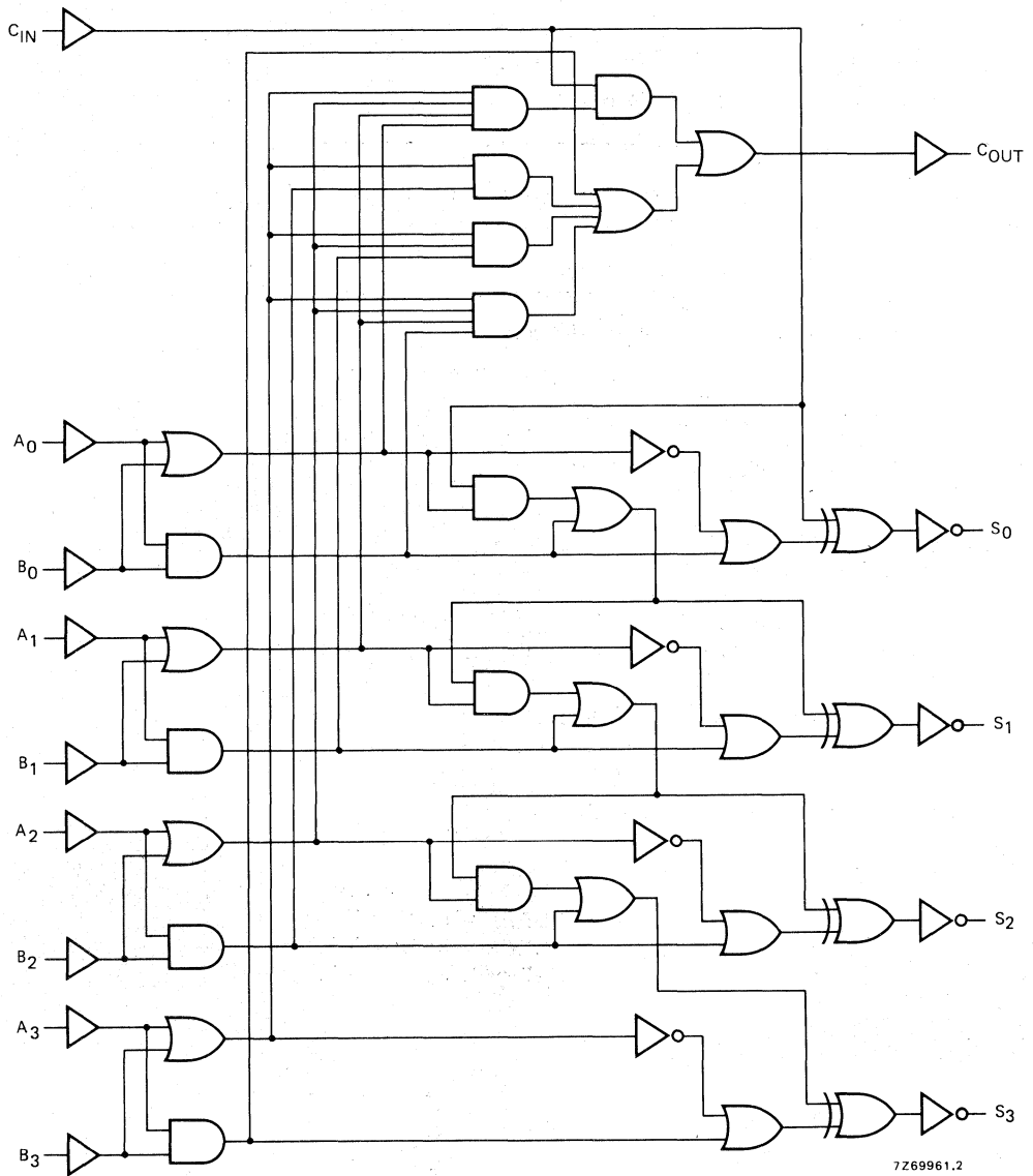
Fig. 3 Logic diagram.
