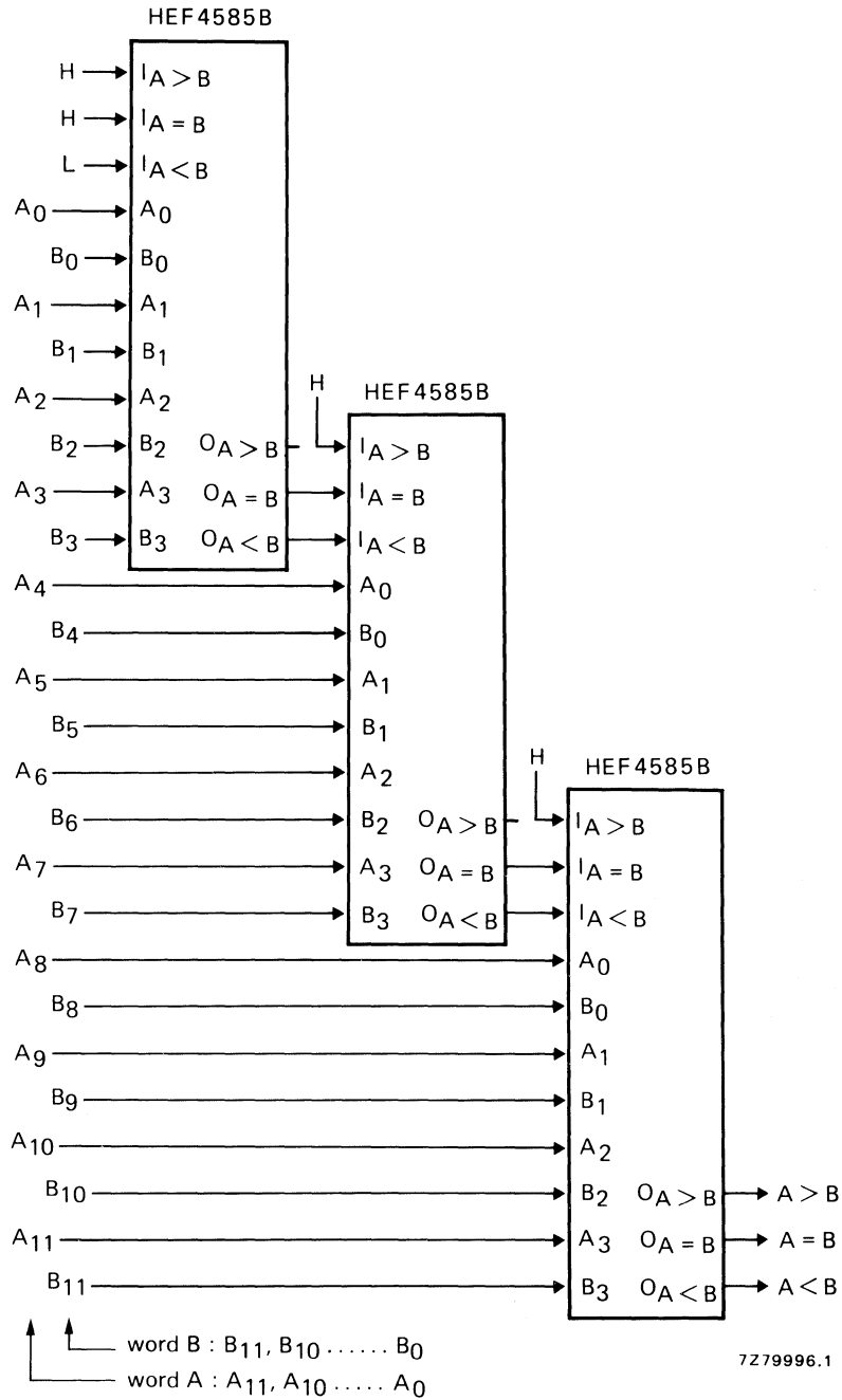
Fig. 4 Example of cascading comparators.
