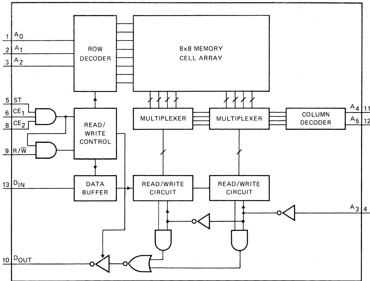
Fig. 2 Functional diagram.
