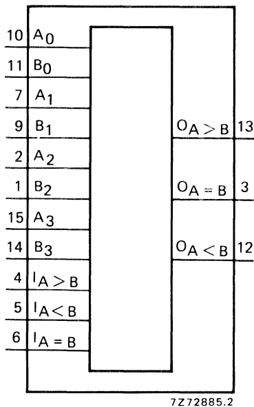
Fig. 1 Functional diagram.
