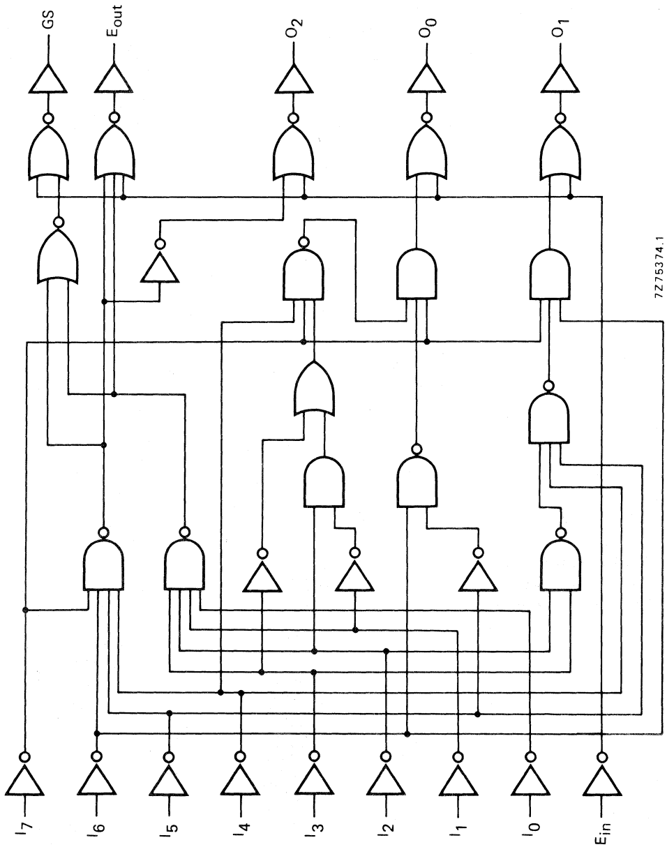
Fig. 3 Logic diagram.
