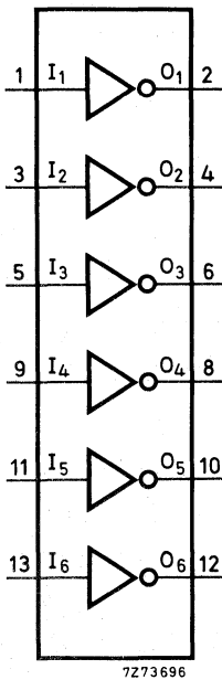
Fig. 1 Functional diagram.
