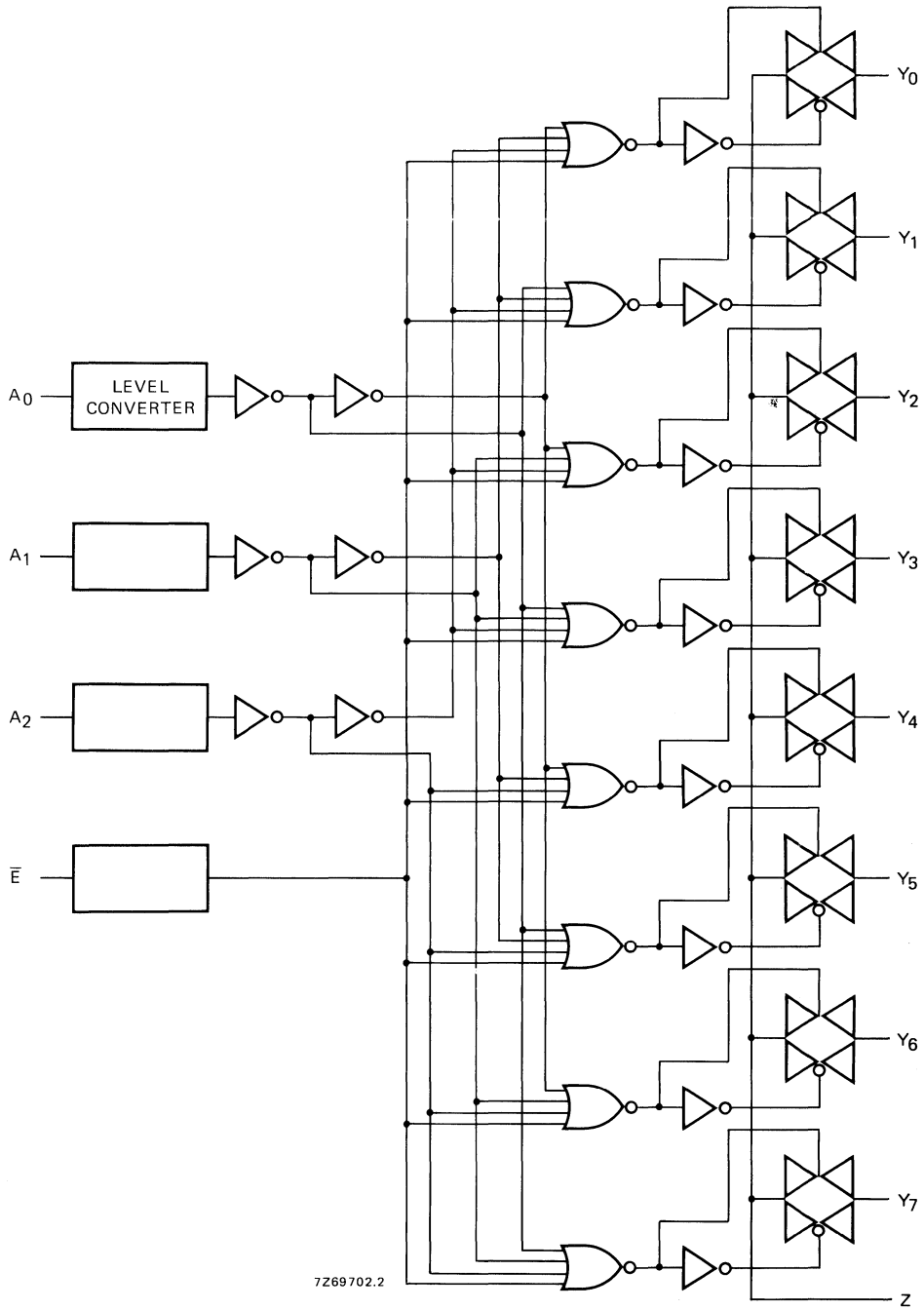
Fig. 4 Logic diagram.
