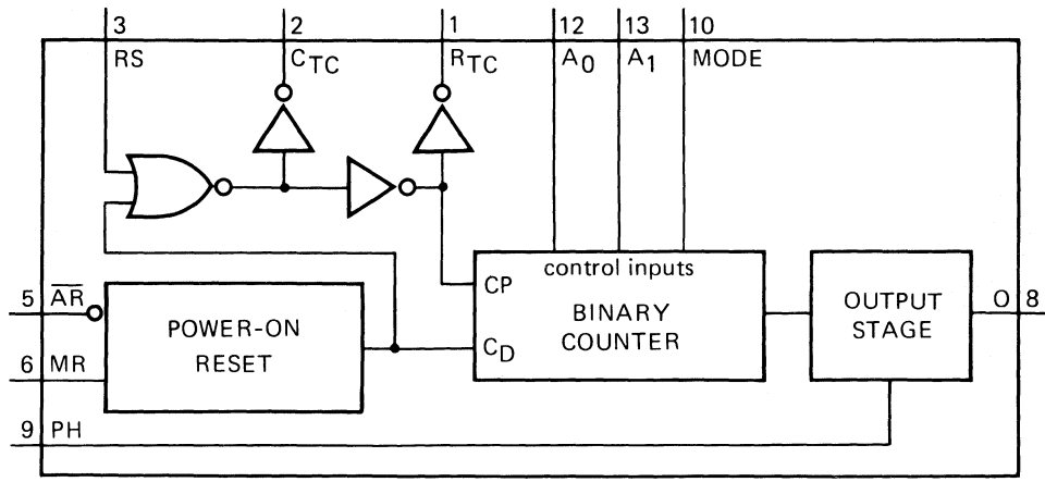
Fig. 1 Functional diagram.
