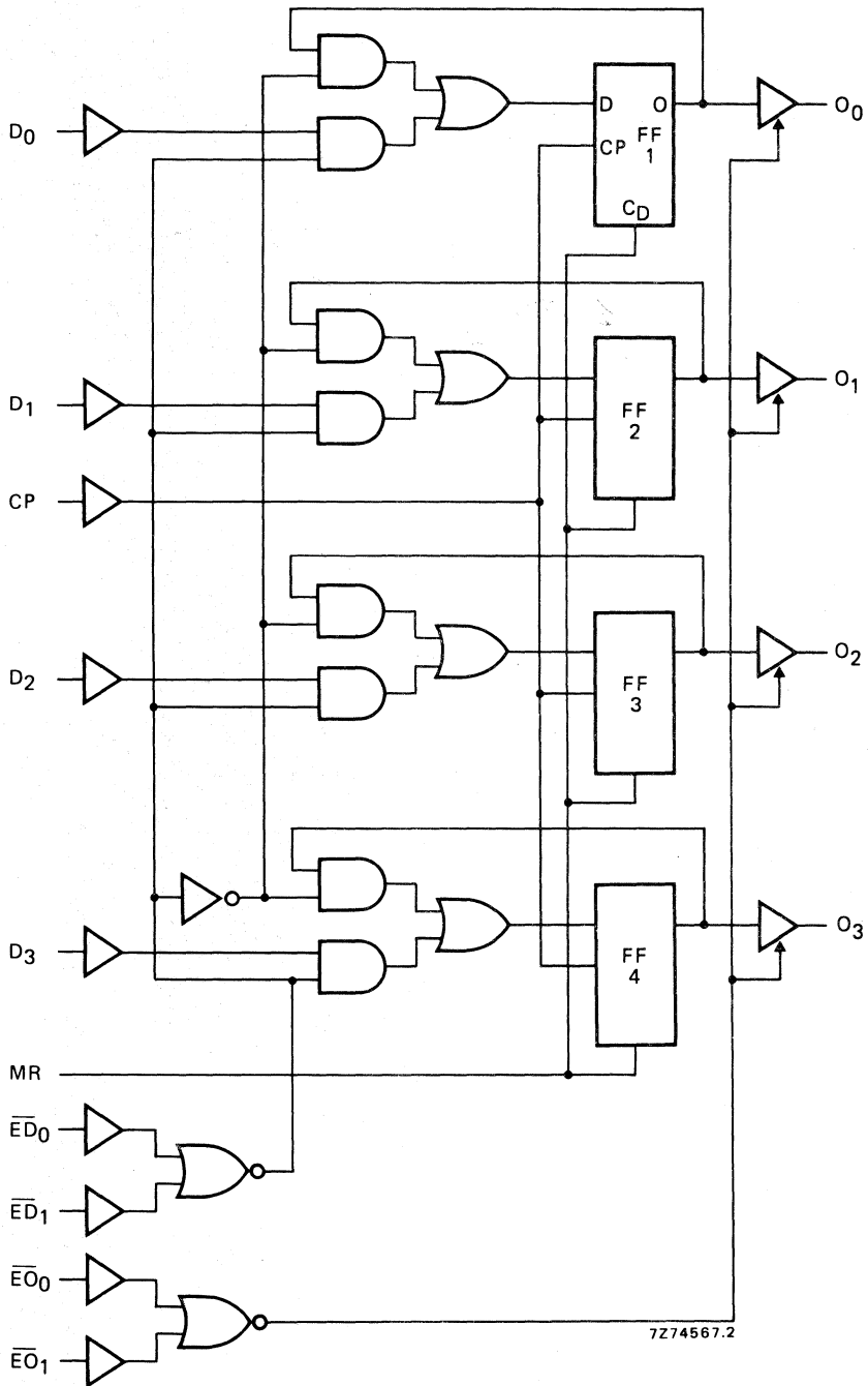
Fig. 3 Logic diagram.
