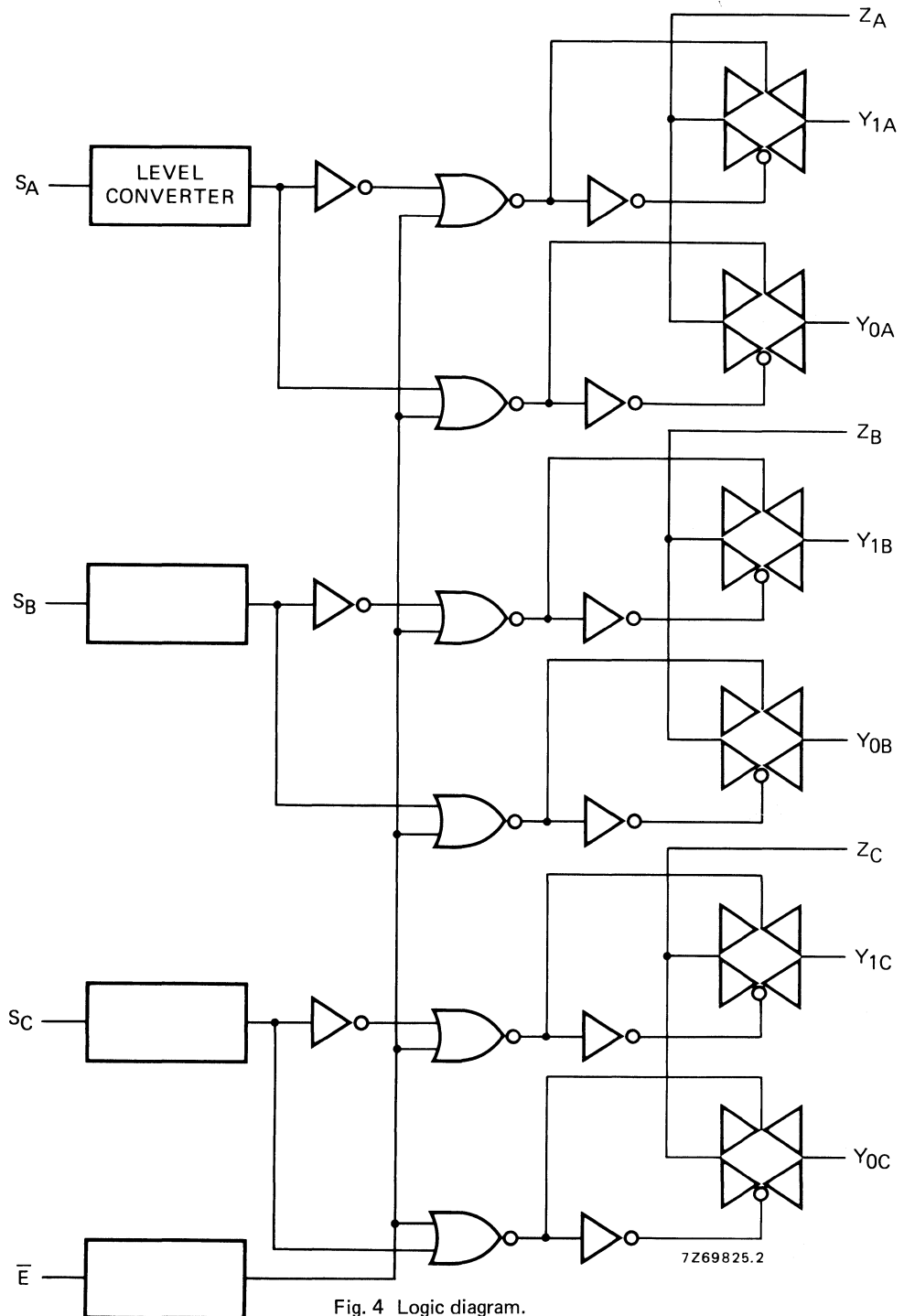
Fig. 4 Logic diagram.
