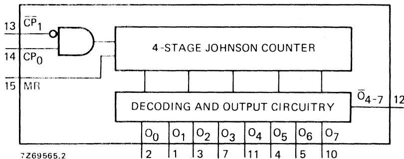
Fig. 1 Functional diagram.
