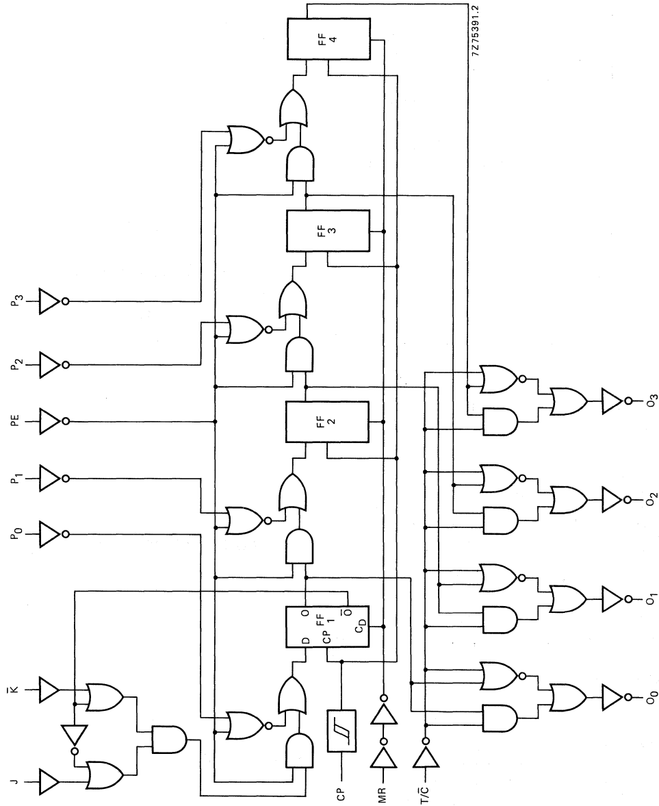
Fig. 2 Logic diagram.
