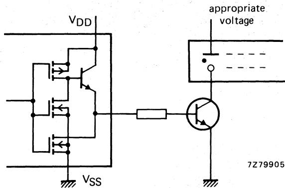
Fig. 13 Connection to gas discharge display readout.
