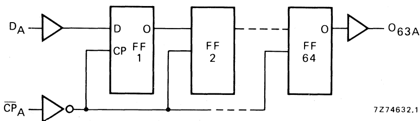
Fig. 3 Logic diagram (one of 64-bit shift register).
