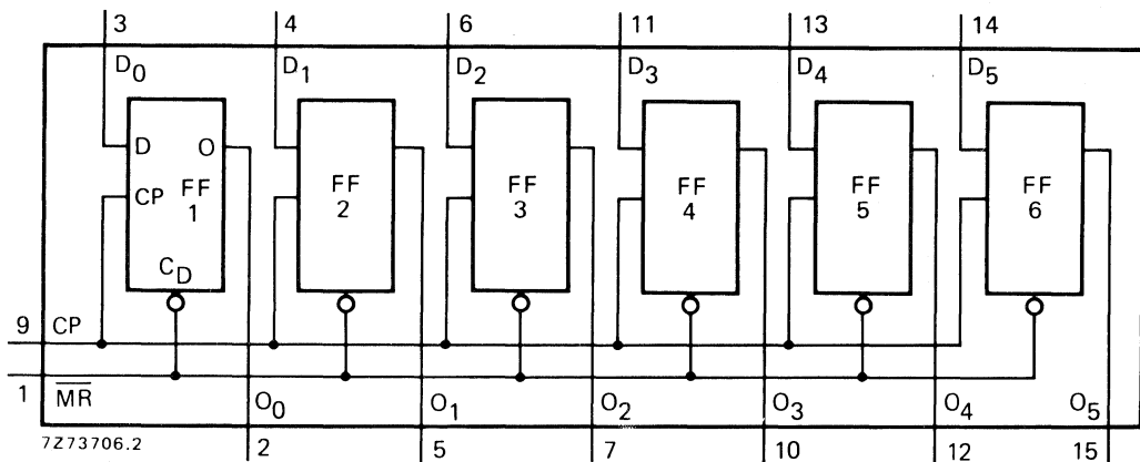
Fig. 1 Functional diagram.
