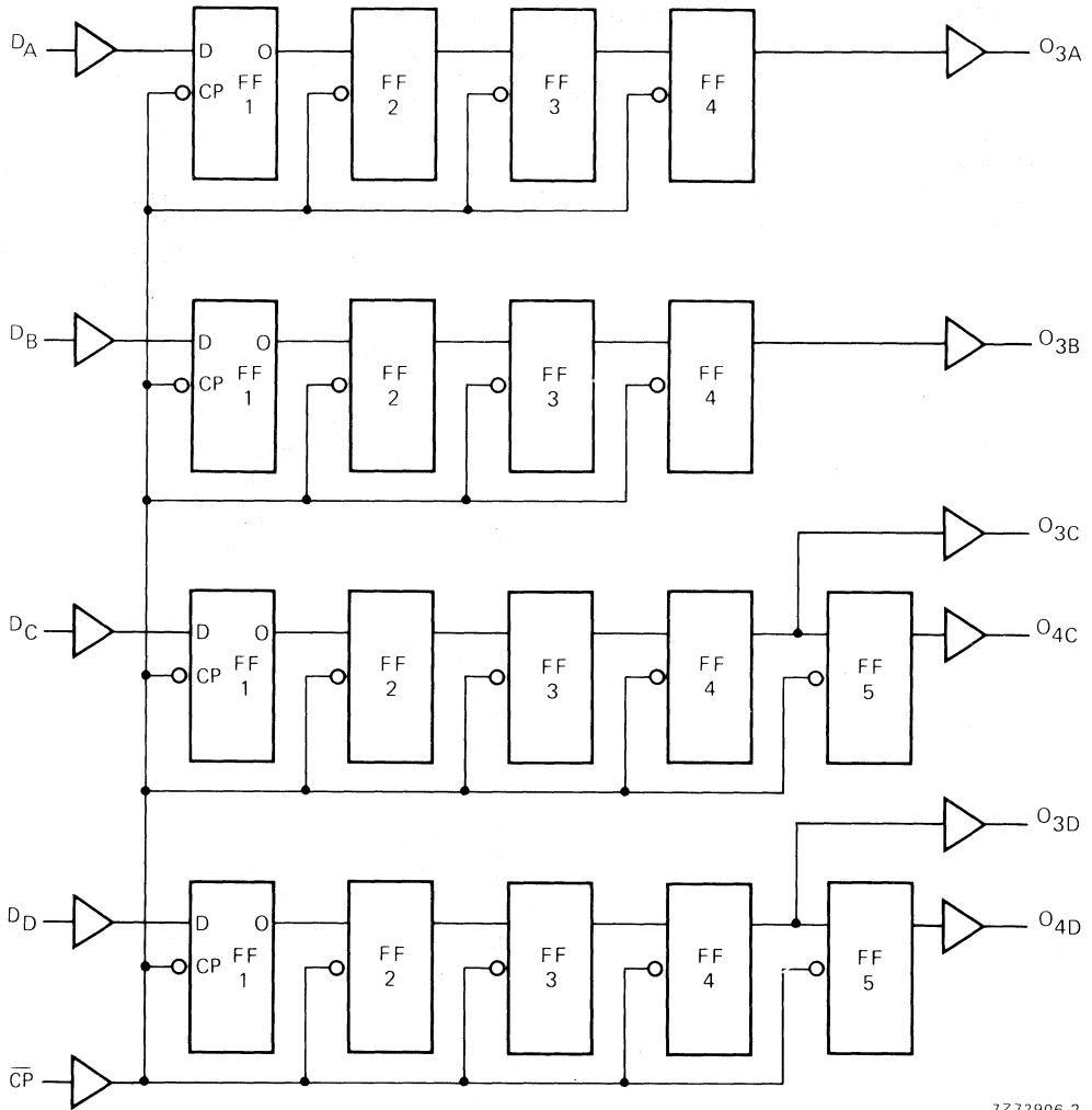
Fig. 3 Logic diagram.
