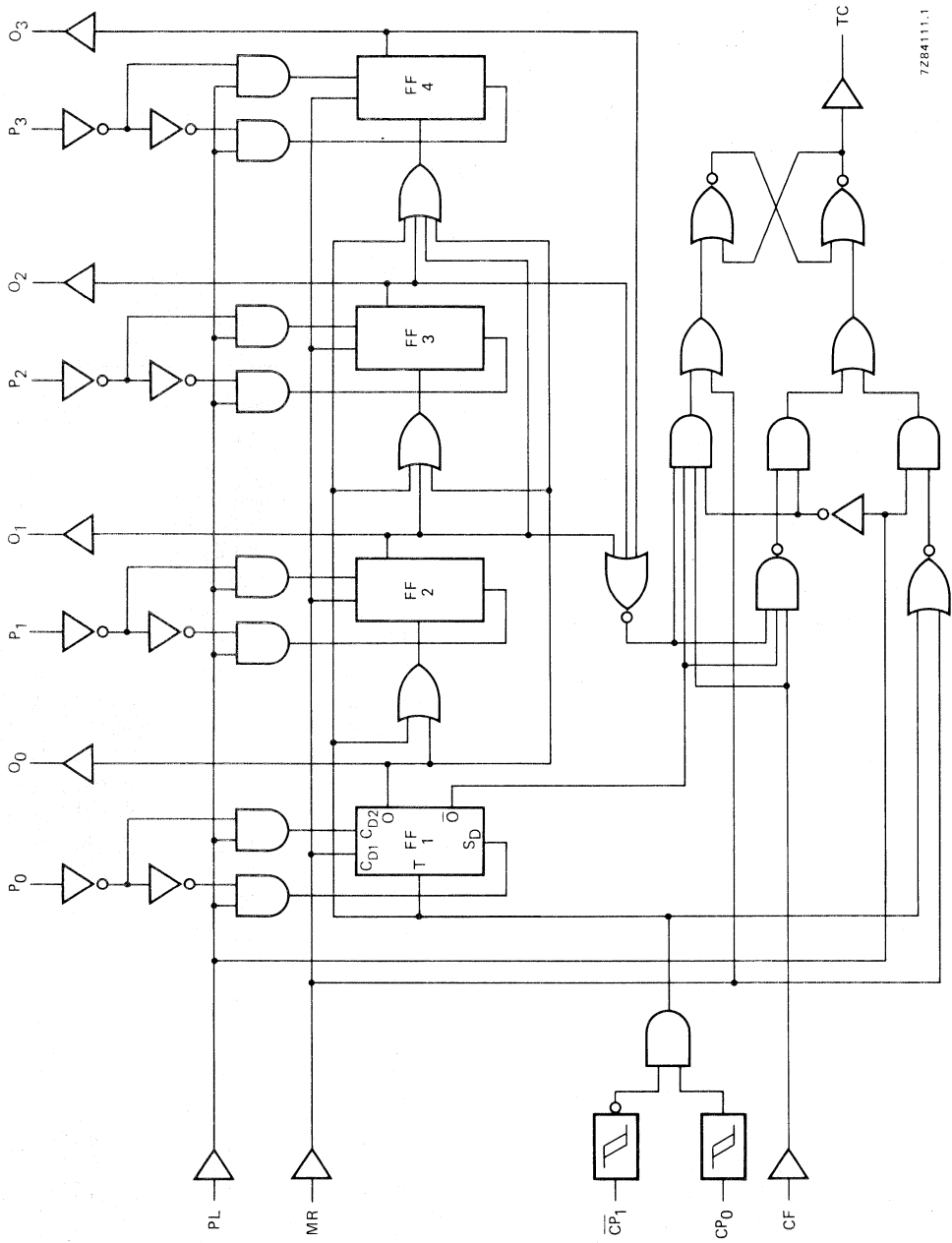
Fig. 4 Logic diagram.
