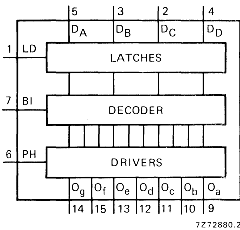
Fig. 1 Functional diagram.
