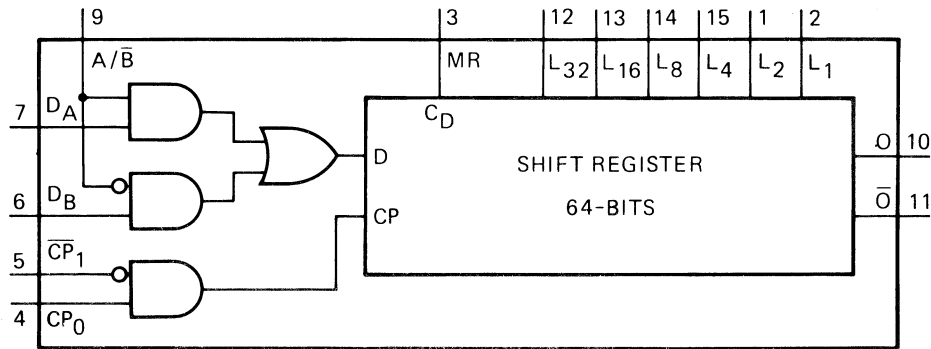
Fig. 1 Functional diagram.
