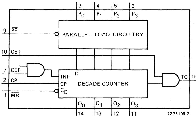
Fig. 1 Functional diagram.
