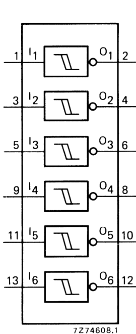
Fig. 1 Functional diagram.
