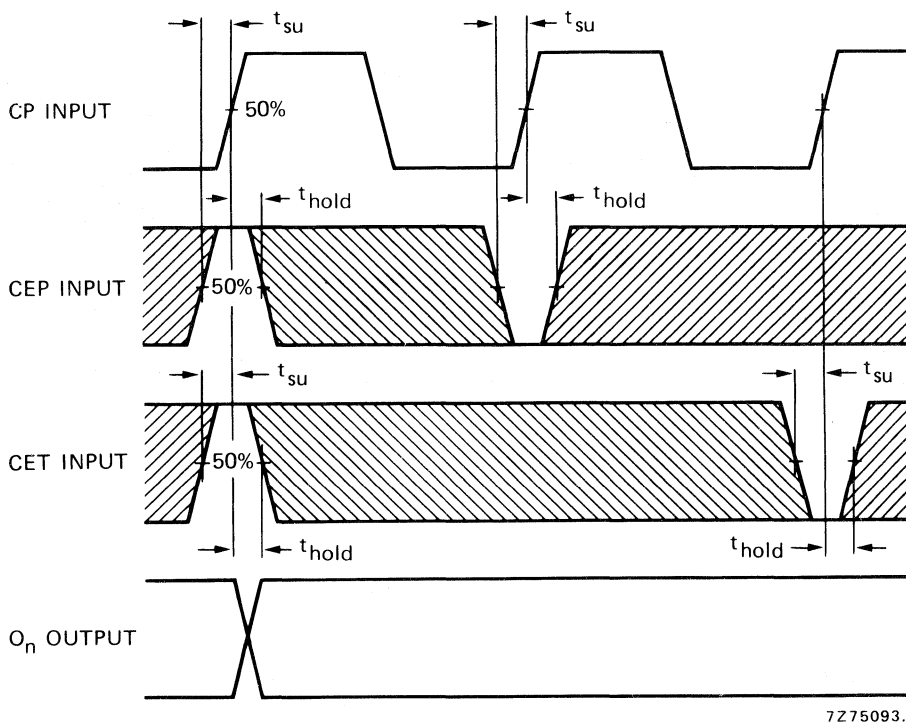
Fig. 6 Waveforms showing set-up times and hold times for CEP and CET inputs. Condition: \overline{PE} = \overline{SR} = \text{HIGH} .
