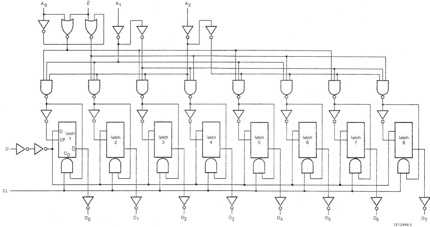
Fig. 3 Logic diagram.
