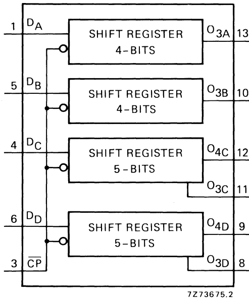
Fig. 1 Functional diagram.
