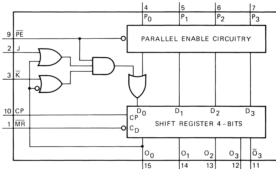
Fig. 1 Functional diagram.
