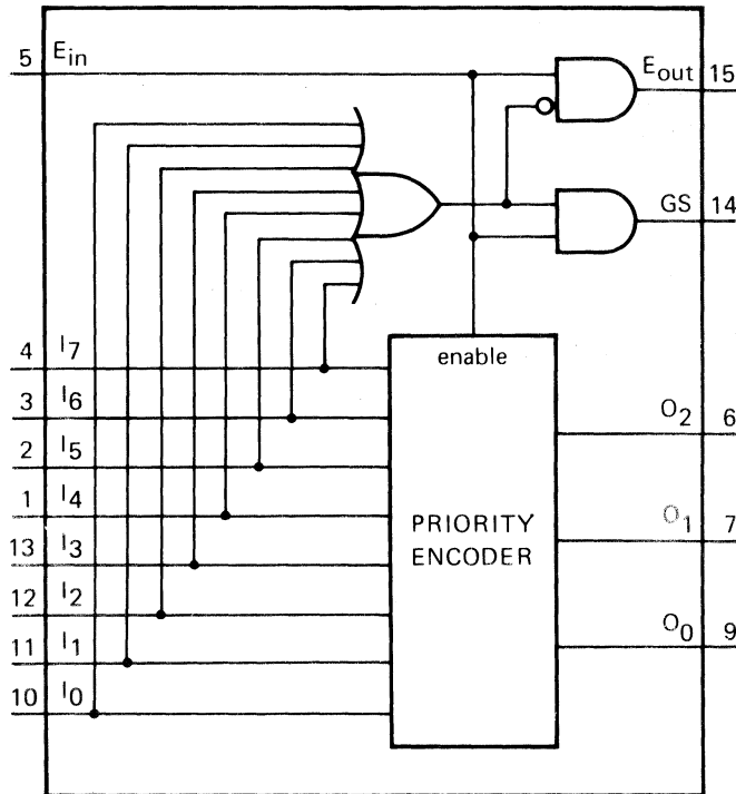
Fig. 1 Functional diagram.
