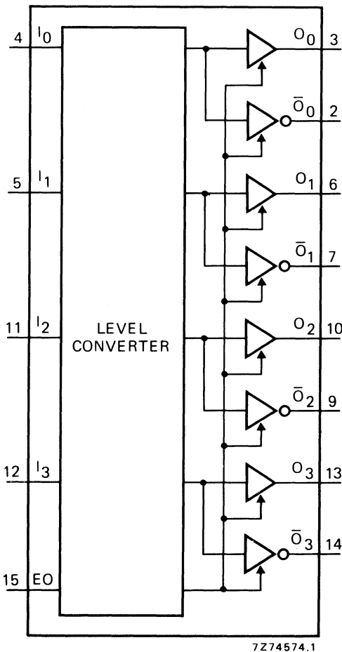
Fig. 1 Functional diagram.
