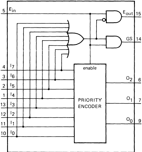
8-input priority encoder.
