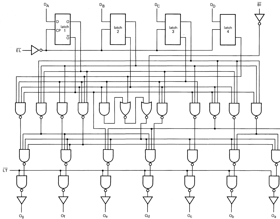
Fig. 5 Logic diagram; for one latch see Fig. 6.
