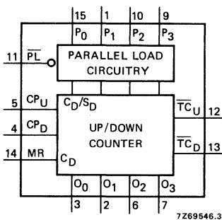
4-bit up/down decade counter.
