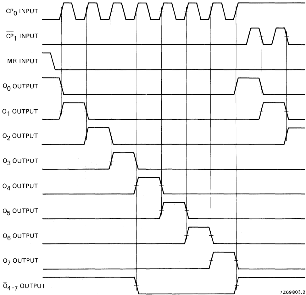
Fig. 6 Timing diagram.
