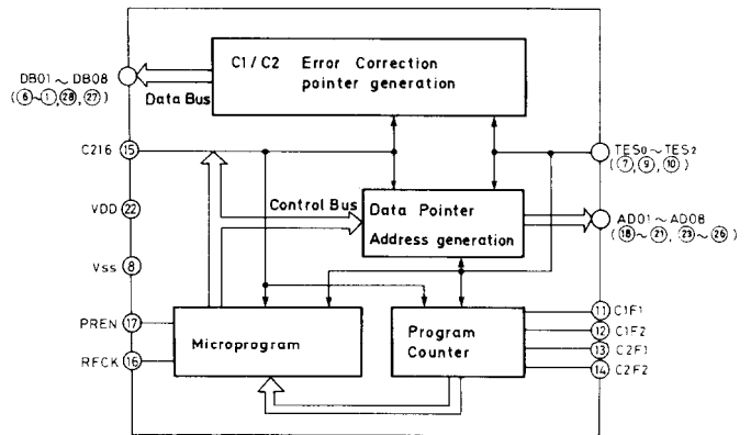
CX7935(Error correction)
