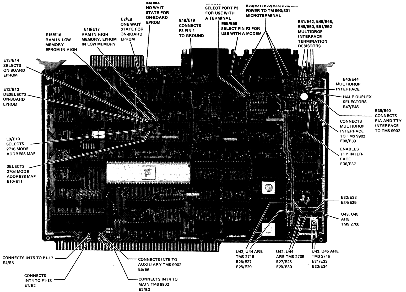
Figure 2-3. TM 990/101M Jumper Locations
