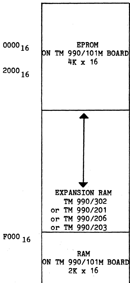
TM 990/101M WITH EXPANSION RAM
