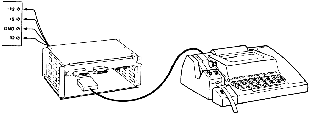
FIGURE 2-6. TM 990/101M BOARD IN TM 990/510 CHASSIS
