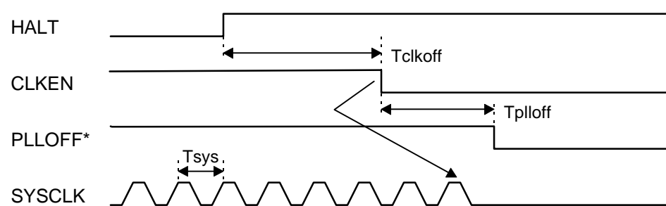
Figure 5-2 Standby mode (PLL stop)
