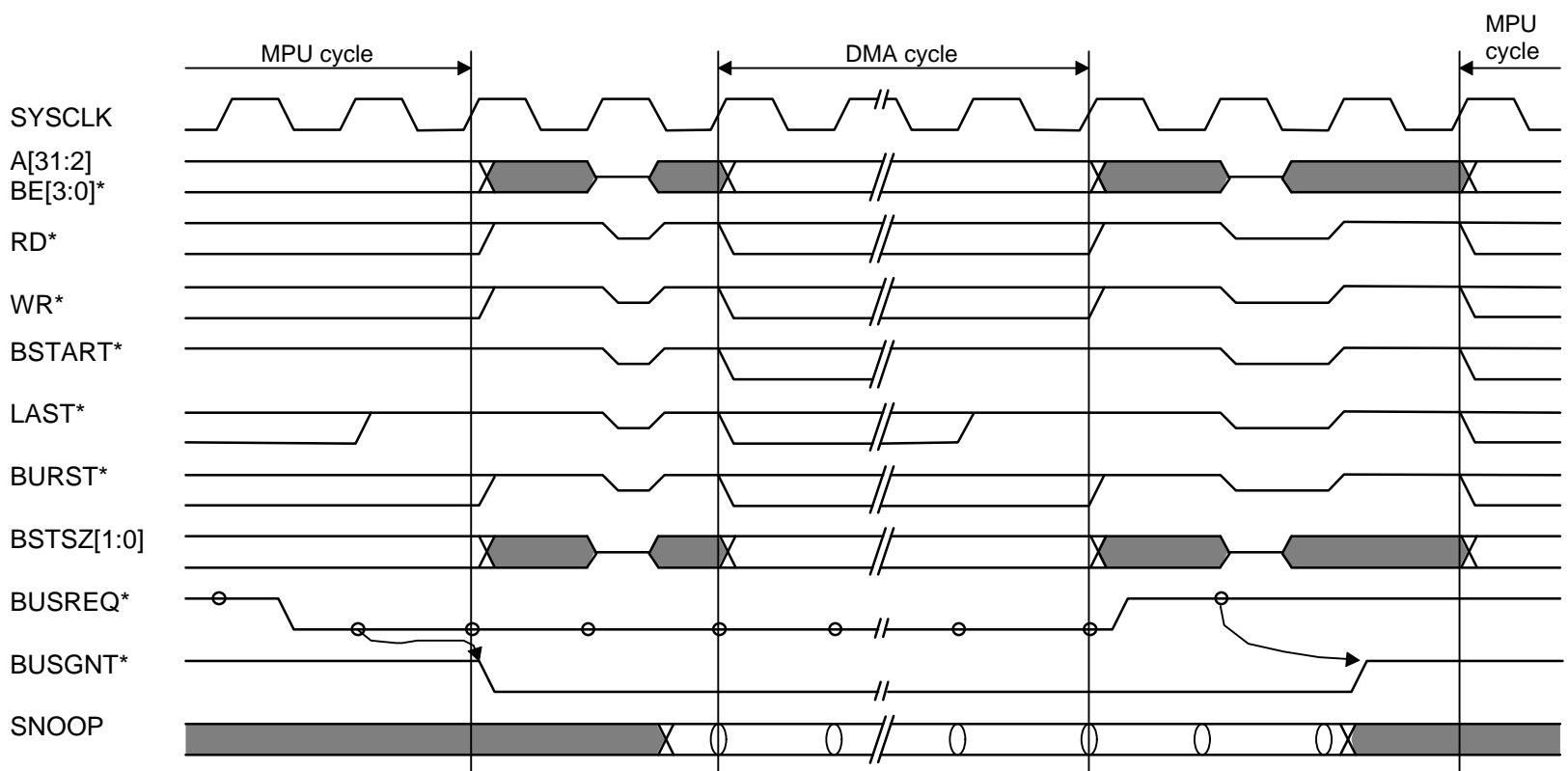
Figure 4-8 Bus arbitration
