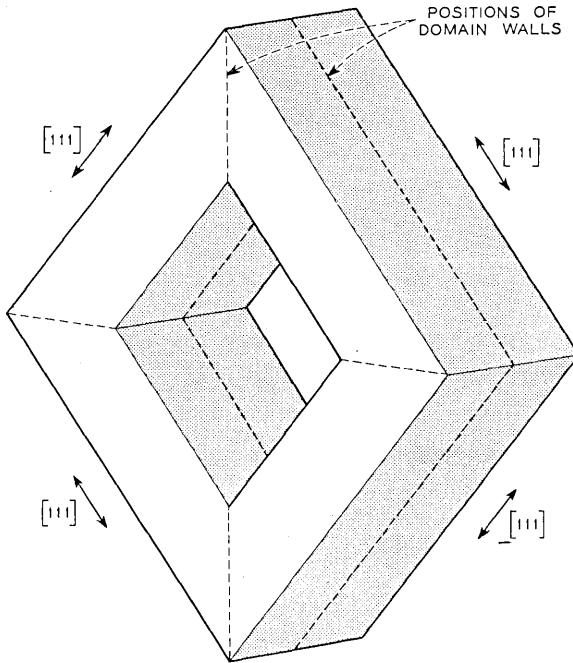
Fig. 1 — Sample of ferrite used in this study.
