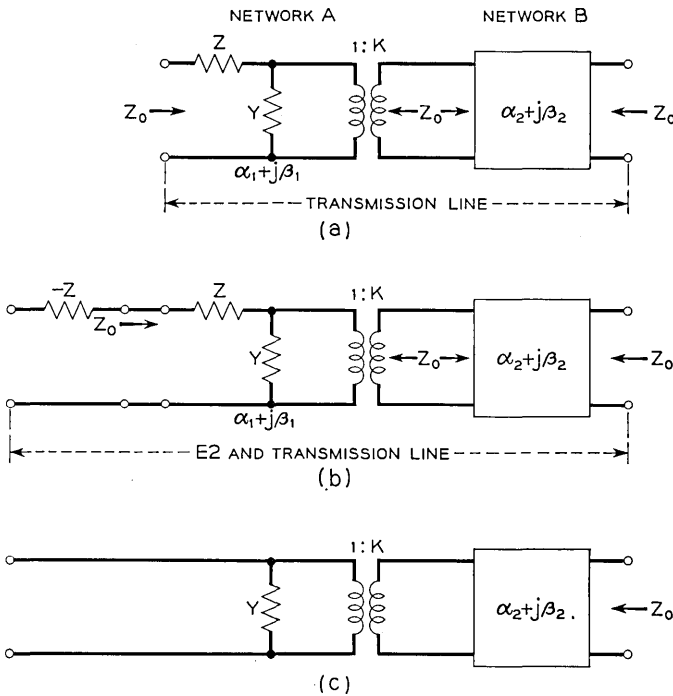
Fig. 9 — Operation of -Z in a transmission line: (a) transmission line, (b) repeater and transmission line, and (c) result of adding repeater.
