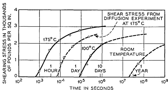
Fig. 9 — Shearing strength of copper-tin-nickel silver connections as a function of time and temperature.
