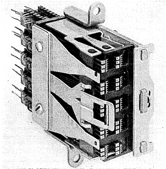
Fig. 1 — New 30-contact relay with contact cover detached.
