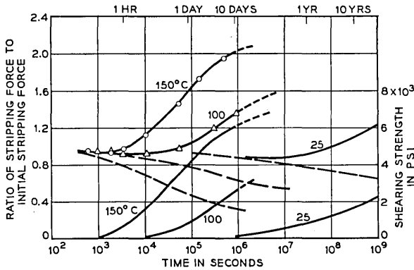
Fig. 14 — Stripping force and shear strength of bare copper on nickel silver connections as a function of time and temperature.
