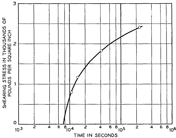
Fig. 8 — Diffusion shearing strength for tinned copper wire on nickel silver at 175°C as a function of time.
