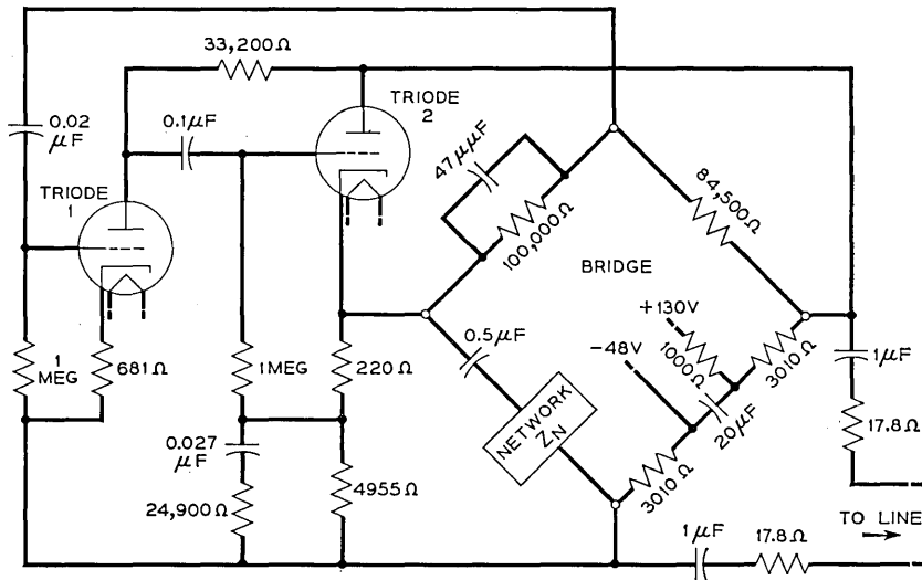
Fig. 17 — Schematic circuit of E3 repeater.
