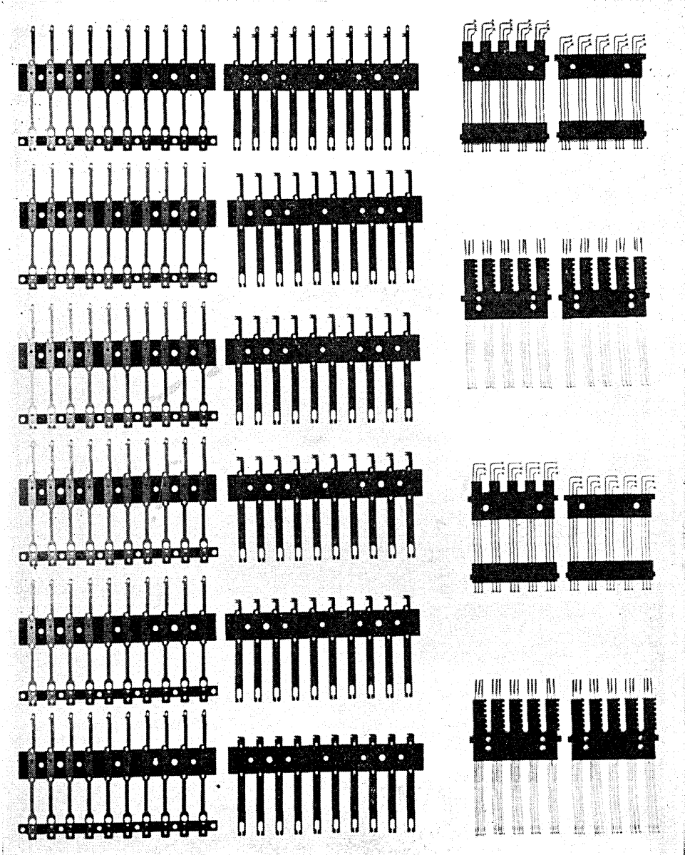
Fig. 9 — A comparison of molded wire assemblies for a 60-contact replacement relay with the corresponding flat spring relay parts.
