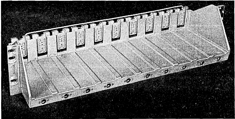
Fig. 21 — Repeater mounting shelves. Upper for 19-inch bays, lower for 23-inch bays.
