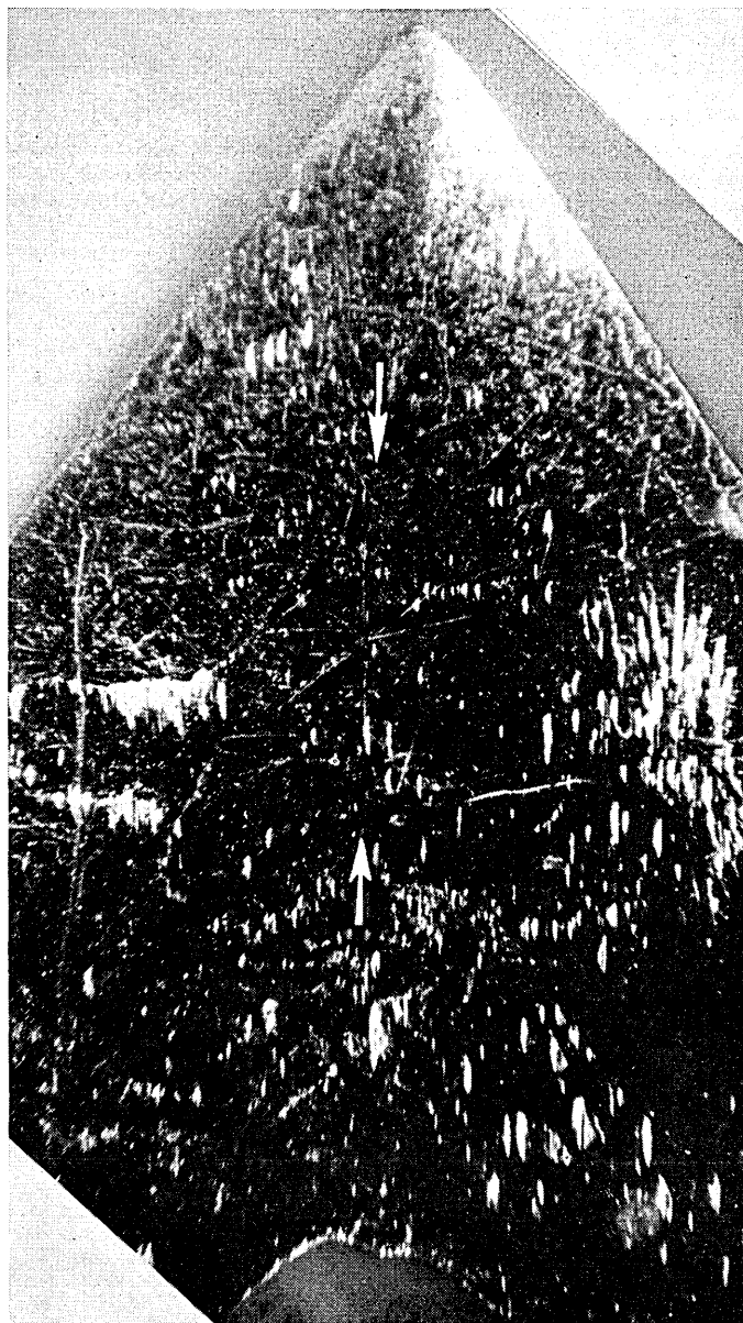
Fig. 4 — Picture of domain pattern at one corner of sample. The stationary wall is indicated by arrows.
