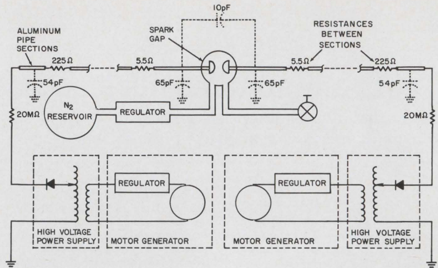
1. Electrical design of long-wire antenna and power supplies. The antenna is comprised of sections of aluminum pipe connected through large resistors. The pipe diameters vary from 12 inches at the center to 4 inches at the ends. The high-voltage supplies charge the gap and antenna capacities.
