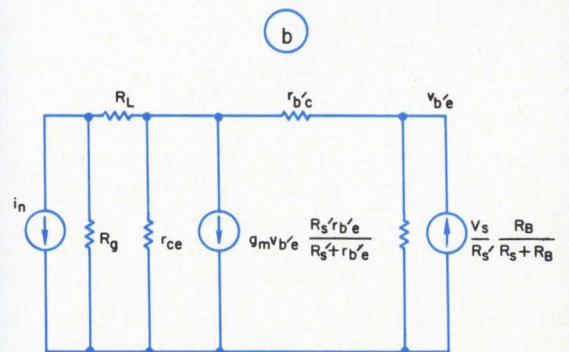
4. A common-emitter stage isolates ground-loop noise if the emitter bypass capacitor is placed at the signal source (a). An equivalent circuit is used for circuit analysis (b).
