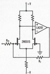
LOW NOISE DIFFERENTIAL AMPLIFIER
