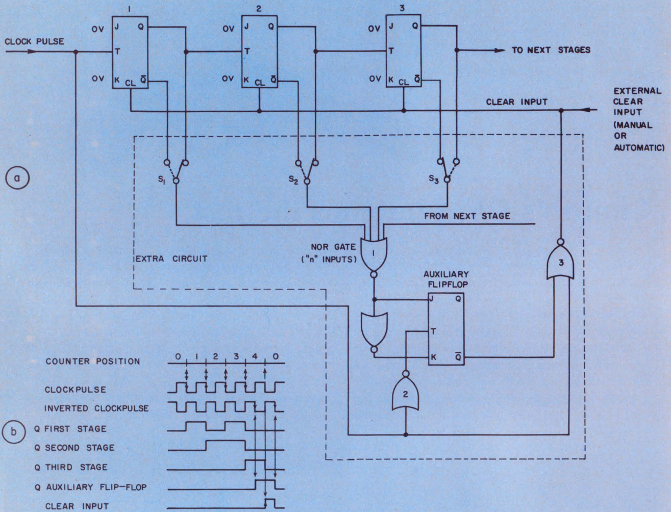
Maximum count is determined by the positions of switches S1, S2, . . . , SN in this variable-length
