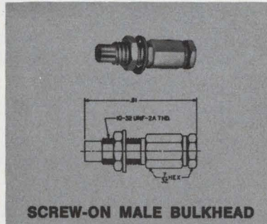
SCREW-ON MALE
