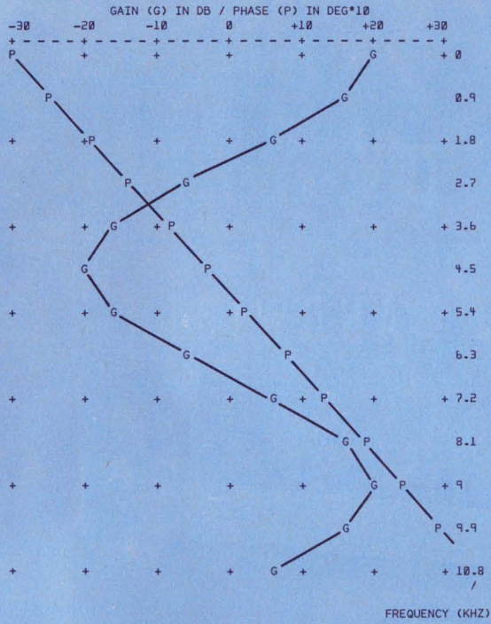
2. Curve plot performed by program is shown for linear (a) and logarithmic (b) frequency scale.
