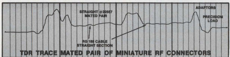
TDR TRACE MATED PAIR OF MINIATURE RF CONNECTORS
