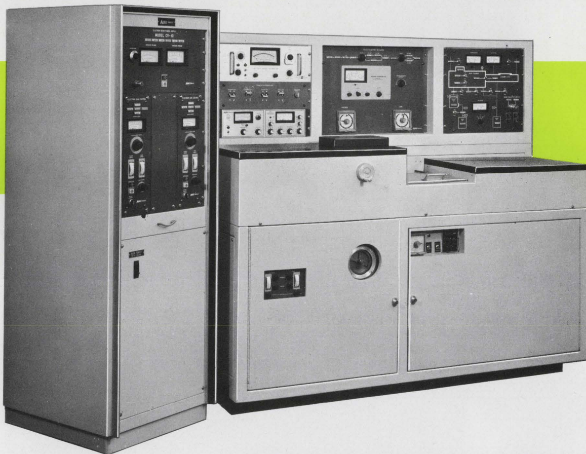
General Electric meters, SCRs, capacitors, selector switches, indicating lights, Volt-Pacs®, gear motors, current transformers and arc pilot devices are used in Airco Temescal's line of Integrated Electron Beam Systems and products such as this Thin-Film Electron Beam Deposition System. (For more information, circle 811.)
