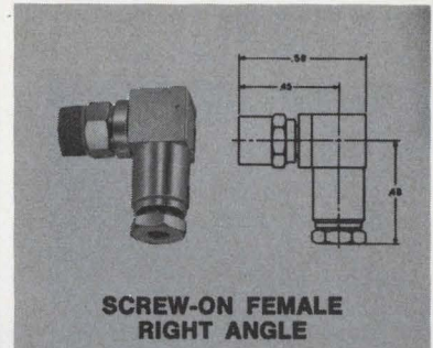
SCREW-ON FEMALE
