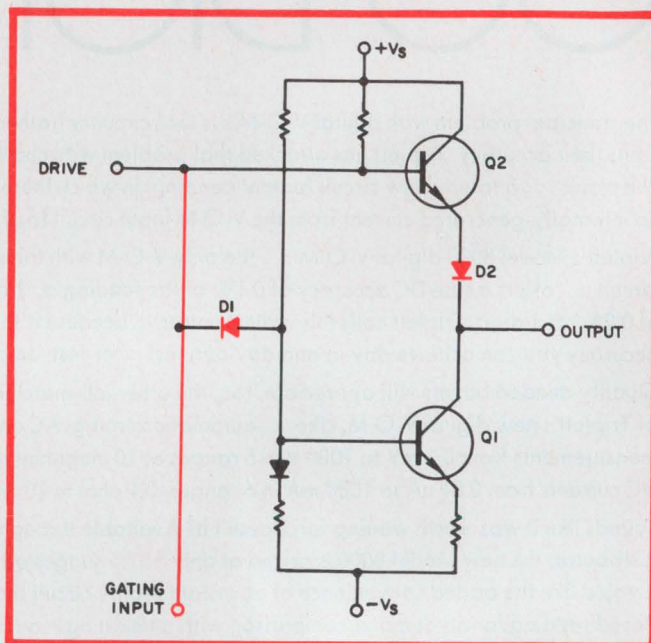
1. Two diodes add gating capability to this Class A output op amp. Similar techniques can be applied for op amps with Class B and emitter-follower output stages.
