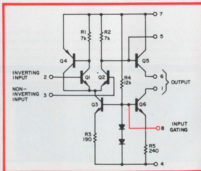
2. One lead is all that is required to convert the ZLD2T operational amplifier for gated operation. External components are required to convert most other existing IC op amps.
