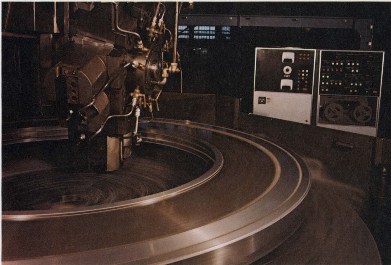
Minicomputers are the heart of many industrial control systems , such as this 86-inch vertical turret lathe, controlled by a Westinghouse Electric Corp. C20 system. It
