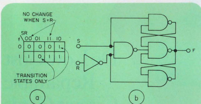
A set-reset flip-flop (b) that does not change state when its inputs are the same can be used as a line receiver because of its high noise rejection. A Karnaugh map (a) tabulates the various input and output functions of the flip-flop.
