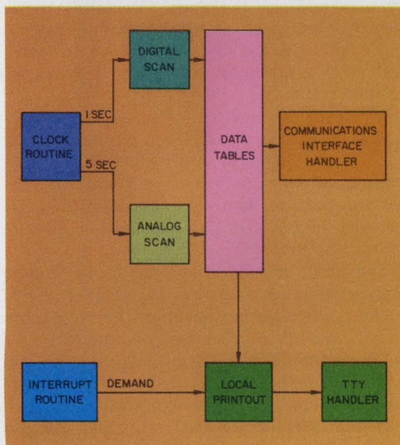
2. Prepare program word estimates more easily by using a block diagram to indicate the programs required and the relations between the programs. This program covers the example of Fig. 1.
