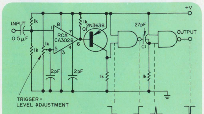
Use just one supply to power both your logic and trigger circuits. Compatible with either TTL, DTL or RTL, this trigger circuit requires only 3 to 9 V. It accepts sine waves of up to 1 V rms.
