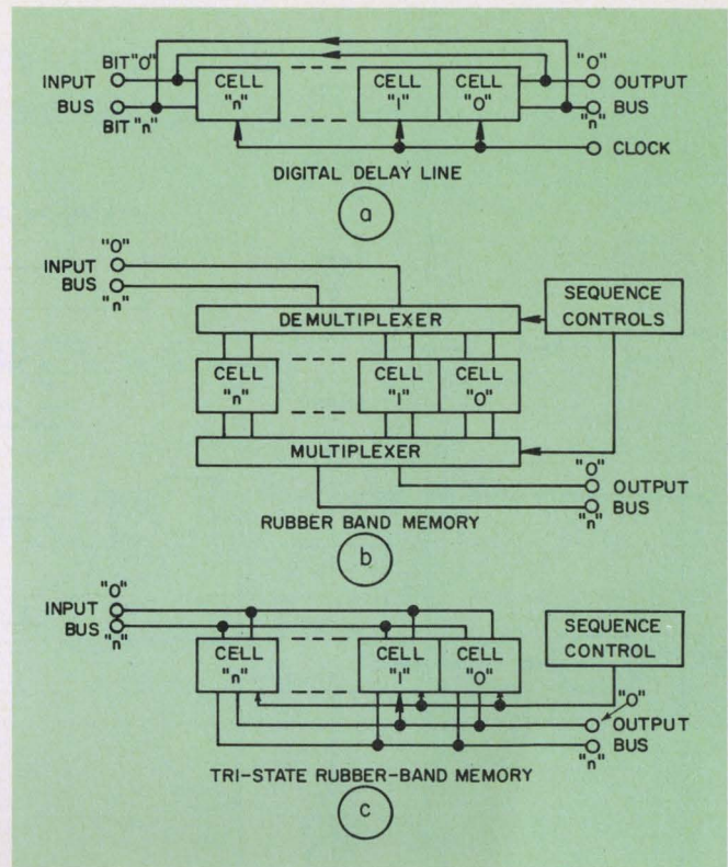
1. Conventional scratchpad memories , such as the digital delay line (a), can't be written into at one rate and out at another. Although this can be done by the memory arrangement of (b), switching problems make the technique impractical. Most efficient asynchronous data transfer is possible with the "rubber-band" scratchpad memory of (c), which uses tri-state logic elements.
