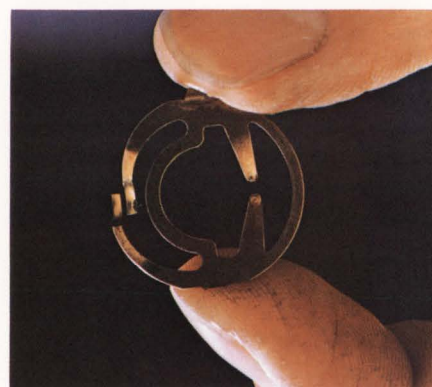
The fine copper springs used in contacting resistors can be coated with conductive/lubricating coatings. This provides for longer life before high electronic noise levels are reached.
