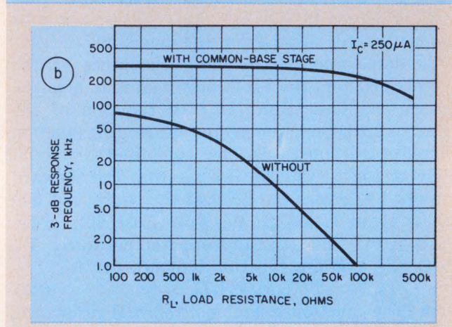
8. Improved frequency response of a phototransistor is obtained with a common-base load-impedance transforming network (a) in either the collector or emitter circuit. The degree of the improvement is shown in "b".
