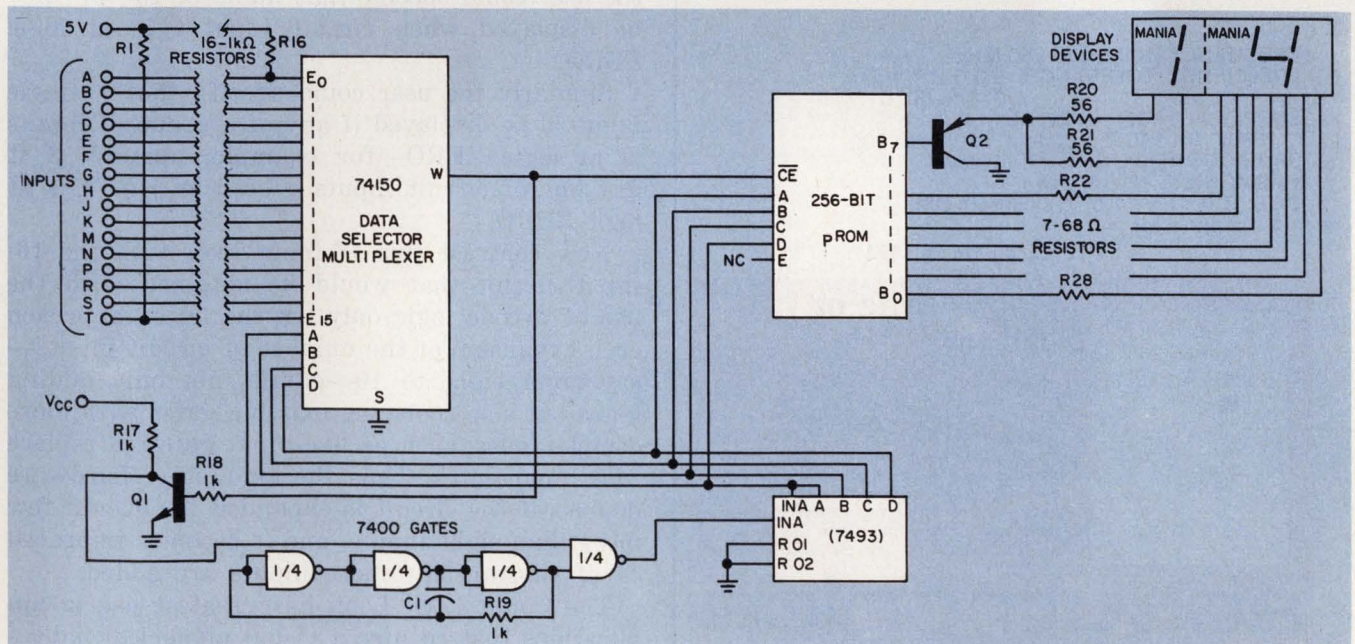
3. A 16-input Count Lock Loop requires only a larger data selector/multiplexer, a pROM instead of a decoder/
