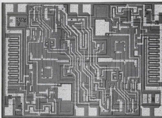
National Semiconductor's new LM119 is a dual precision comparator. It has faster response than the LM111 and lower input currents than the \mu A710 . Unlike other dual comparators, it can operate from a single +5-V supply or from symmetrical positive and negative lines.
