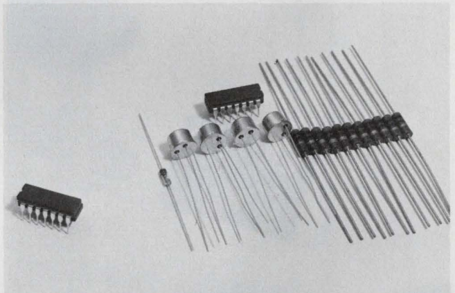
Fairchild's \mu A750 dual-comparator subsystem (left) can replace (right) a conventional dual comparator, 11 resistors, four transistors and one zener diode. The monolithic circuit includes two independent high-current comparators, a voltage reference and circuitry for hysteresis control and overload protection.
