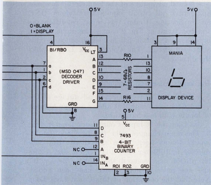
decode logic only, but the octal configuration insures that only one input determines the numeral displayed. And it can be easily expanded for more inputs.
