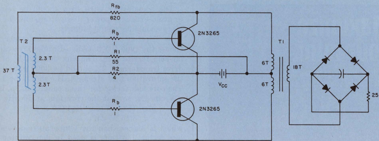
7. The complete schematic of a 250-W converter shows component values calculated in the example.
