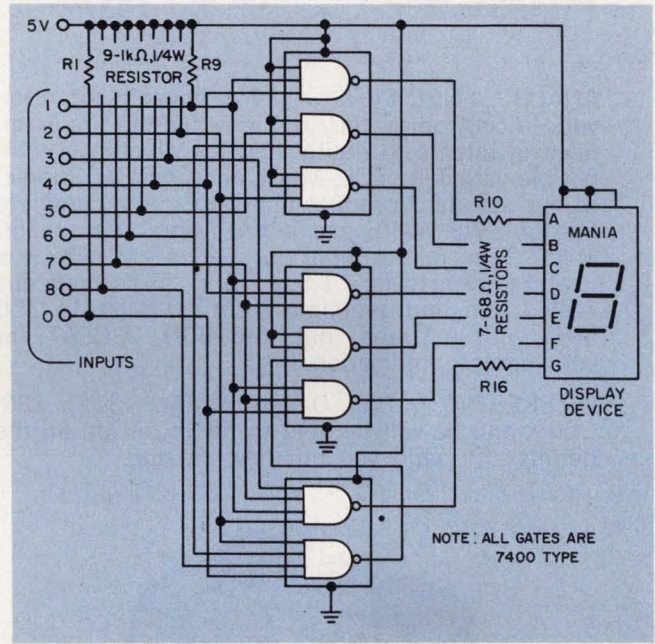
2. With decode logic only, you can build this circuit. But the disadvantages include erroneous displays, non-significant numerals and limited expandability.
