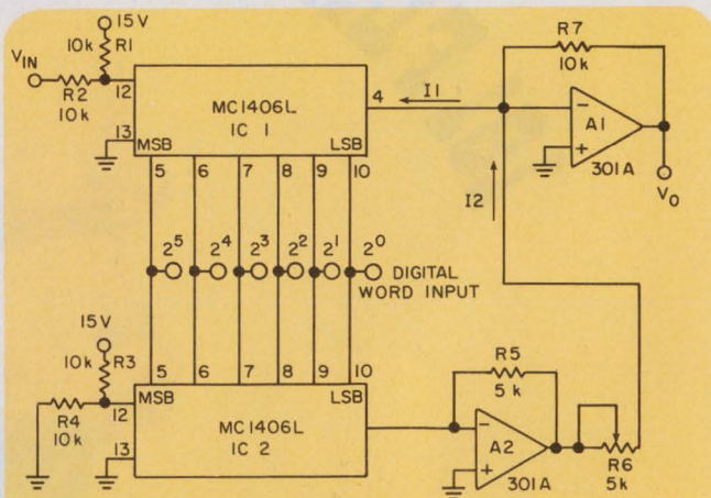
A combination of two unipolar multiplying d/a converters provides a bipolar-output scaled by the digital word input. Resistor R 6 should be set to equal the value of R 5 .
