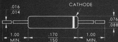
CASE STYLE "H"
