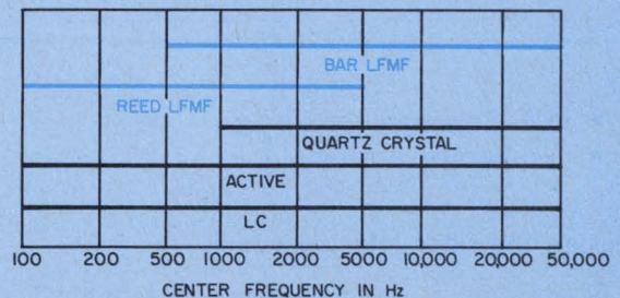
2. A wide range of applications for low-frequency, mechanical filters makes them highly competitive with other types, including crystal, active and LC filters.
