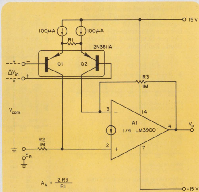
1. Basic instrumentation amplifier sums the differential collector currents of Q 1 and Q 2 , caused by incremental signal \Delta V_{IN} .
