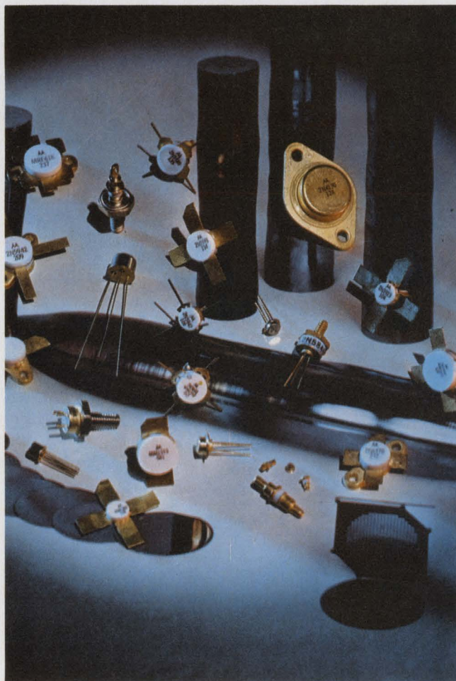
Motorola offers rf transistors in a variety of packages, including TO-3 types and its SOE configuration.
