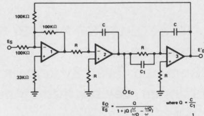
Active filter with high Q and excellent stability.
