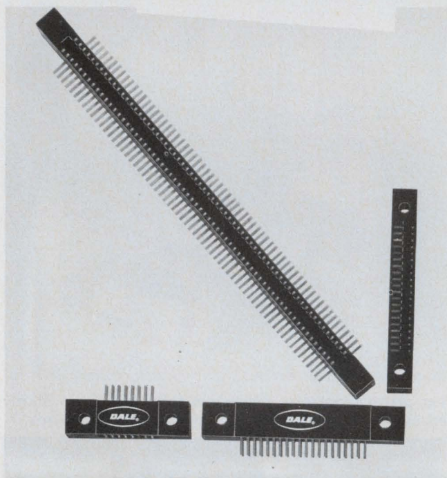
These Dale card-edge connectors feature 50-mil contact spacing, which is the highest density available for this type of connector.
