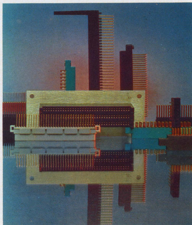
One- and two-piece connectors from ITT Cannon Electric show three types of termination tails—dip solder, solder eyelet and wrapped wire.
