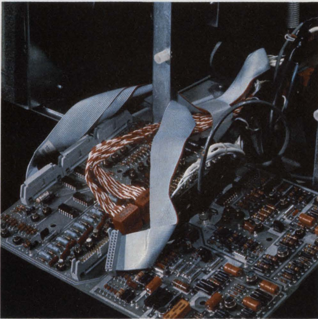
Flat-cable connectors from 3M, with wrapped-wire or dip-solder tails, can be mounted on the surface of a board, either vertically or horizontally.
