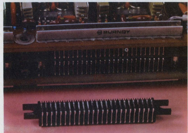
High pressure contacts in Burndy's brand new board-to-board connector allow stacking of boards without solder or jumper cables.
