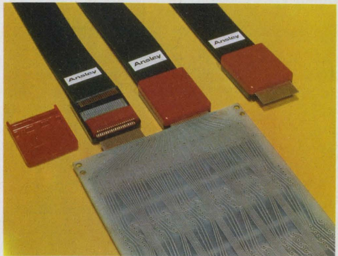
This flat cable, zero-insertion-force connector from Ansley clamps spring-loaded contacts to the PC board.
