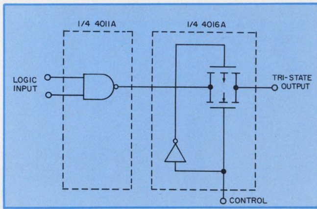
7. CMOS Tri-State outputs can also be obtained with a bilateral switch circuit. A simple gate and a transmission switch in series with the output form the basic circuit.
