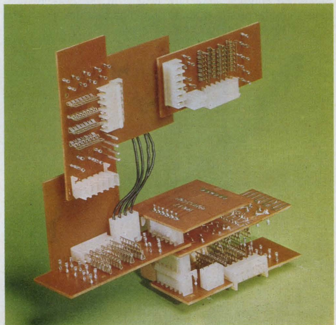
Two-piece Konektcon connectors from Molex are sturdy enough to support a stack of small daughter boards.
