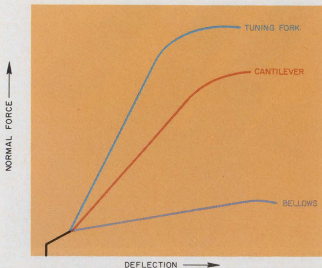
2. The normal force at the contact-mating surfaces depends on contact deflection which, in the case of one-piece connectors, depends on board thickness. The force also depends on contact style.
