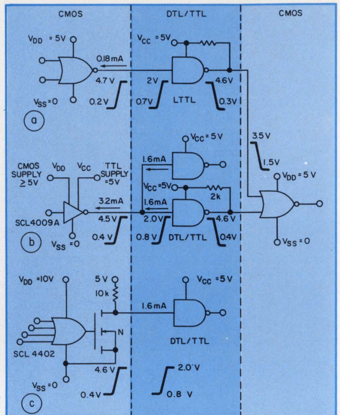
4. For the CMOS-to-TTL interface, special considerations for speed (CMOS can't be operated at high speed with 5-V TTL supplies) and sinking current are required. For LTTL, the CMOS device must be able to sink 0.18 mA (a), while for standard TTL the sinking current per TTL load is 1.6 mA at less than 0.5 V (b). For higher CMOS supplies, use the configuration in c.
