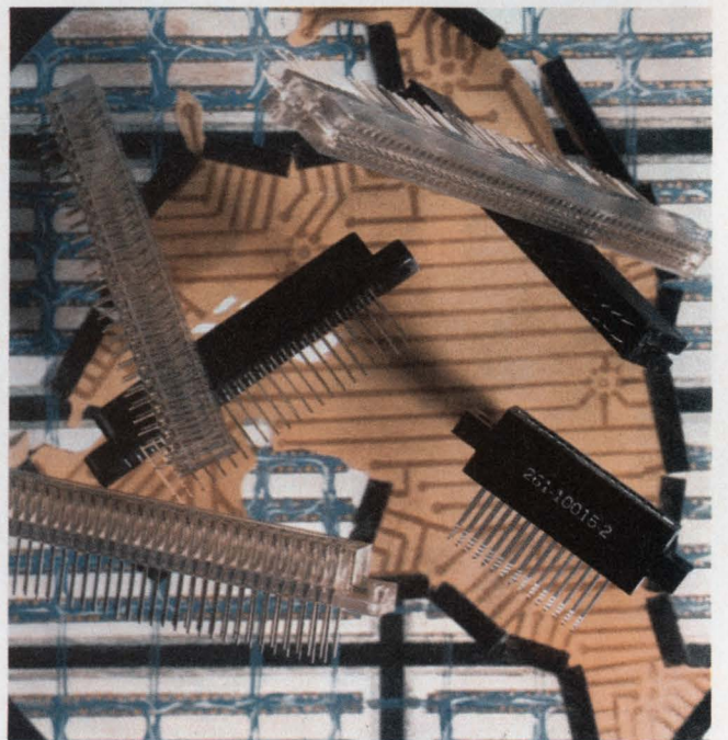
Transparent nylon housing shows the cantilever contacts in the first standard PC-connector line from Texas Instruments. The contacts have gold mating surfaces.
