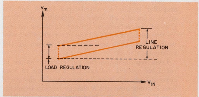
3. Graph depicts scope display when V_{in} drives horizontal input and V_m drives vertical input. Line and load regulation are read directly from display.
