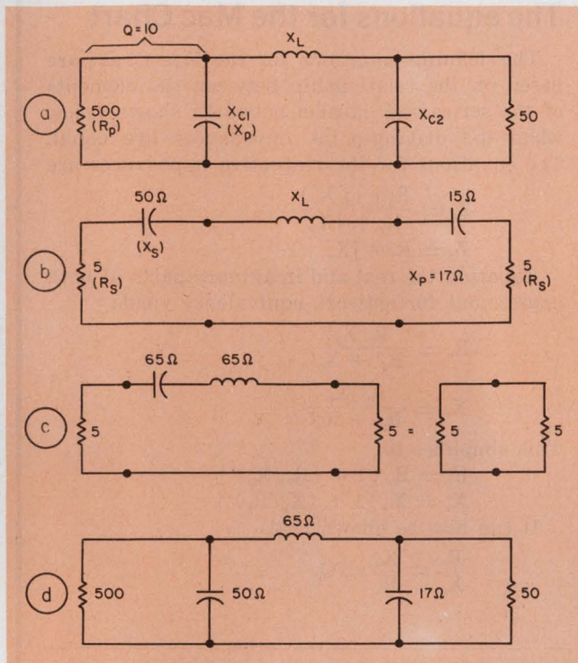
2. A \pi -network problem is solved with two parallel-to-series transformations (b, c). The value of inductive reactance is chosen to cancel the capacitive reactance. Just two resistance values and the circuit Q constitute the initial design data (a).
