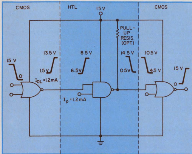
5. CMOS-to-high-threshold-logic interfaces require only a direct connection, since sufficient drive currents are obtained with supplies of 12 V or more. Noise margins are 4 to 5 V.
