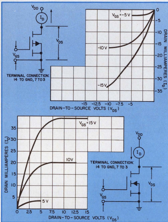
2. Typical drain characteristics for a p-channel (above) and n-channel (below) device—the transistors in the basic CMOS inverter. The current-limiting nature of the nonlinear, I_D vs V_{DS} curves results in a degree of short-circuit protection.
