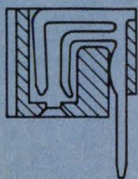
Cross section of bottom entry connector.
