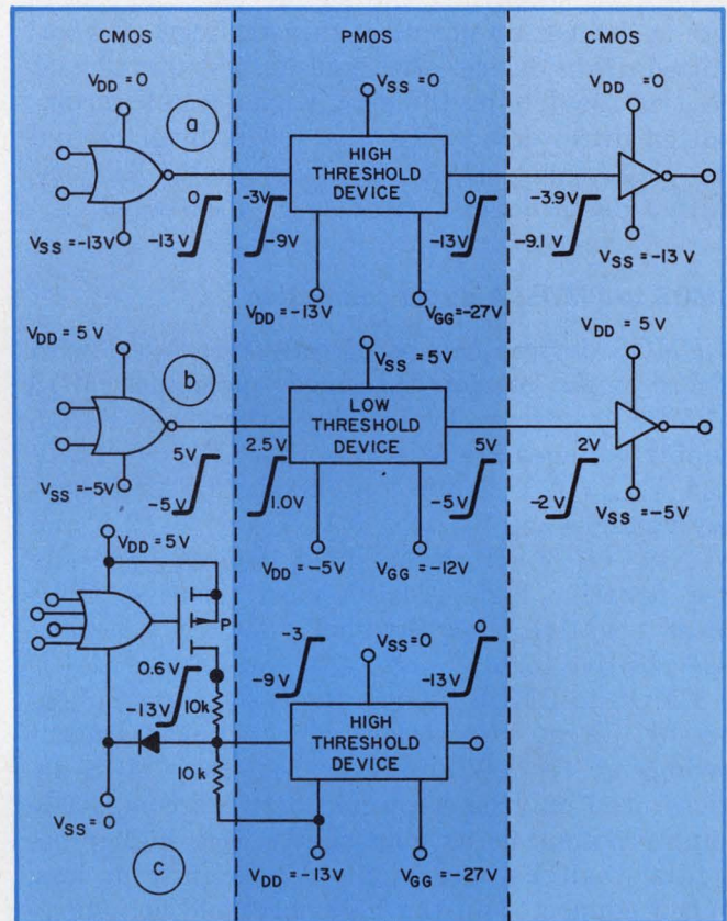
3. The CMOS-PMOS interface can be accomplished by a direct connection, since typical output swings go from V_{SS} to V_{DD} (a and b). When interfacing positive-logic, positive-supply CMOS with negative-logic, negative-supply PMOS, the configuration in c can be used.
