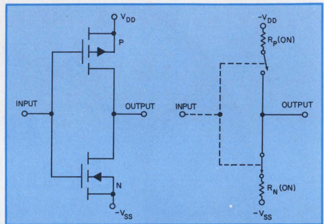
1. The basic CMOS circuit element is composed of a CMOS inverter (left) with its equivalent circuit (right). In SCL devices output signals are driven off the chip with just such an inverter for higher sinking currents. Output impedance—the ON-channel resistance—is typically 500 \Omega for either a HIGH or LOW output.
