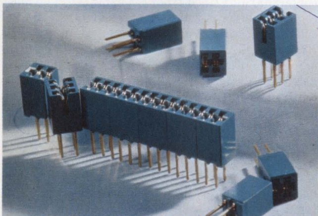
The modularity of Elco's Series 6308/6318 allows a user to join individual sections together to form almost any size of card-edge connector.
