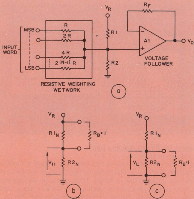
1. Resistive divider, interposed between binary weighting network, allows d/a conversion with outputs that lie between two specified limits (a). The circuit model for calculation of R_1 and R_2 places the binary network across R_1 at maximum output (b) and across R_2 at minimum output (c).
