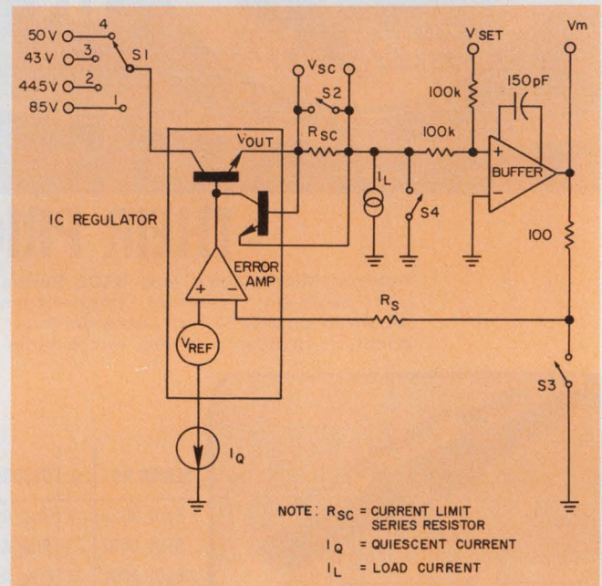
1. General-purpose test circuit for IC voltage regulators is similar to that used to check op-amps. Regulator parameters are measured at the error amplifier input.
