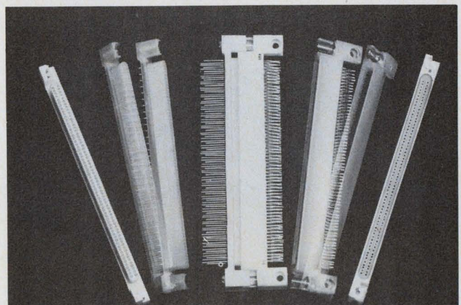
Keyed slots at the ends of the housing prevent incorrect mating of the two halves of this Malco pin-and-socket connector.
