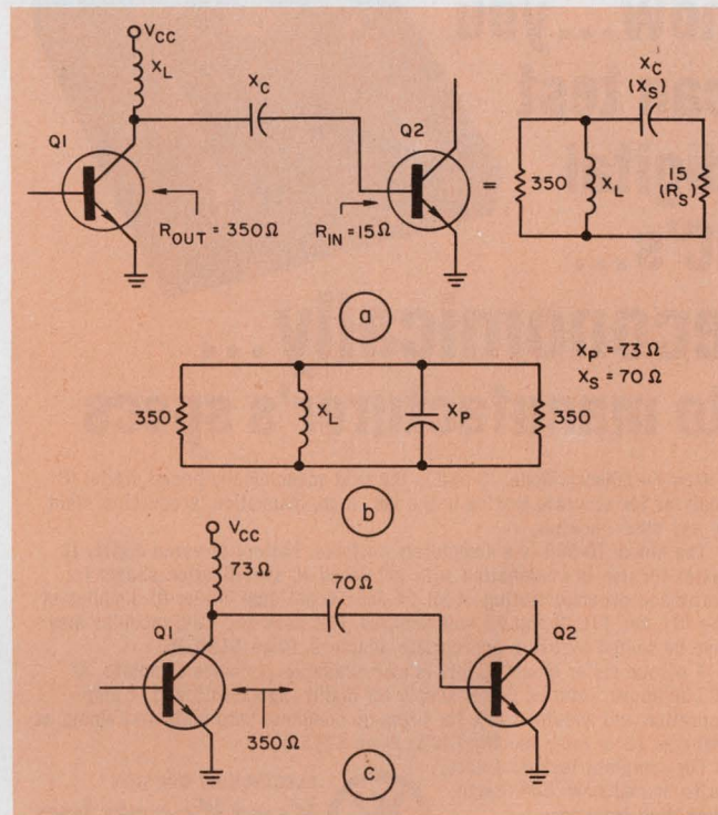
3. A series-to-parallel conversion solves the interstage coupling problem (a) for X_L and X_c . The inductive reactance is made equal to the equivalent parallel capacitor reactance of X_c . No additional transformations are required to determine the value for X_L .
