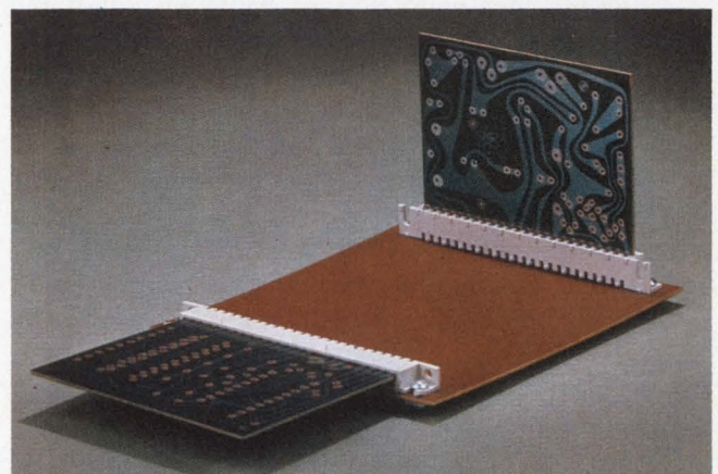
With solder tails, either straight or right-angled, these units from AMP allow daughter boards to be mounted parallel to or perpendicular to a mother board.
