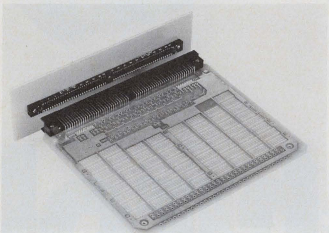
A two-piece connector from Robinson-Nugent is shown here used with a circuit board for DIP ICs.
