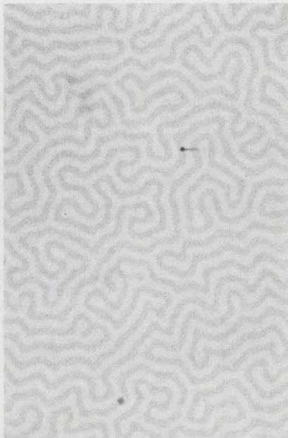
Experimental shift-register configuration (left) uses amorphous film sputtered onto a glass substrate. Magnetic stripe domains (right) are clearly visible when viewed with polarized light.
