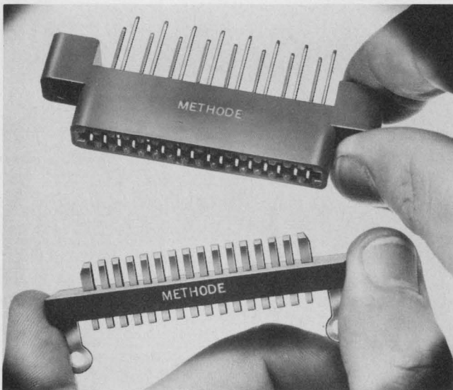
Blade-and-tuning-fork two-piece connector from Methode comes with single-readout, wrapped-wire tails in two staggered rows for easy tool access.
