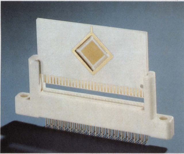
An edgemount connector from Cinch is specially designed for ceramic LSI substrates.
