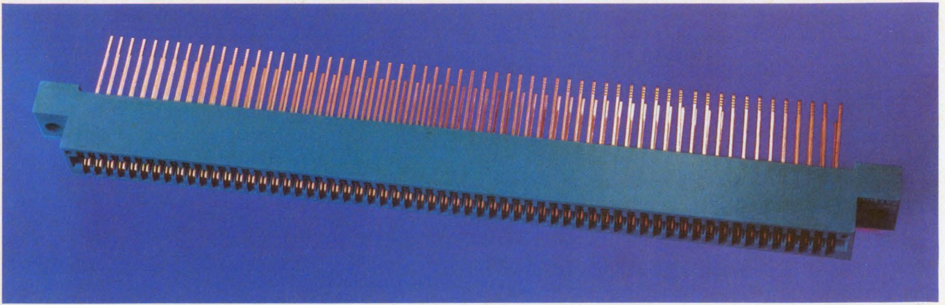
Bifurcated contacts are housed in a diallyl phthalate molded body in this Augat unit.
