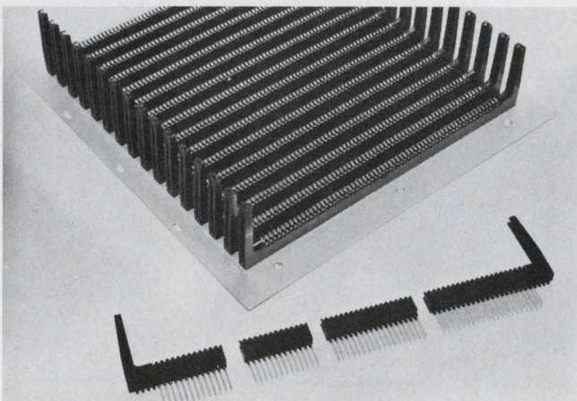
Built-in card guides and modularity are features of these metal-backplane, card-edge connectors from Fabri-Tek.
