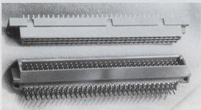
Square pins and sockets appear in three rows in Amphenol's Series 128.
