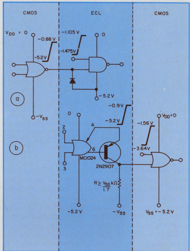
6. For higher-speed operation in a CMOS-to-ECL interface, connect the CMOS V_{SS} terminal to any supply from -5 to -15 V and diode-clamp the ECL gate input (a). Going from ECL to CMOS requires level shifting (b).
