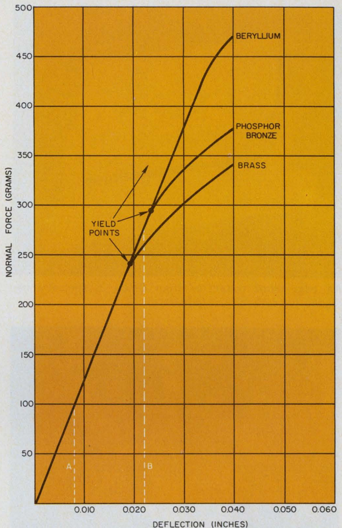
3. Theoretical curves show the normal force developed for cantilever-beam contacts as a function of contact deflection. Beyond its yield point, each material deforms permanently. Curves are based on advertised yield points of the materials. For a 62-mil nominal board, line A represents the deflection for a minimum-thick board (54 mils) with maximum contact gap (38 mils) and line B represents deflection for a maximum-thick board (70 mils) with minimum gap (26 mils). Curves are for contacts designed for a minimum of 100-grams normal force and a spring rate of 12.5 g/mil. (Courtesy of Marvin Yeager and Leon Ritchie of AMP Inc.)
