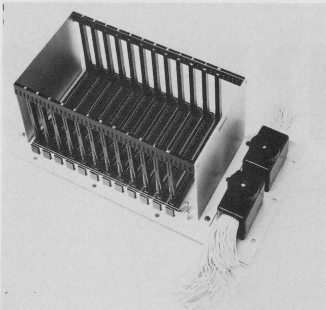
Card-edge connectors from Teradyne Components can be pressure fitted into a metal backplane. The units come with bifurcated contacts and detachable card guides.
