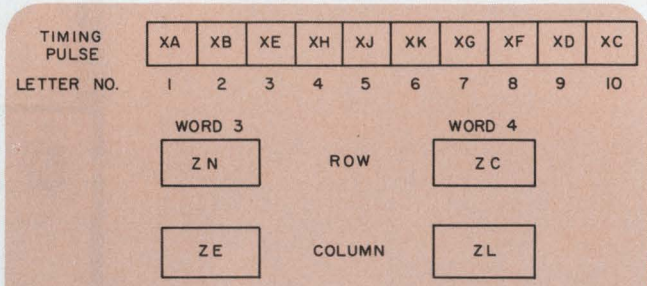
2. Sequence of 10 timing pulses on pins XA through XC selects the position in which a character is displayed. Current levels, applied by a timing pulse to control lines ZN and ZE or ZC and ZL, select the character to be displayed on the scope-face readouts.
