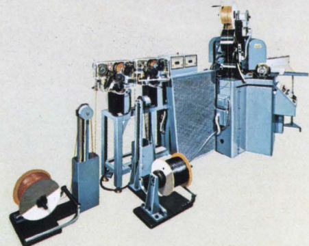
AMPOMATOR machine with miniature applicator can produce up to 5700 doubly-terminated leads an hour.
