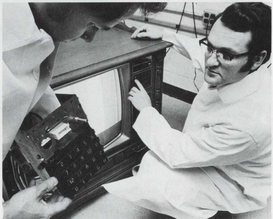
ICs and discrete solid-state components are taking over in color television sets like this GTE Sylvania receiver. Here, engineers check the varactor tuning.
