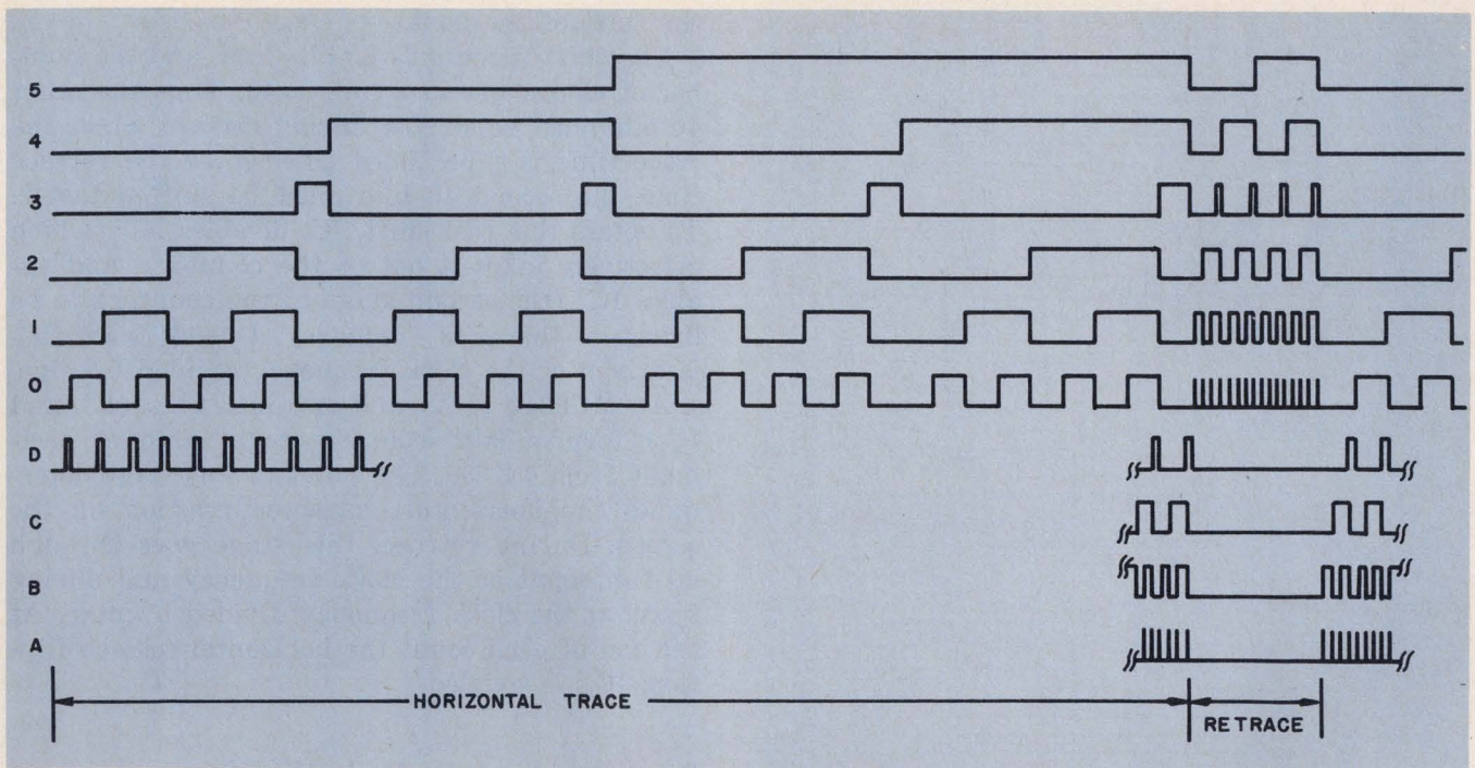
4. During trace, 40 characters per line can be shifted out of the 80-bit registers. The remaining 40 bits must
