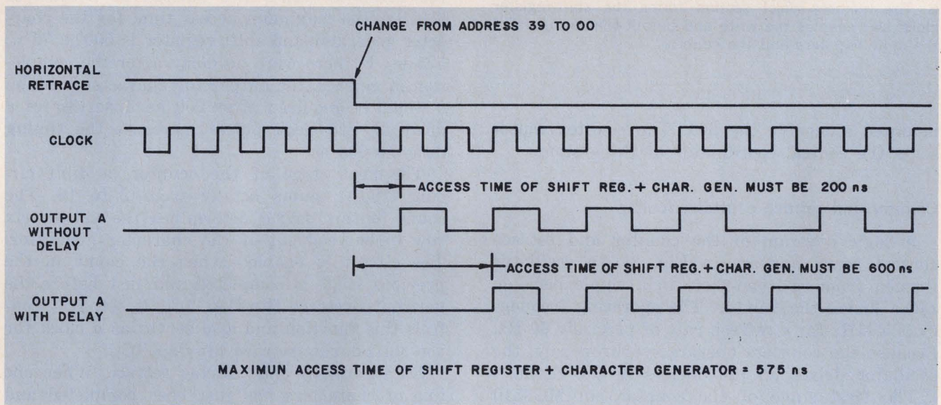
5. Character codes shift at a 5-MHz rate during retrace. A delay must be added after retrace to ensure sufficient
