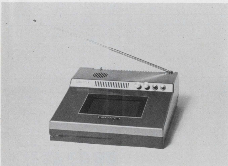
Prototype dc plasma-panel TV from Sony consumes 90 W of power—10 W for the panel and drivers and 80 W for the rest of the electronics.
