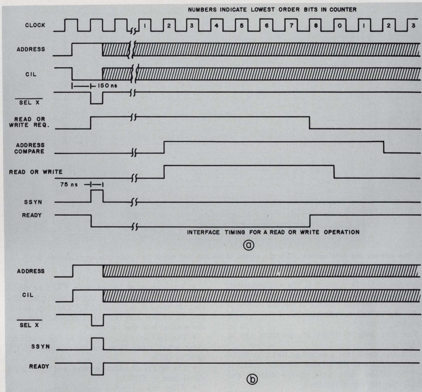
9. A write sequence commences with the application of the address and data to the system input lines (a). To
