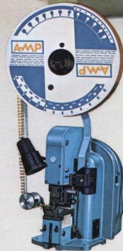
AMP-O-MATIC stripper/crimper machine strips wire and attaches contact during each machine cycle—at rates up to 1500 an hour.
