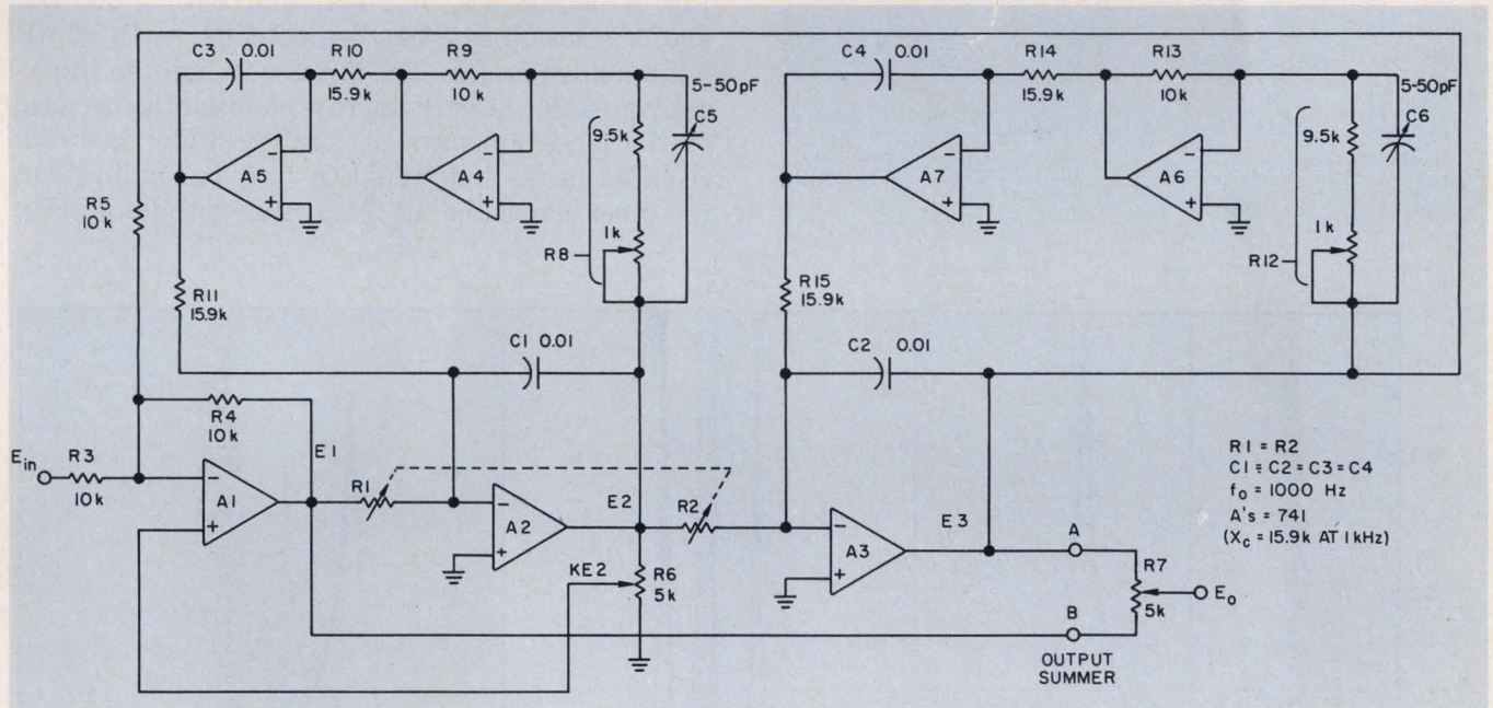
7. A working version of the biquartic filter can be built with the circuit shown here. Though it uses seven op
