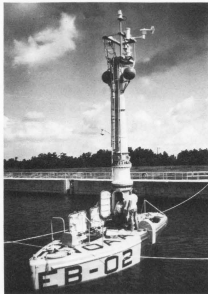
This new prototype, 30-ton buoy, built by Lockheed Missile & Space Company for the National Oceanic and Atmospheric Administration, has been placed in the Gulf of Mexico to record meteorological and oceanographic data. It is equipped with a Rolm Ruggednova for data acquisition and communications processing.
