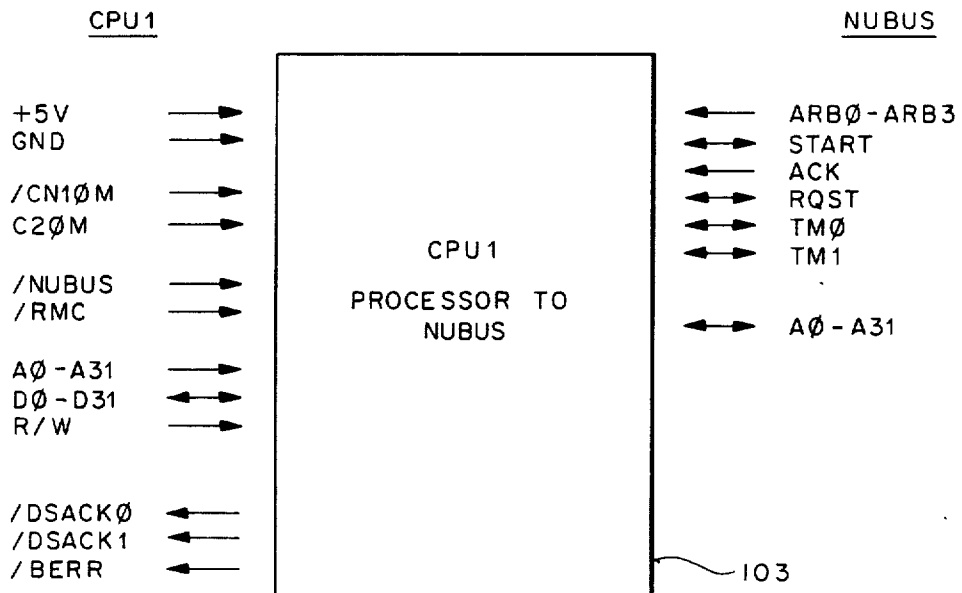
FIG 8 PROCESSOR TO NUBUS BLOCK DIAGRAM
