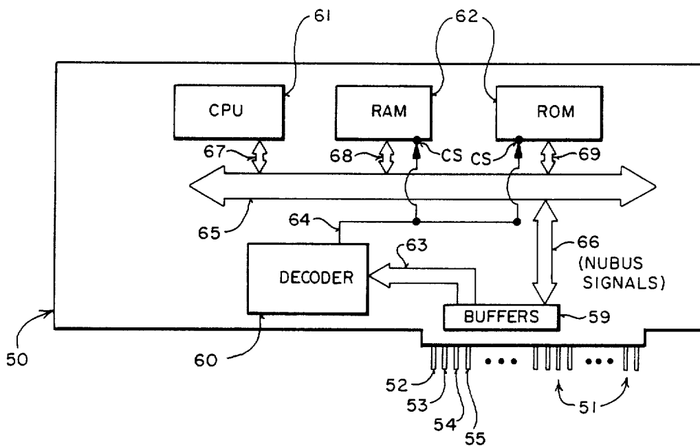
FIG 5 NUBUS INTERFACE BLOCK DIAGRAM
