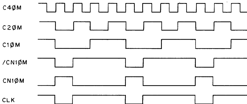
FIG 7 PHASE RELATIONSHIP OF NUBUS CLOCKS
