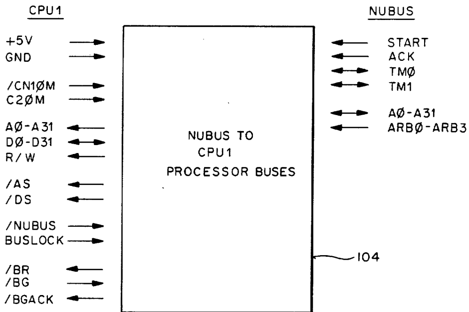
FIG 9 NUBUS TO PROCESSOR BUS BLOCK DIAGRAM
