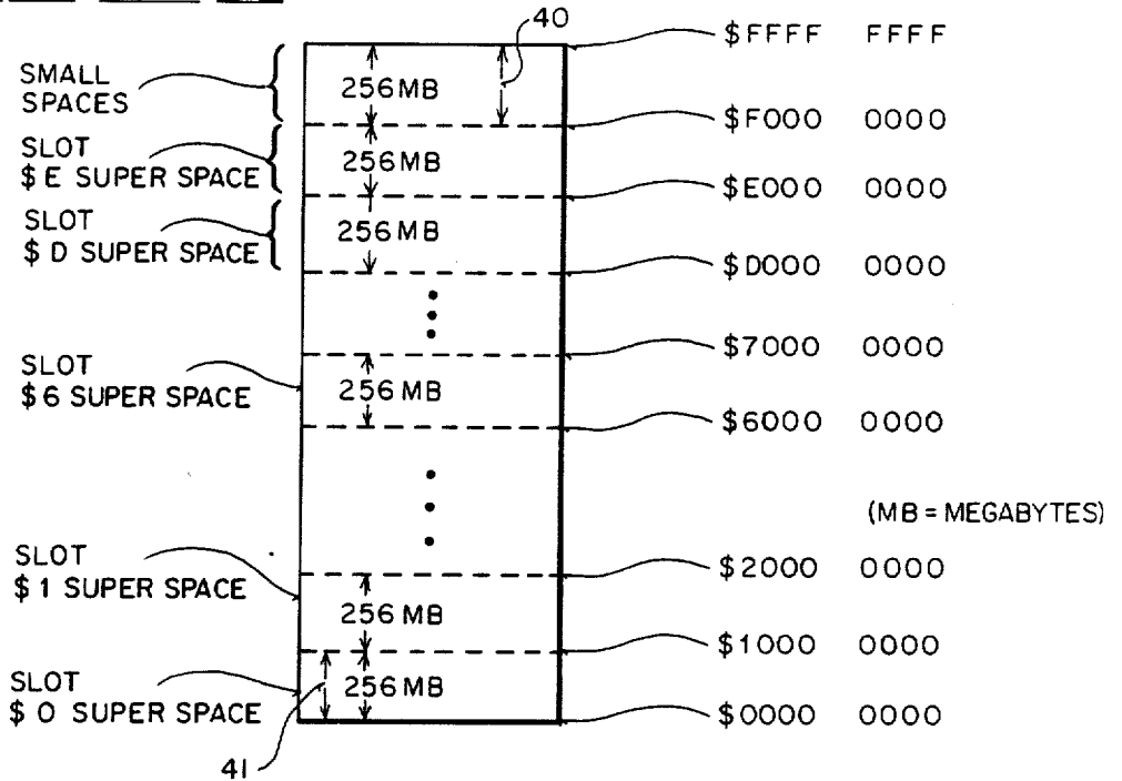
FIG 2 PHYSICAL ADDRESS MEMORY SPACE
