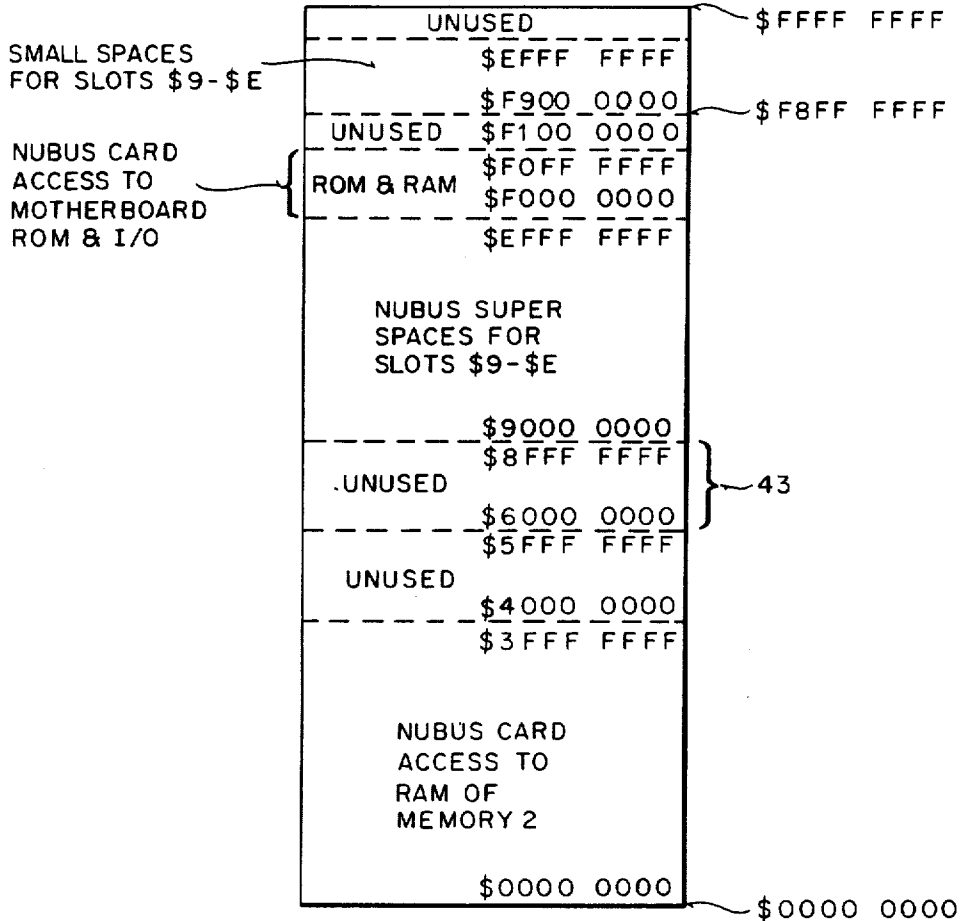
FIG 10 ADDRESS MEMORY SPACE FOR NUBUS CARD
