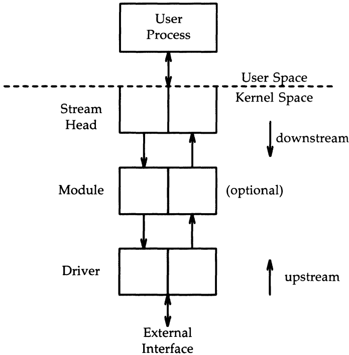
Figure 2-1: Basic Stream
