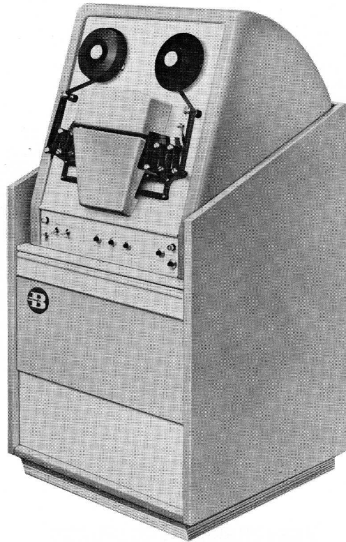
Figure 2-1. Paper-Tape Photoreader.
