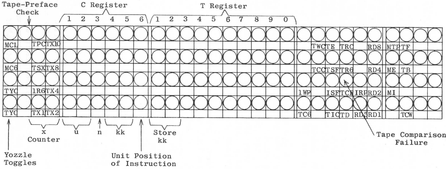
Figure 2-13. Magnetic-Tape Control Unit Control Panel.
