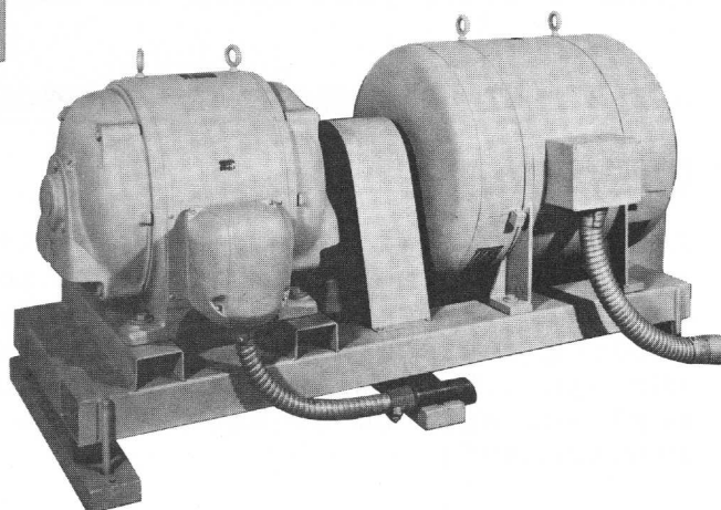
Figure 3-15. Motor Alternator.
