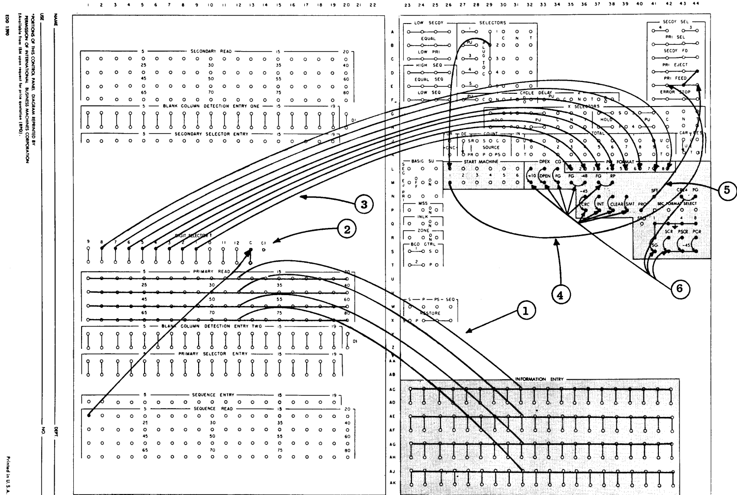
Figure 2-25. Basic 87 Control-Panel Wiring.
