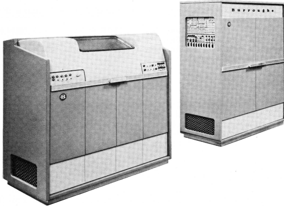
Figure 2-28. BURROUGHS 220 High-Speed Printer System.
