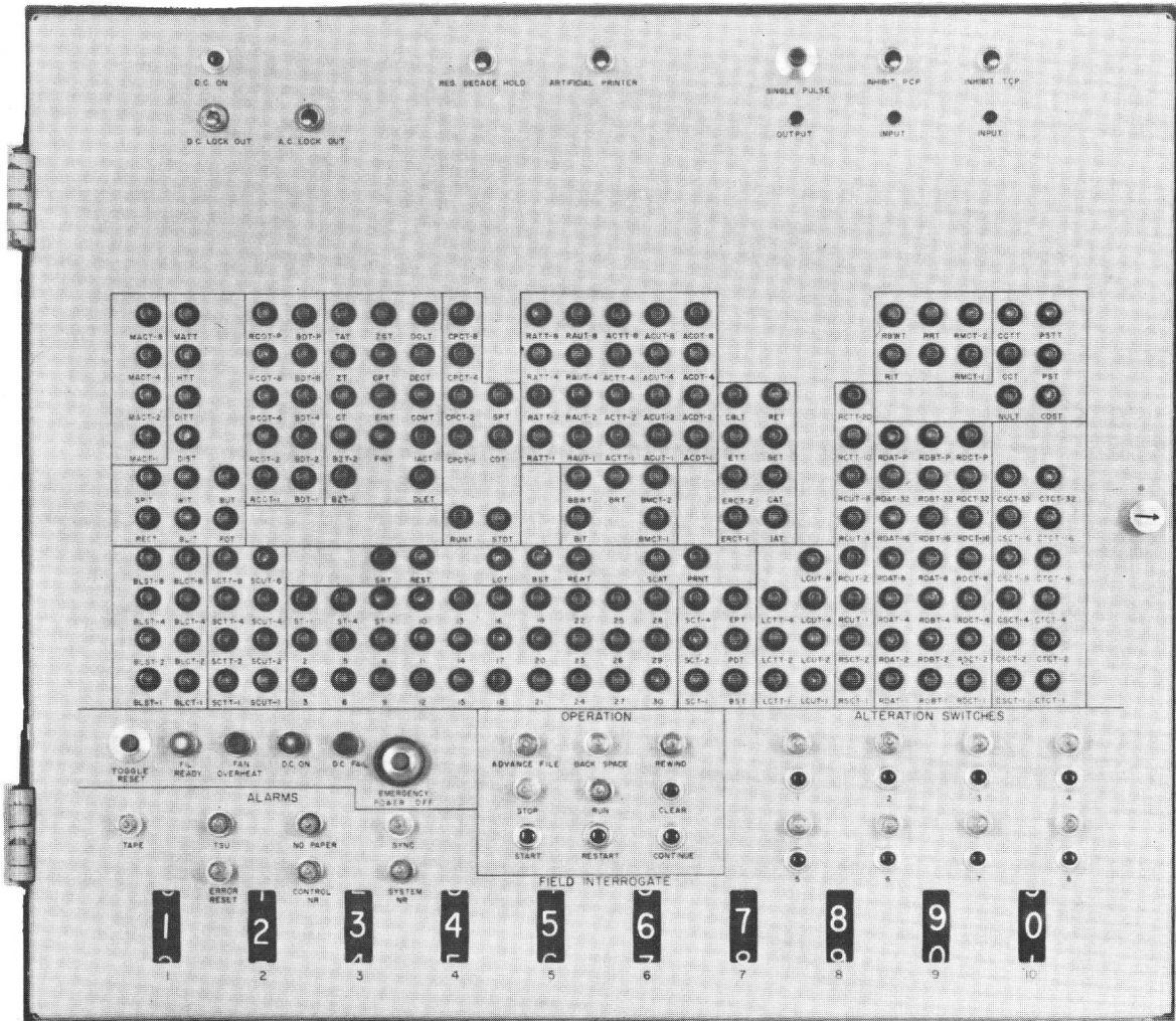
Figure 2-29. High-Speed Printer Control Unit, Operator's Panel.
