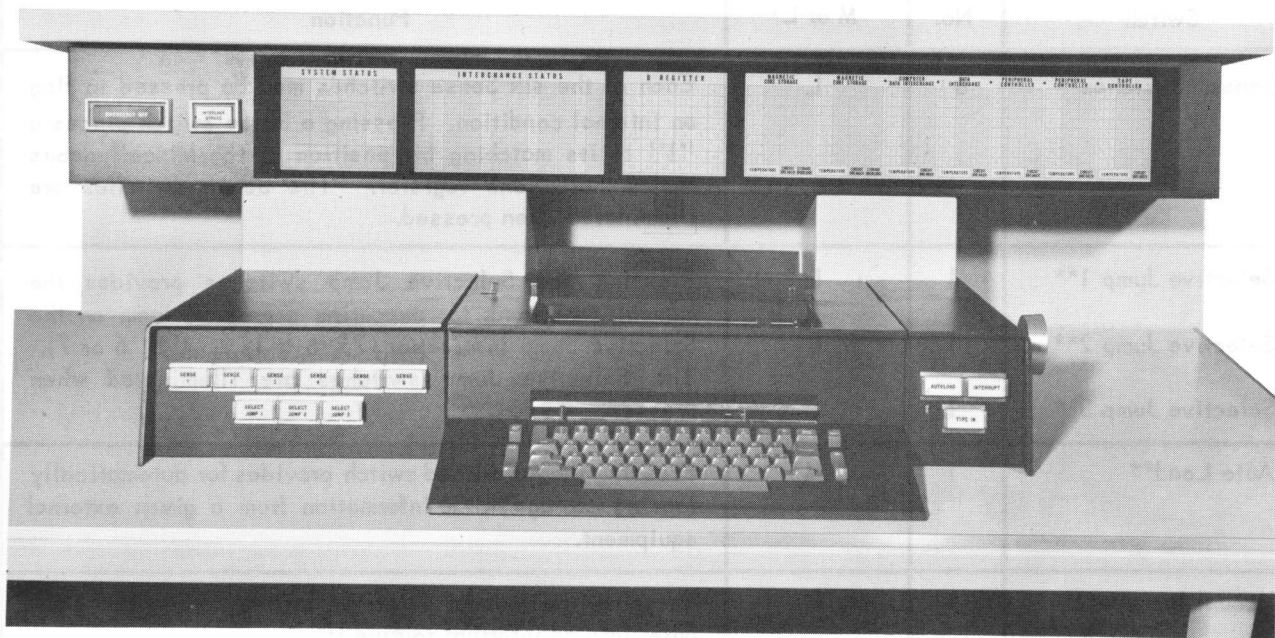
Figure 7-4. Console Typewriter
