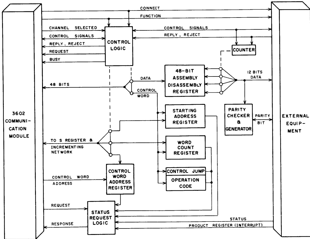
Figure 5-3. 3606 Data Channel
