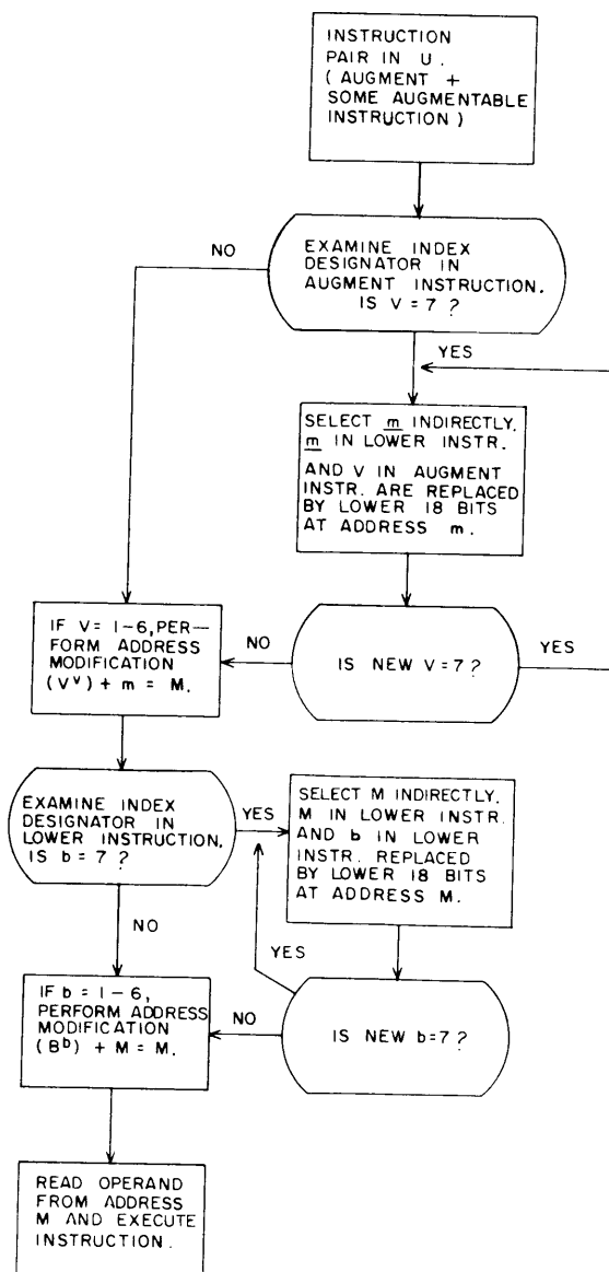
Figure 3-1. Indirect Addressing
