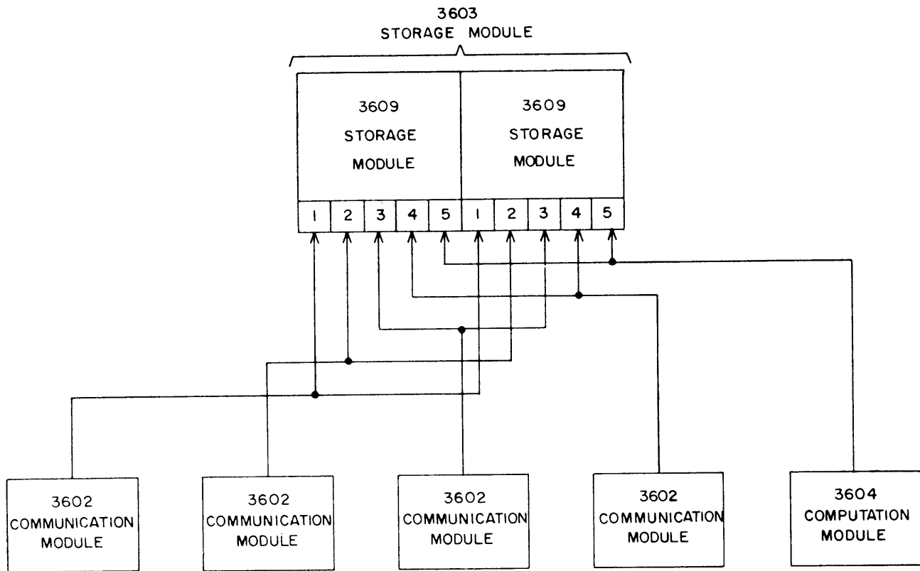
Figure 2-1. Typical Storage Access Channel Hook-up
