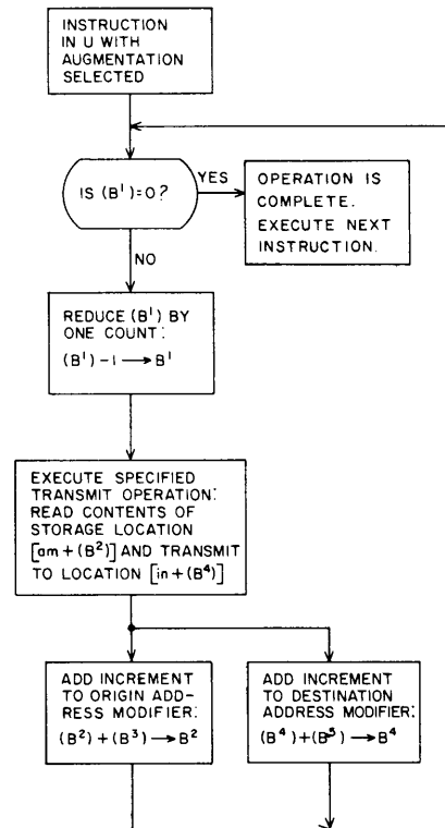
Figure 3-2. Augmented Transmit Operation.
