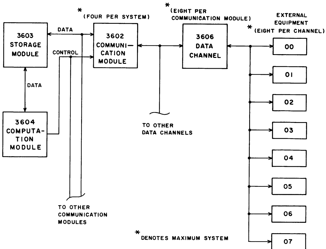
Figure 5-1. 3600 System
