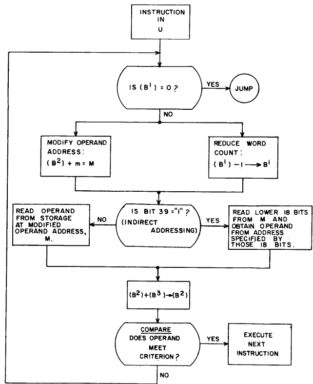
Figure 3-3. Sequencing for 63.4 Search Operations
