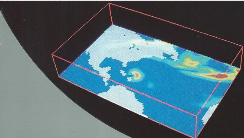
Wind speeds of Hurricane Hugo. Shaded image with false color map depicts high (red) and low (blue) wind speeds two days before landfall in South Carolina. Code: SPM. Data courtesy of Tony Meys and Anders Grimsrud, Cray Research, Inc., in association with European Center for Medium Range Weather Forecasting (ECMWF).
