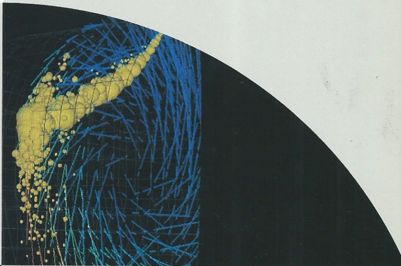
Fuel injection and droplet impingement on the wall of a diesel pre-chamber. The lines show air velocity vectors. Code: CRI/TurboKiva. Data courtesy of Reza Taghavi, Cray Research, Inc.
