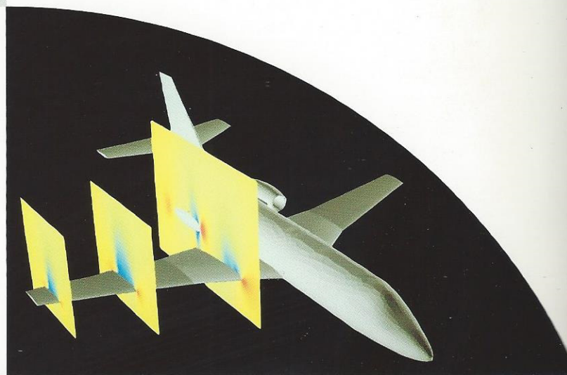
AMD/BA Falcon aircraft pressure contours. The pressure coefficient distribution is shown in clipping planes. Data courtesy of J. Peiro, Jaime Peraire and K. Morgan, Imperial College of Science, Technology and Medicine.
