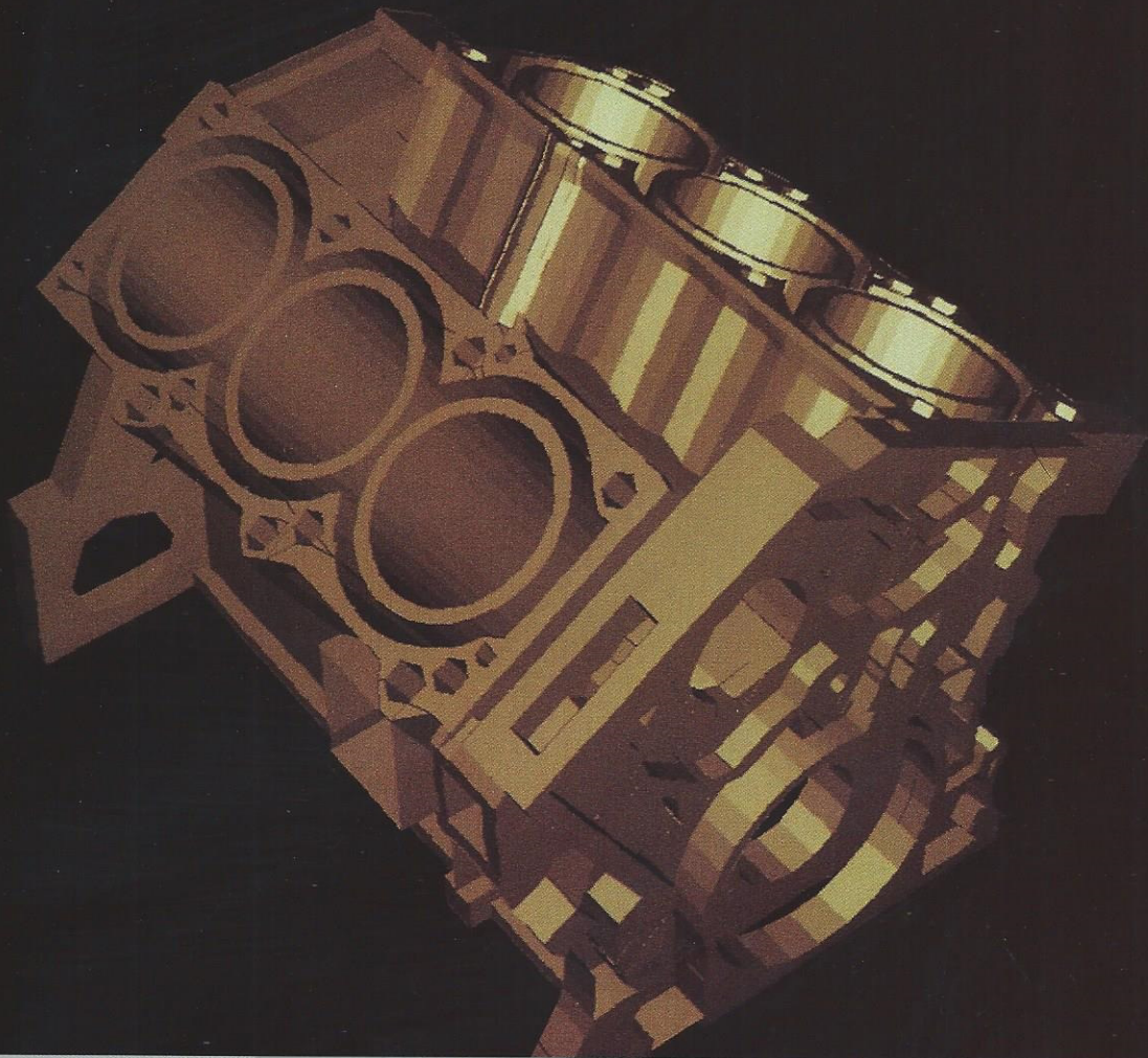
Engine block depicted with shaded images. Code: MSC/NASTRAN. Data courtesy of General Motors Corporation.
