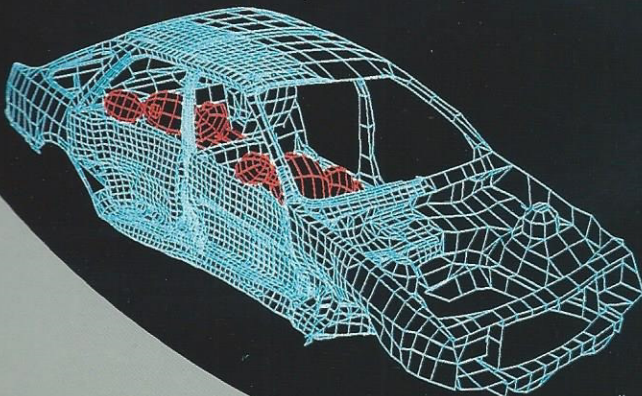
Side impact with crash dummies. Image depicts automobile and passengers in a side collision. Code: RADIOSS. Data courtesy of Ford Motor Company, United Kingdom.
