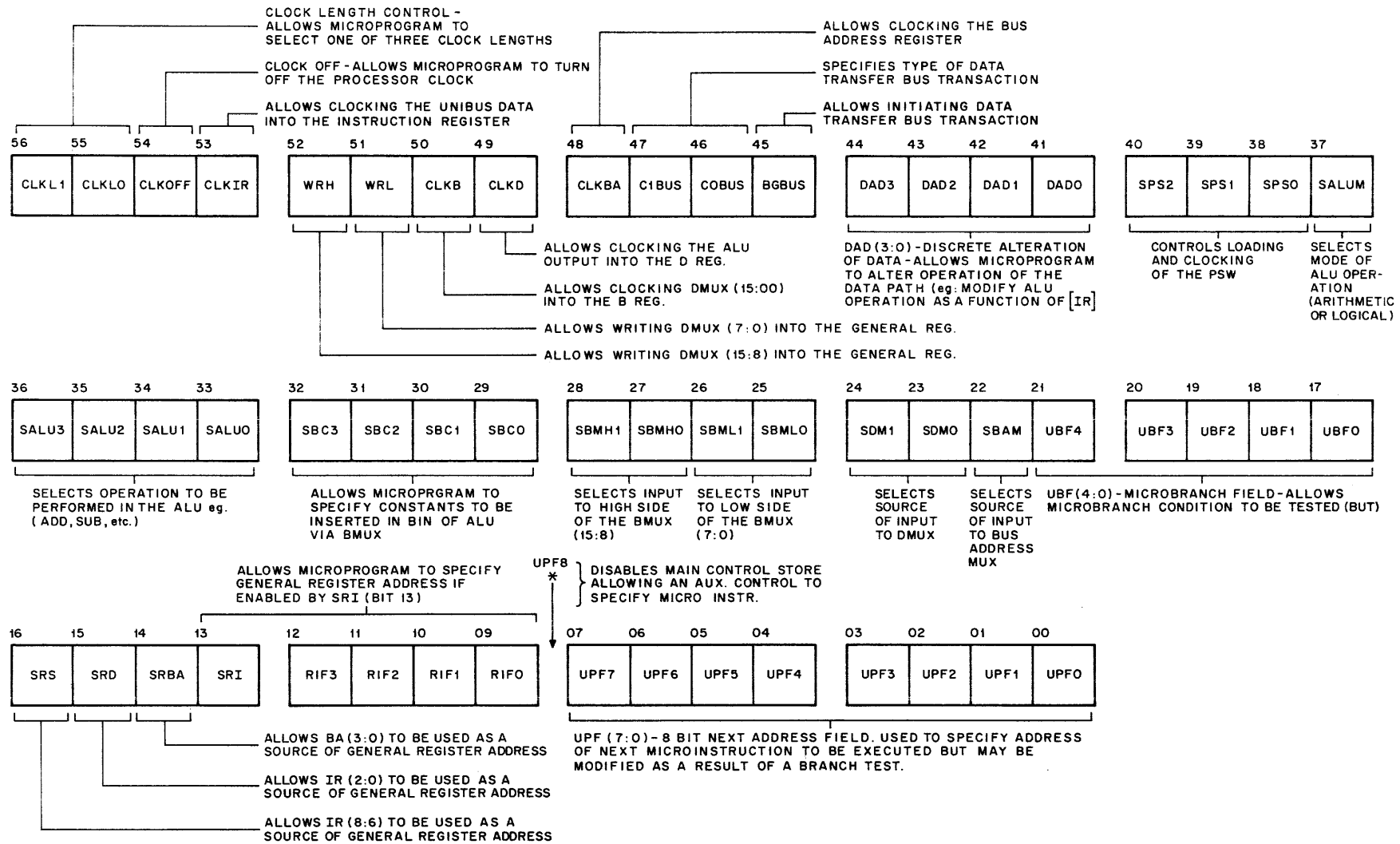
Figure 4-3 KD11-A ROM Format
