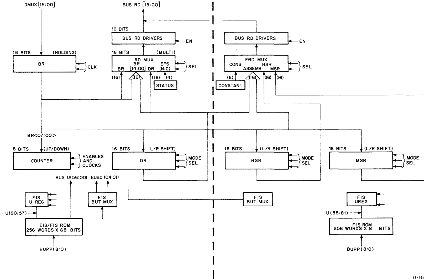
Figure 4-1 EIS/FIS Functional Block Diagram
