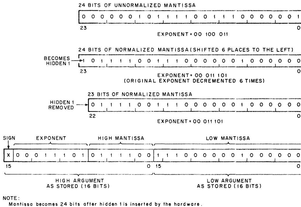
Figure 3-5 Floating-Point Representation
