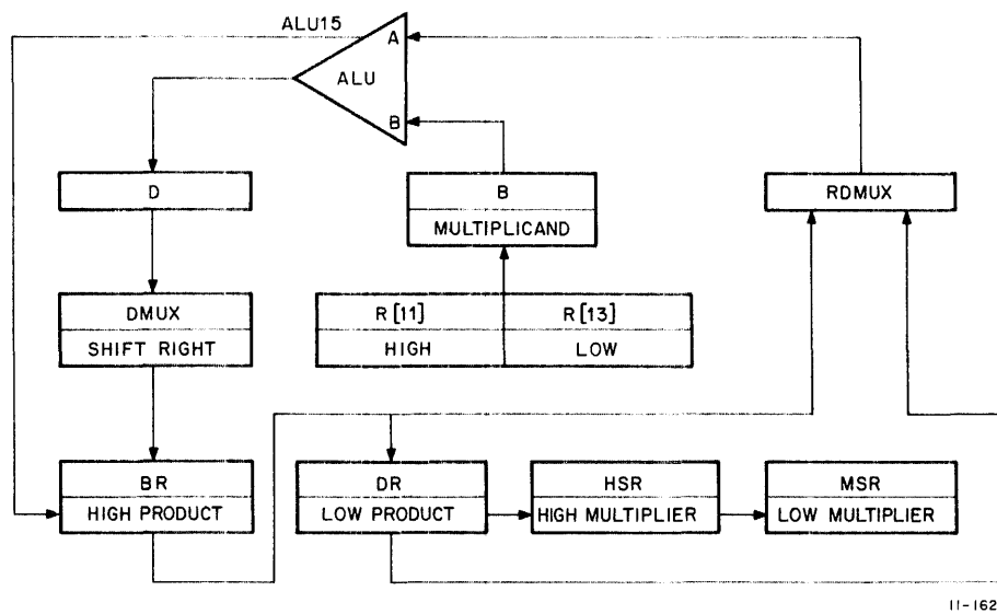
Figure 4-12 FMUL Flow, Block Diagram
