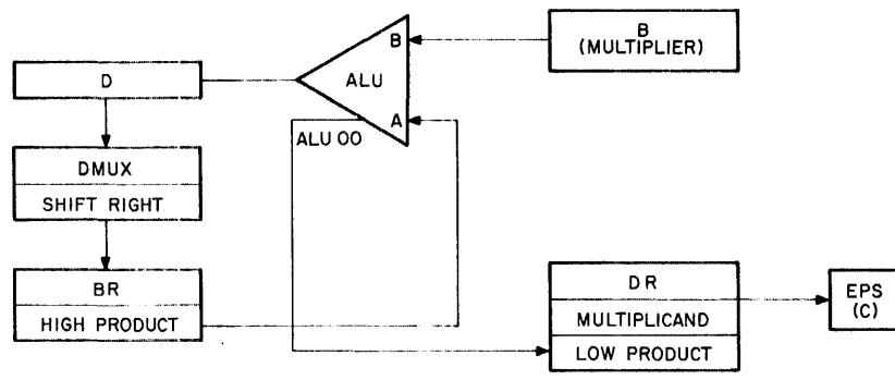
Figure 4-9 MUL Flow, Block Diagram
