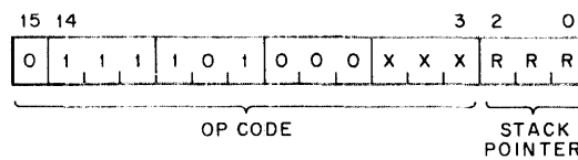
Figure 2-6 FIS Instruction Format
