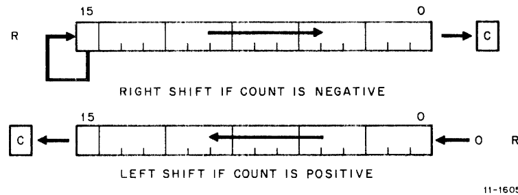
Figure 2-3 ASH Operation
