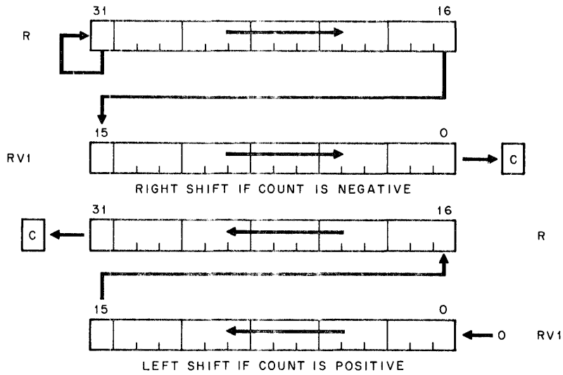
Figure 2-4 ASHC Operation
