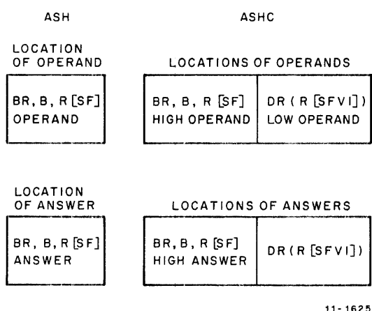
Figure 4-8 ASH and ASHC Locations of Operands and Answers
