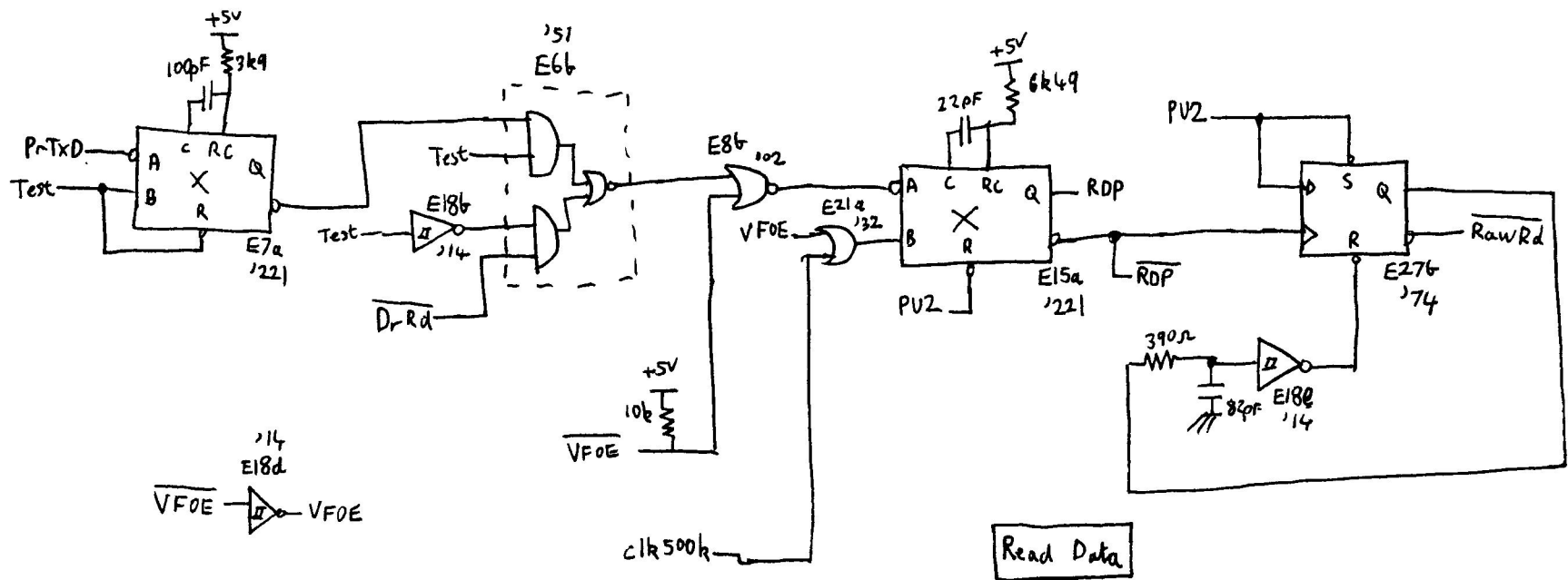
Rainbow Floppy Controller Sheet (4)
