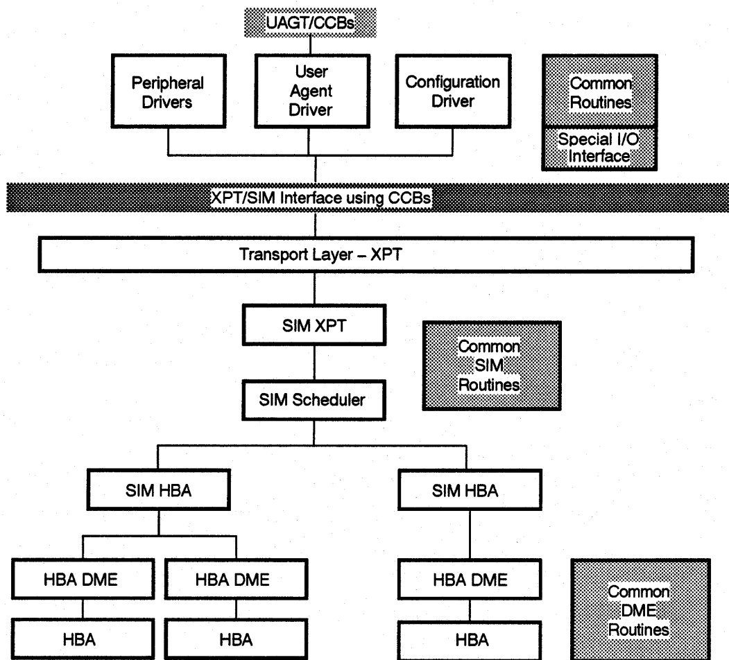
Figure 1-2: ULTRIX SCSI/CAM Architecture Implementation Model
