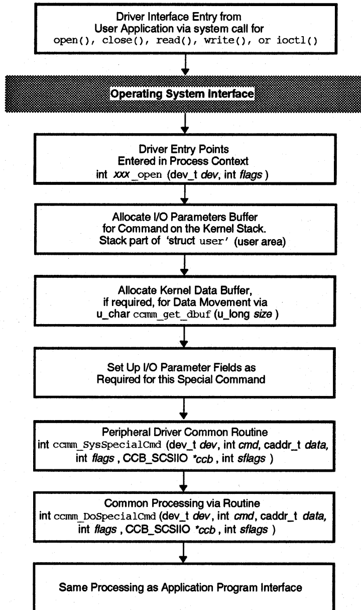
Figure 12-2: Device Driver Flow Through SCSI/CAM Special I/O Interface
