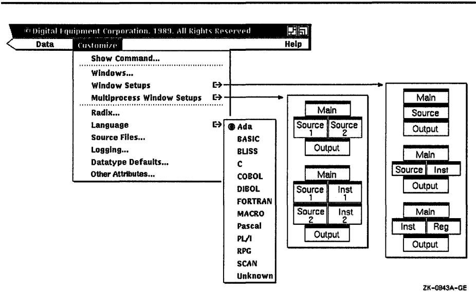
Figure 1-5 Customize Menu and Submenus
