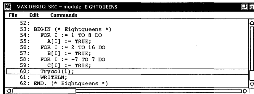
Figure 1–9 Execution Suspended at Line 60
