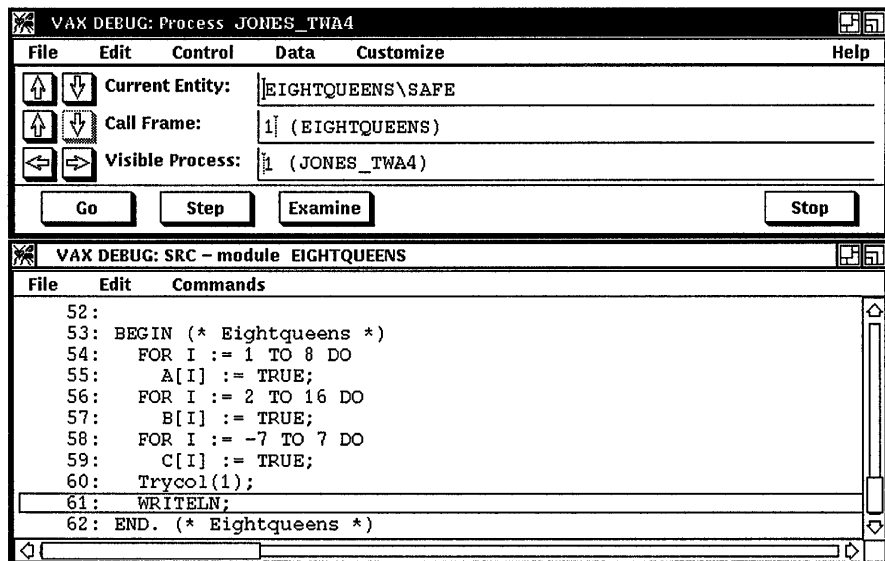
Figure 1–14 Displaying Source Code in the Calling Routine
