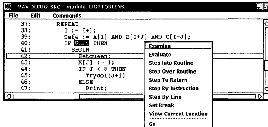
Figure 1-6 Pop-Up Menu Over Source Window
