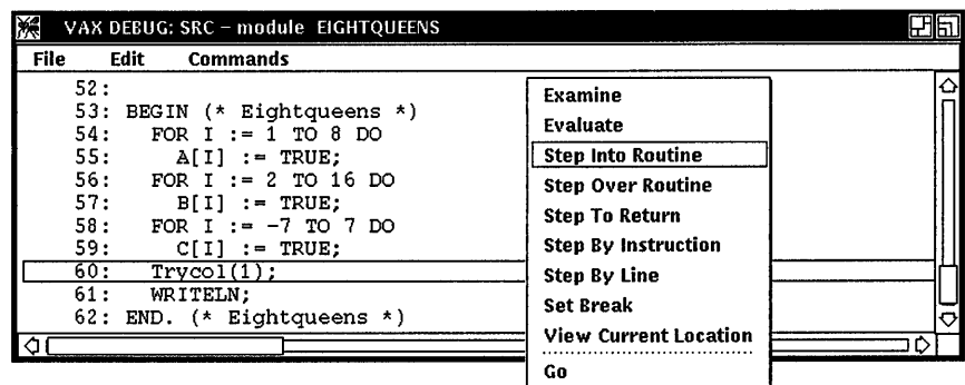
Figure 1-10 Stepping into a Called Routine
