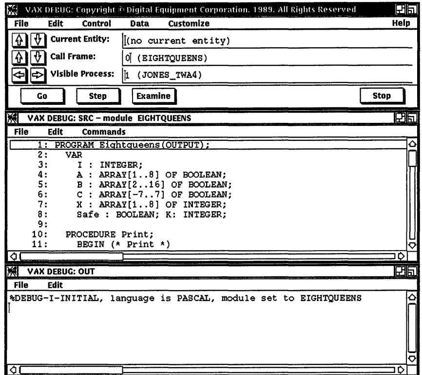
Figure 1-1 Debugger Windows at Startup
