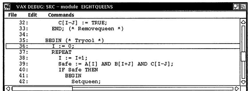
Figure 1-11 Execution Suspended Within the Called Routine
