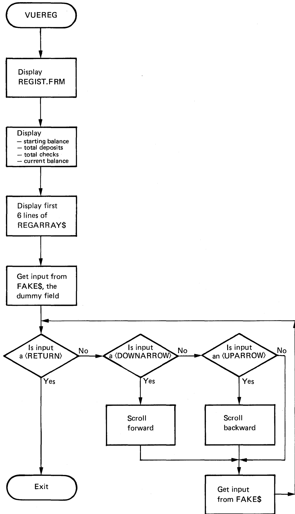
Figure 7-1: Flowchart for the VUERG Subroutine
