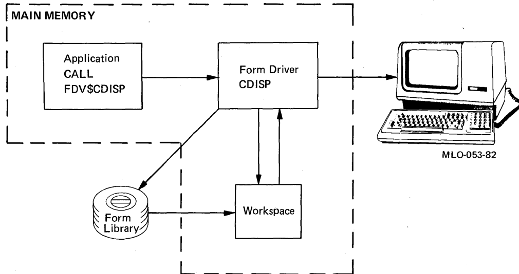
Figure 5-5: Displaying a Form
