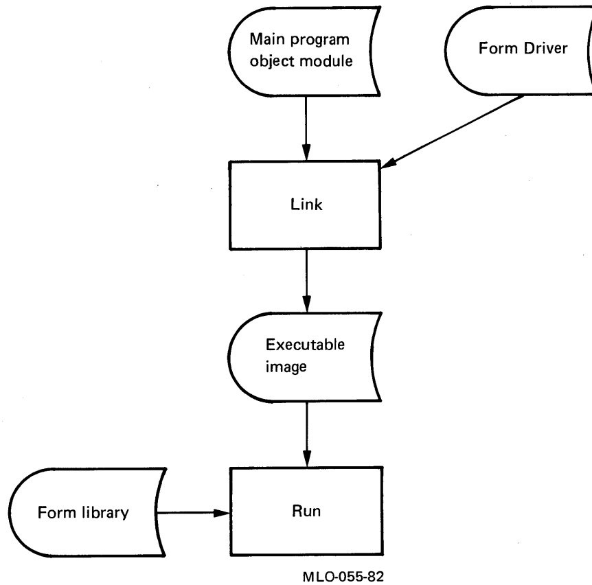
Figure 6-1: FMS Application Development Cycle
