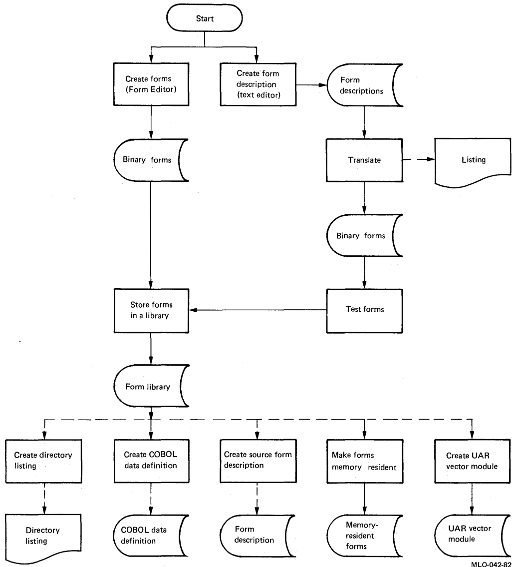
Figure 1-1: Form Development Cycle
