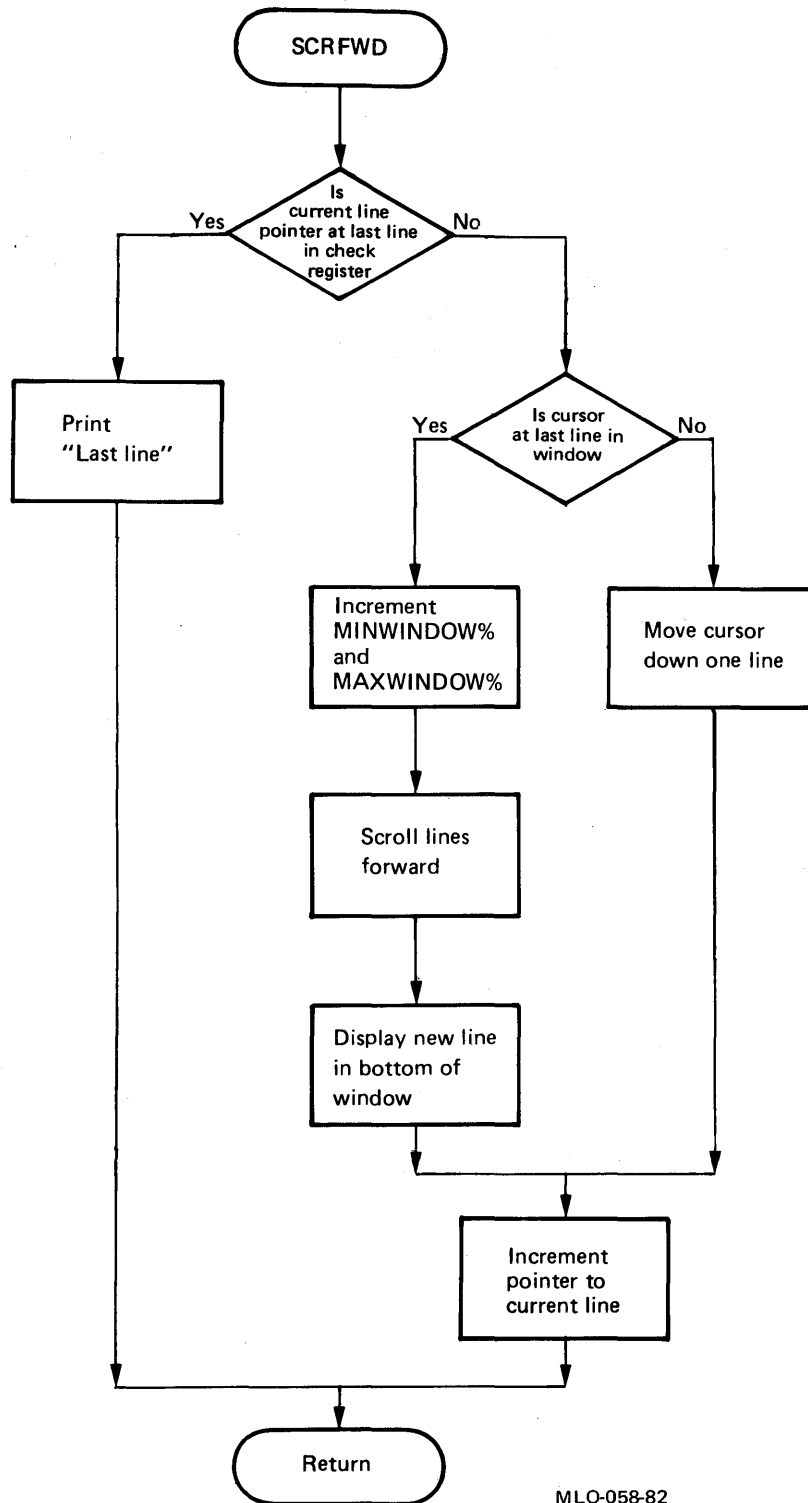
Figure 7-3: Flowchart for the SCRFWD Subroutine
