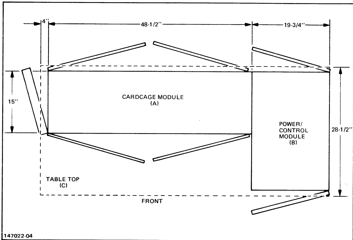
Figure 2-4. Top View
