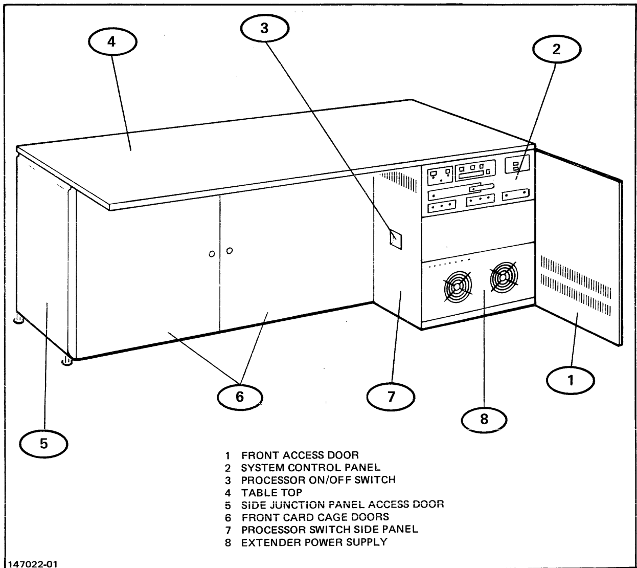
Figure 2-1. Front/Side View
