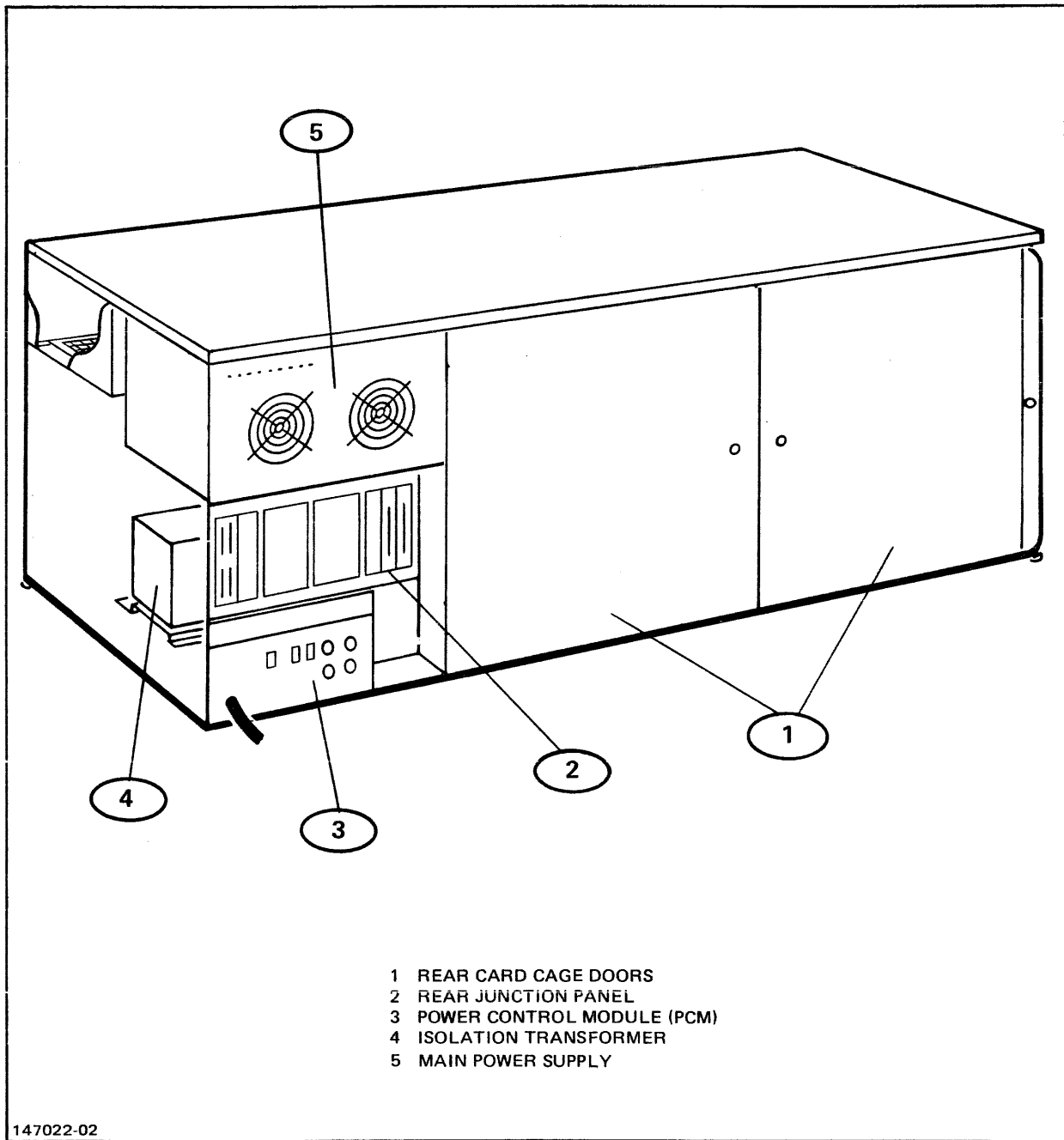
Figure 2-2. Rear View
