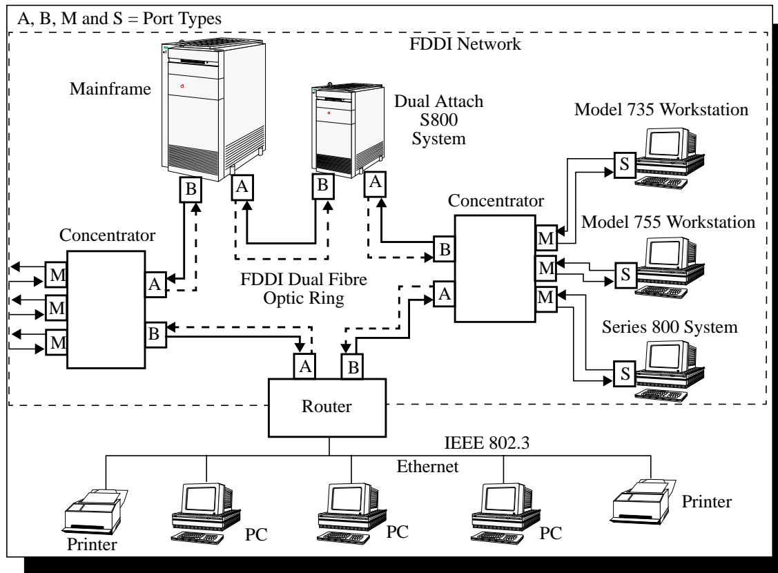
Figure 2 FDDI Network Map
