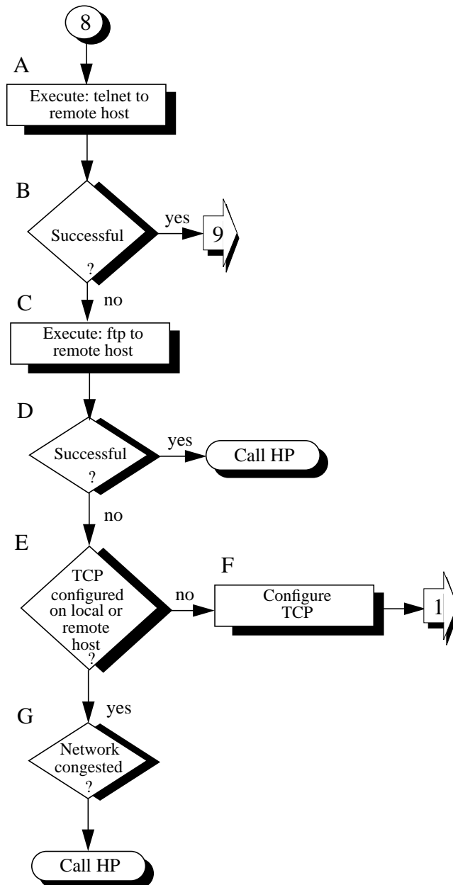
Flowchart 8: Transport Level Loopback Test (using ARPA)
