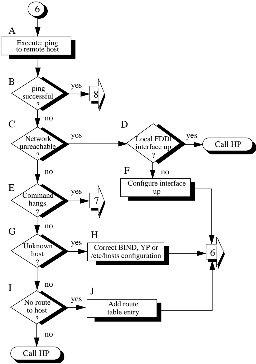
Flowchart 6: Network Level Loopback Test
