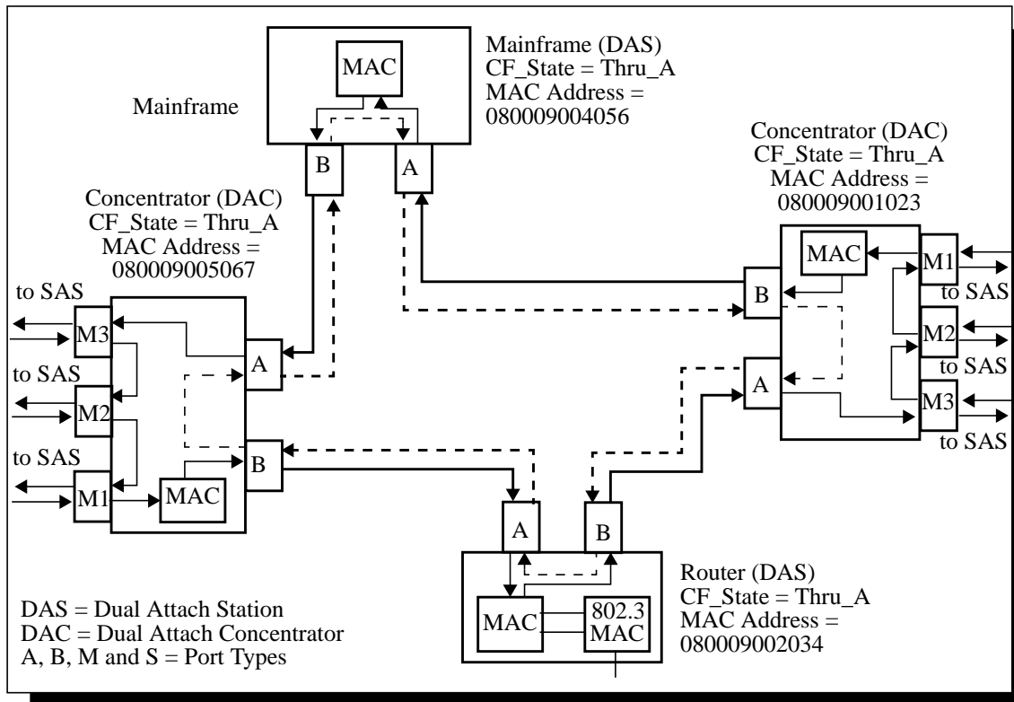
Figure 3 FDDI Dual Ring During Normal Operation
