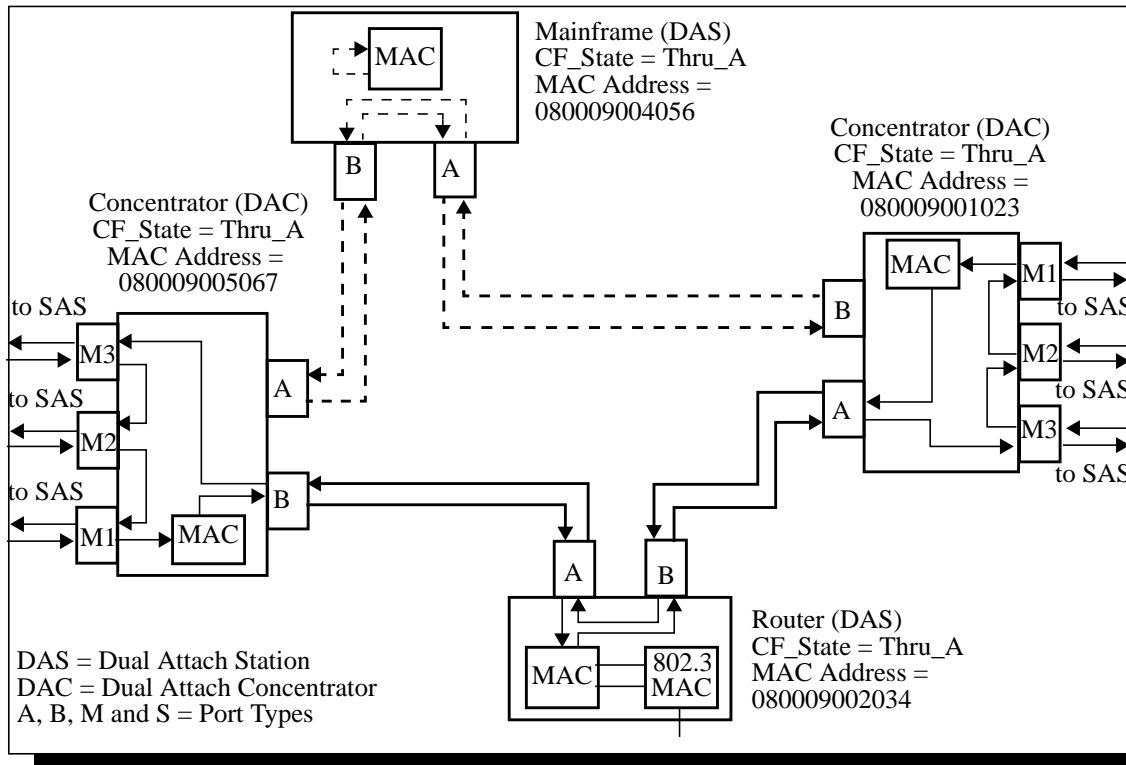
Figure 4 FDDI Dual Ring In Wrap Mode
