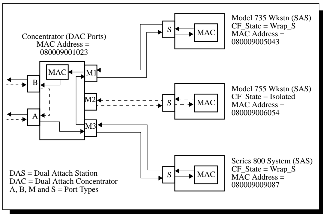
Figure 5 FDDI Single Attached Station When Bypassed
