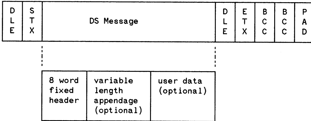
Figure 3-9. Data Format for PRTX or PSTX Entries.
