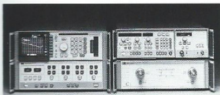
The HP 8510E Network Analyzer is a complete 20-GHz measurement system consisting of the HP 8510B, an s-parameter test set, broadband sweeper, and accessories.
