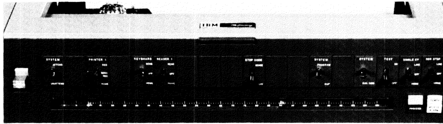
Figure A-2. 1052 switch panel.
