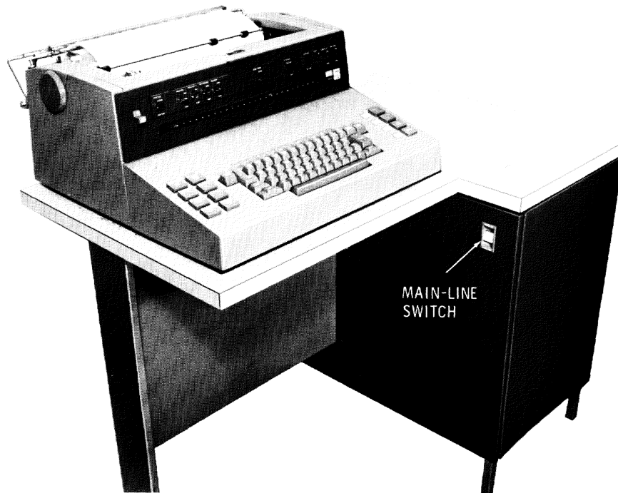
Figure A-1. 1051 Control Unit and 1052 Printer-Keyboard.
