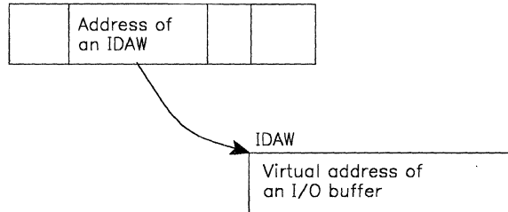
CCW (Format 0)
