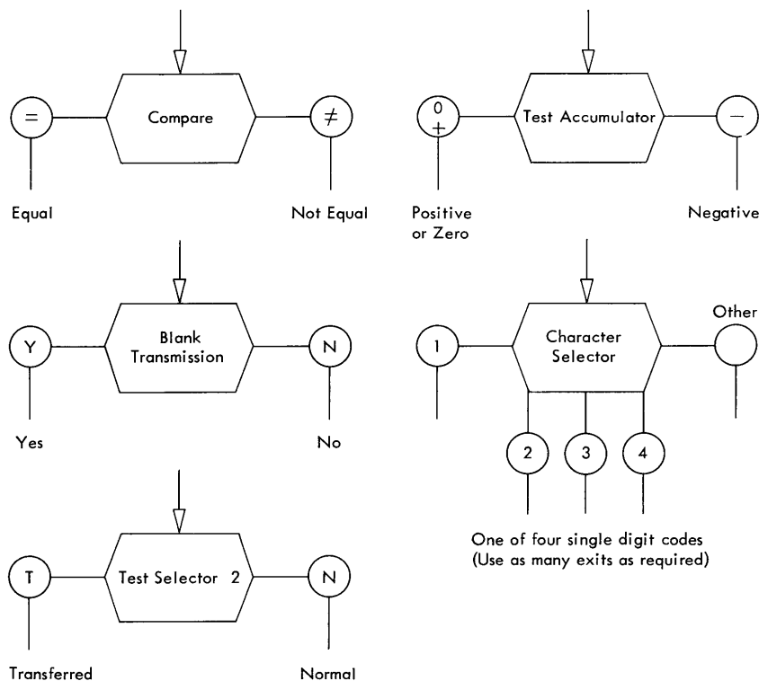
Figure 18. RAMAC Decision Symbols
