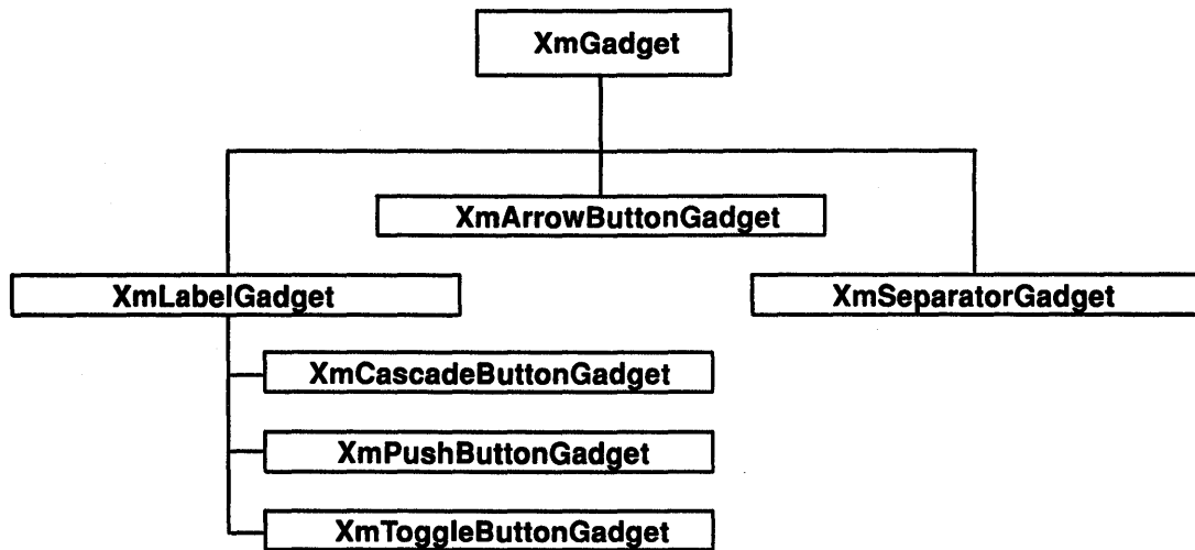
Figure 2. The AIXwindows XmGadget Gadget Class Hierarchy
