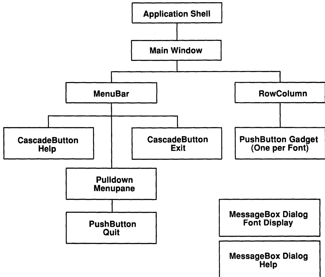
Figure 5. Example of AIX Toolkit Parent-Child Widget Tree
