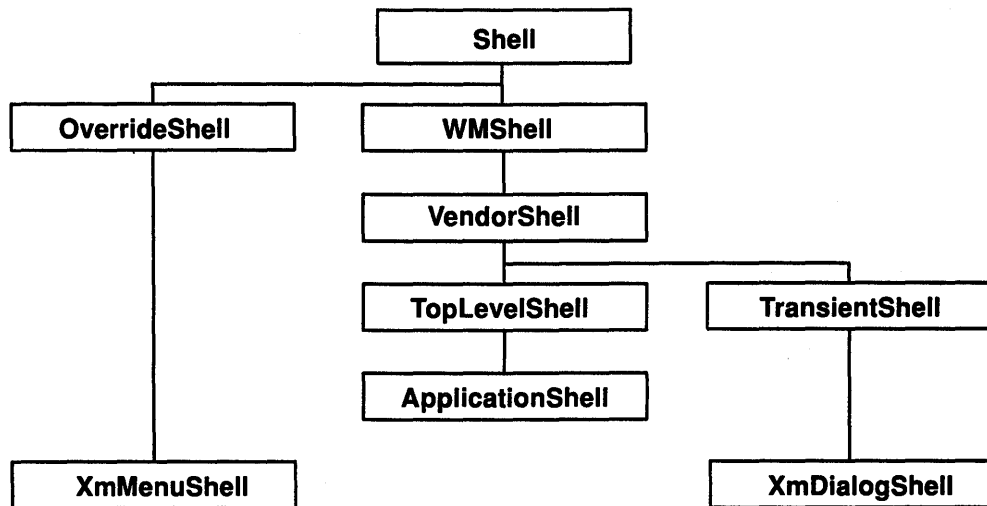
Figure 4. AIXwindows Shell Widget Class Hierarchy
