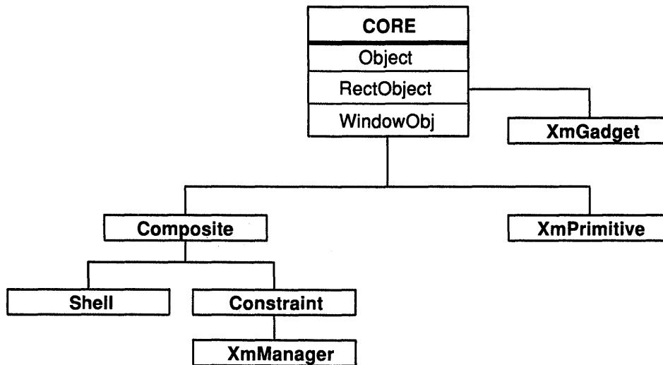
Figure 1. AIXwindows Top-level Class Hierarchy
