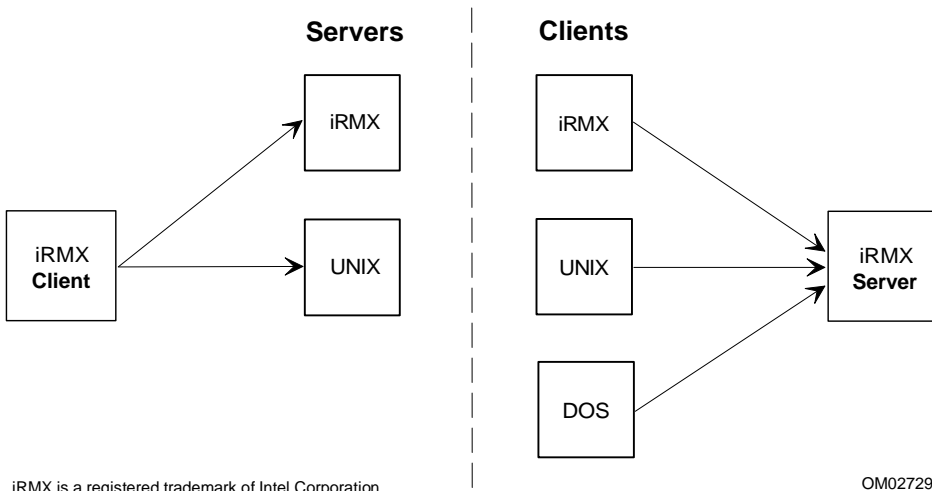
Figure 7-1. iRMX-NET Interoperability with other OpenNET Systems
