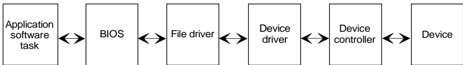
Figure 3-7. I/O Requests from the Application Go Through BIOS and Device Drivers
