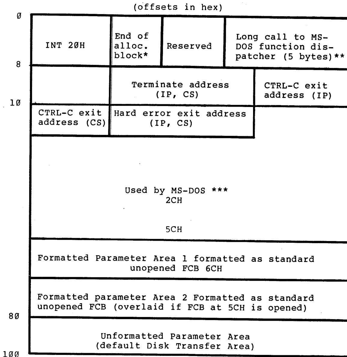
Figure 5. Program Segment Prefix
