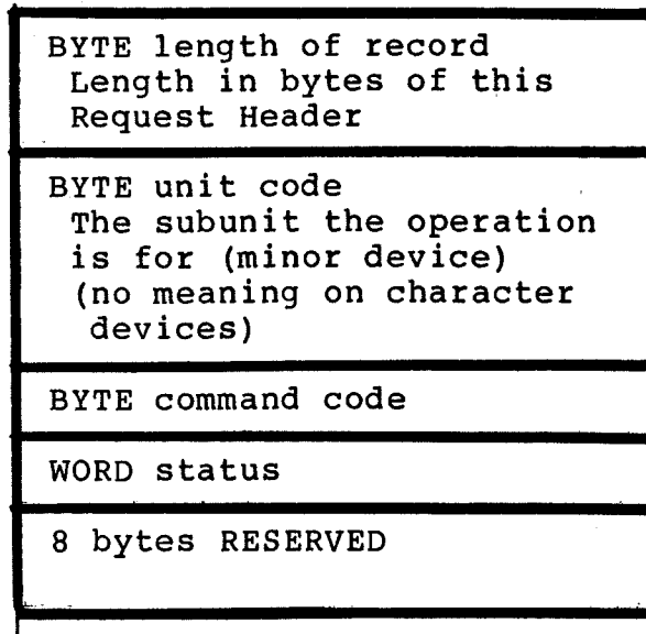
Figure 3. Request Header
