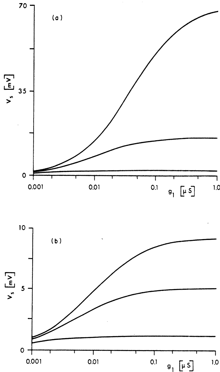
Figure 2 (a) Nonlinear saturation of the somatic voltage as a function of a steady state conductance input g_1 for three different cases: The synapse lies on the dendritic shaft directly below a proximal spine (top curve), the synapse is situated on the spine head of a proximal spine with the standard neck dimensions ( d_N = 0.1\mu m and l_N = 1.0\mu m ; middle curve) and the synapse lies on the spine head of a proximal spine with a stretched spine neck ( d_N = 0.05\mu m and l_N = 2.0\mu m ; lower curve). (b) Same as (a) except that the distal spine of figure 1 has been used (Notice the decrease in voltage scale).
