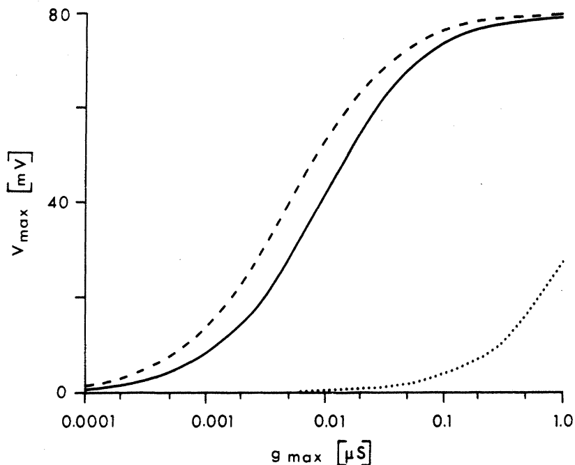
Figure 5 The maximum depolarization at the synapse, for a fast transient conductance input of peak amplitude g_{max} ( t_{peak} = 0.25msec and total duration 0.9msec ) at the distal spine of figure 1 (solid line) or at the dendritic shaft just below the spine (dotted line). The dashed line shows that a steady state conductance change yields essentially the same depolarization in the spine as the transient input; \tau_m = 8msec .
