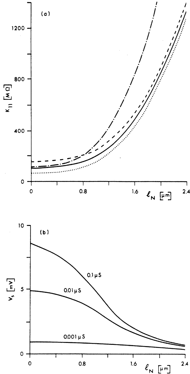
Figure 3 (a) The steady state input impedance \tilde{K}_{11}(0) = K_{11} (for the distal spine) as a function of the spine neck length and diameter calculated for different membrane parameters (the spine neck dimensions were changed in such a way as to leave the total neck surface area constant: d_N l_N = 0.1 \mu m^2 ). The solid curve is for R_m = 4000 \Omega cm^2 , the dotted one for R_m = 1000 \Omega cm^2 and the dashed curve for R_m = 16000 \Omega cm^2 ; while for these curves R_i is everywhere homogeneous with R_i = 70 \Omega cm ; for the dot-dashed curve R_m = 4000 \Omega cm^2 and R_i = 70 \Omega cm holds in the soma and dendrites but R_i has twice this value ( 140 \Omega cm ) for the cytoplasm of the spine. The corresponding transfer resistances to the soma are 12.75, 1.51, 39.25 and 12.75 M\Omega . (b) The somatic depolarization for the distal spine of figure 1 with changing spine neck dimensions (see (a)) for different inputs.
