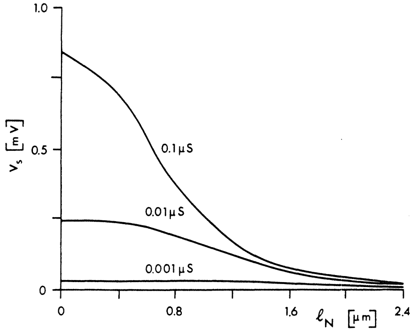
Figure 6 Somatic depolarization as a function of spine geometry and maximal amplitude of the transient conductance change for a distal spine. V_s was approximated by using K^{eff} for a conductance input with t_{peak} = 0.25 msec (see figure 3b).
