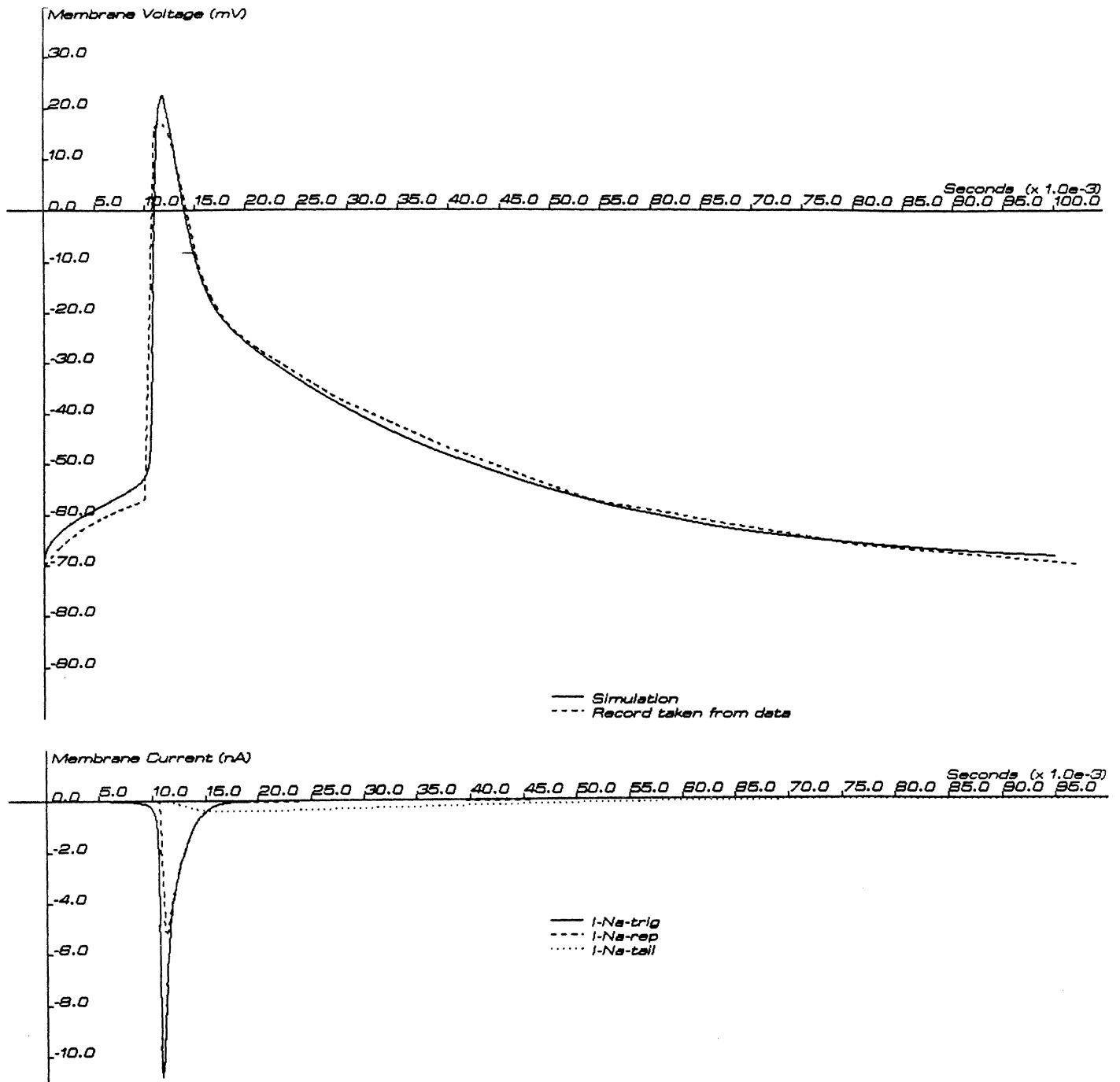
Figure 5.6: Current clamp simulation of Na^+ -only single spike. Spike stimulus - 0.78 nA. Top - Simulation of spike compared with record taken from data. Bottom - I_{Na-trig} , I_{Na-tail} , I_{Na-rep} currents during spike.
