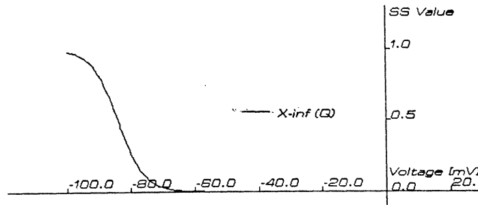
Figure 7.27: Steady-state curve ( x_\infty ) for x_Q .
