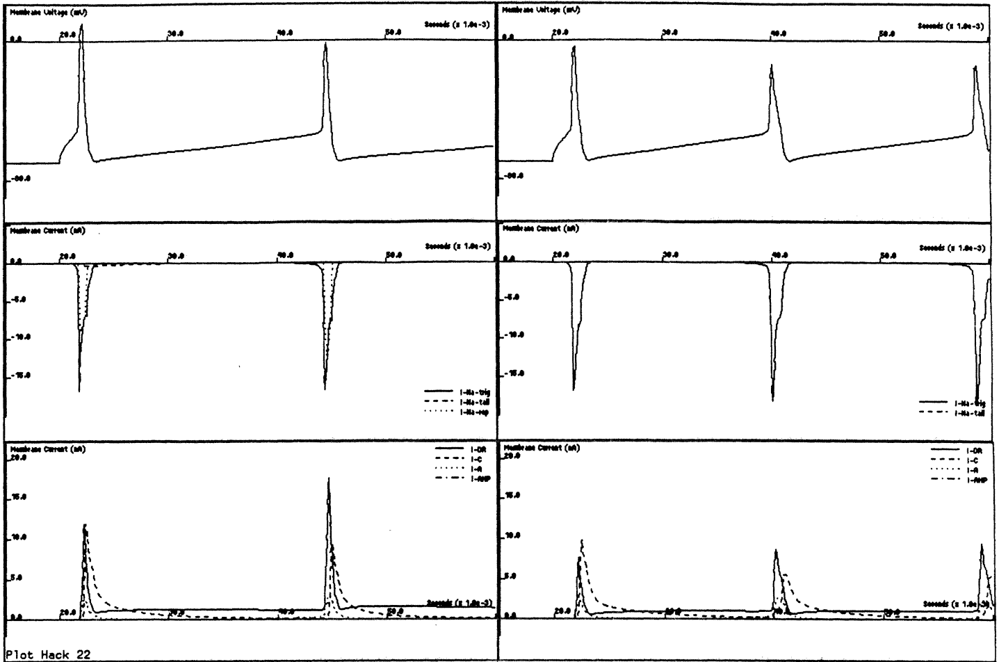
Figure 9.14: Comparison of initial spikes of spike train with and without I_{Na-cep} - Soma response and Na^+ and K^+ currents.
