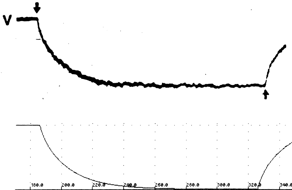
Figure 3.5: Typical response to current step ([7]) (top) and response to current step of model based on Brown et. al. parameters (bottom), where \rho = 1.2 , L = 0.95 , R_{in} = 39M\Omega , a_{soma} = 73\mu m , a = 3.0\mu m , and l = 1800\mu m .
