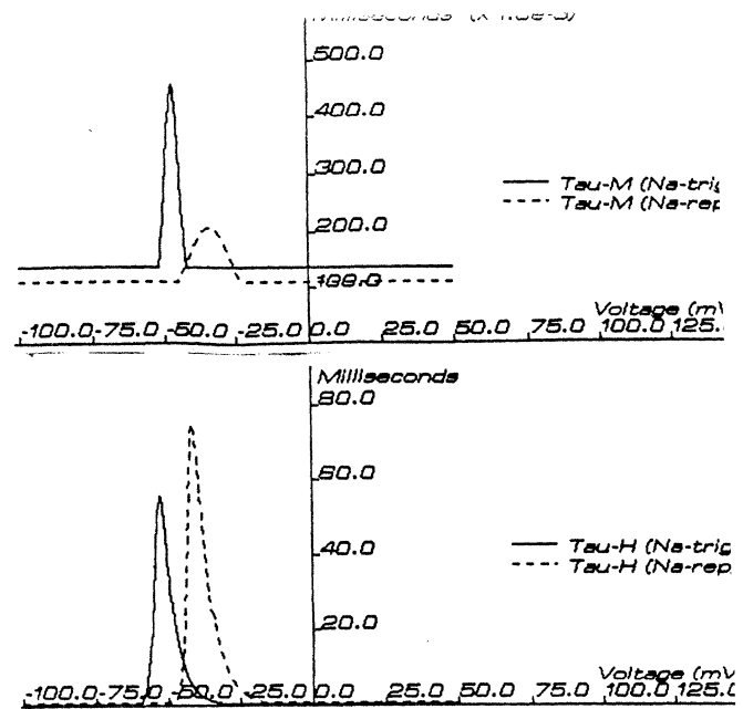
Figure 5.16: Time constant curves ( \tau_m and \tau_h ) for squid axon I_{Na} and the hippocampal I_{Na-trig} and I_{Na-rep} .
