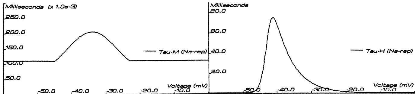
Figure 5.12: Time constant curves ( \tau_m and \tau_h ) for m_{Na-rep} and h_{Na-rep} .
