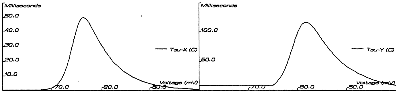
Figure 7.14: Time constant curves ( \tau_x and \tau_y ) for x_C and y_C .
