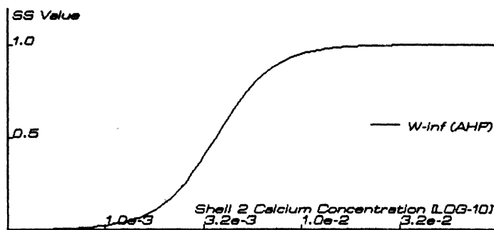
Figure 7.22: Relation between w_x and [Ca^{2+}]_{shell.2} for w_{AHP} .
