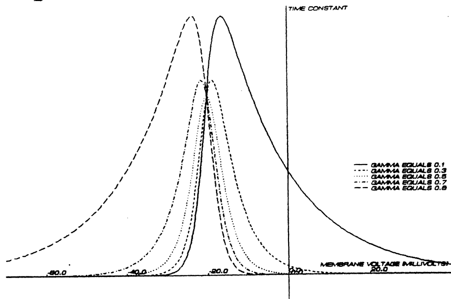
Figure 4.7: Effect of the relative position, \gamma , of the transition state within the membrane for the gating particle, x , on the \tau_s curve. z = 16 and V_{\frac{1}{2}} = -20mV . The time scale is arbitrary, as in Figure x. \tau_0 is set to 0.
