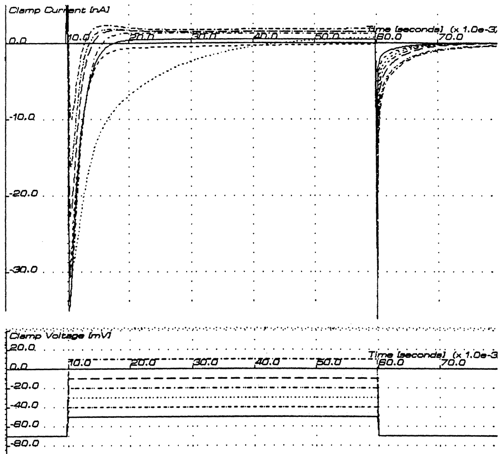
Figure 8.2: Voltage clamp simulations in which all currents have been blocked except for the Na^+ currents.
