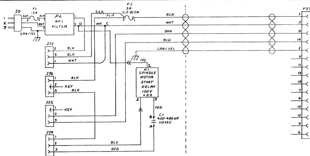
AC DISTRIBUTION BOX 100 V-130V
