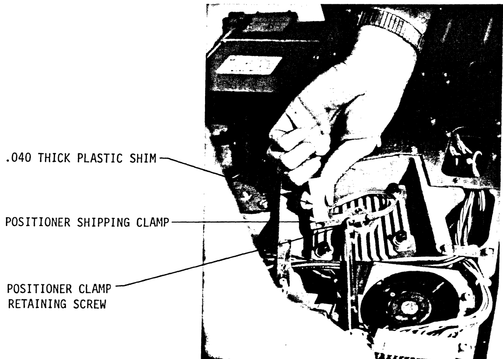
Figure 5-31 Shimming Shipping Clamp Arm
