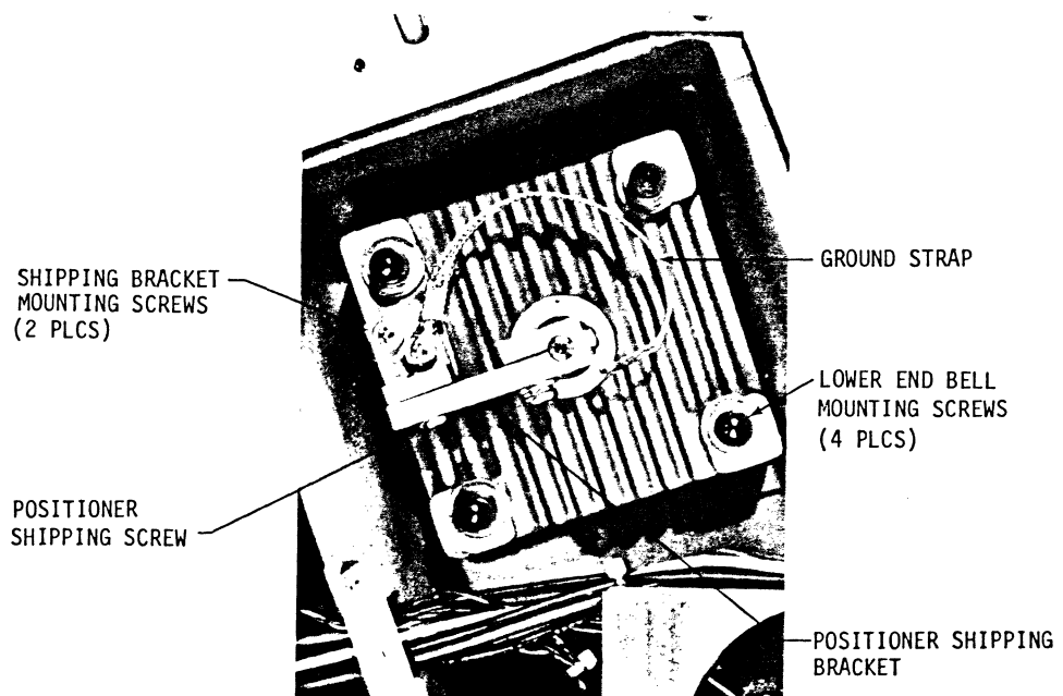
Figure 5-27 Positioner Motor Assembly
