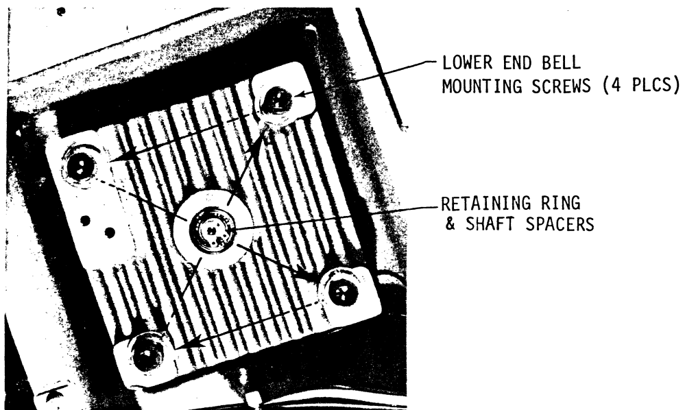
Figure 5-28 Positioner Motor (Retaining Ring)
