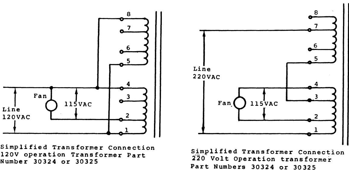
Figure 4-3 Transformer Primary Connections
