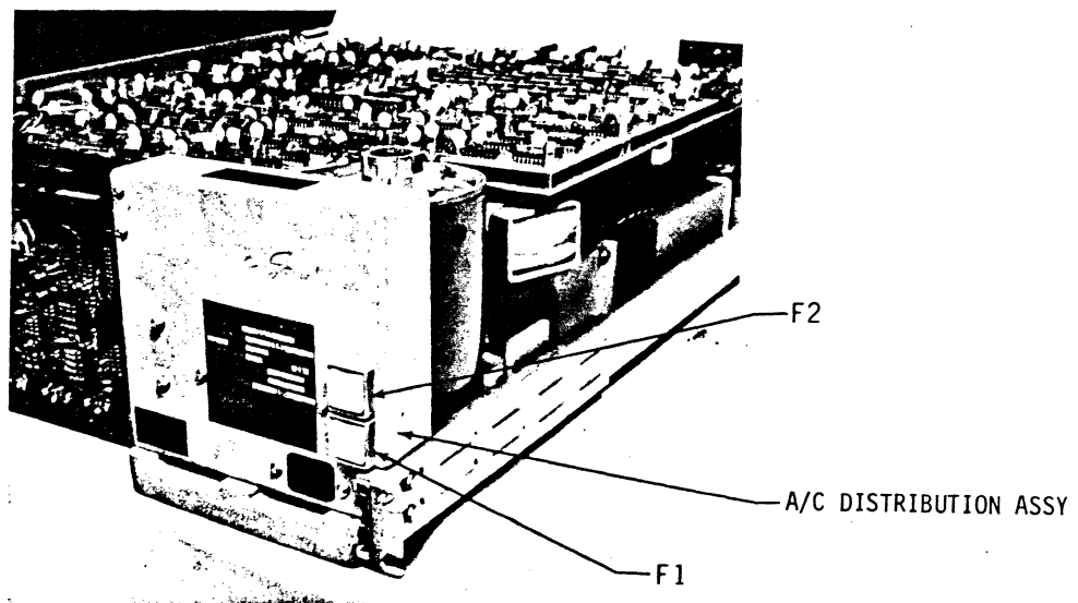
Figure 5-34 AC Distribution Assembly
