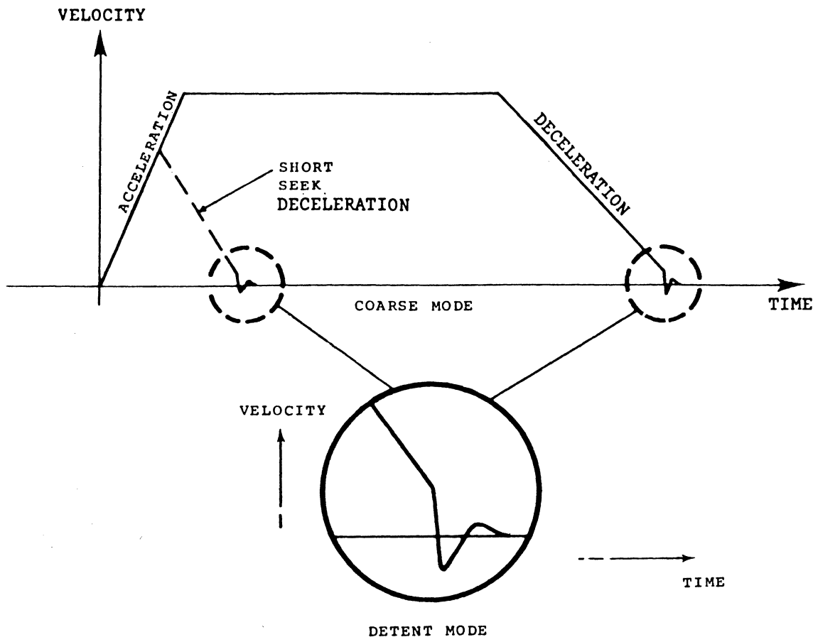
Figure 4-6 Positioner Motion During Seek
