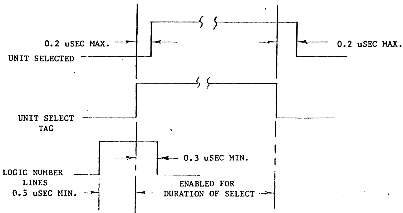
FIGURE 3-2 LOGIC NUMBER SELECT CODE AND TIMING DIAGRAM
