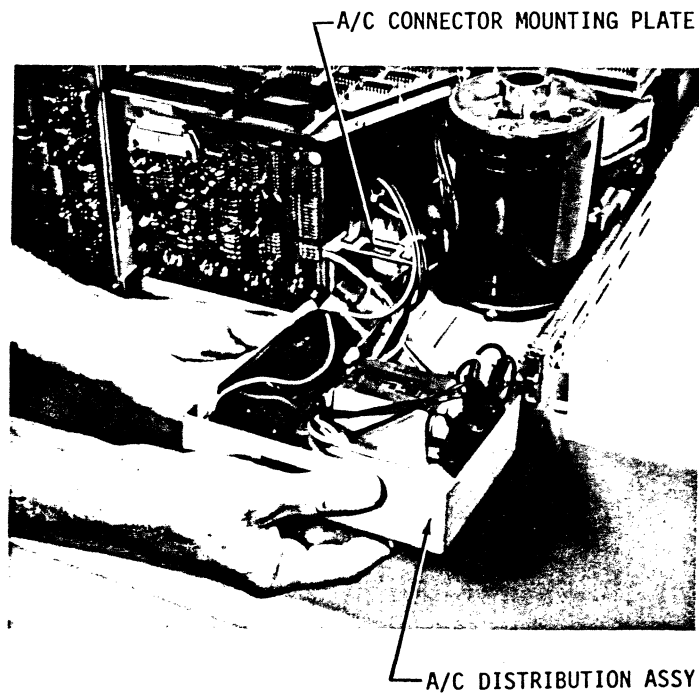
Figure 5-36 AC Distribution Assembly in Repair Position
