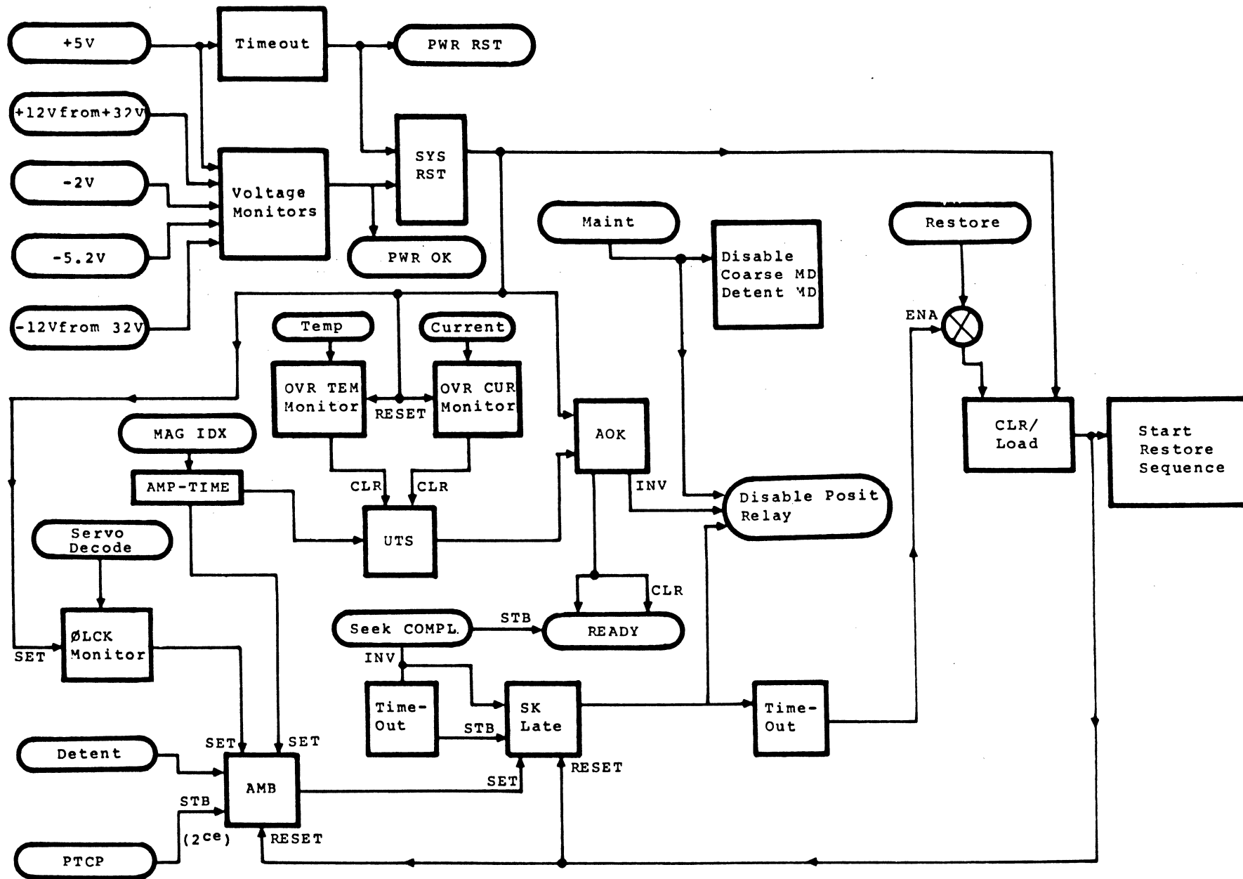
Figure 4-21 Fault Logic
