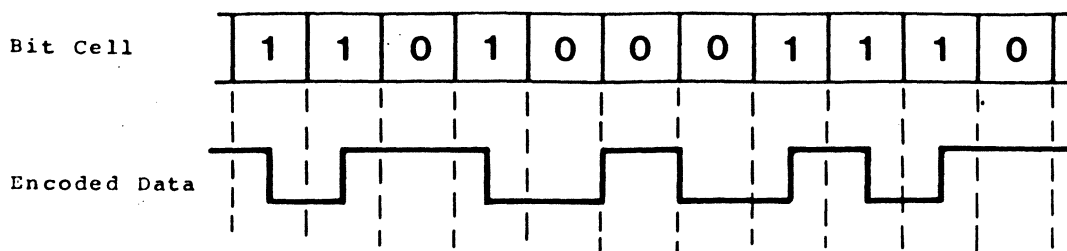
Figure 4-27 MFM Encoding
