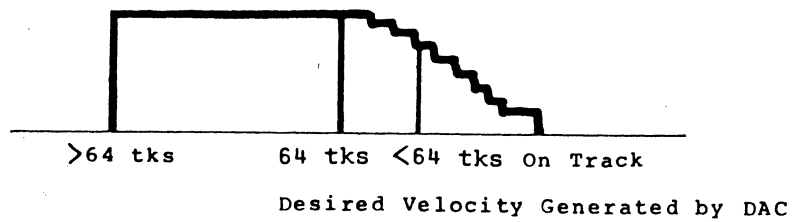
Figure 4-18 Desired Velocity Generated by DAC
