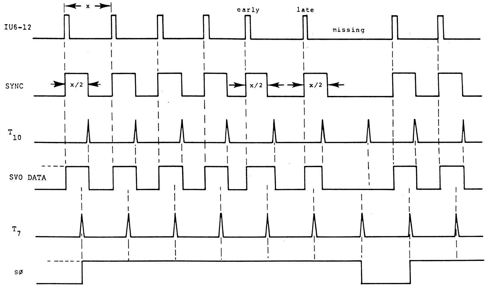
Figure 4-10 Phase Lock Timing
