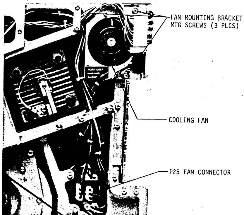
Figure 5-33 Cooling Fan Assembly
