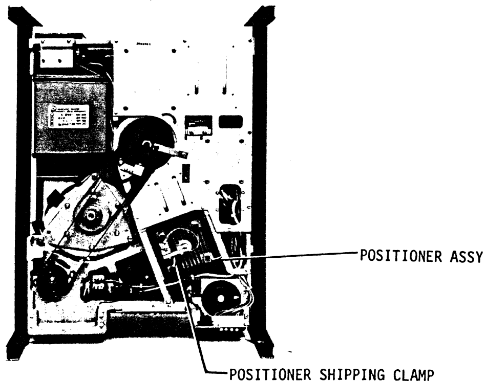
Figure 5-26 Positioner Removal (Machine Orientation)
