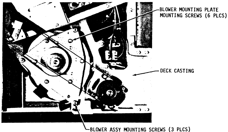
Figure 5-21 Blower Assembly
