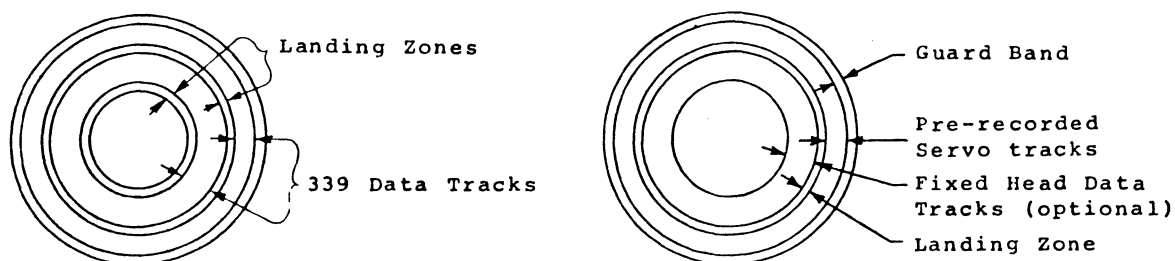
Figure 4-4 Disc Servo and Data Locations
