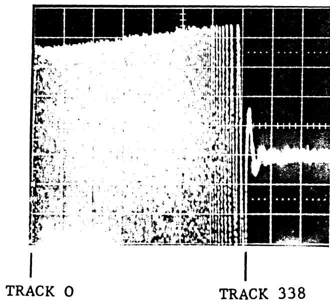
FIGURE 5-10 SERVO DEMODULATED SIGNAL (TP-21)
