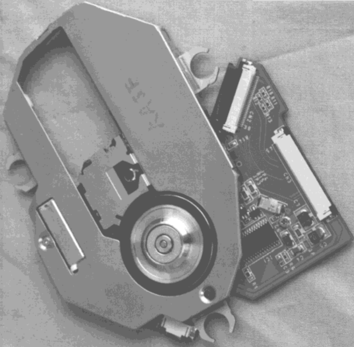
Fig.6 - Pickup Module (PCB Soldering Side) FCC ID:BBP7040A RICOH Co.,Ltd,
