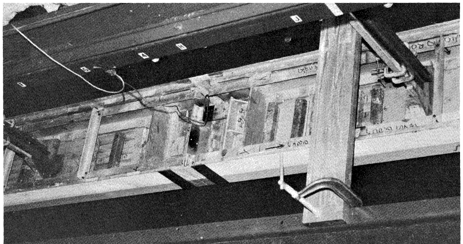
Figure 2b. Sensors on the midsection of the model pick up its bending moment. Dr. Armin Troesch is making some adjustments to the instrumentation.
