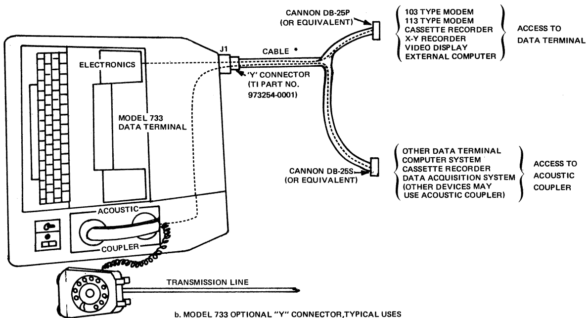
b. MODEL 733 OPTIONAL "Y" CONNECTOR, TYPICAL USES
