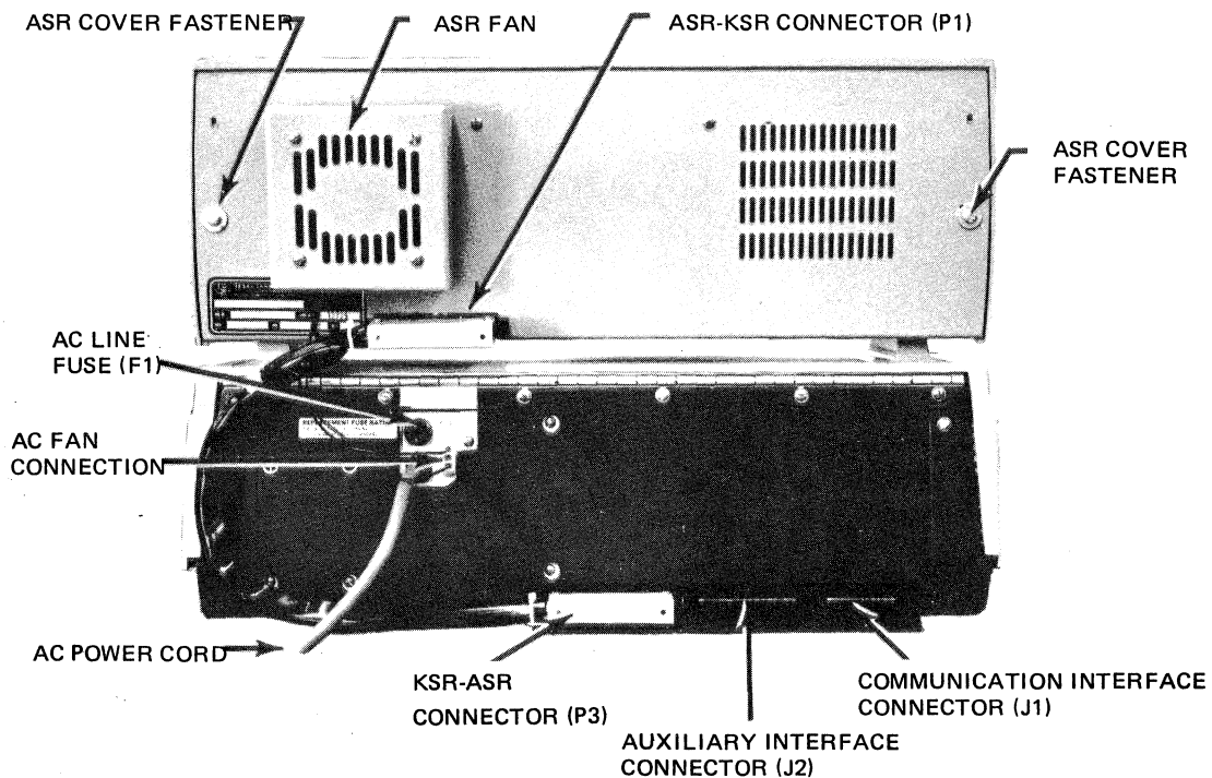
FIGURE 2-4. ASR/KSR DATA TERMINAL EXTERNAL CONNECTIONS (REAR VIEW)
