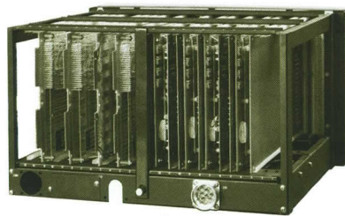
16K Memory and I/O
