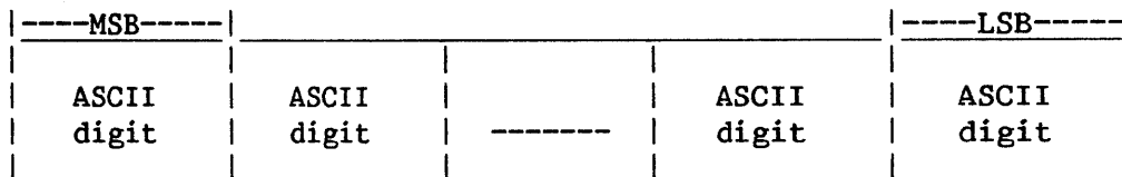
Figure 3-4. External Decimal Number Format
