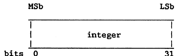
Figure 3-1. Fixed-Point Fullword Data Format
