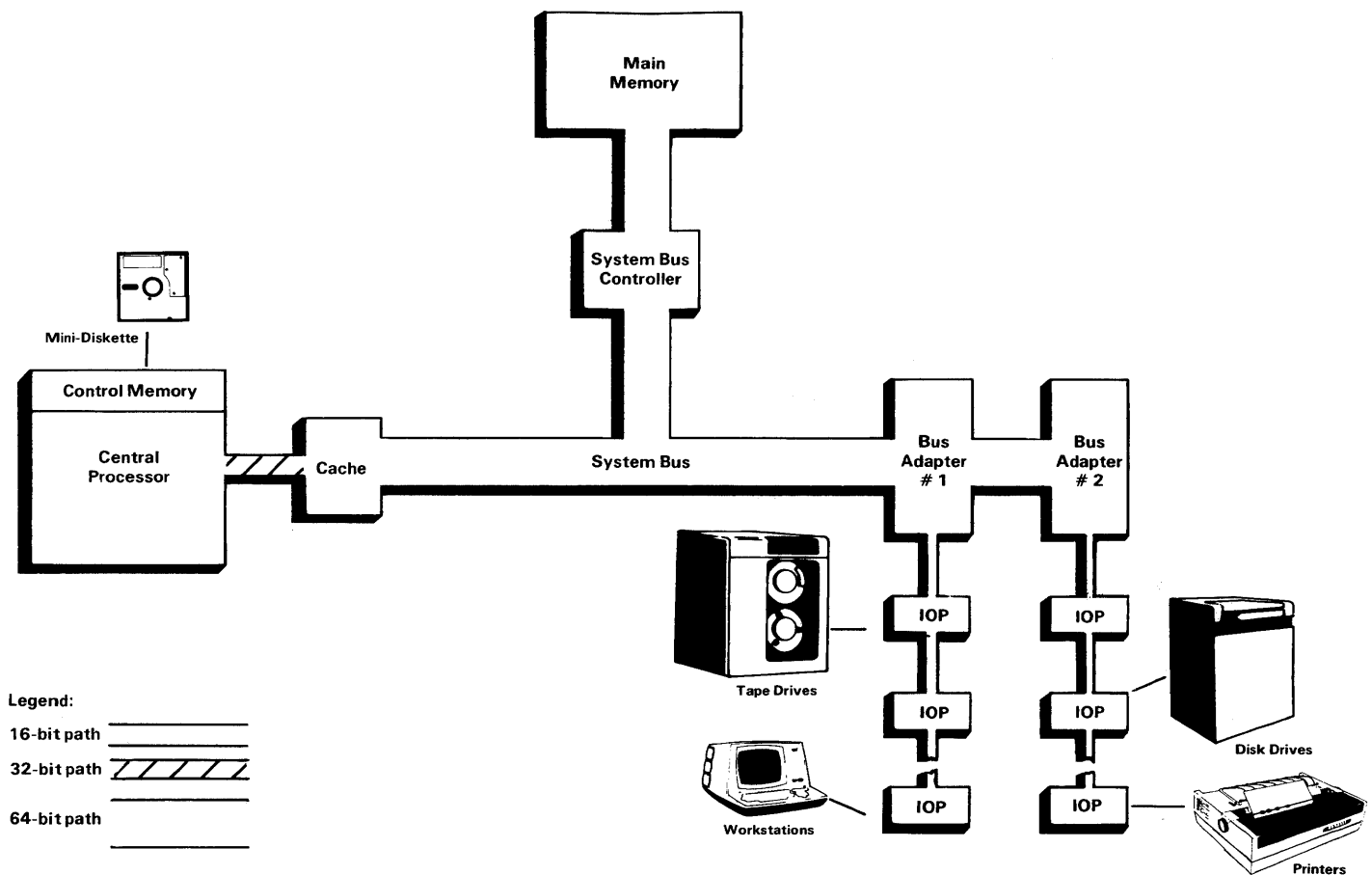
Figure 1-3. VS100 Architecture
