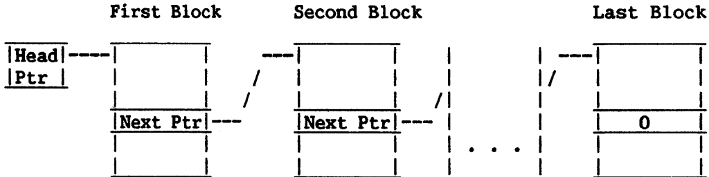
Figure 3-8. LIFO List
