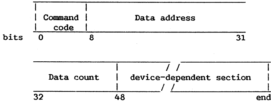
Figure 8-8. I/O Command Word (IOCW) Format
