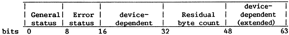
Figure 8-9. IOSW Format
