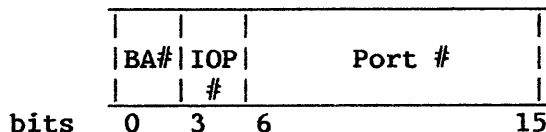
Figure 8-1. I/O Device Address (IODA)
