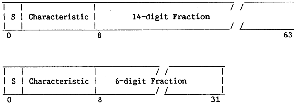
Figure 3-5. Long and Short Floating-Point Numbers
