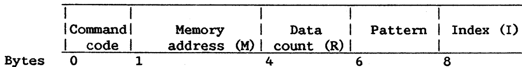
Figure 8-11. IOCW Format for Diagnostic Commands
