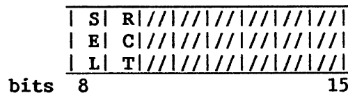
Figure 1. Format of Operand M2 in RRCB Instruction for Reference and Change Table
