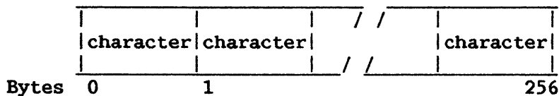
Figure 3-7. Variable-Length Logical Operand (up to 256 bytes)
