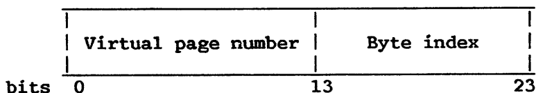
Figure 4-3. Virtual Address Format
