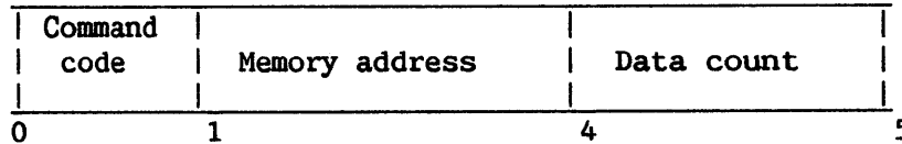
Figure 8-4. IOCW Format for Microcode Commands
