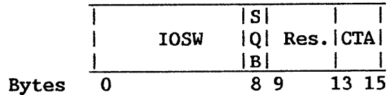
Figure 8-2. DA Status Table (DAST) for the VS25
