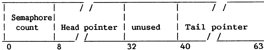
Figure 3-10. Semaphore
