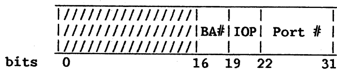
Figure 8-7. R1 Format for SIO, CIO, and HIO Instructions
