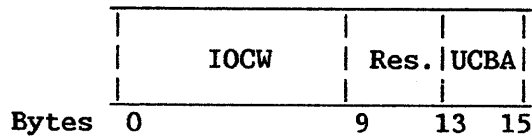
Figure 8-4. I/O Command Table (IOCT)
