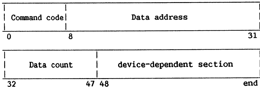
Figure 8-2. I/O Command Word Format
