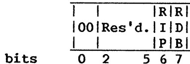
Figure 8-5. Status Qualifier Byte (SQB)
