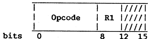
Figure 8-6. SIO, CIO, and HIO Instruction Format
