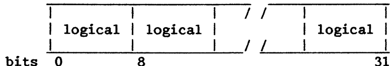
Figure 3-6. Fixed-Length Logical Operand (one to four bytes)
