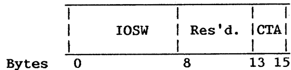
Figure 8-3. IOP Status Table (IOPST) for the VS100
