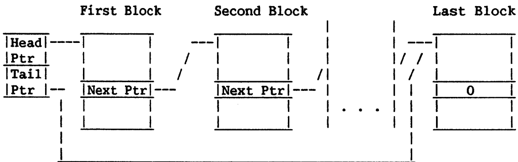
Figure 3-9. FIFO List
