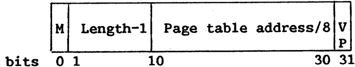
Figure 4-5. Segment Control Register (SCR) Entry Format
