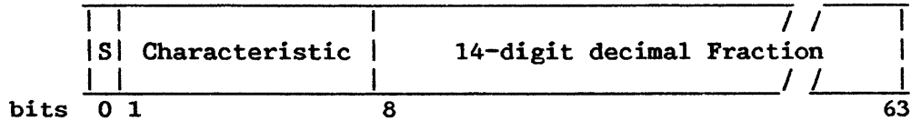
Figure 3-5.1. Decimal Floating-Point Number Format
