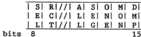
Figure 2. Format of Operand M2 in RRCB Instruction for VS25 and VS100 T-RAM Monitor Area
