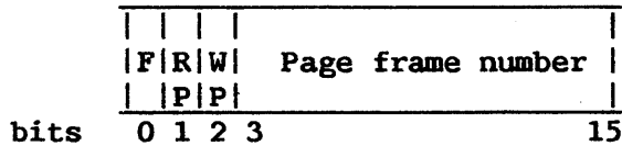
Figure 4-4. Main Memory Page Table Entry Format
