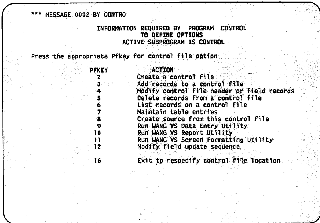
Figure 2-3. Control File Options Screen
