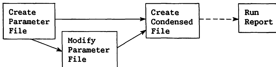
Figure 7-1. CONDENSE Processing
