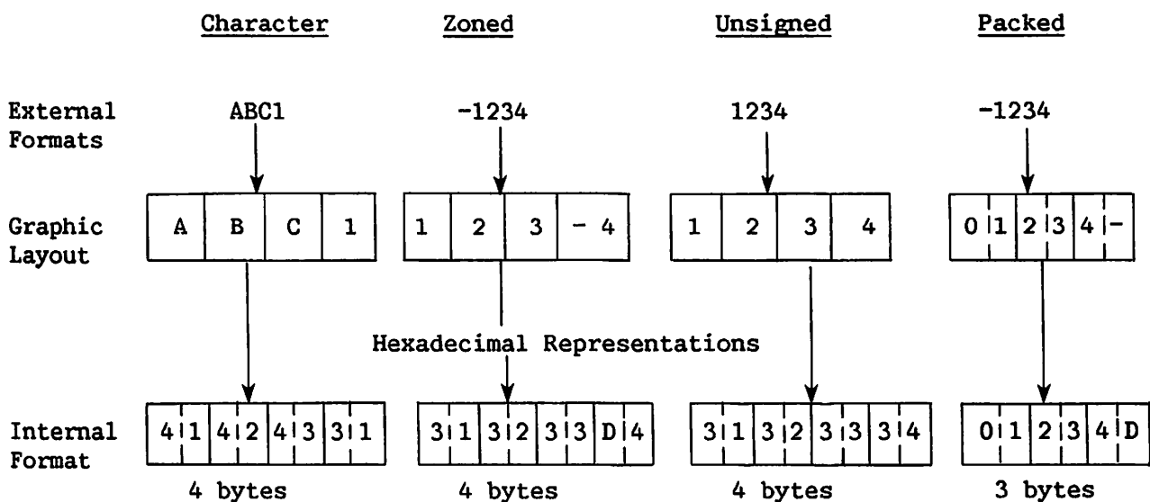
Figure 8-1. Data Representation
