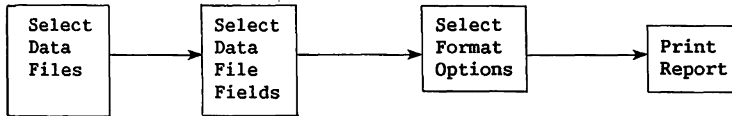
Figure 5-1. REPORT Processing
