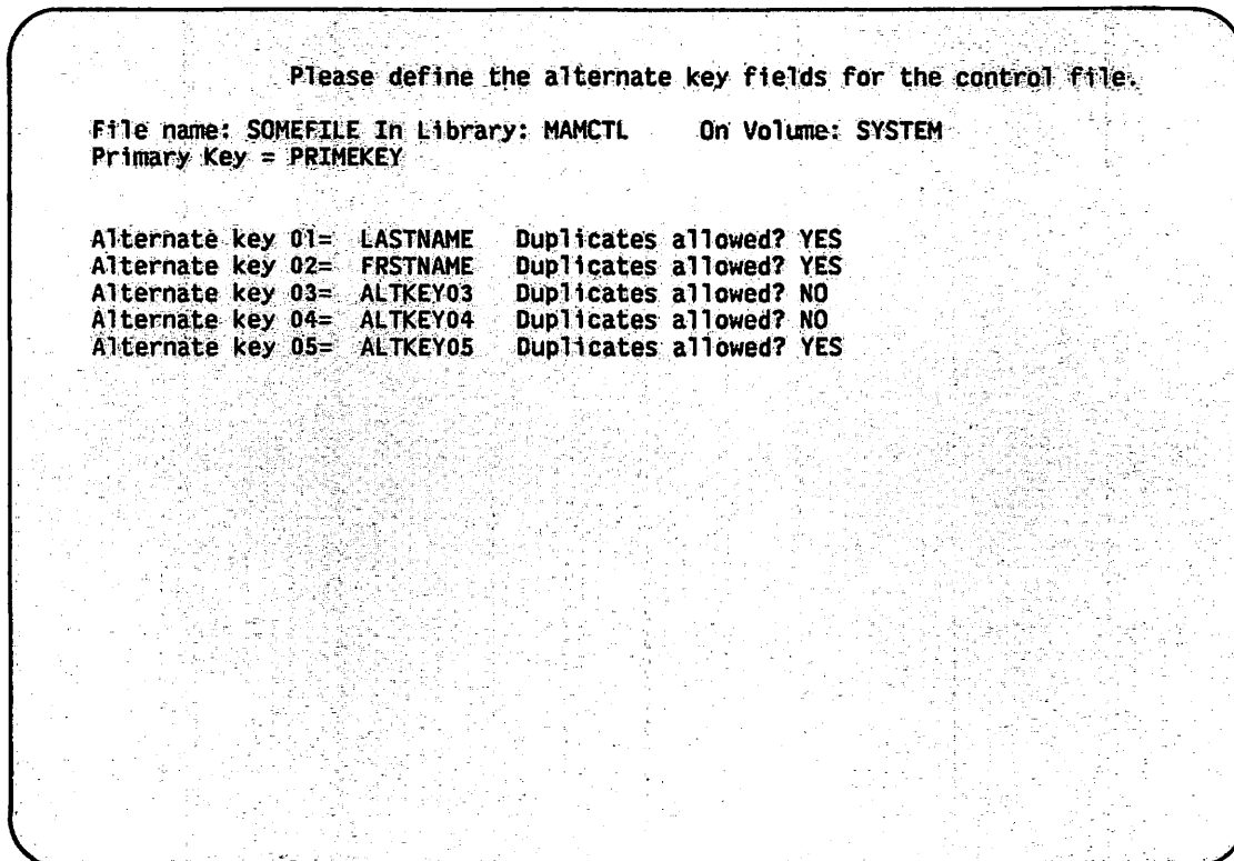
Figure 2-5. Alternate Key Fields Definition Screen
