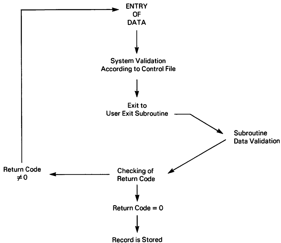
Figure 2-11. Running a Linked Data Entry Program
