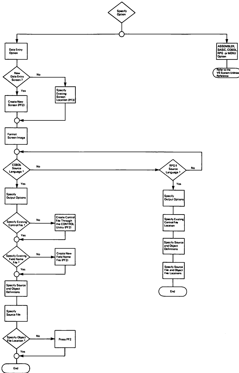
Figure 4-1. EZFORMAT Processing
