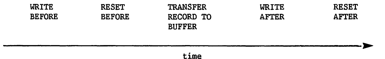
Figure 7-2. Relative Processing of WRITE and RESET
