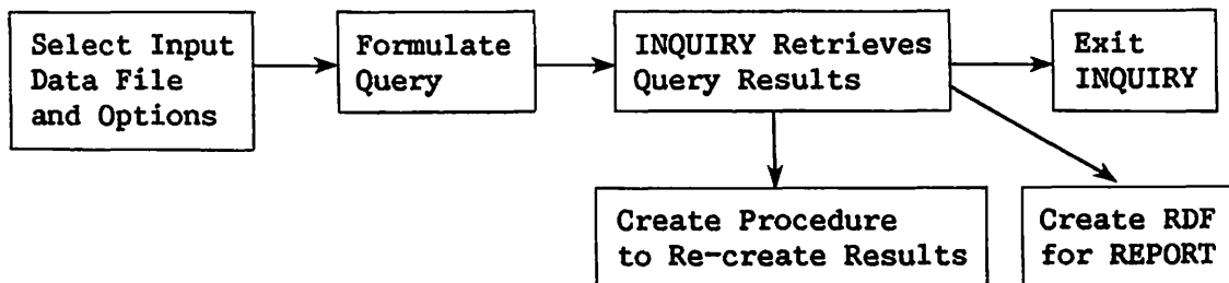
Figure 6-1. INQUIRY Processing
