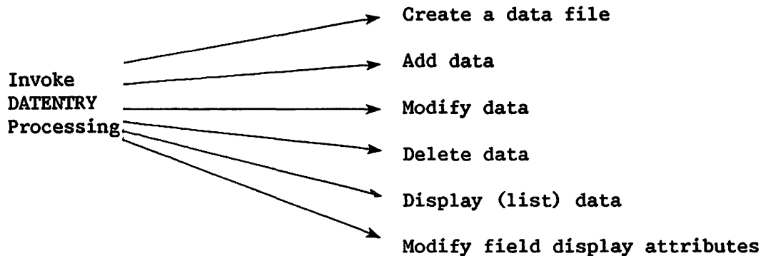
Figure 3-1. DATENTRY Processing
